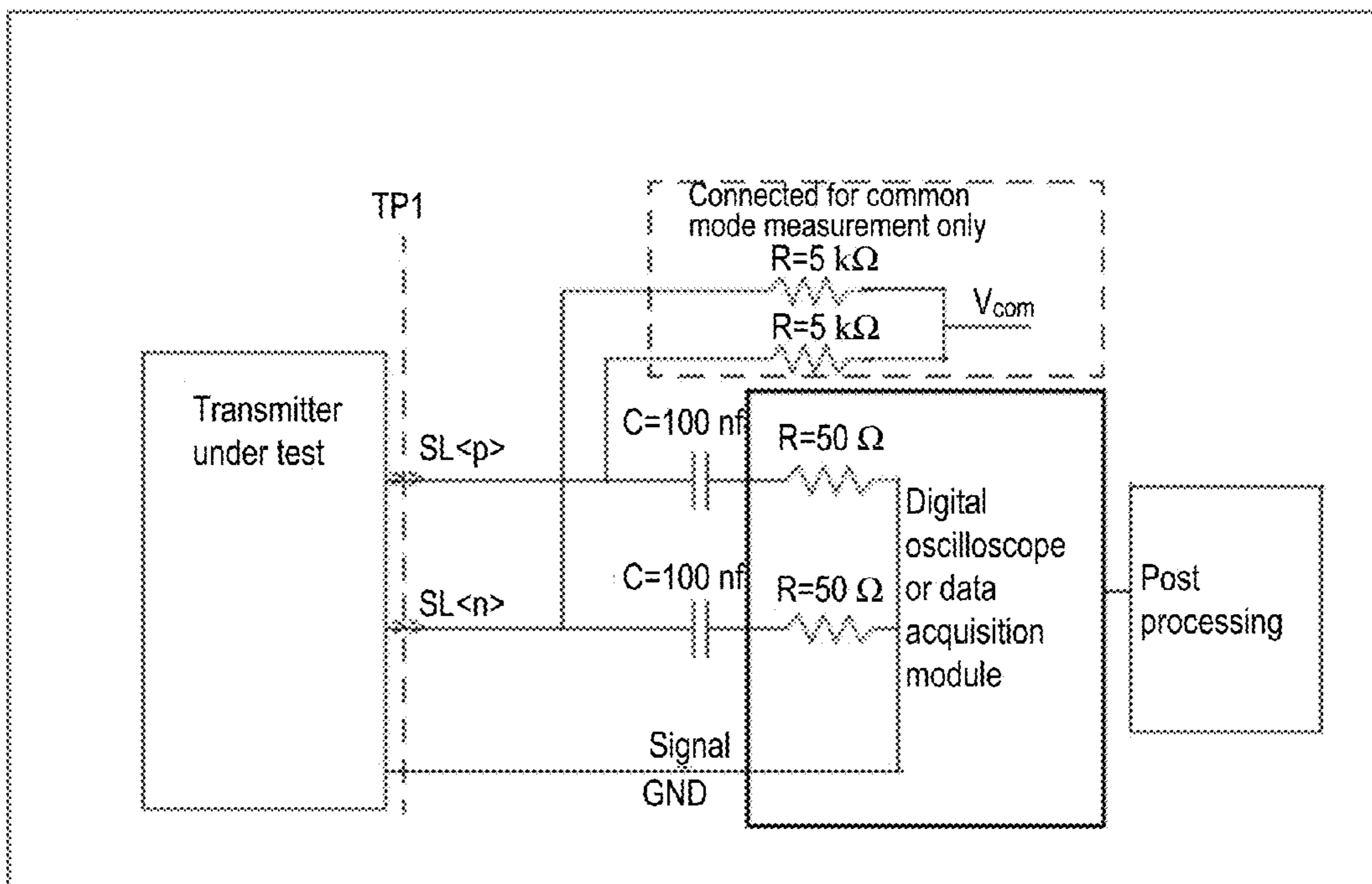
Fig. 1 (Prior Art)
