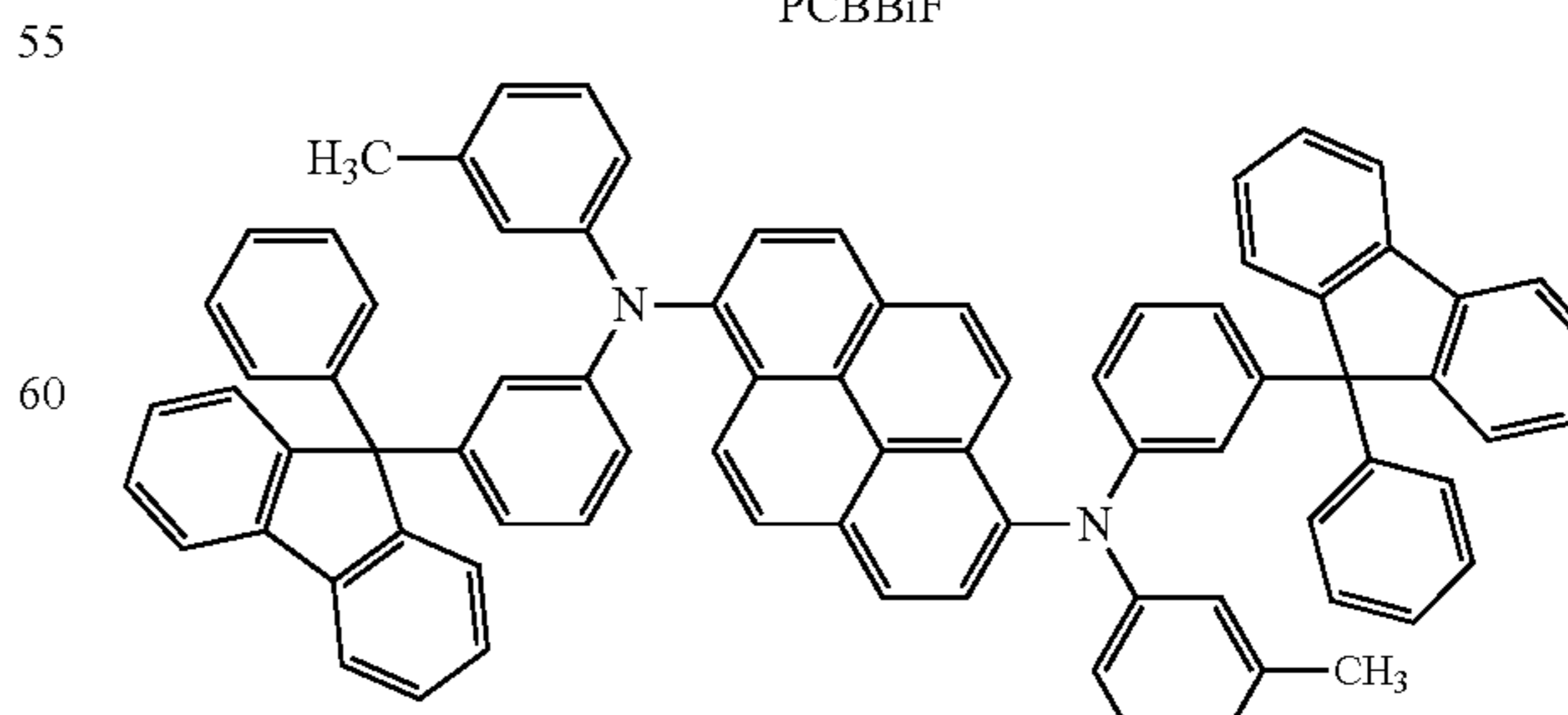
1,6mMemFLPAPm
