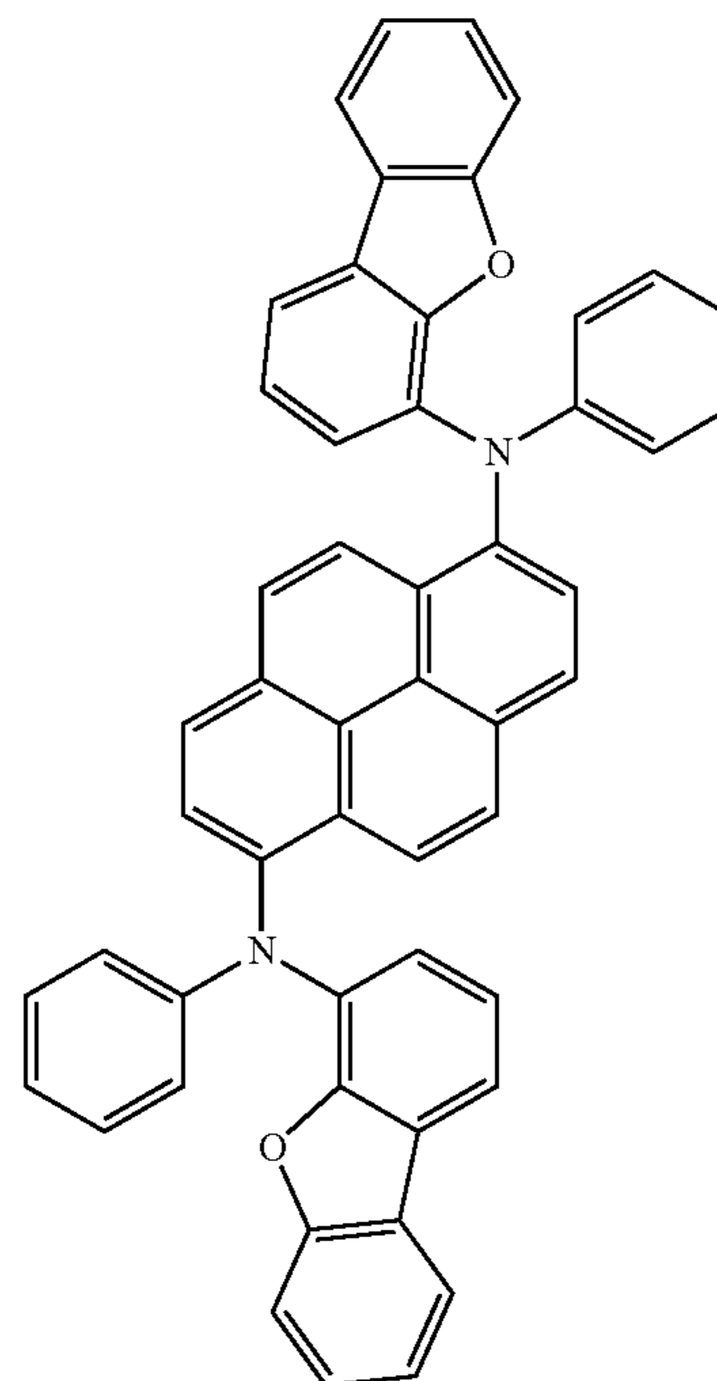
1,6FrAPrn-II
