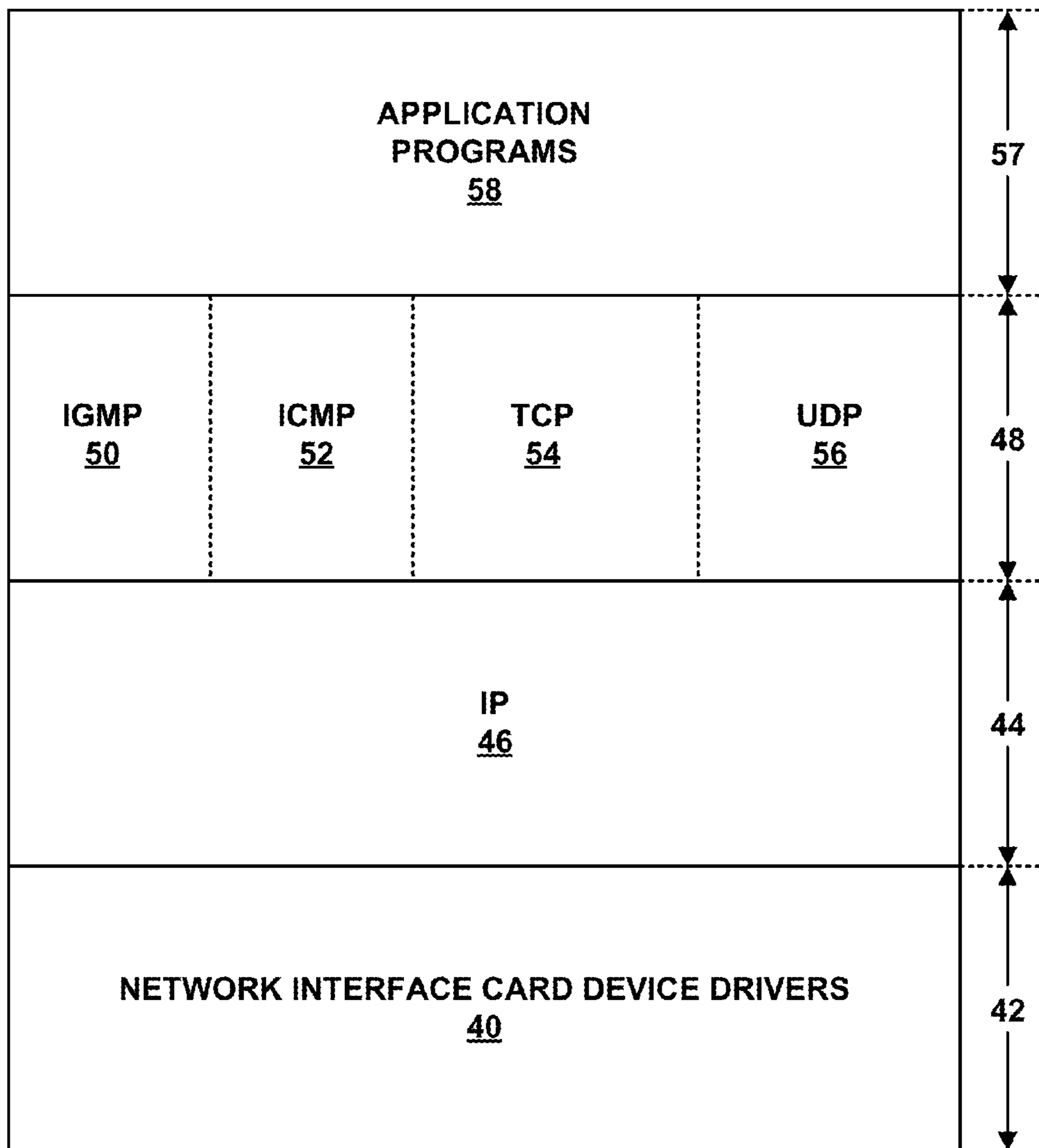
FIG. 3 PROTOCOL STACK
