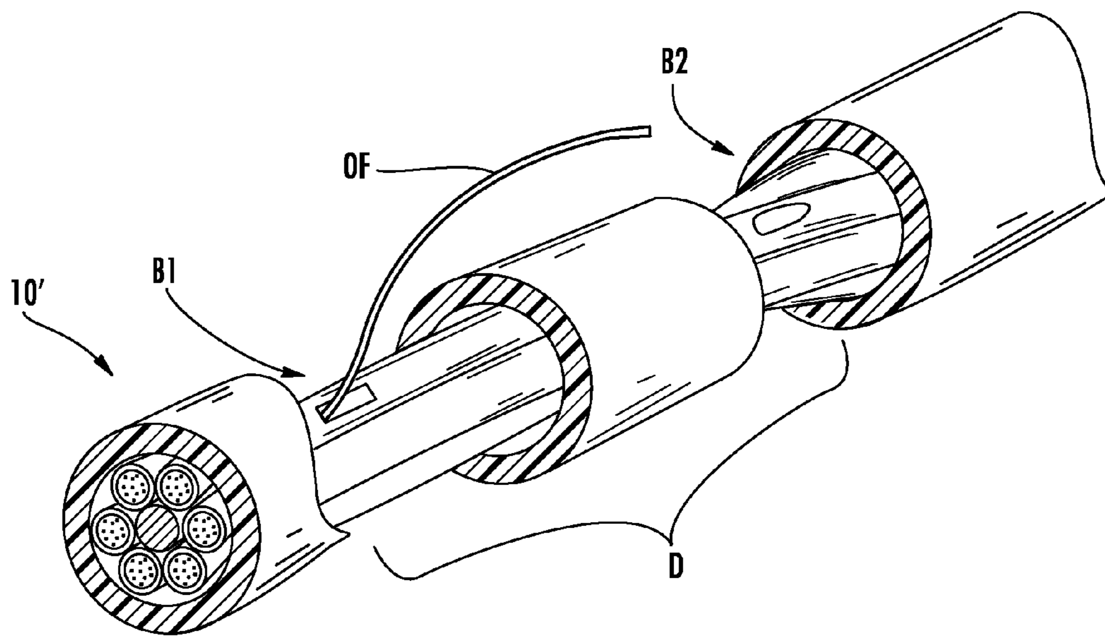
FIG. 2 (PRIOR ART)
