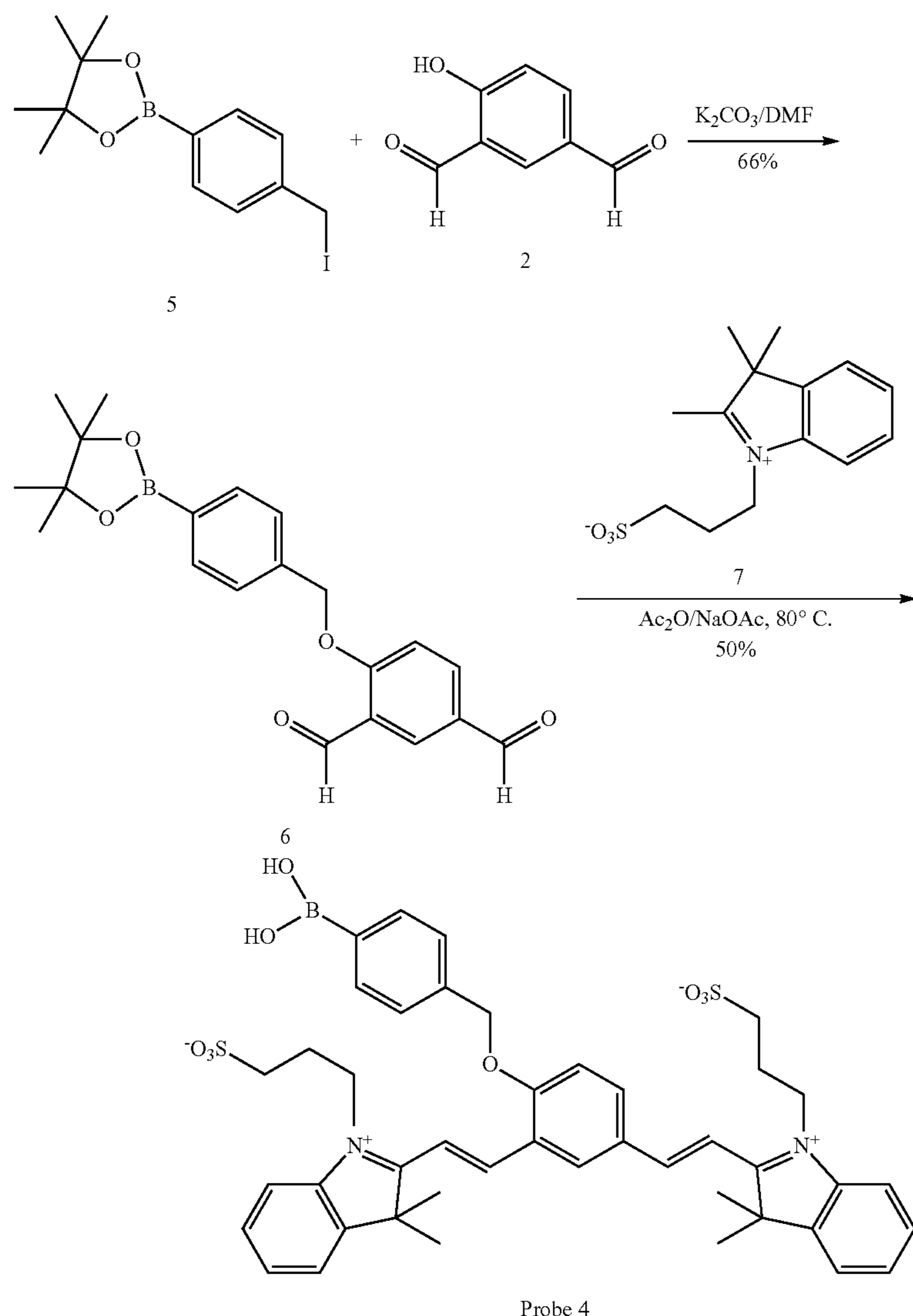
Scheme 7
