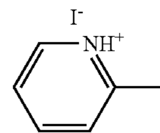
Picolinium iodide
