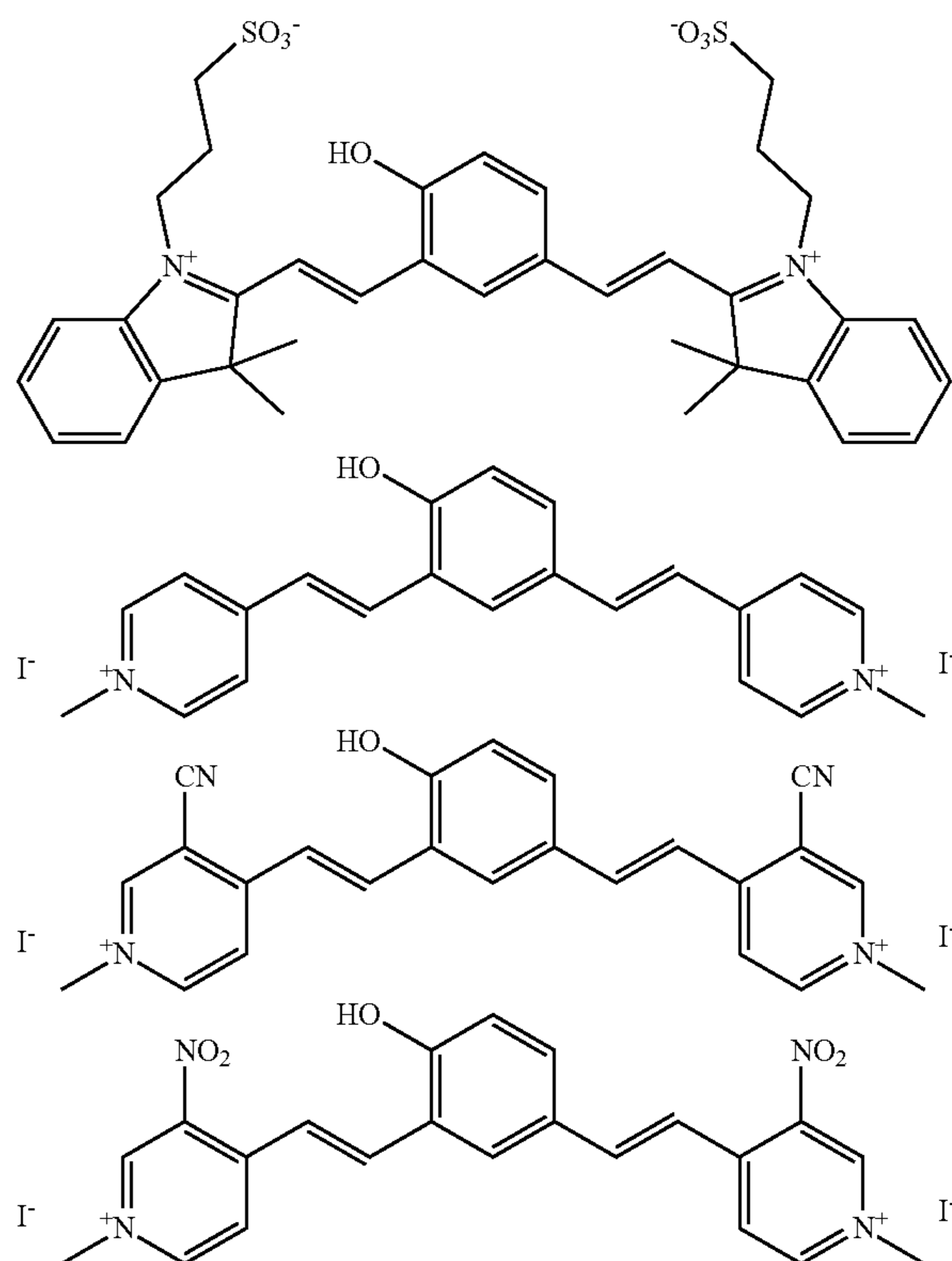
Formula IIIA
