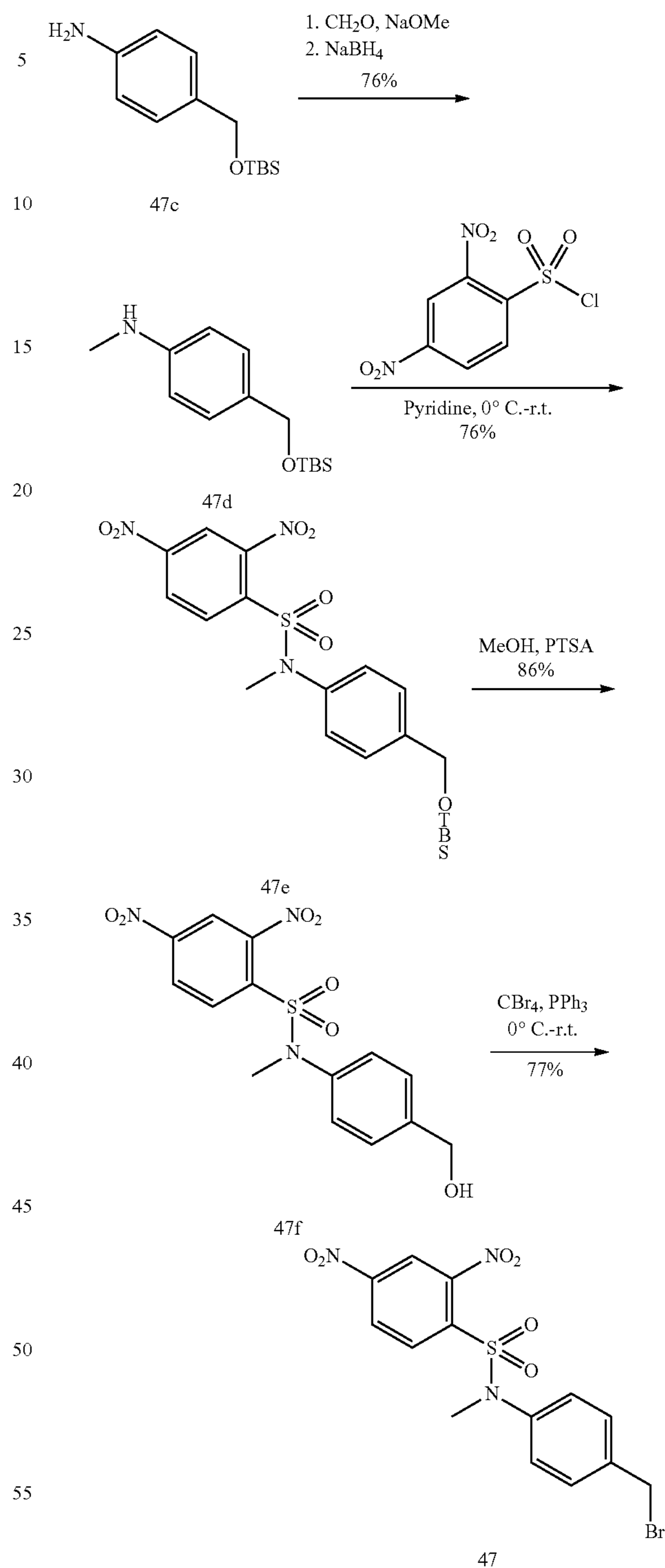
Scheme 9
