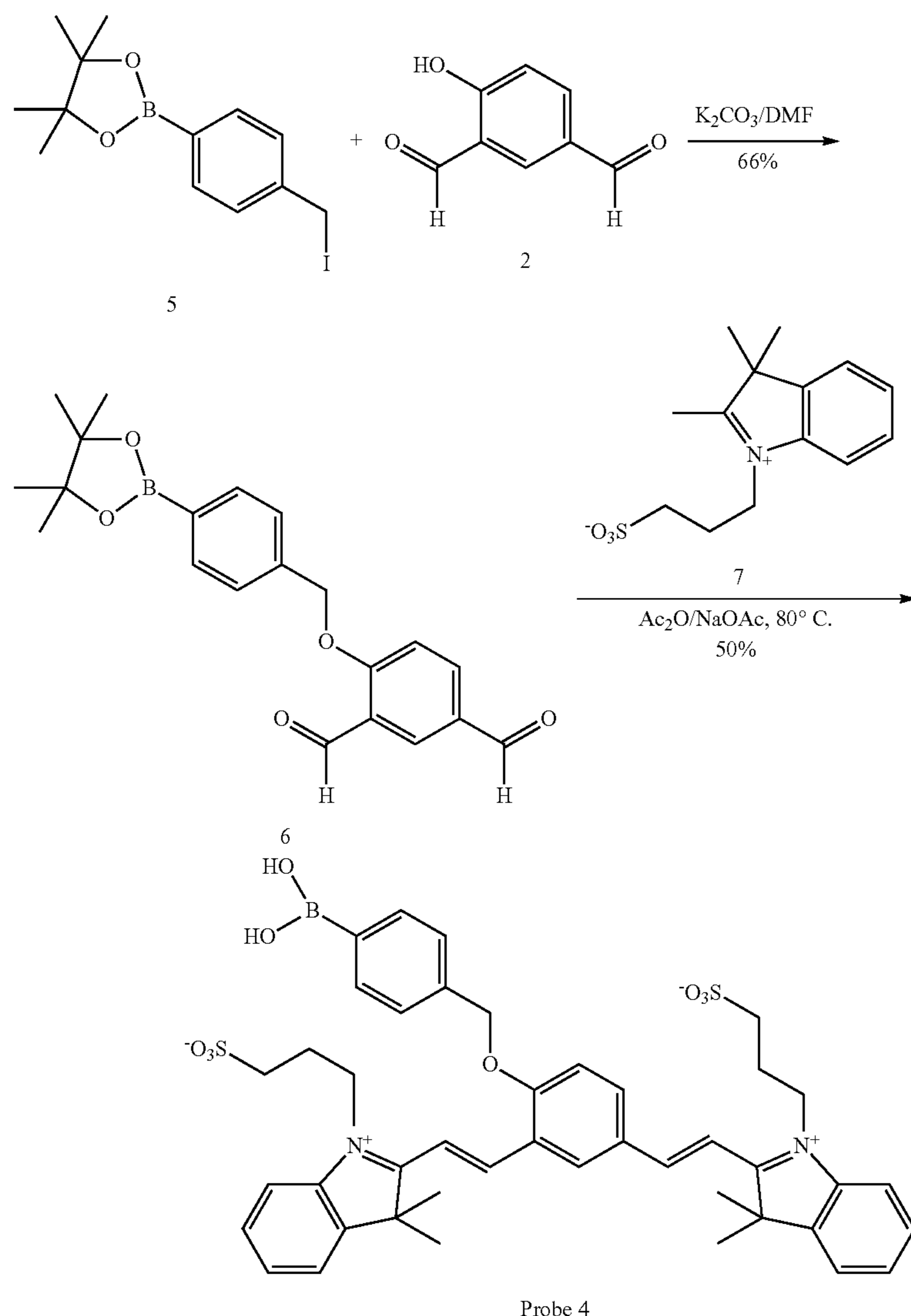
Scheme 7
