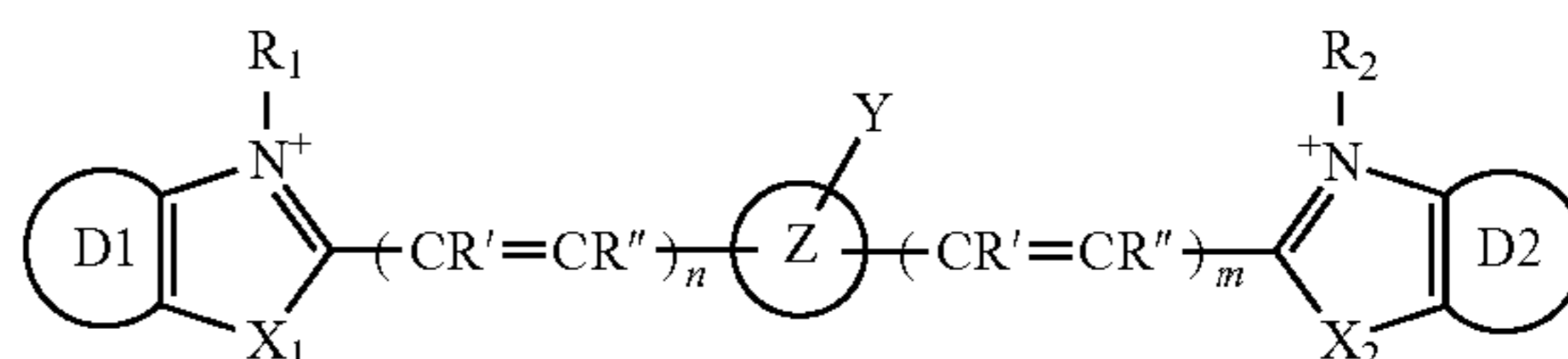
Formula IIIB
