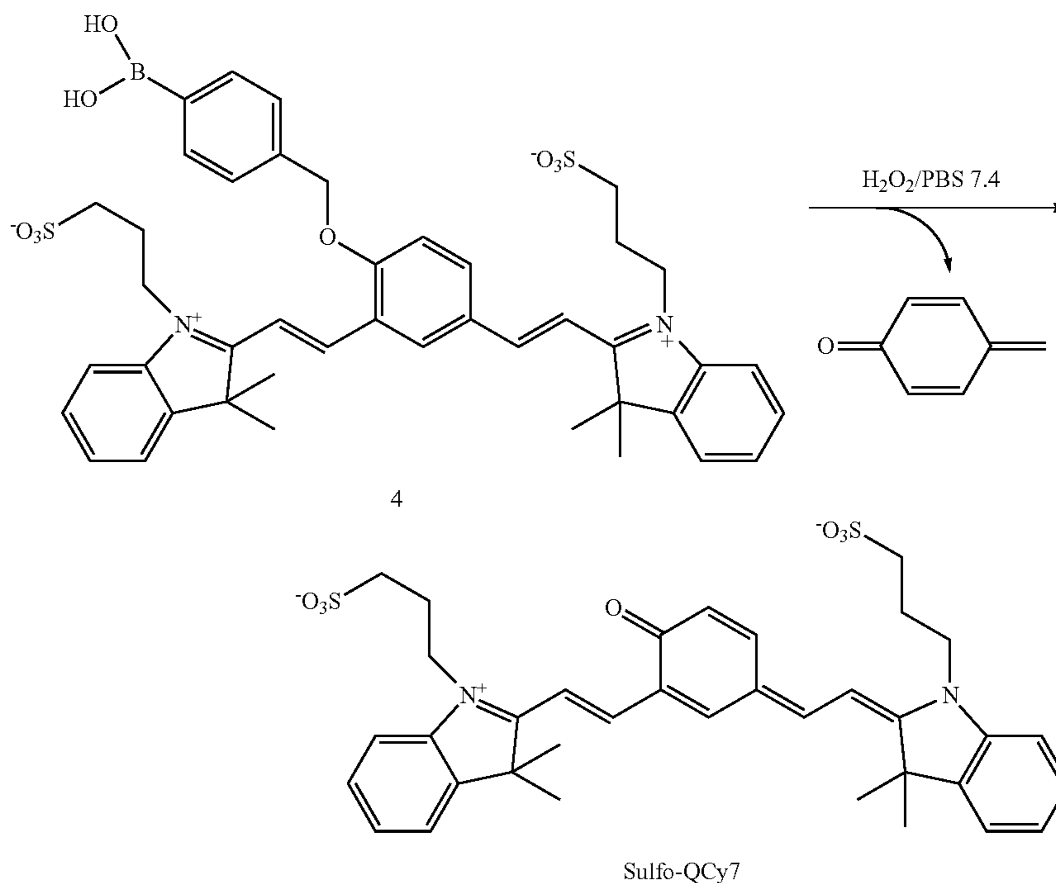
Scheme 6
