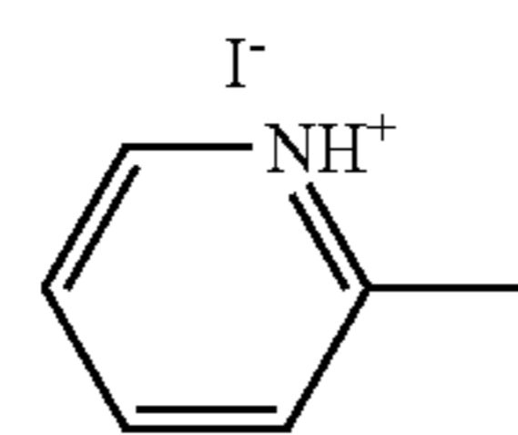
Picolinium iodide
