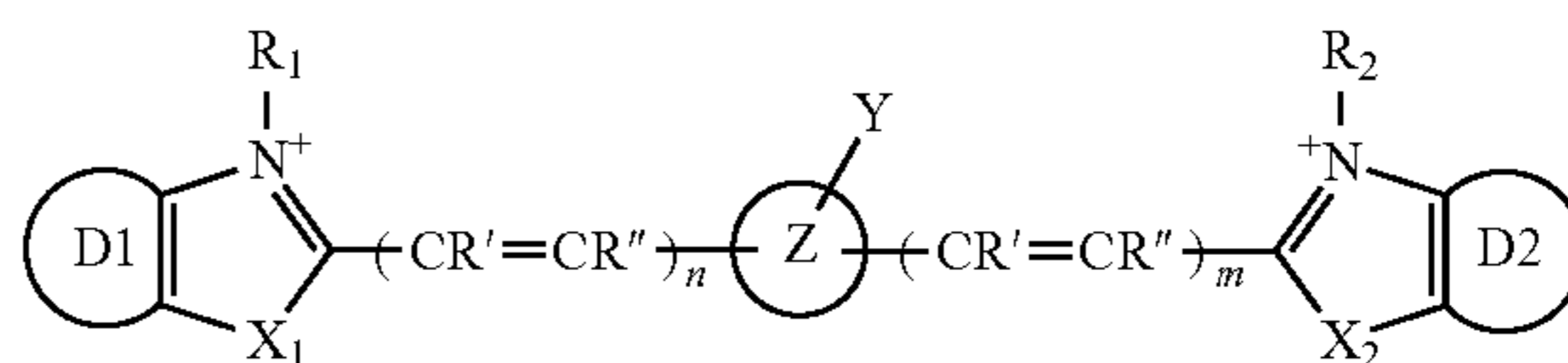
Formula IIIB
