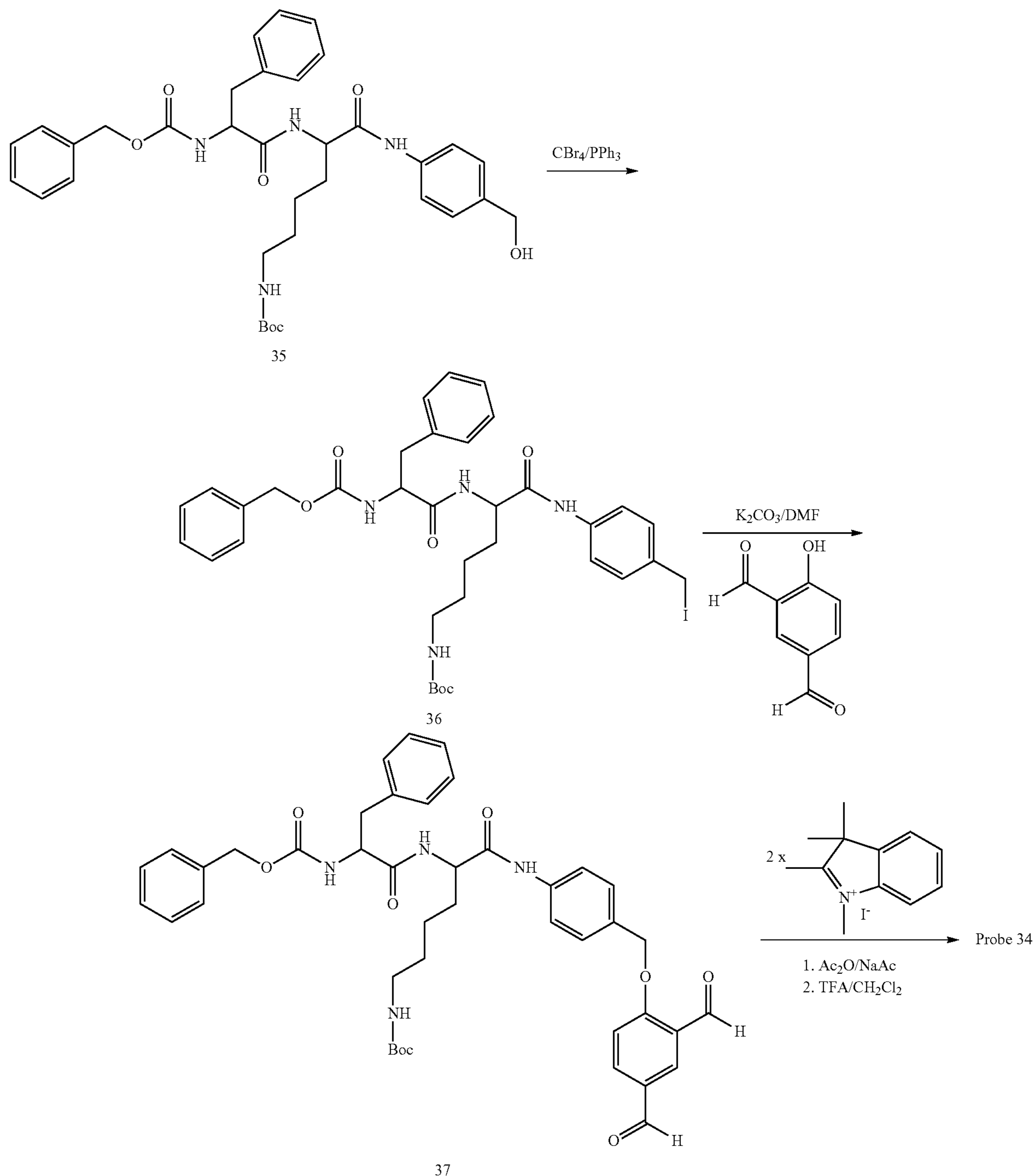
Scheme 8
