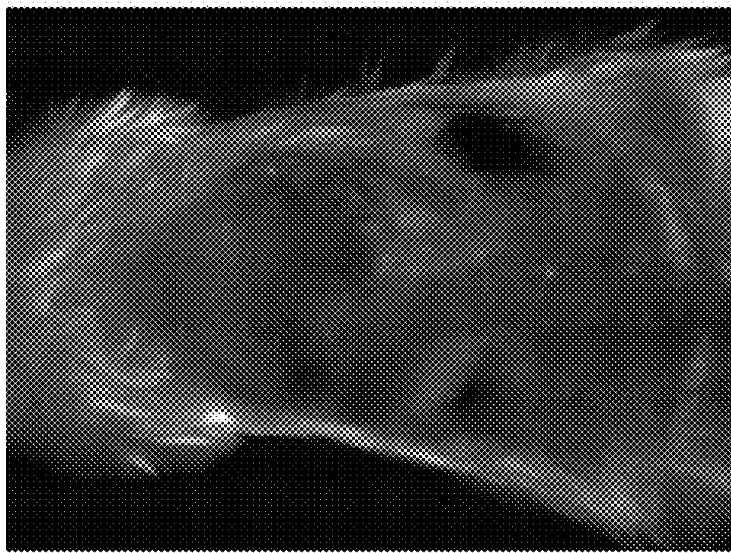
Probe 4 (1 mM)
