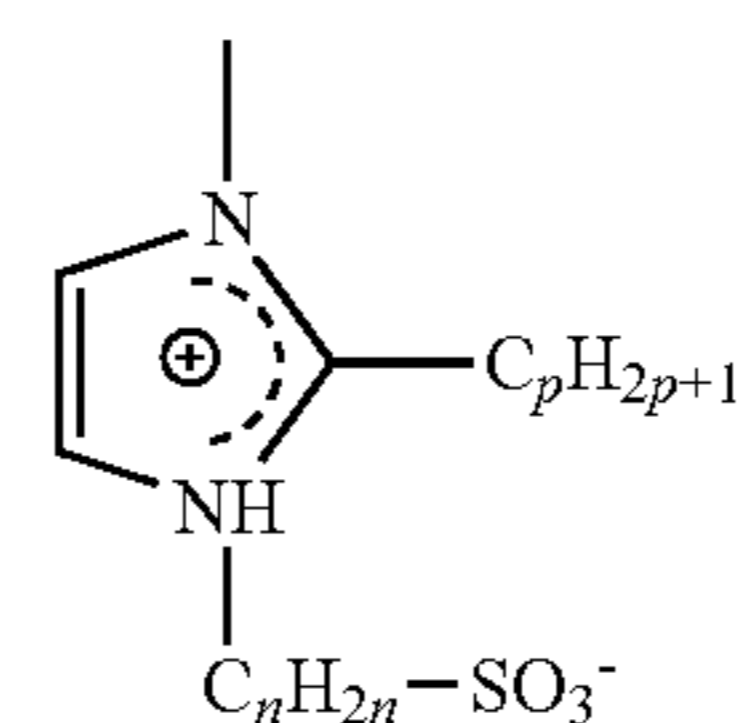
Sulfoalkyl imidazolium salts
