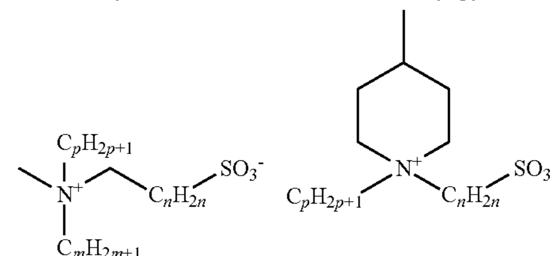
Sulfoalkyl ammonium salts (sulfobetaine)
