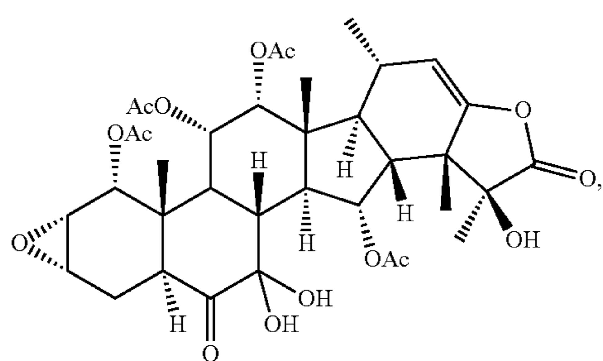
taccalonolide AE
