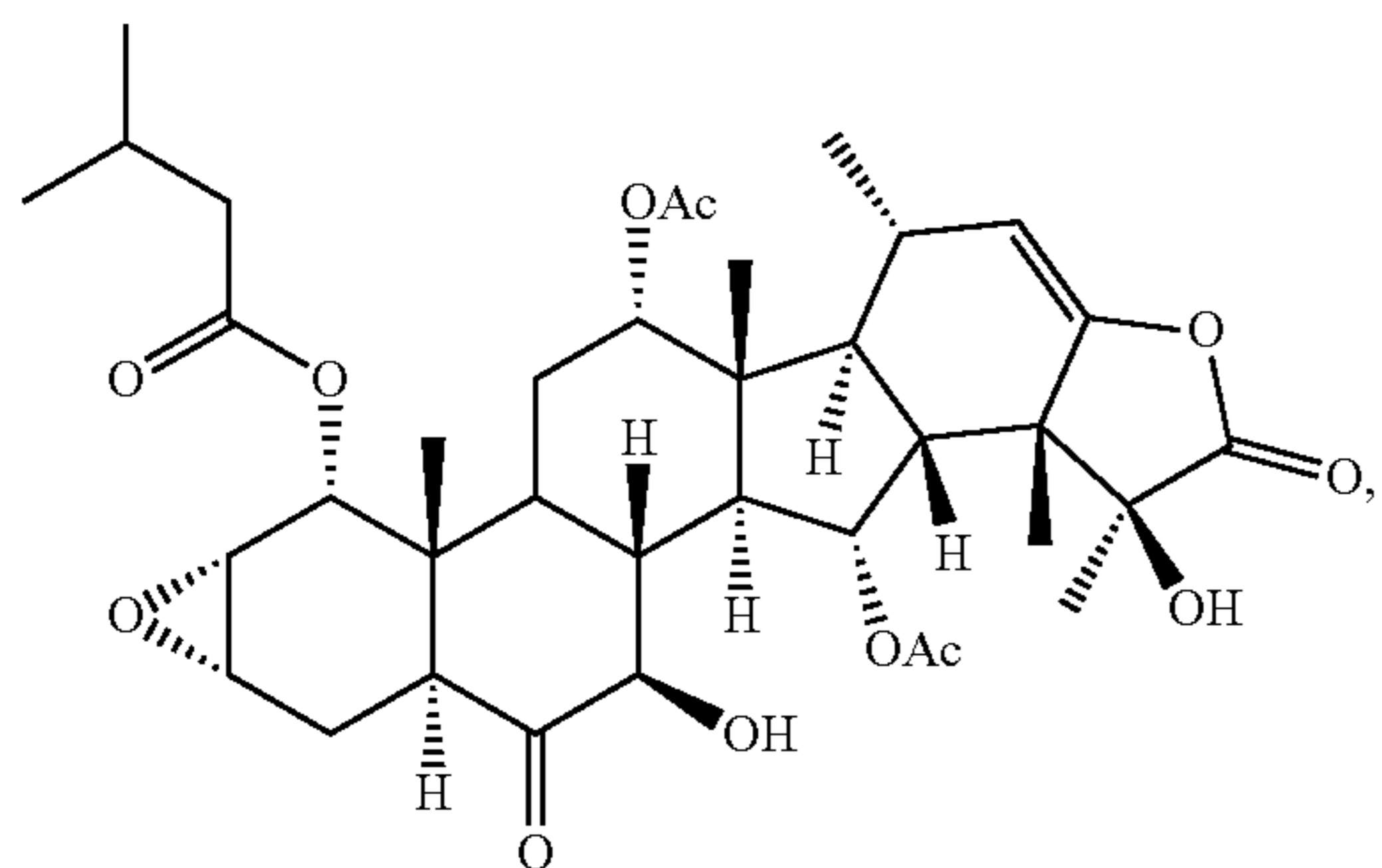
taccalonolide AH
