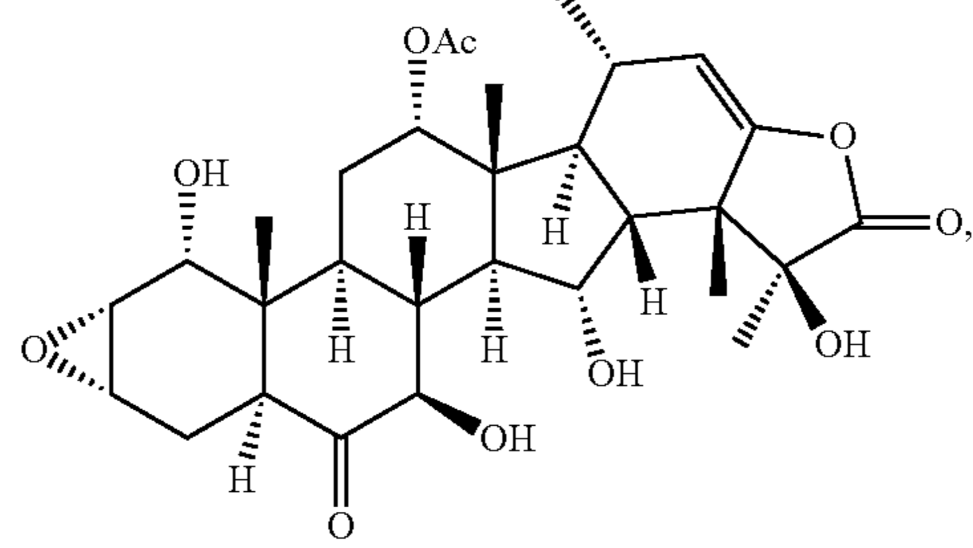
Taccalonolide AN
