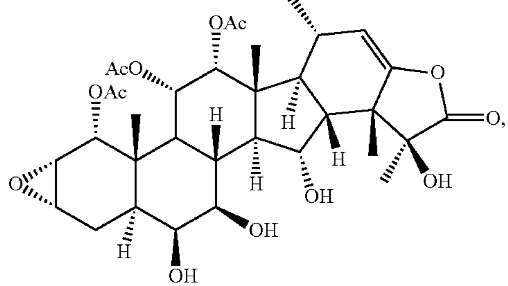
TA-NaBH4-10
