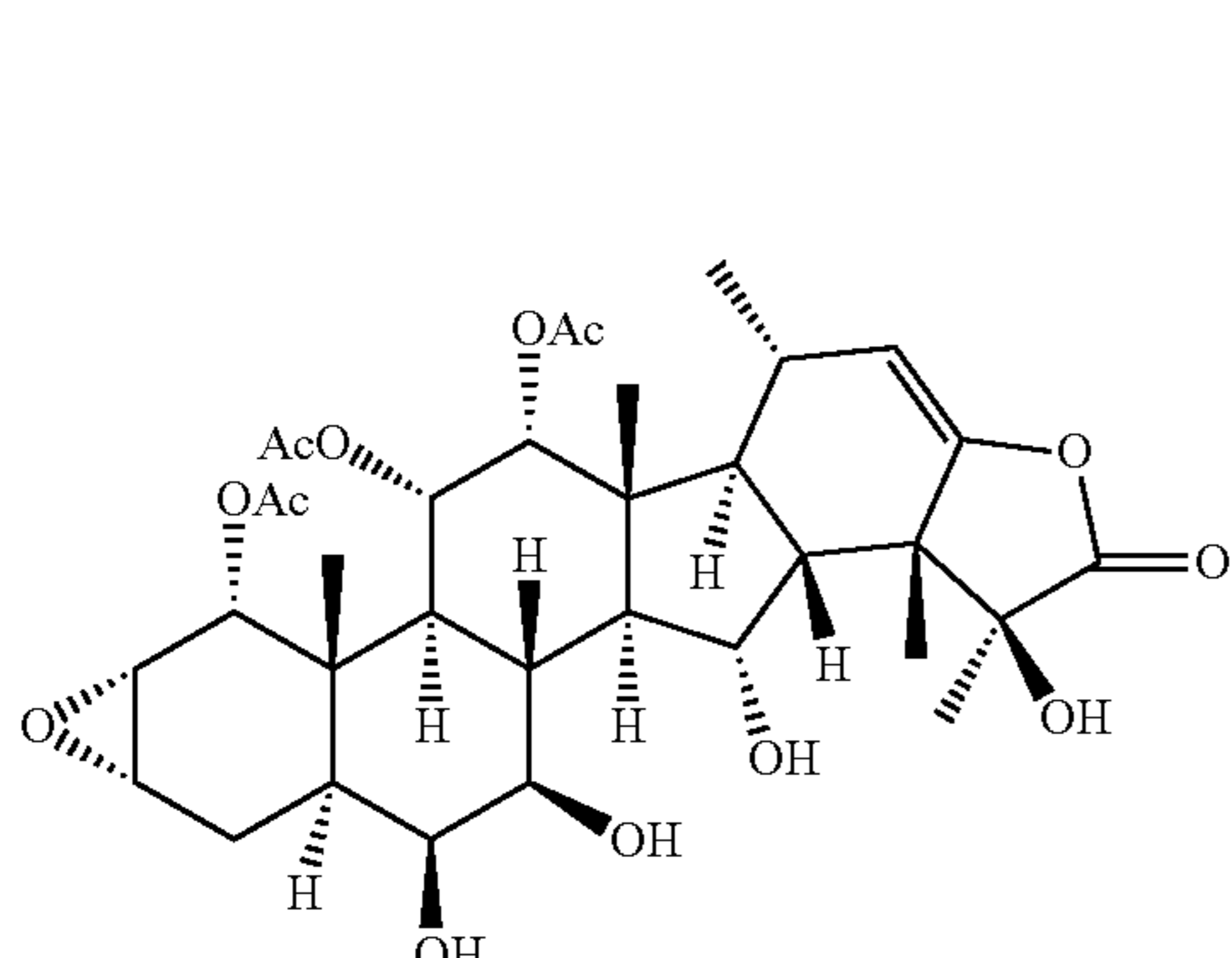
TA-NaBH4-10
