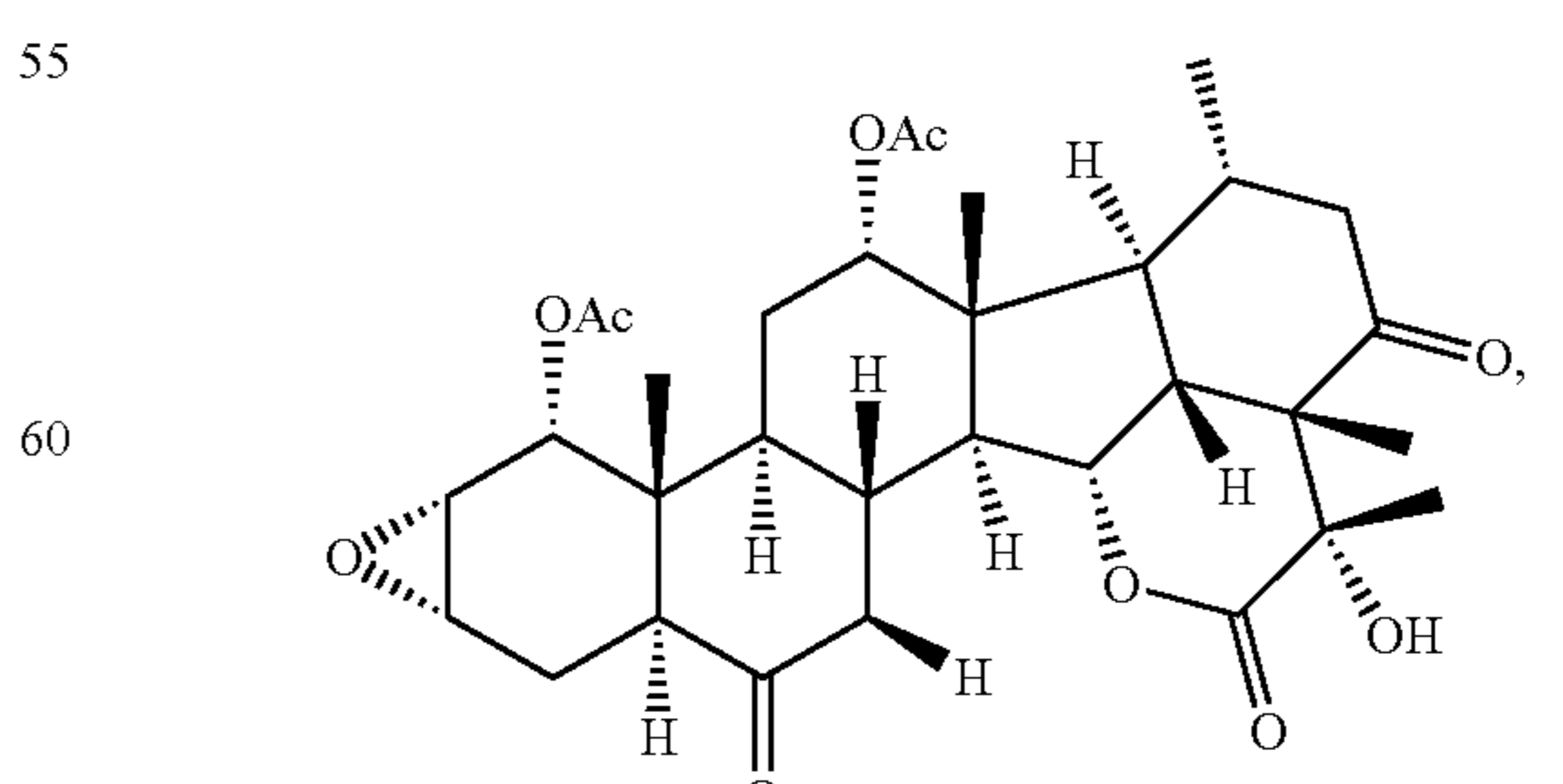
Taccalonolide AK
