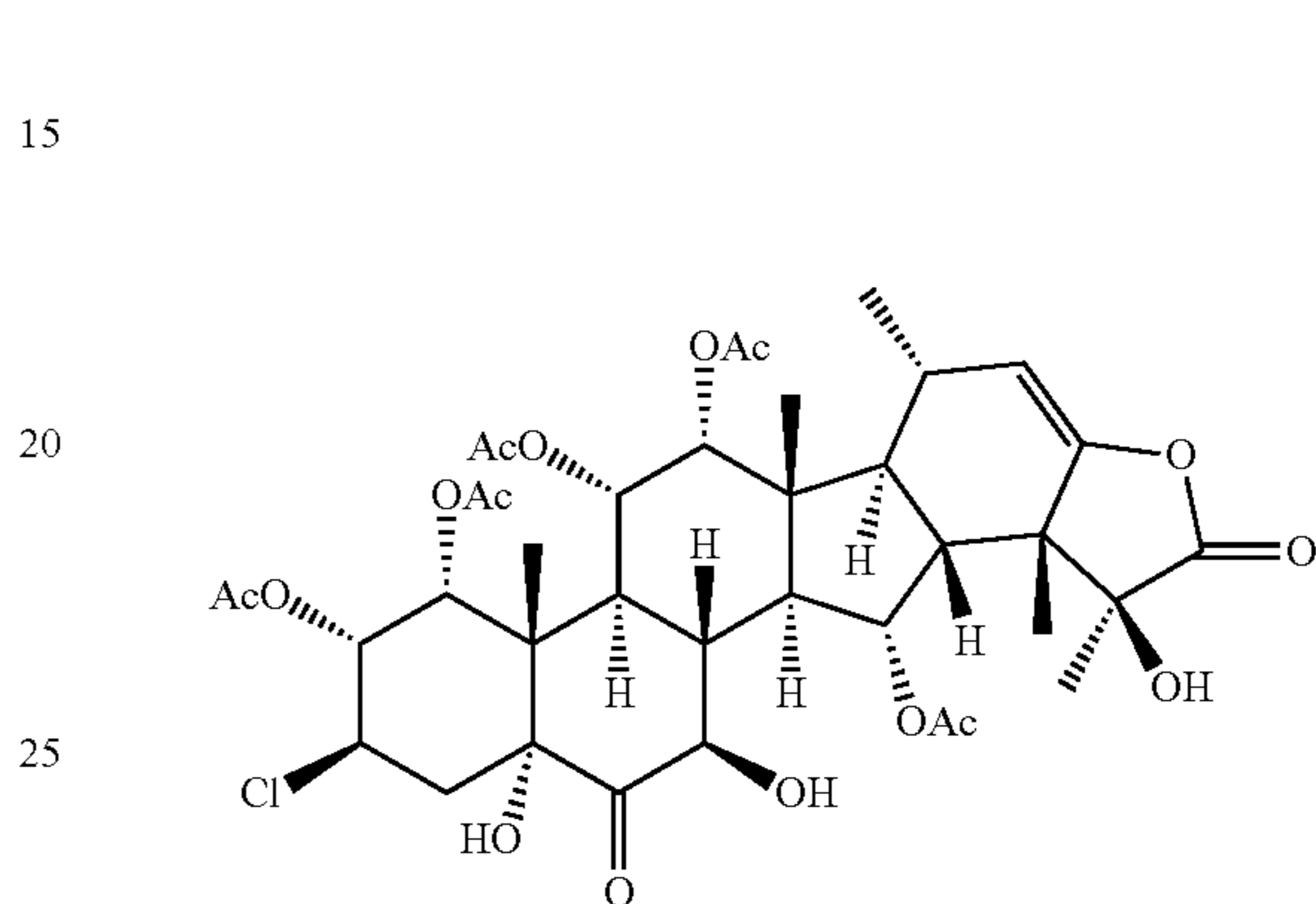
Taccalonolide AQ
