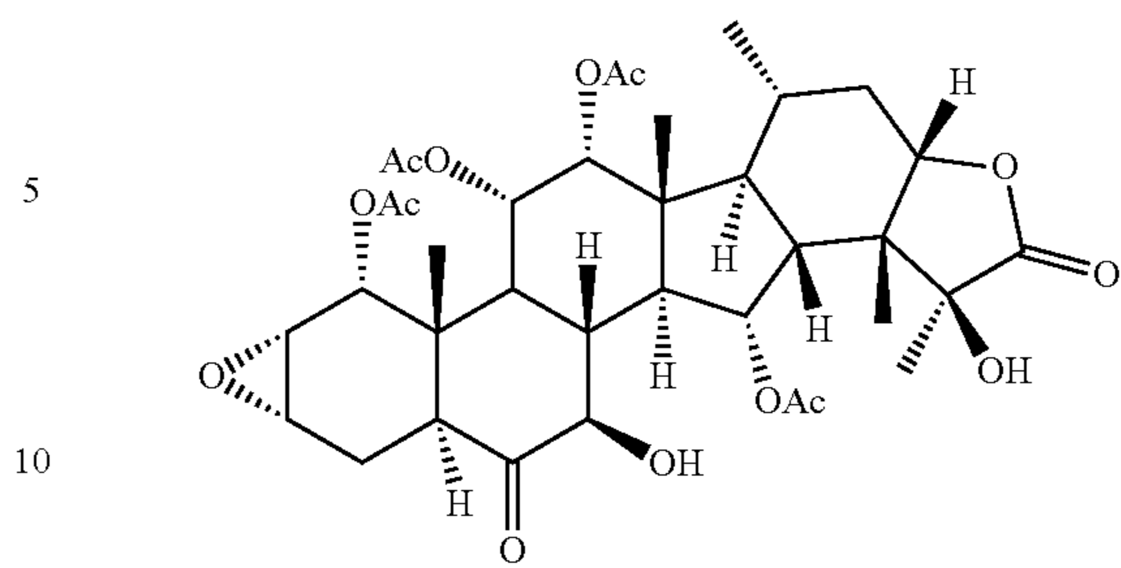
dihydrotaccalonolide A
