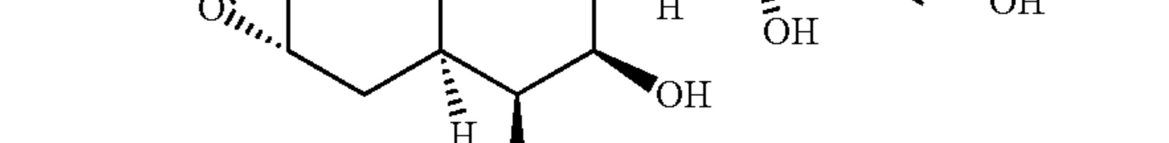
TA-NaBH4-12
