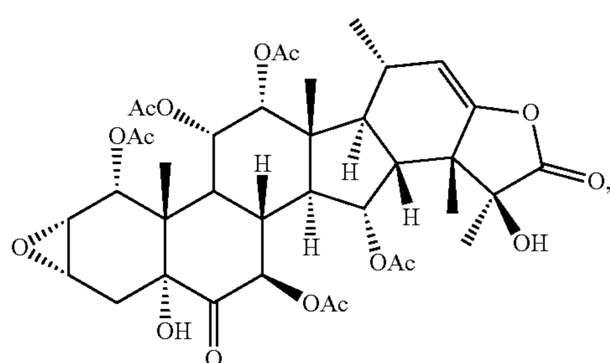
taccalonolide AA
