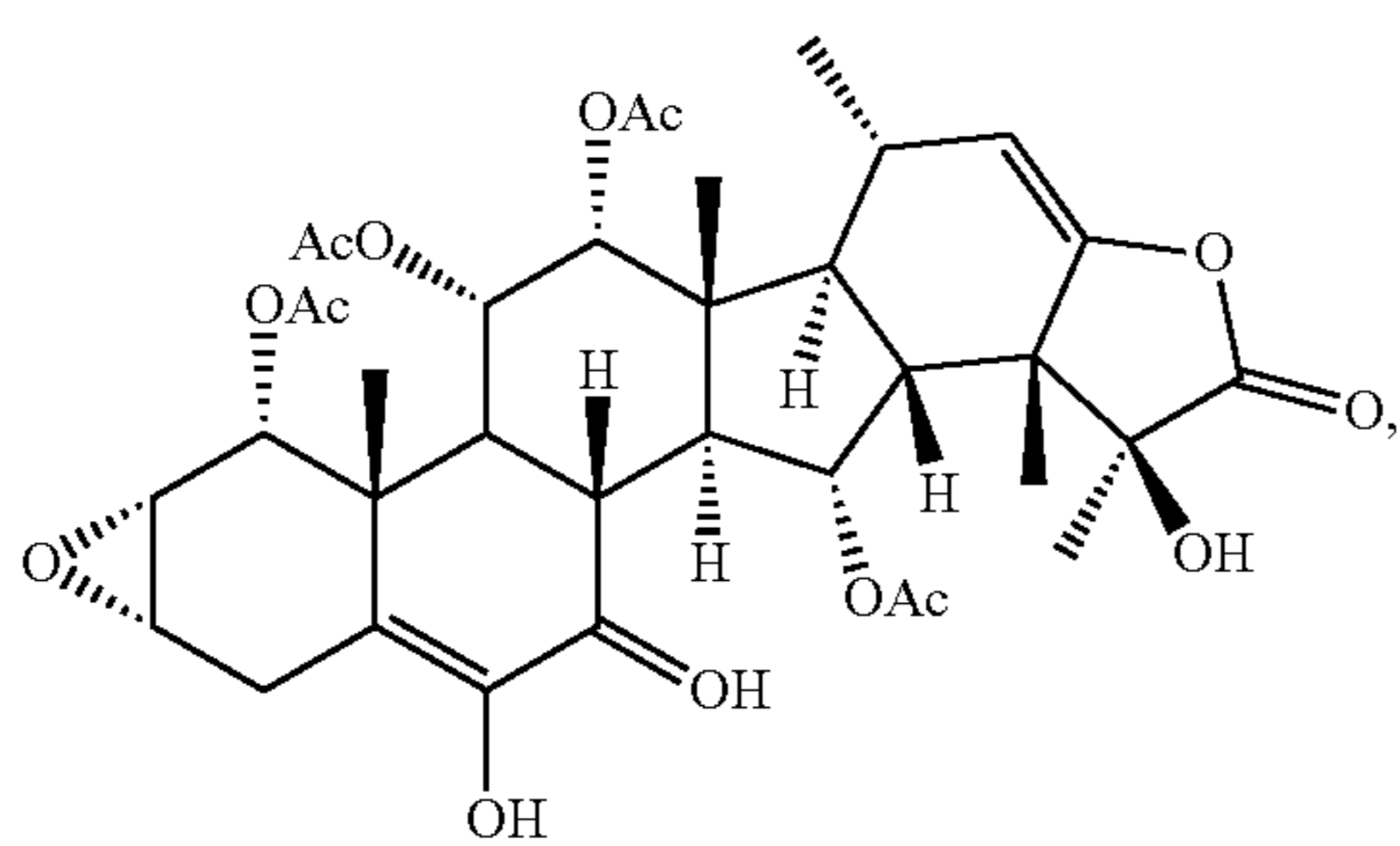
taccalonolide AD
