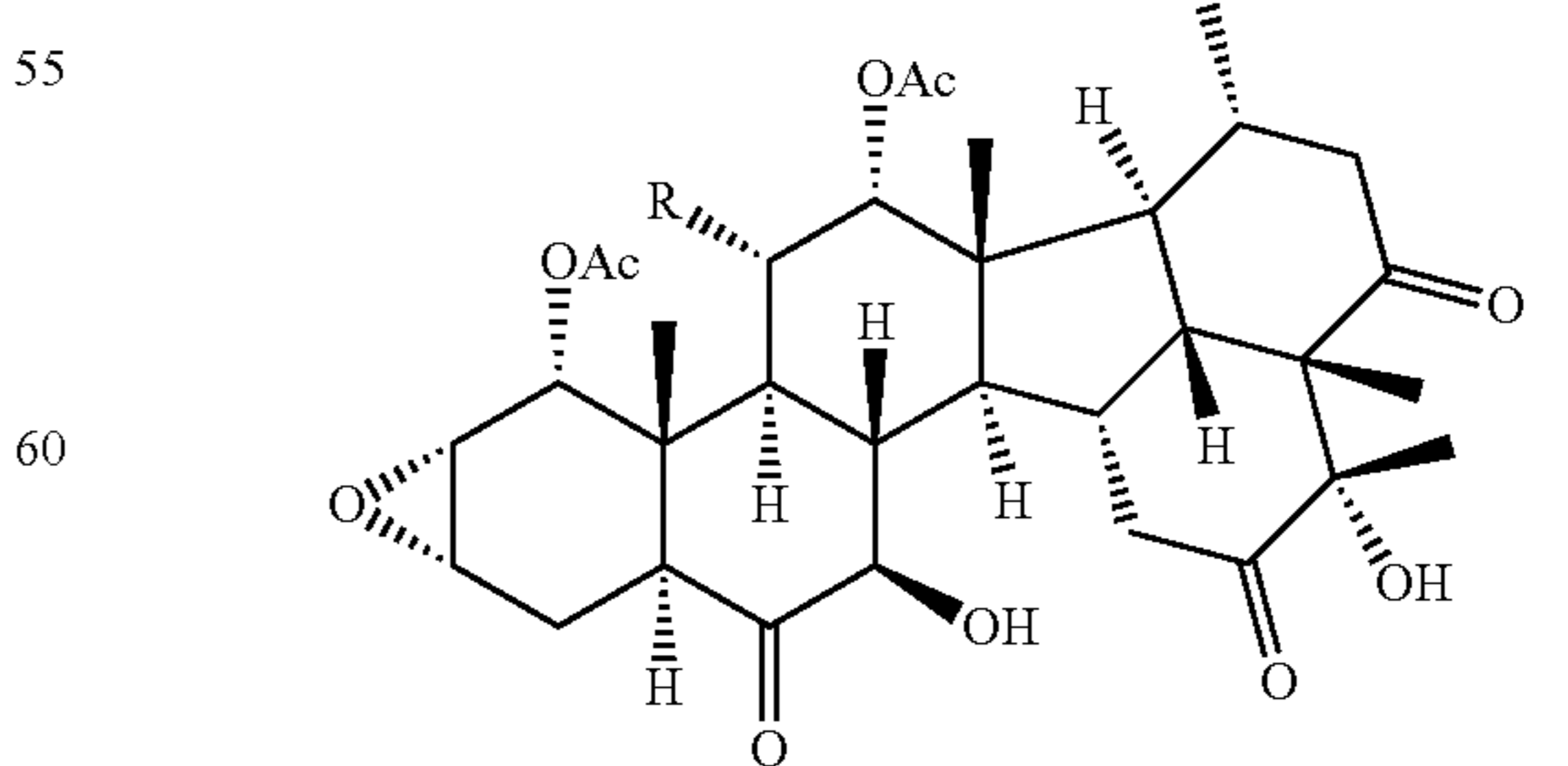
taccalonolide AJ
