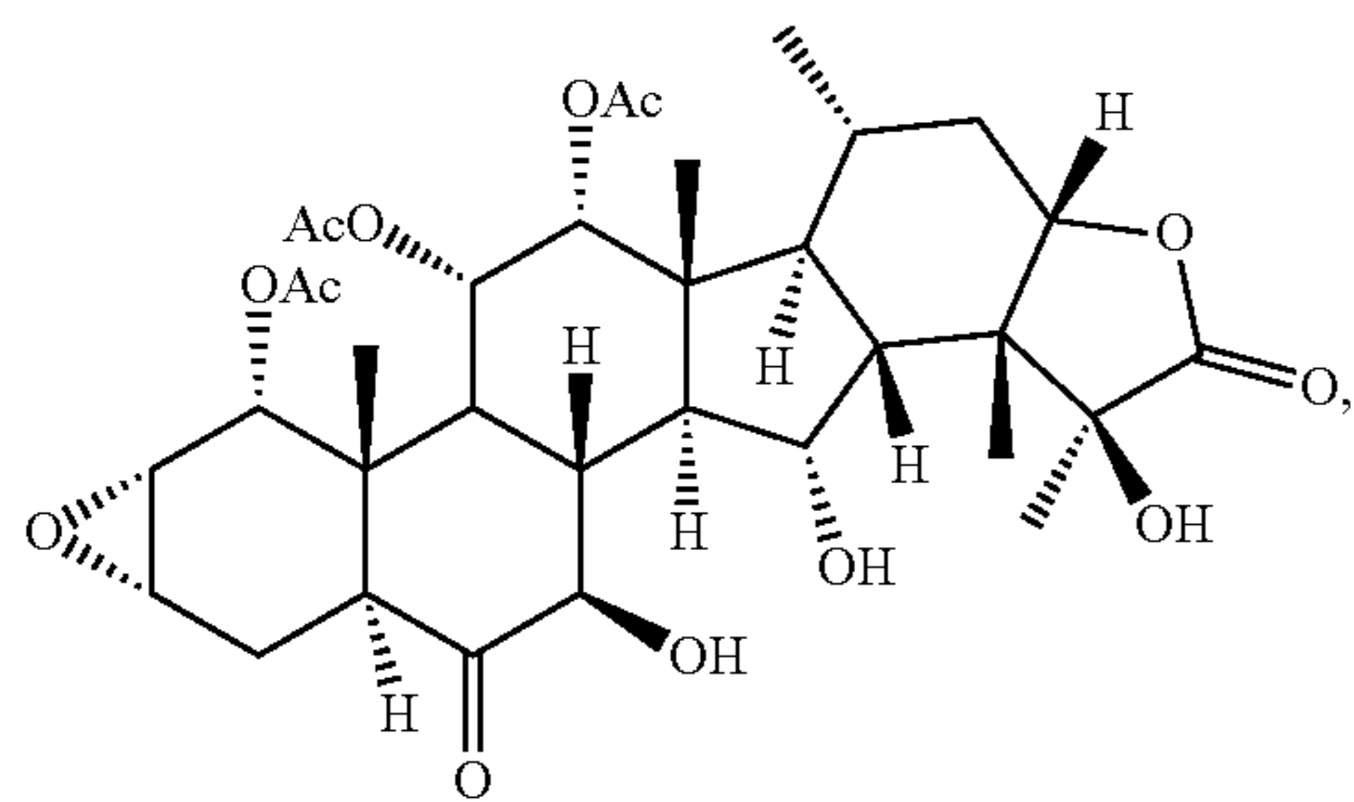
dihydrotaccalonolide B
