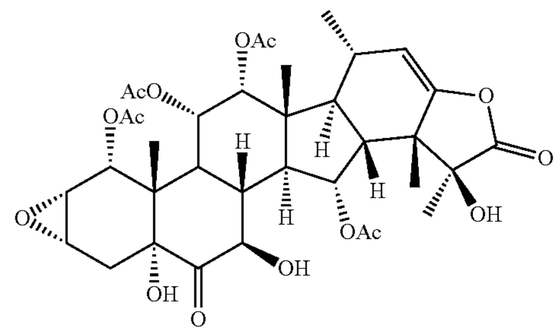
taccalonolide Z
