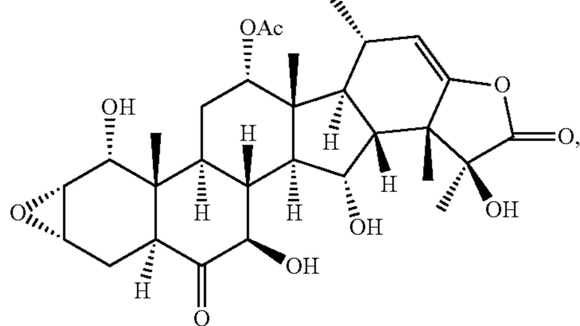
Taccalonolide AN
