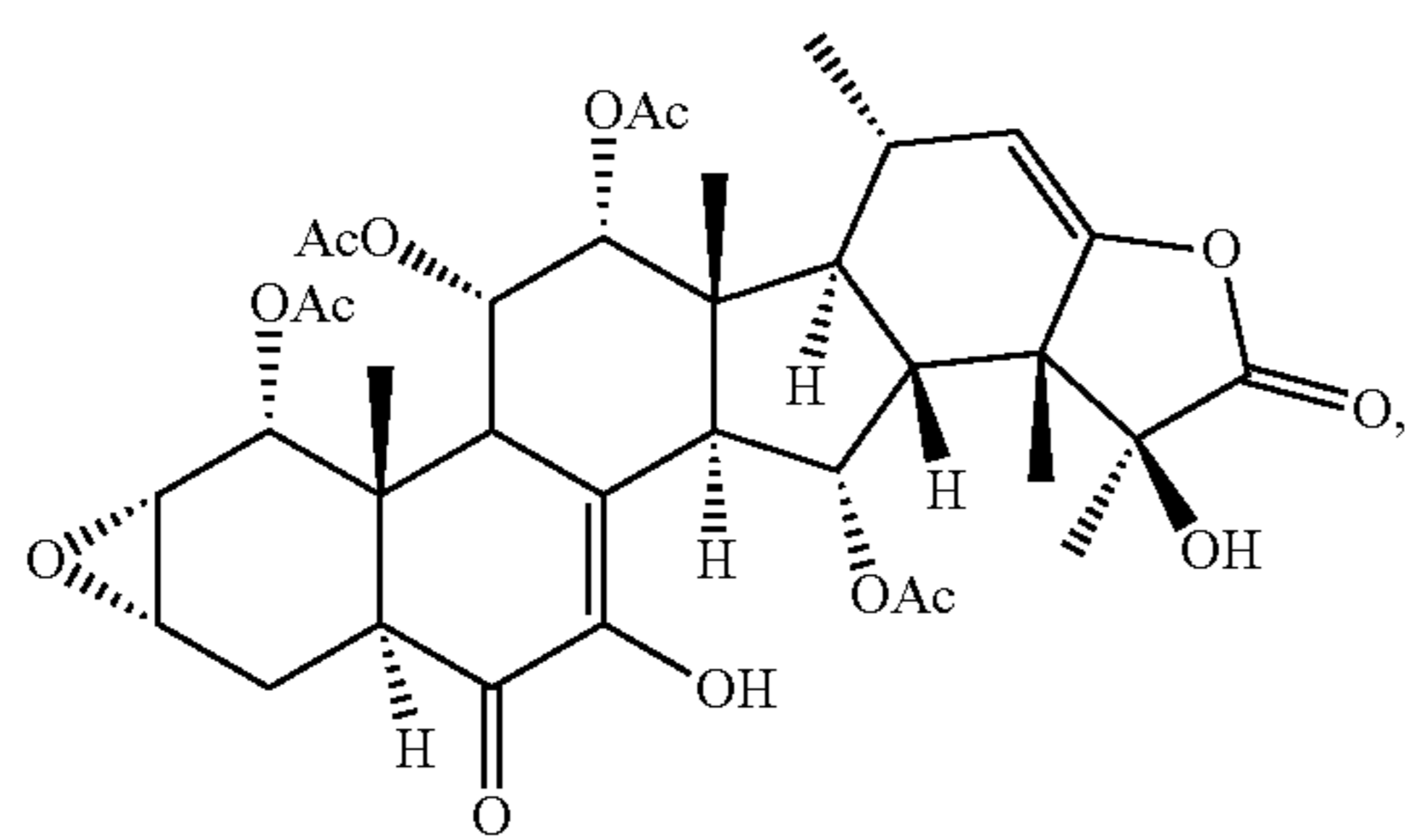
taccalonolide H2
