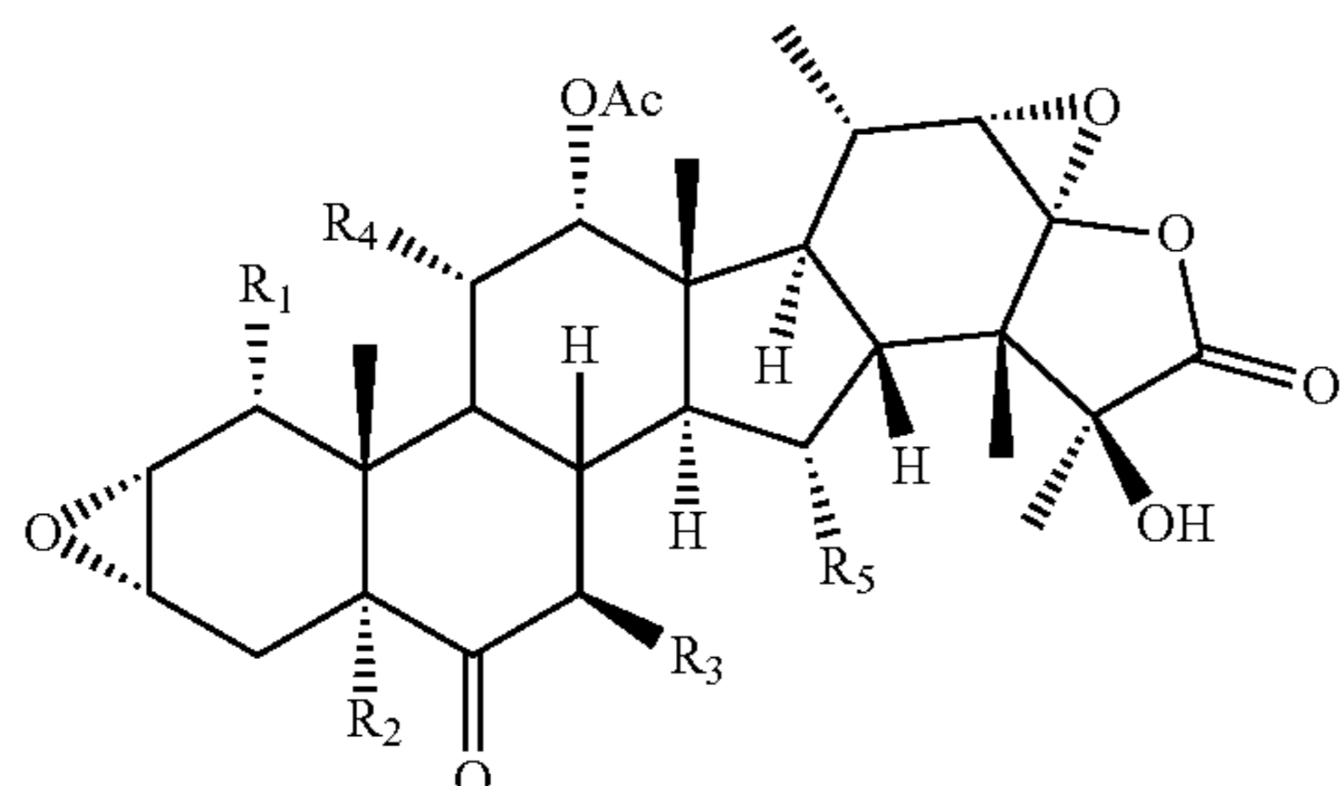
epoxy-TB-Ac-16
