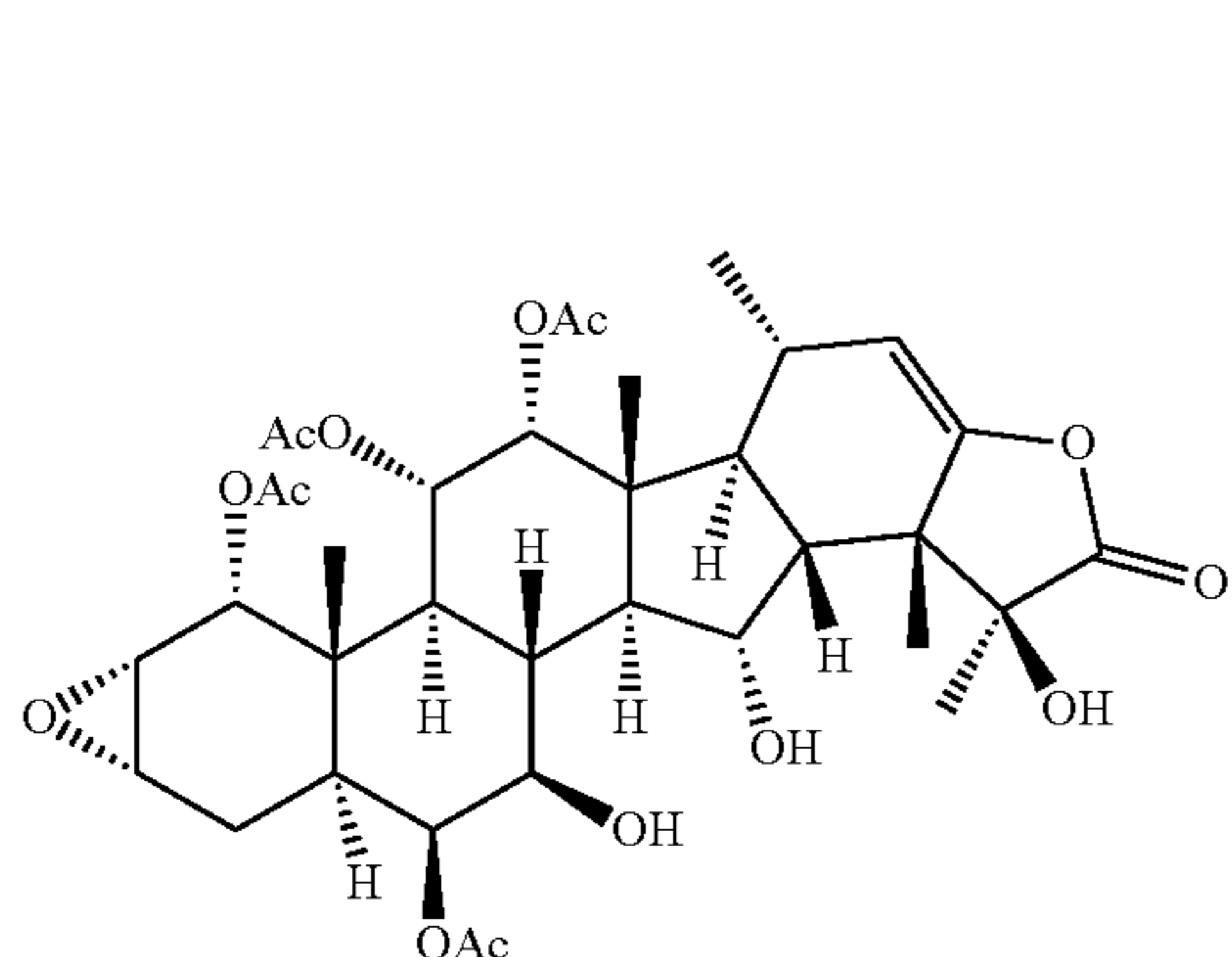
TA-NaBH4-12
