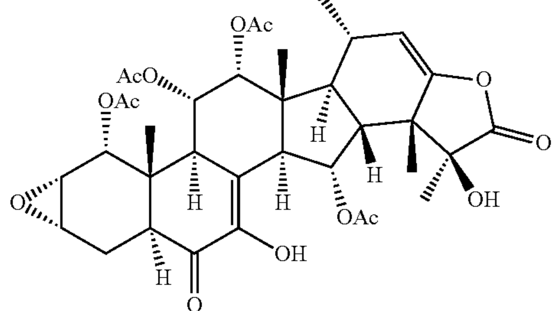
taccalonolide H2
