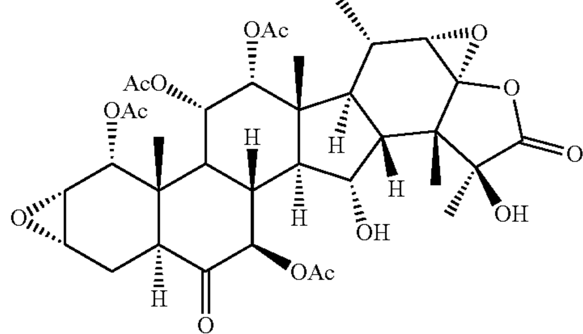
epoxy-TB-Ac-16
