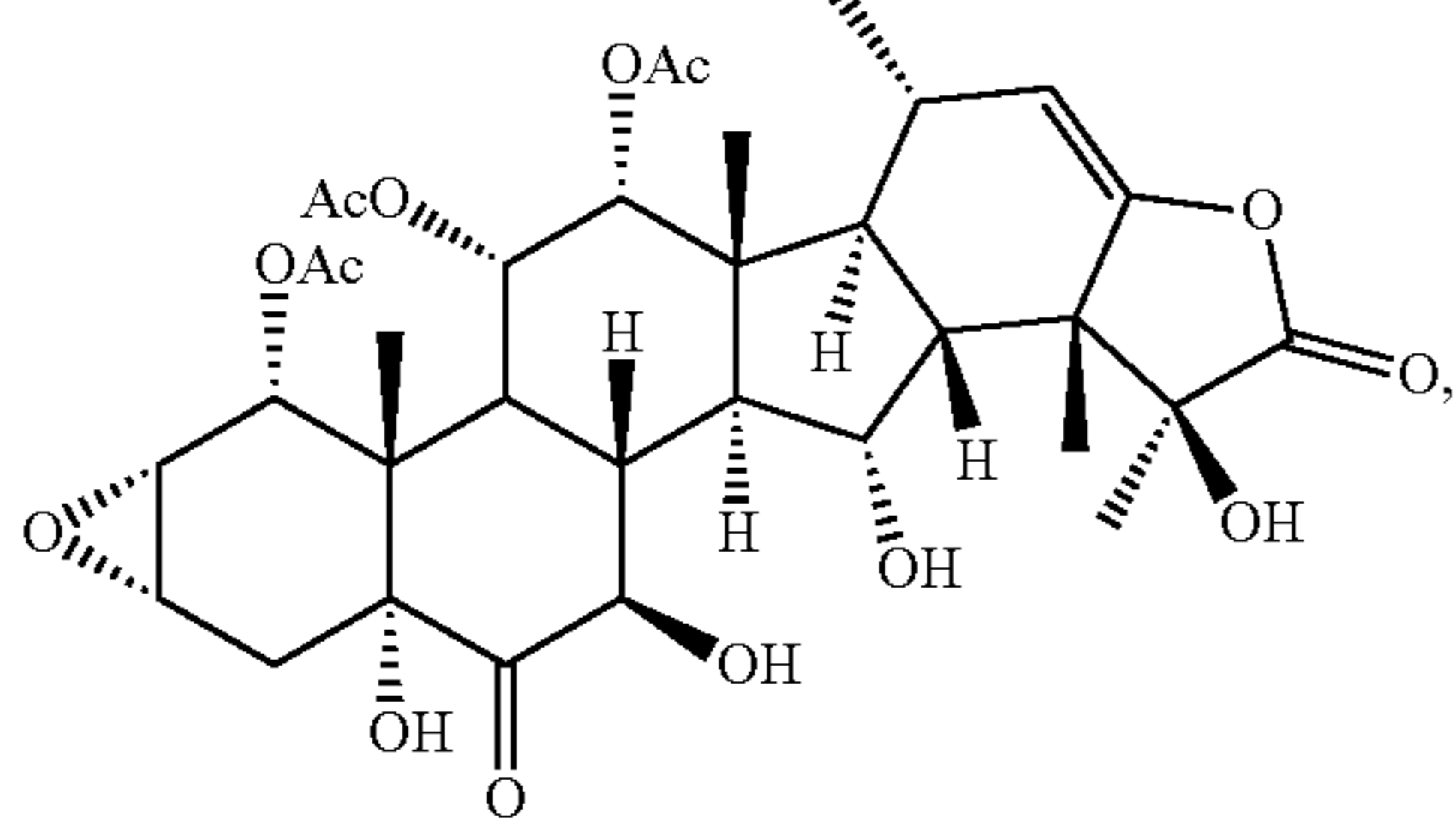
taccalonolide AB
