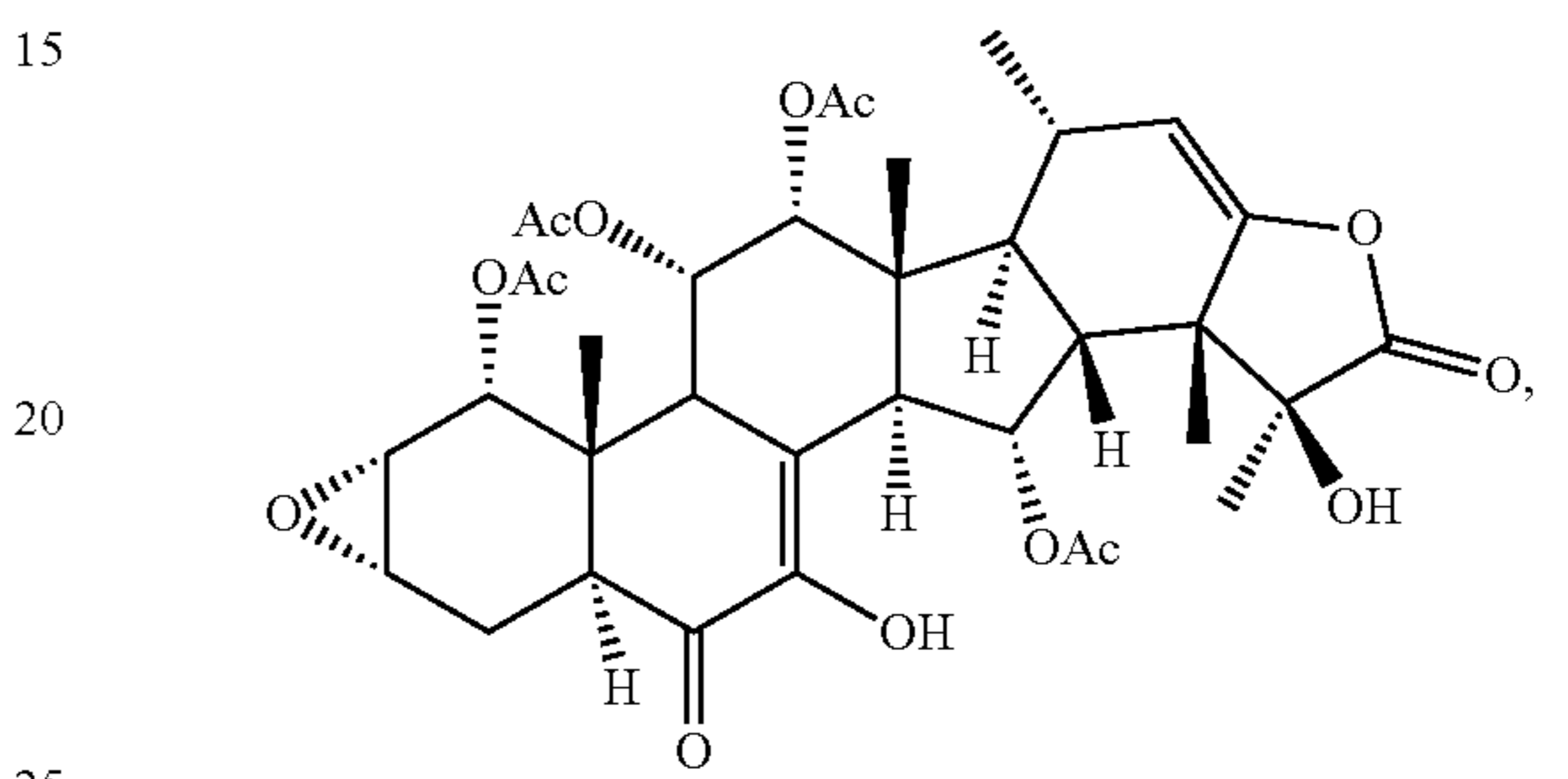
taccalonolide H2
