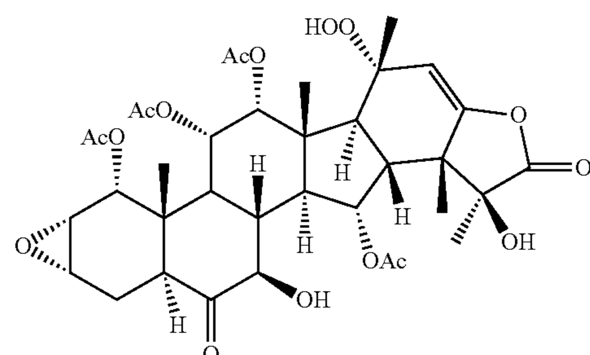
taccalonolide AC
