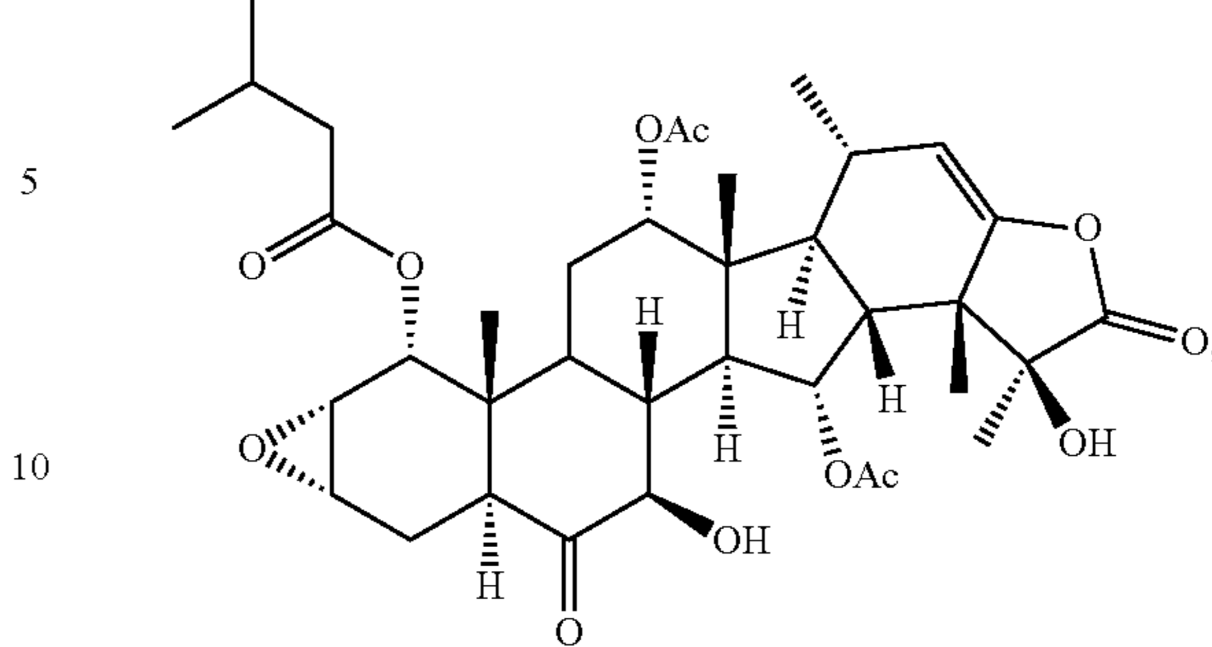
taccalonolide AH
