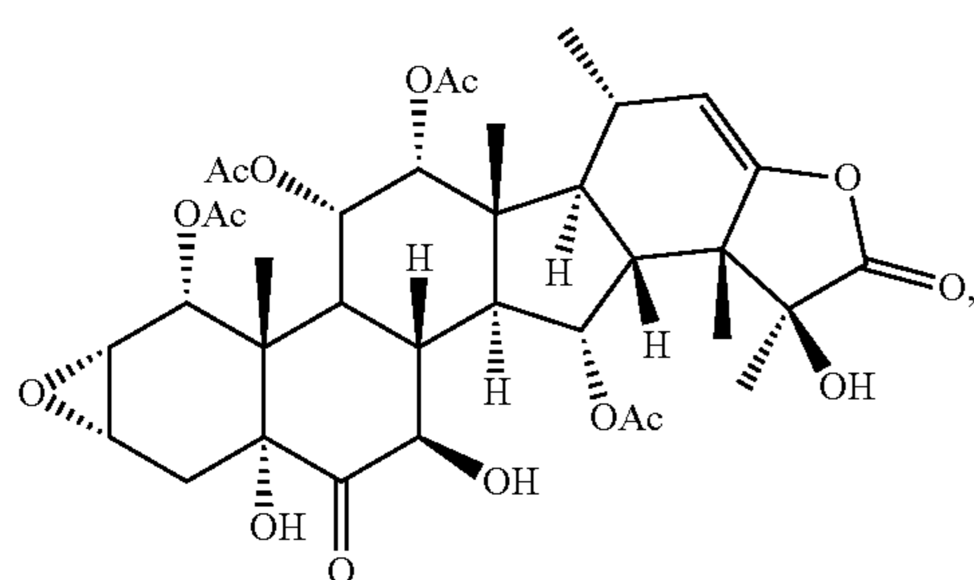
taccalonolide Z
