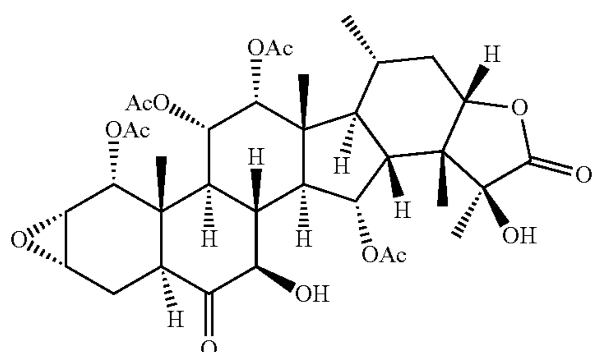
dihydrotaccalonolide A
