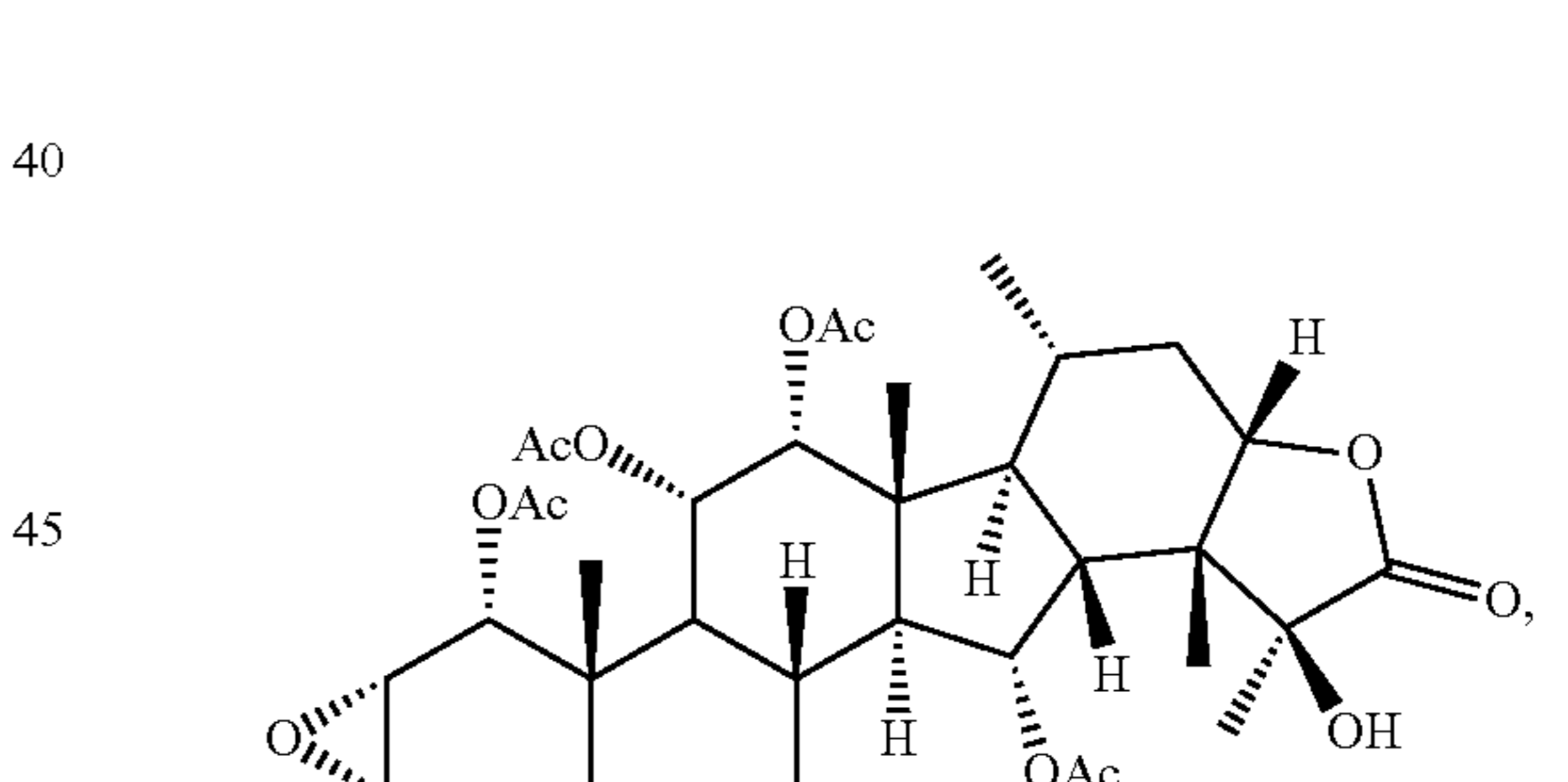
dihydrotaccalonolide A
