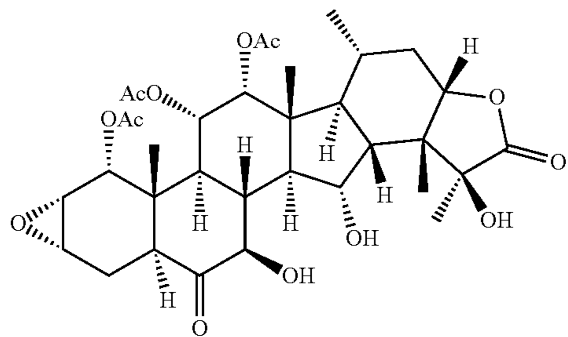
dihydrotaccalonolide B
