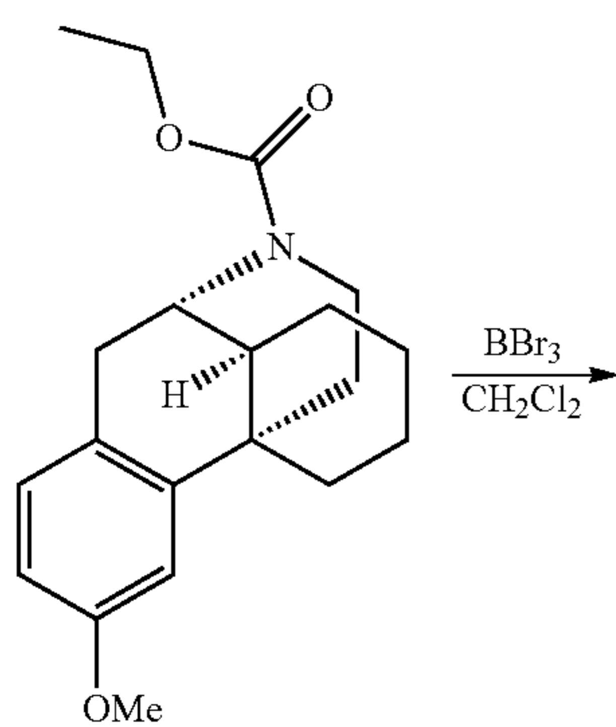
Scheme 1. Synthesis of a Compound of Formula I ( R^1 is —O—(C_2-C_4) alkyl)
