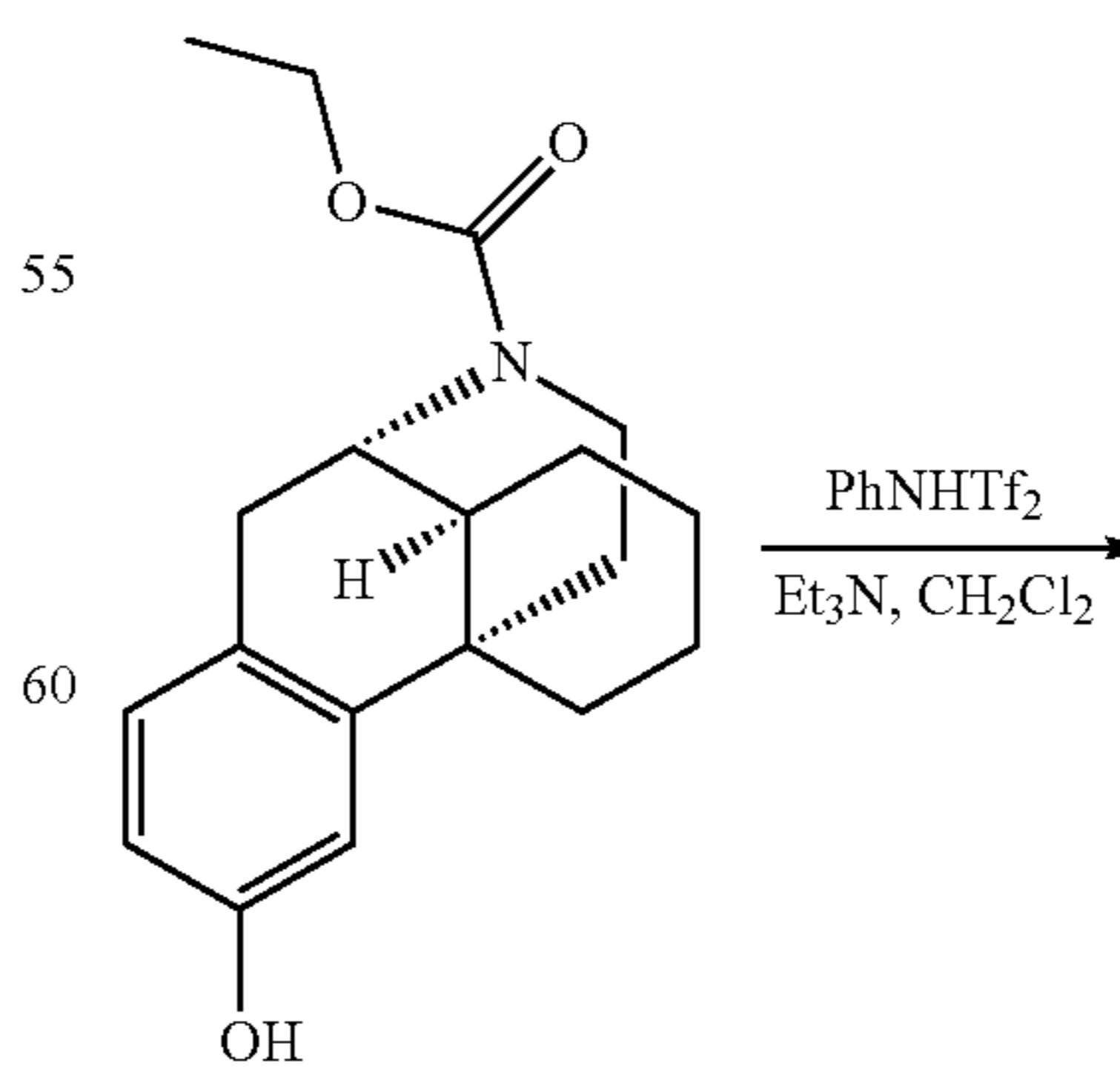
Scheme 2. Synthesis of a Compound of Formula I ( R^1 is —(C_1-C_4) alkyl)
