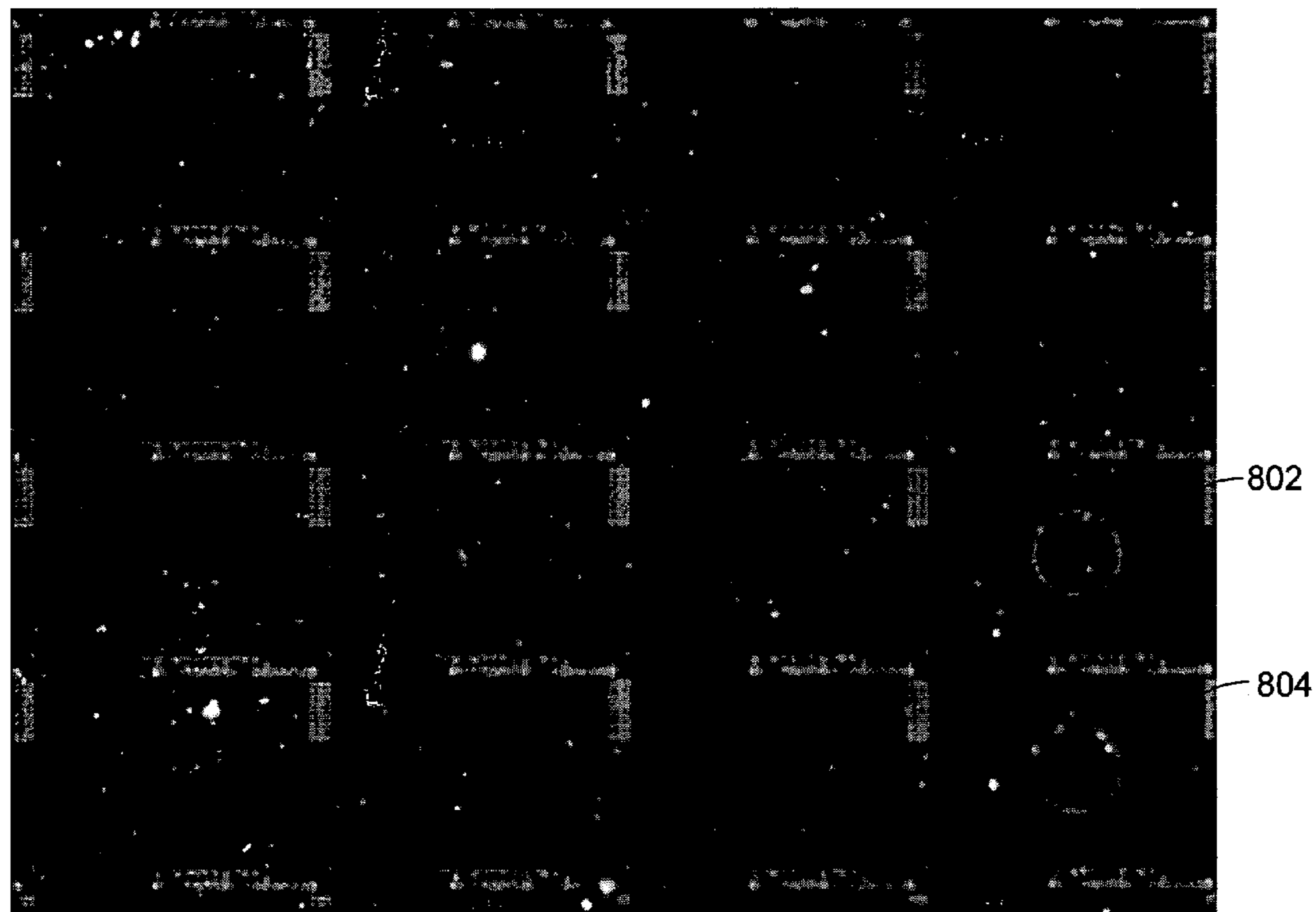
Ethylene Glycol
