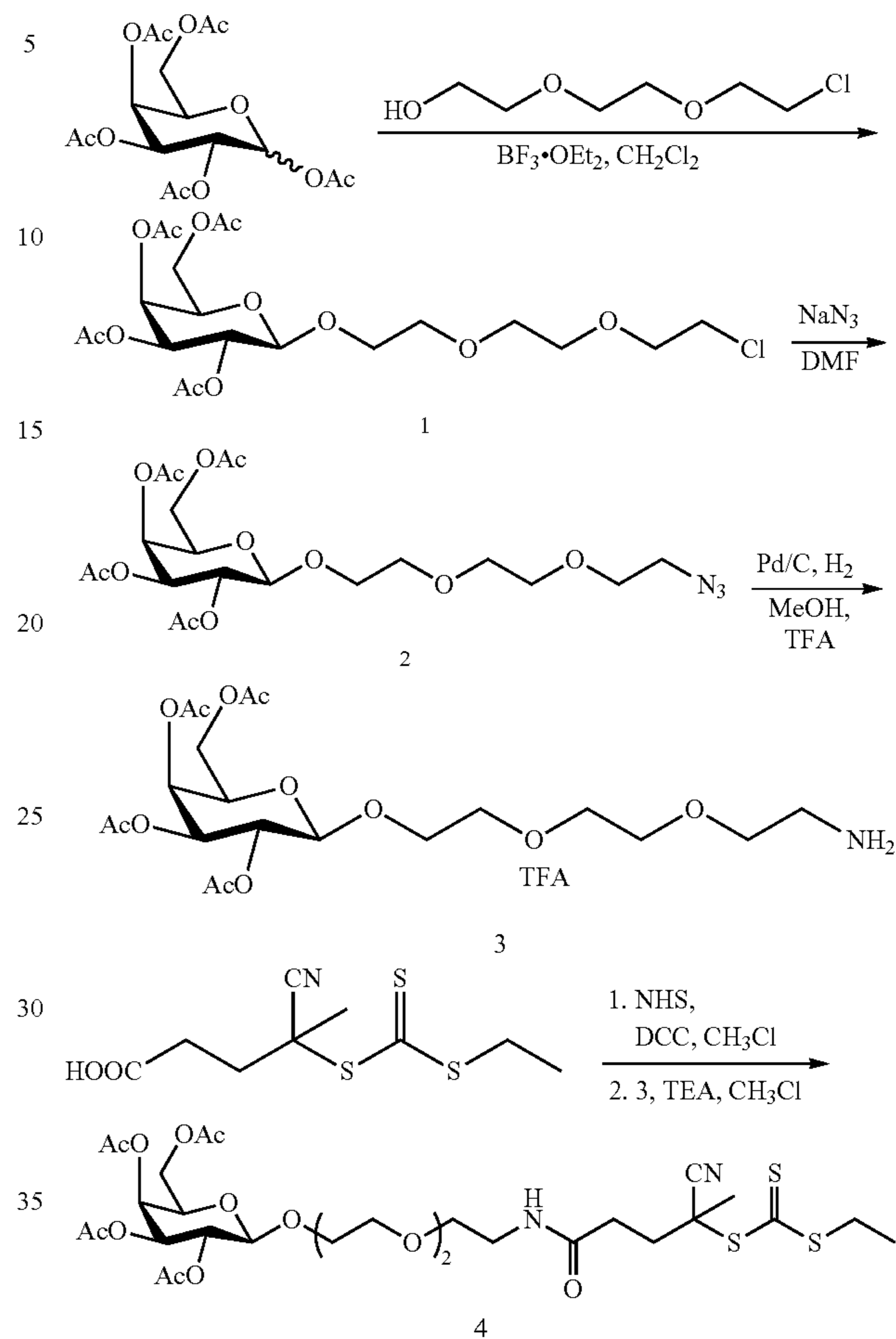
Scheme 1. Synthesis of galactose-PEG-amine (cpd 3) and galactose-CTA (cpd 4)
