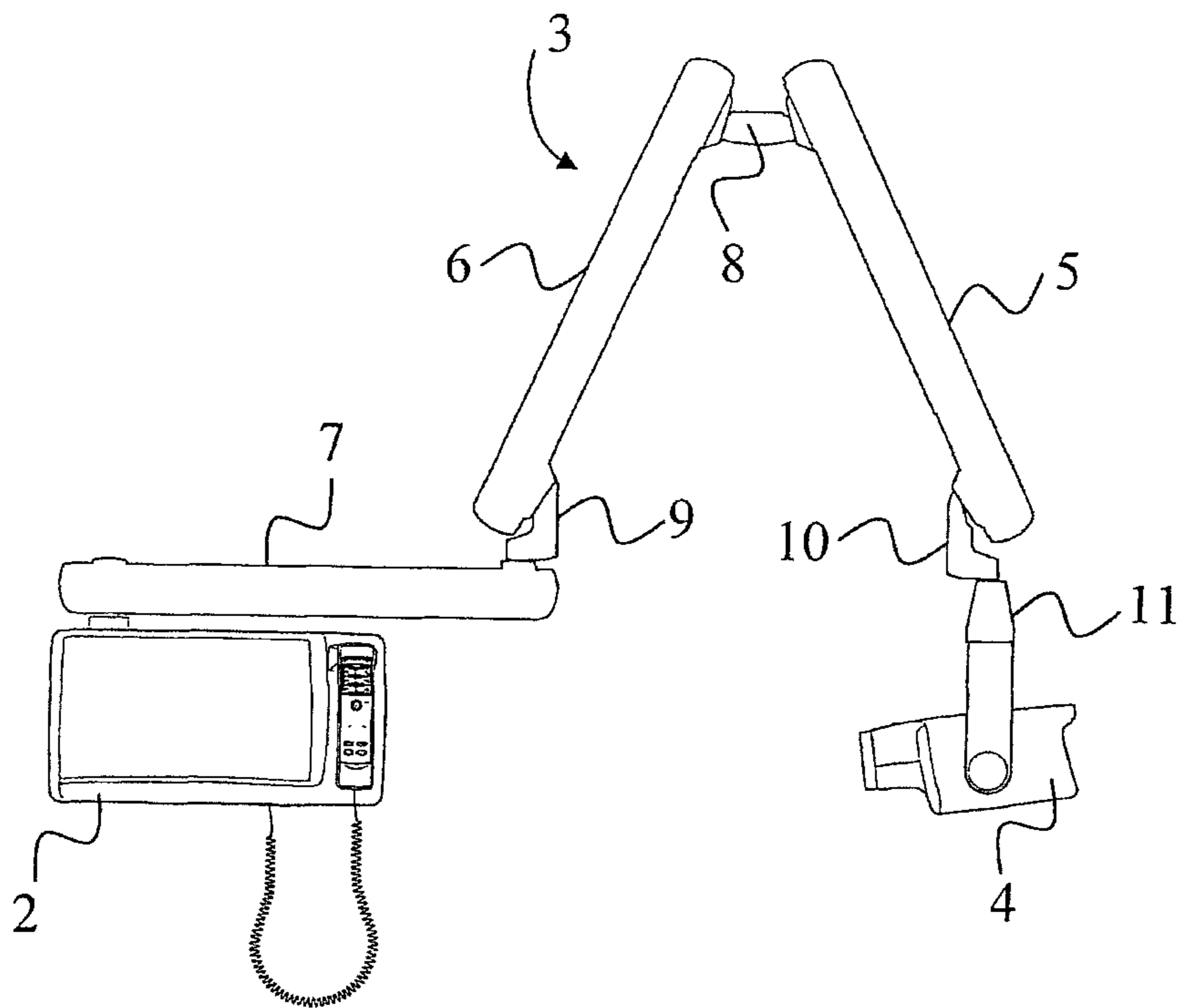
Fig. 1 (PRIOR ART)
