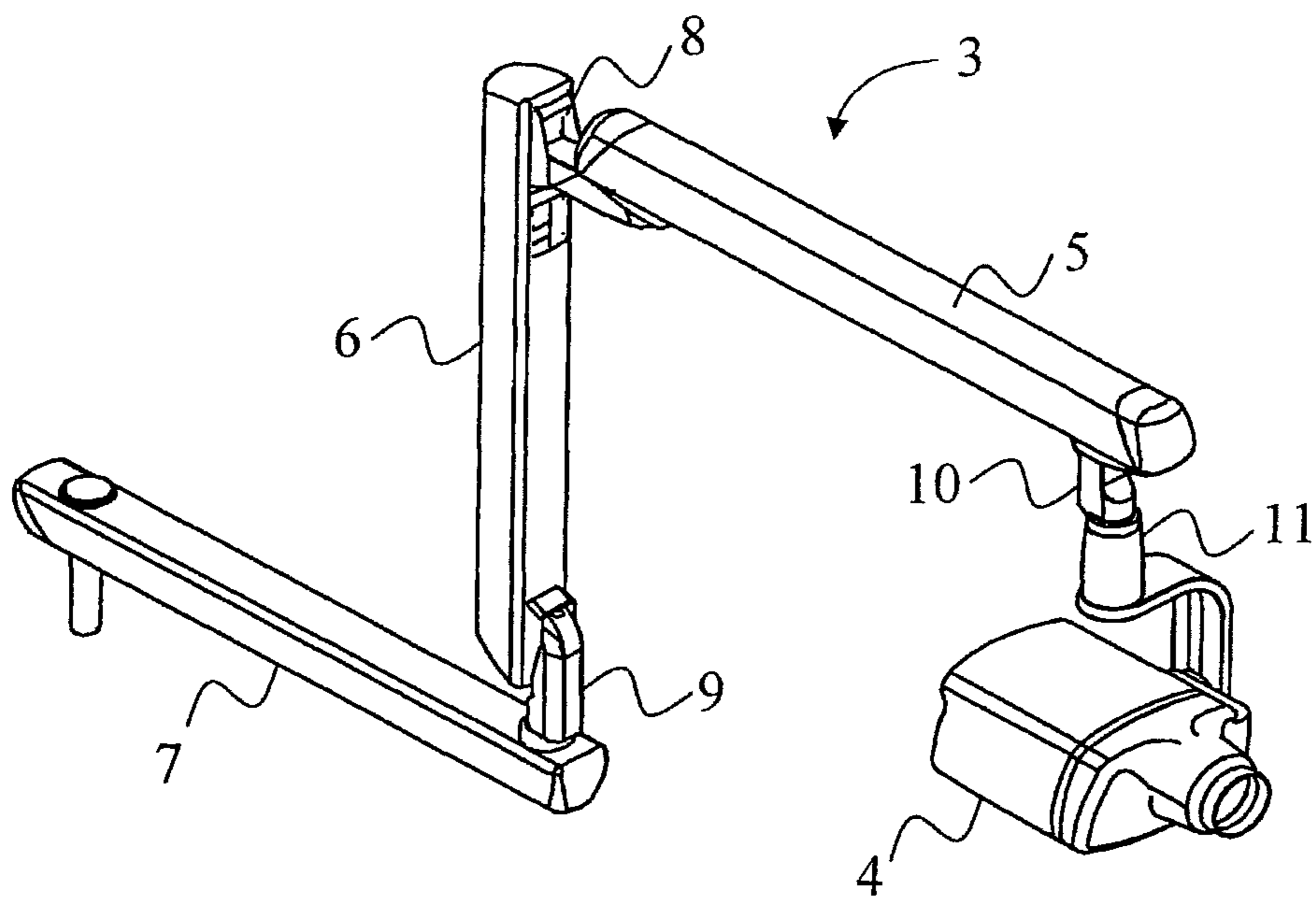
Fig. 2 (PRIOR ART)
