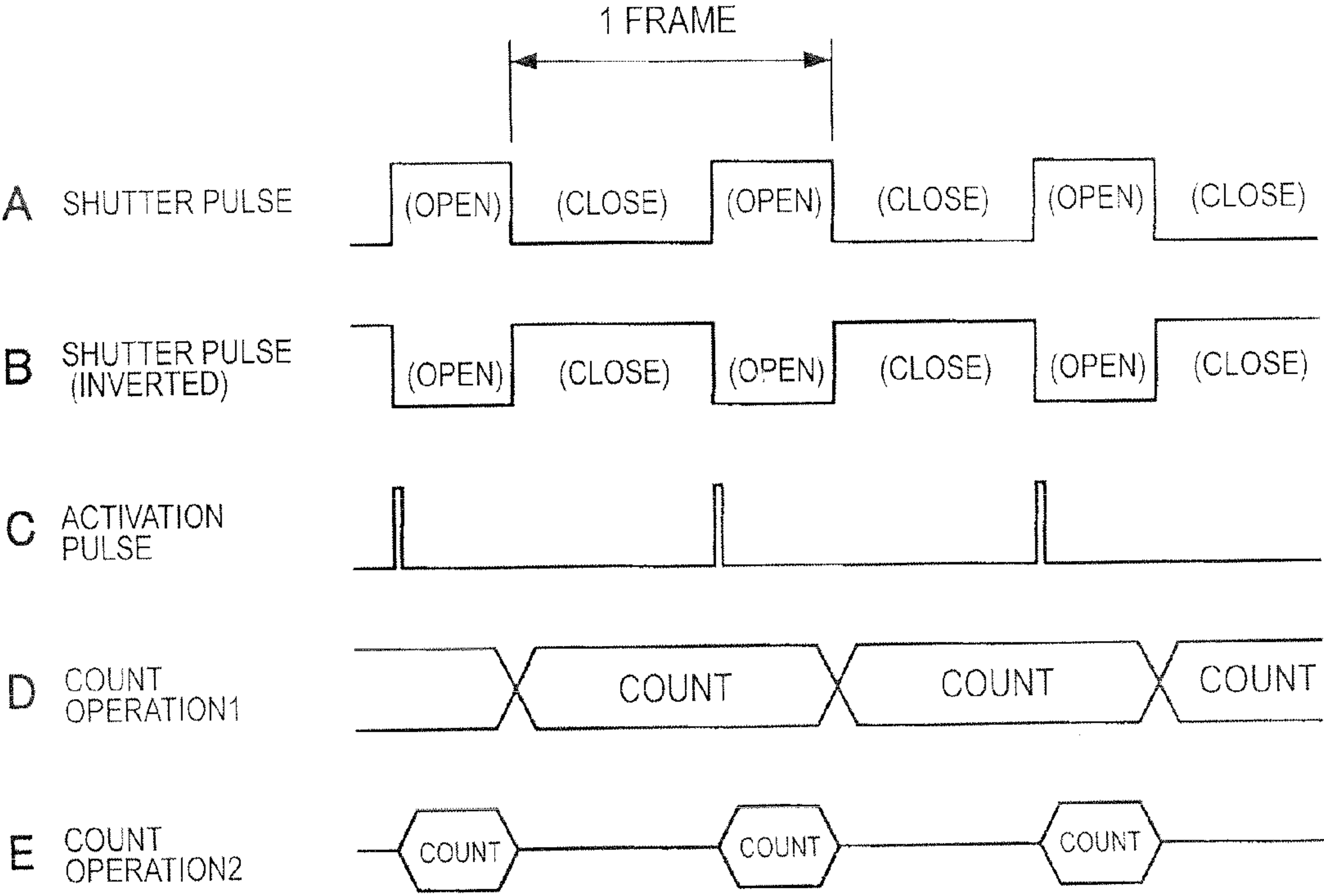
EXAMPLE OF ANALOG PULSE
