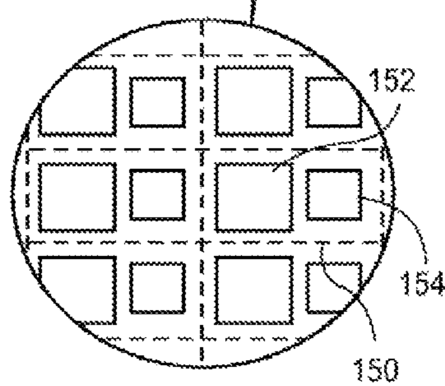
FIG. 1C PRIOR ART
