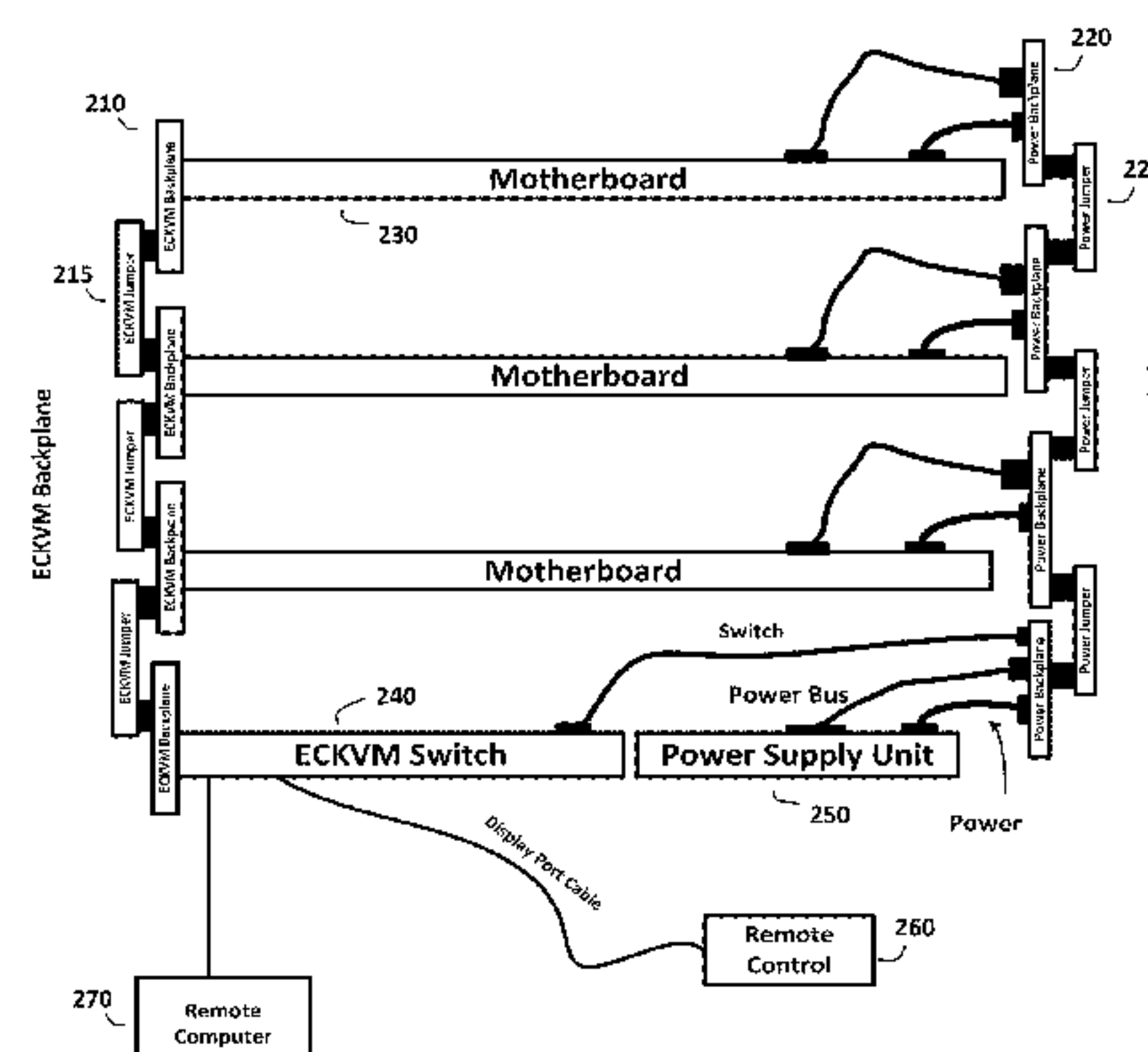
Connection Diagram
