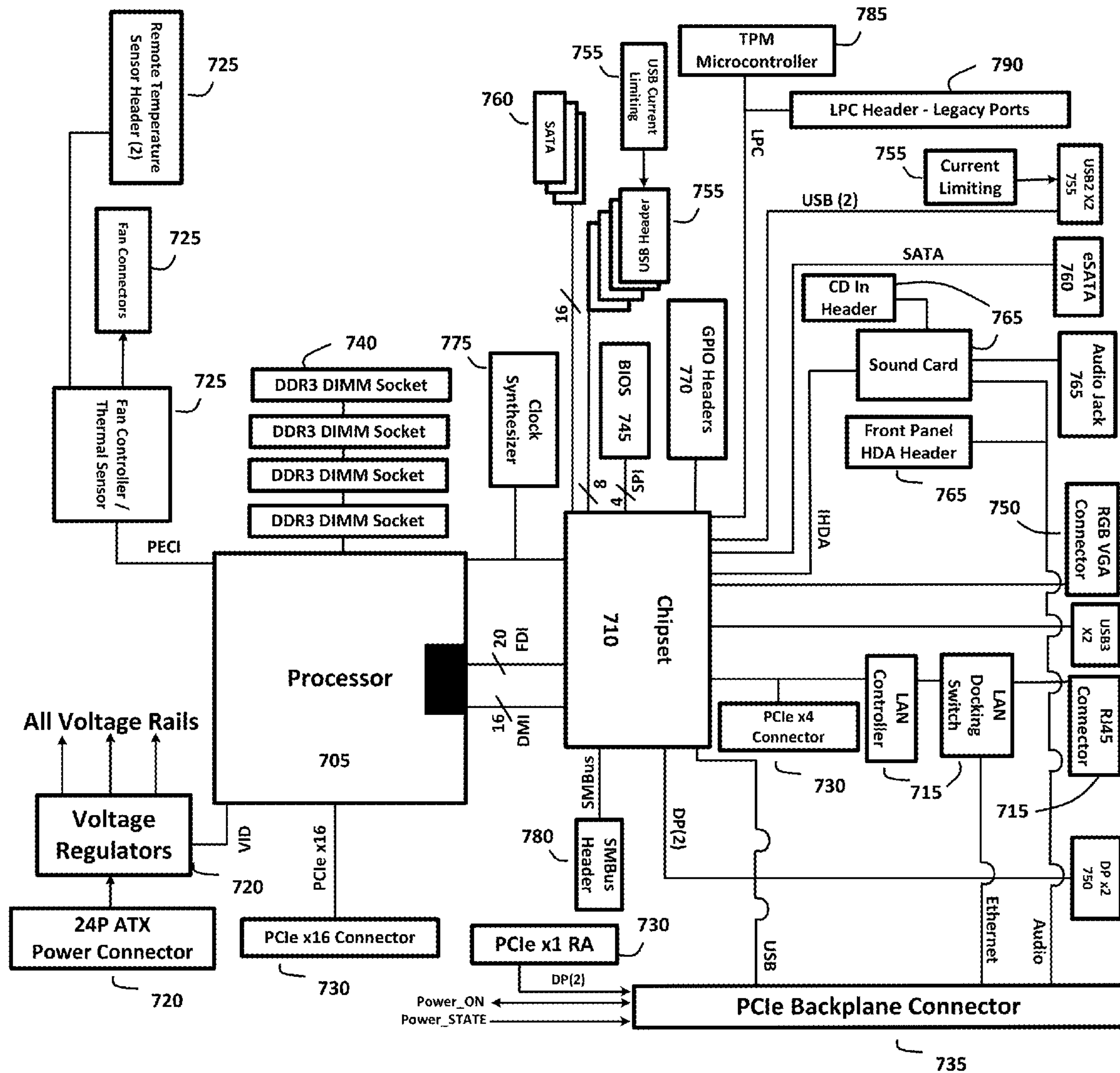
Figure 7 Motherboard - Computer Module
