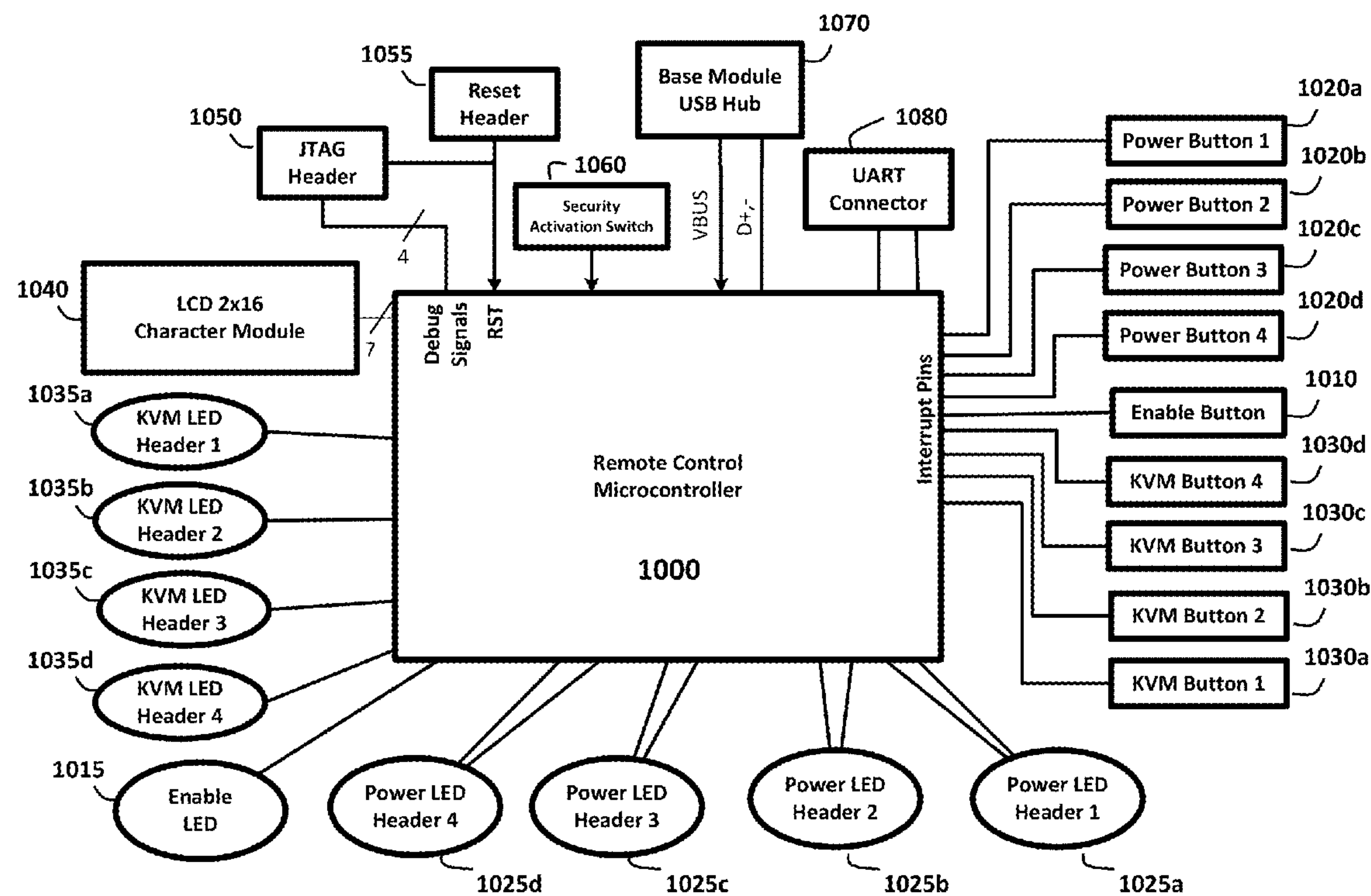
Figure 10 Remote Control Block Diagram
