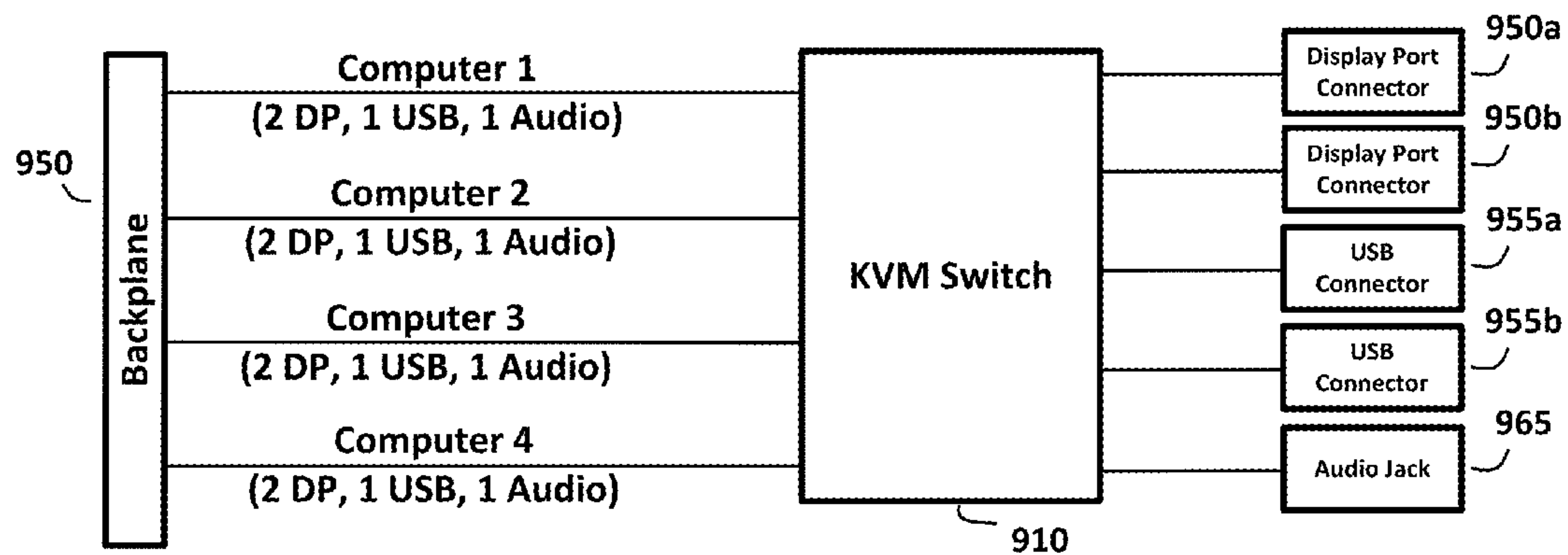
Figure 9 KVM Switch Diagram
