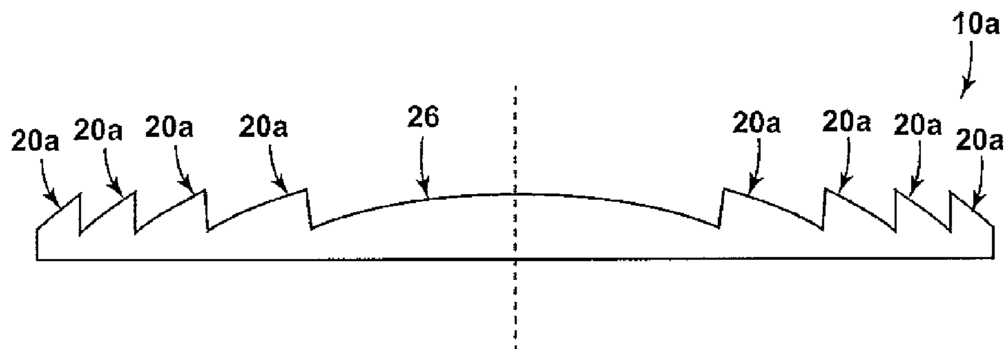
FIG. 4 (PRIOR ART)
