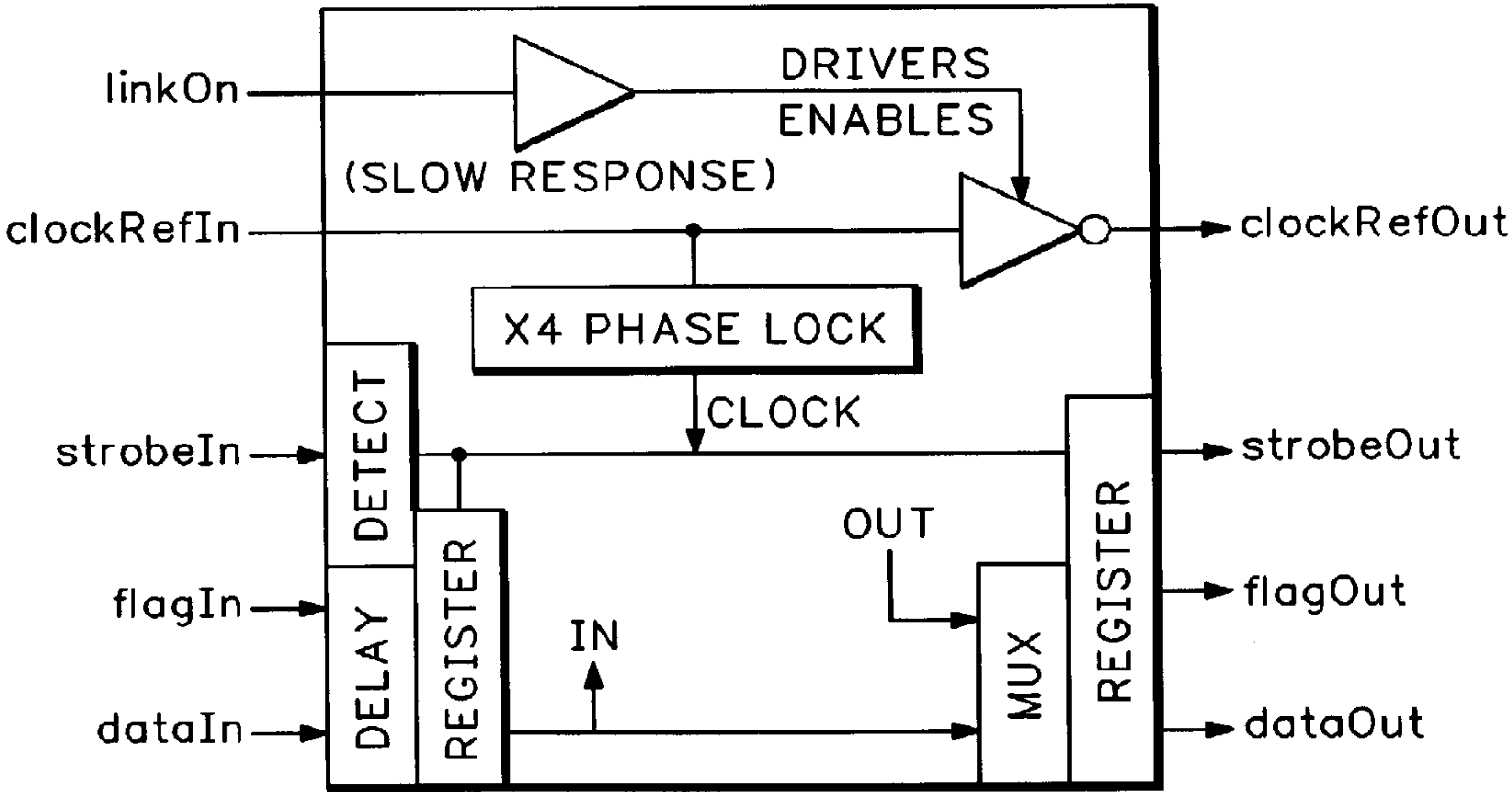
FIG.2 (PRIOR ART)
