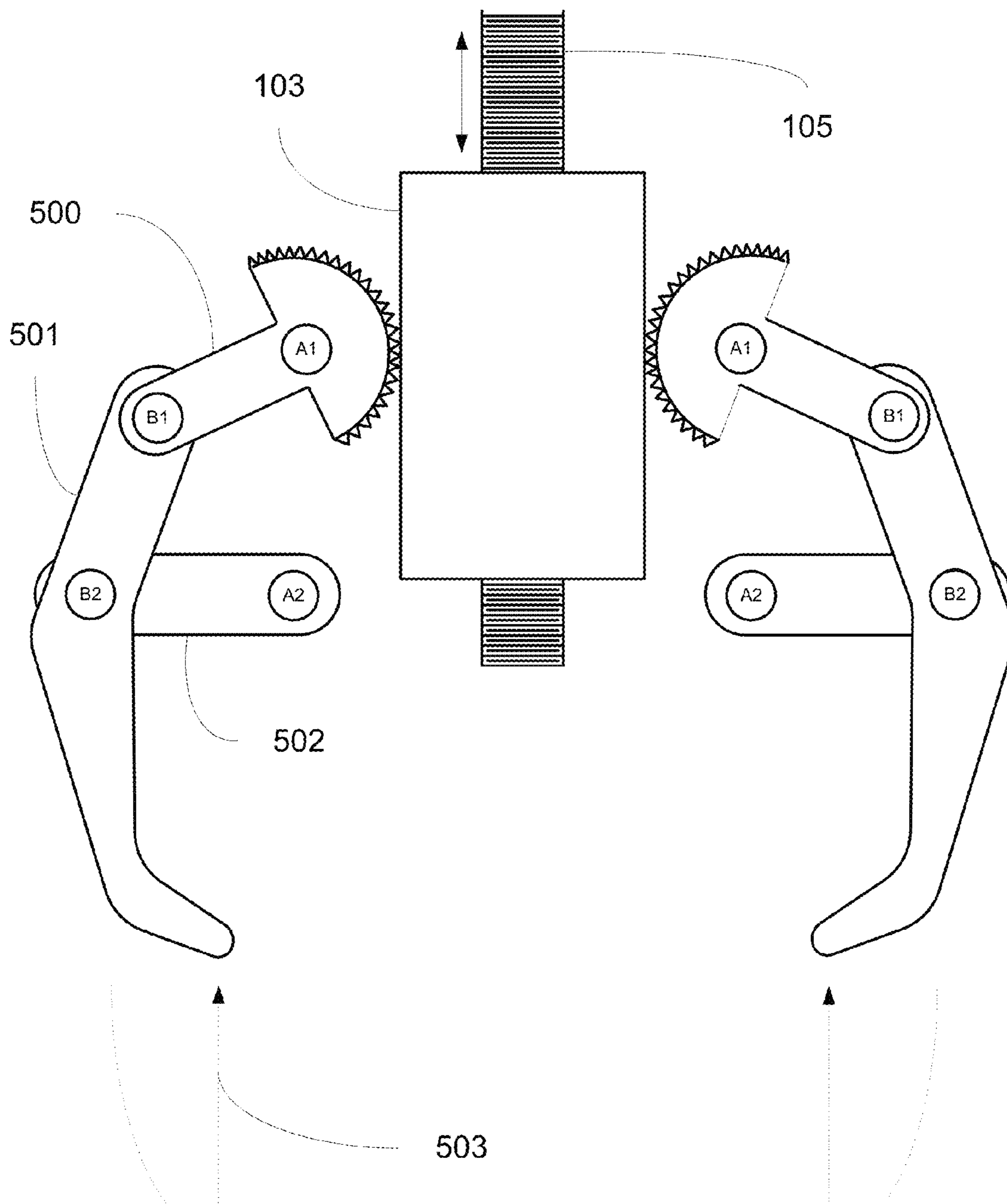
Fig. 5 -- Configuration 1 Linkage Details (Not to Scale)
