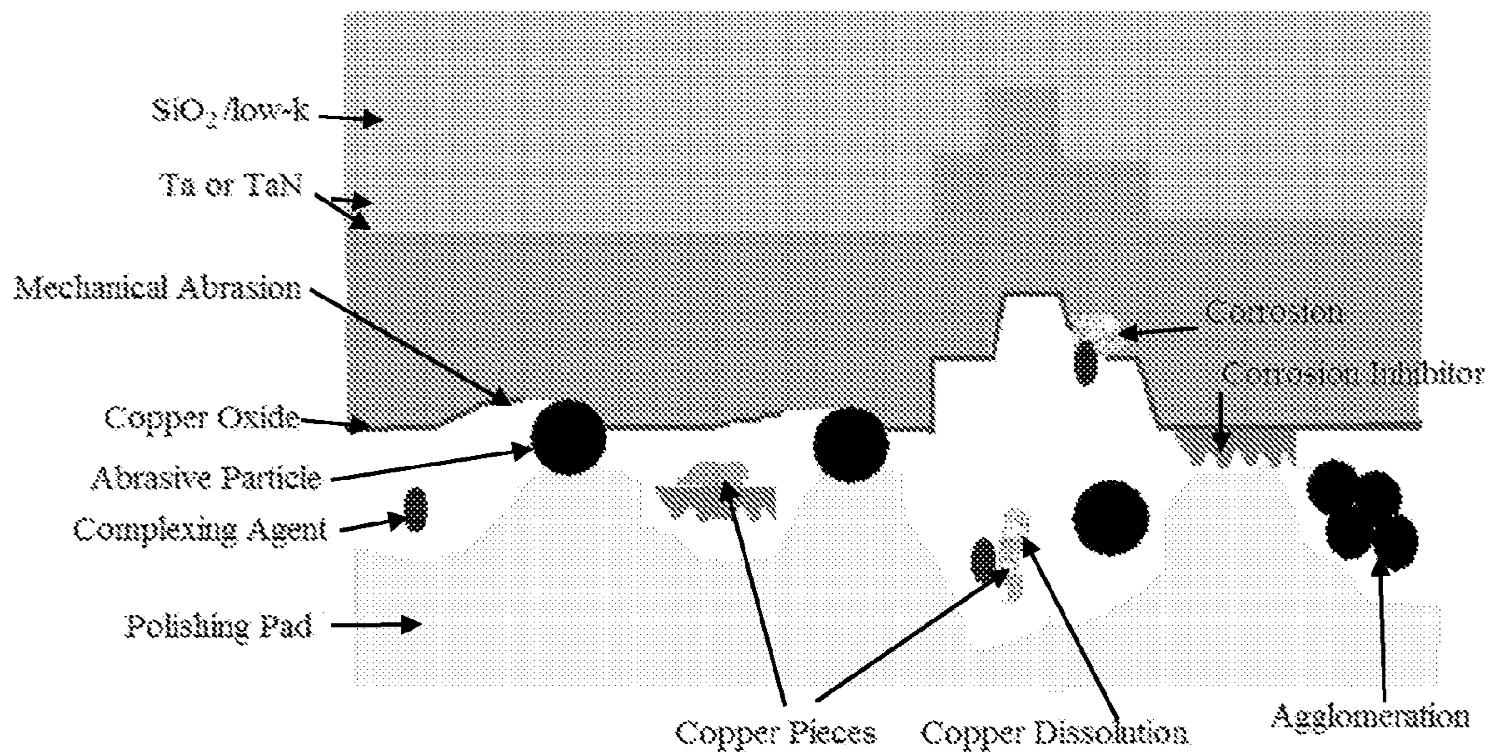
Figure 4 Schematic of typical Copper CMP mechanisms during processing.
