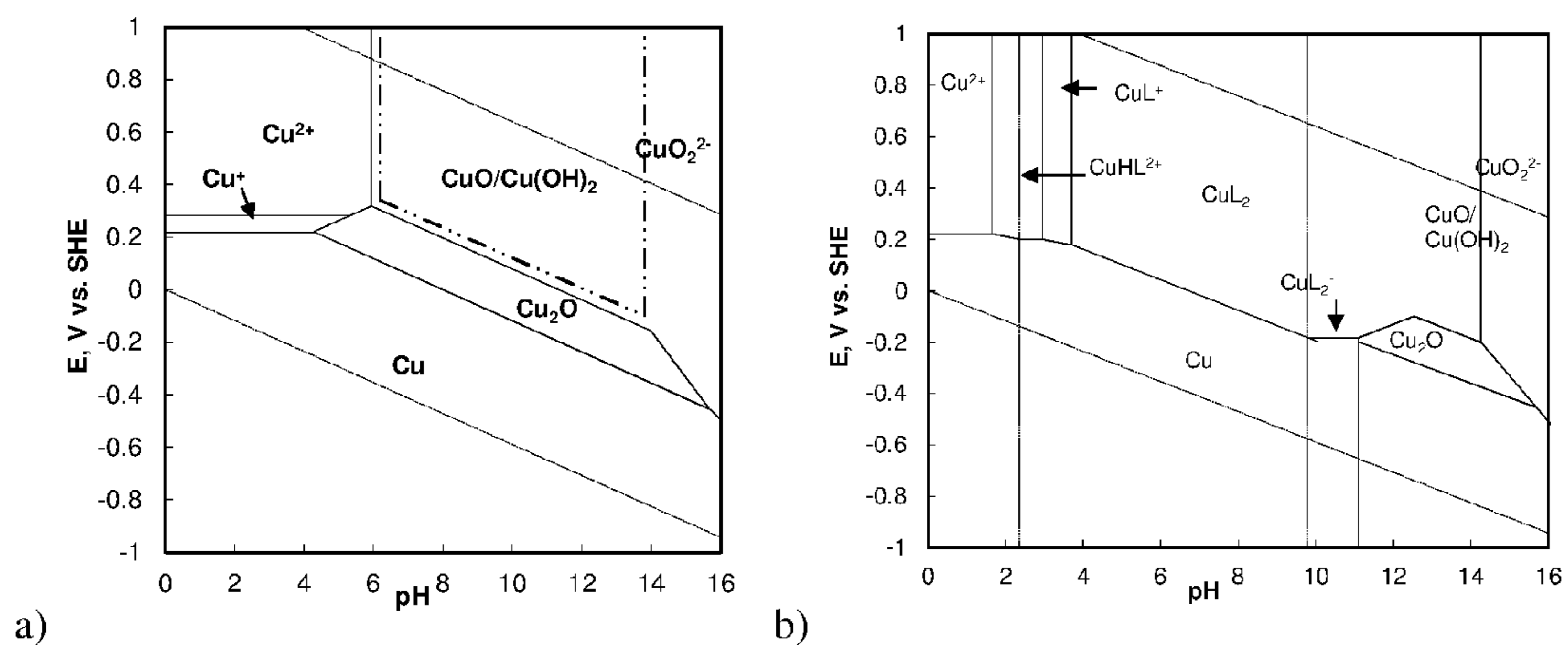
Figure 3 Potential-pH diagram for the a) copper-water and b) copper-water-glycine systems at total dissolved copper activity of 10^{-4}\text{M} and a total glycine activity of 0.1\text{M} at 25^\circ\text{C} and 1\text{ atm} .
