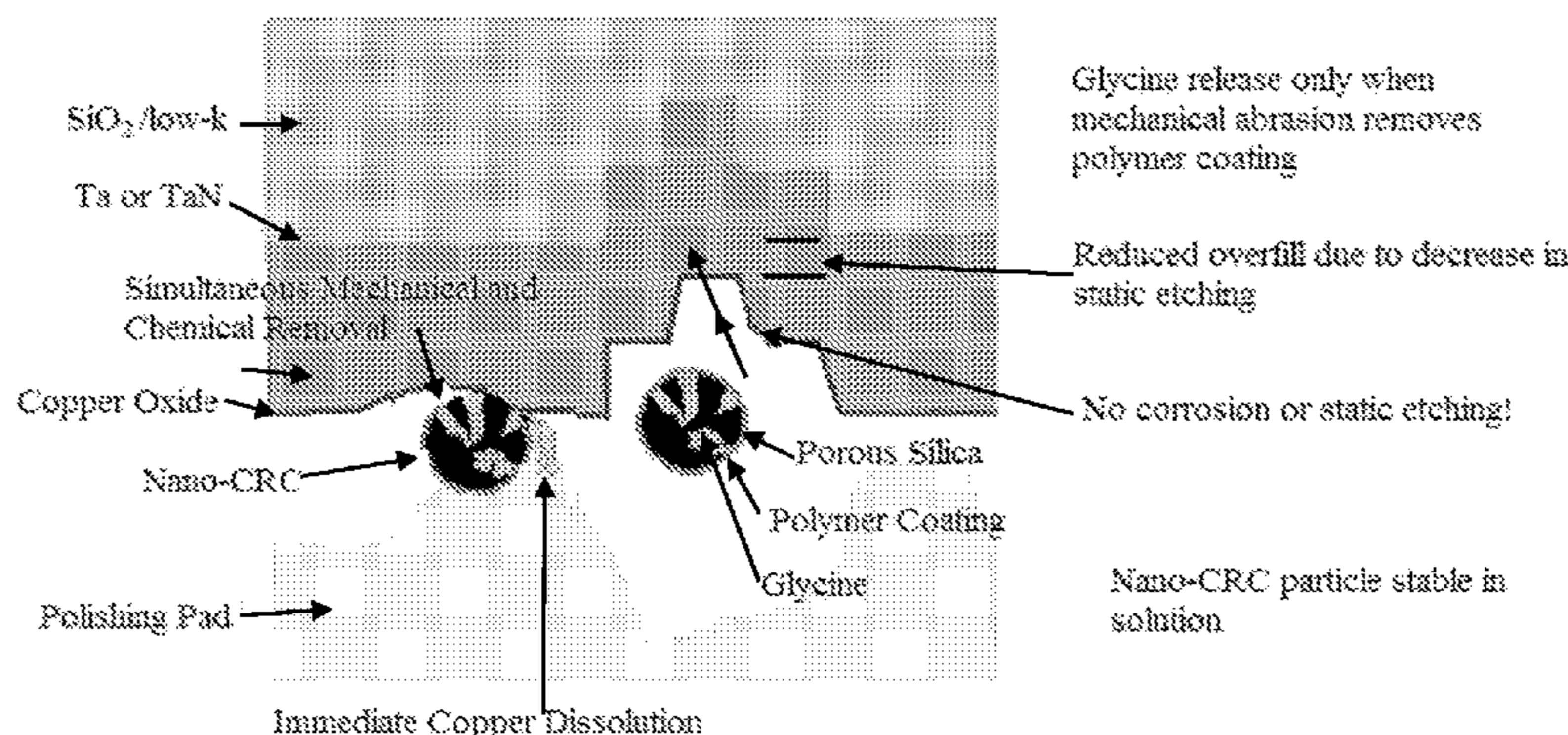
Schematic of removal mechanism for the contact release capsule technology in a copper CMP slurry.
