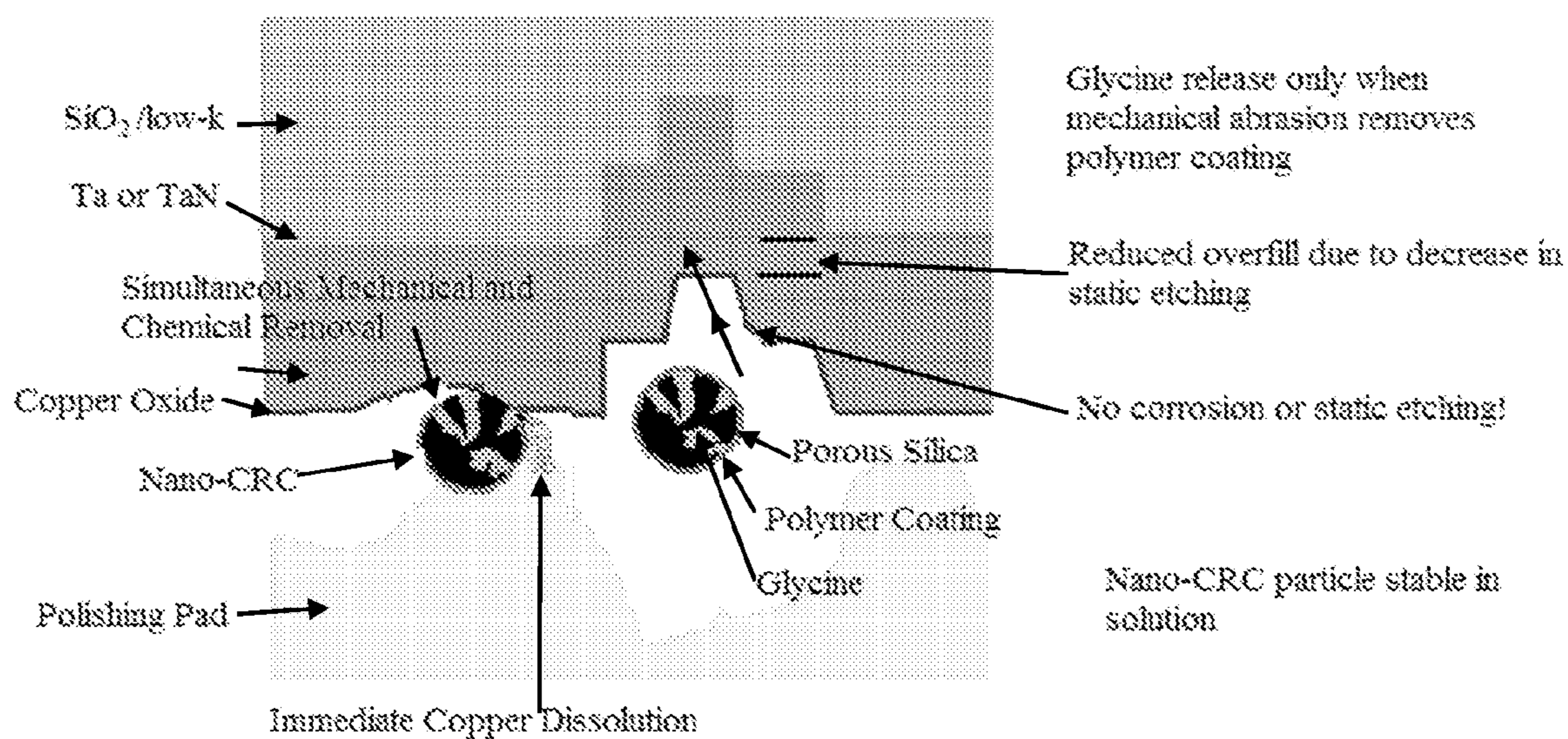
Figure 5 Schematic of removal mechanism for the contact release capsule technology in a copper CMP slurry.
