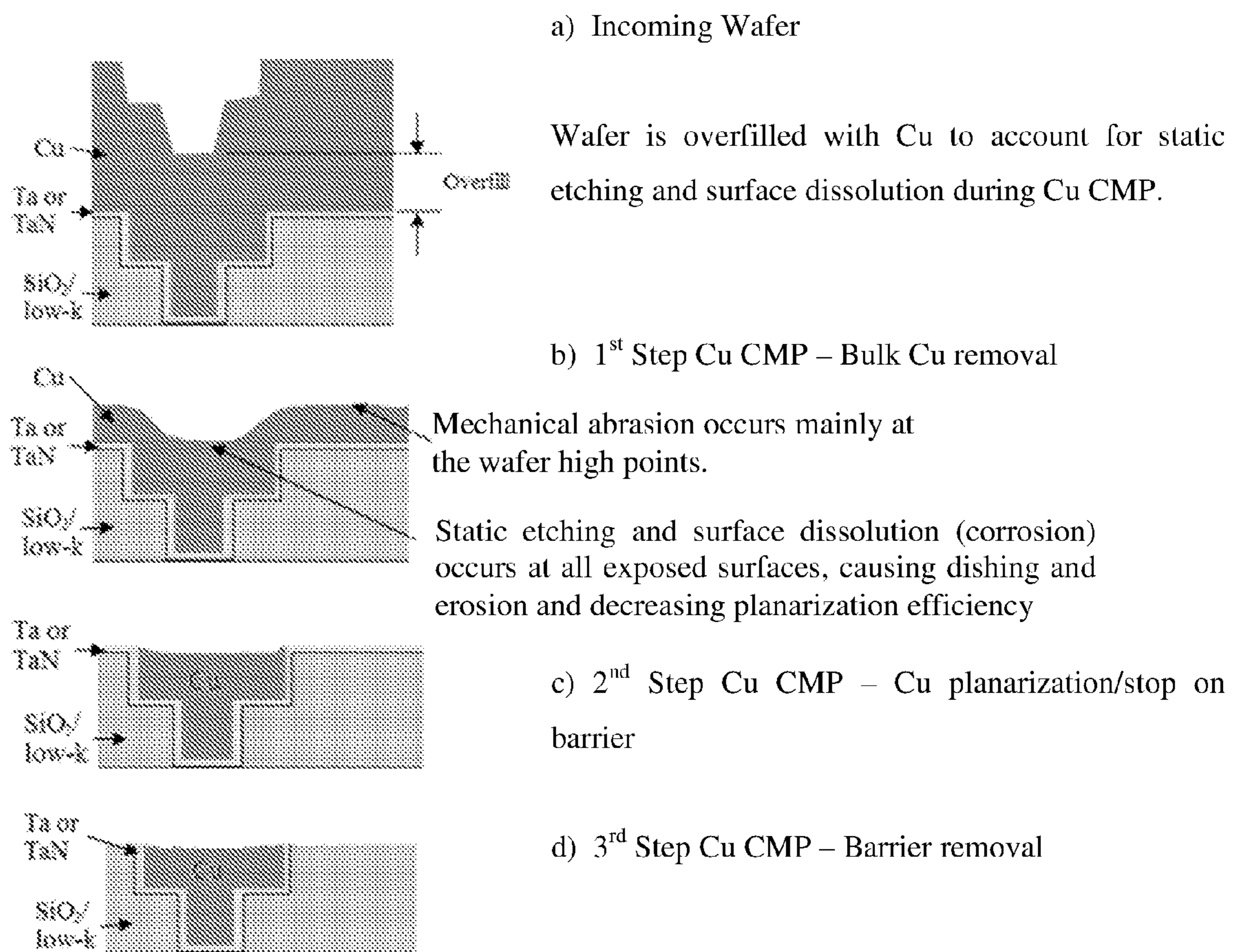
Figure 2 Schematic of the Copper CMP process.
