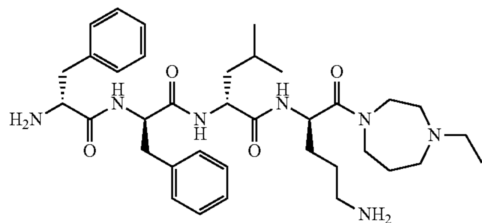
D-Phe-D-Phe-D-Leu-D-Orn-[4-ethylhomopiperazine amide]
