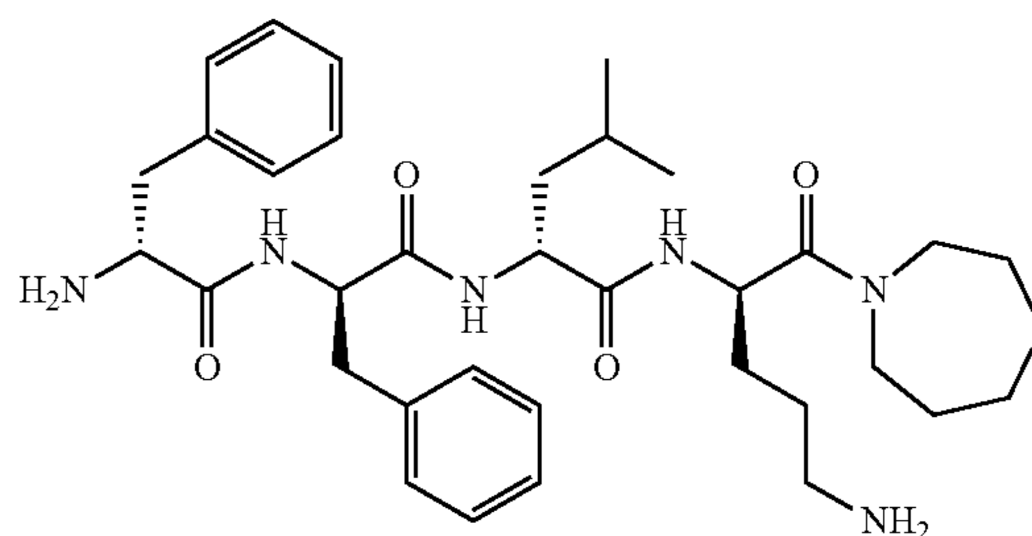
D-Phe-D-Phe-D-Leu-D-Orn-N(homothiomorpholine)
