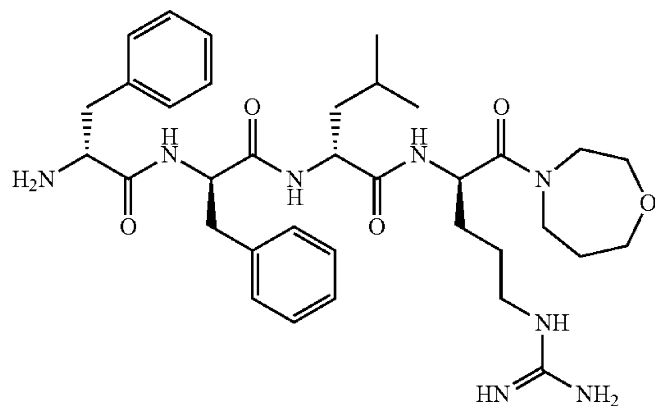
D-Phe-D-Phe-D-Leu-D-Arg-[homomorpholine amide]
