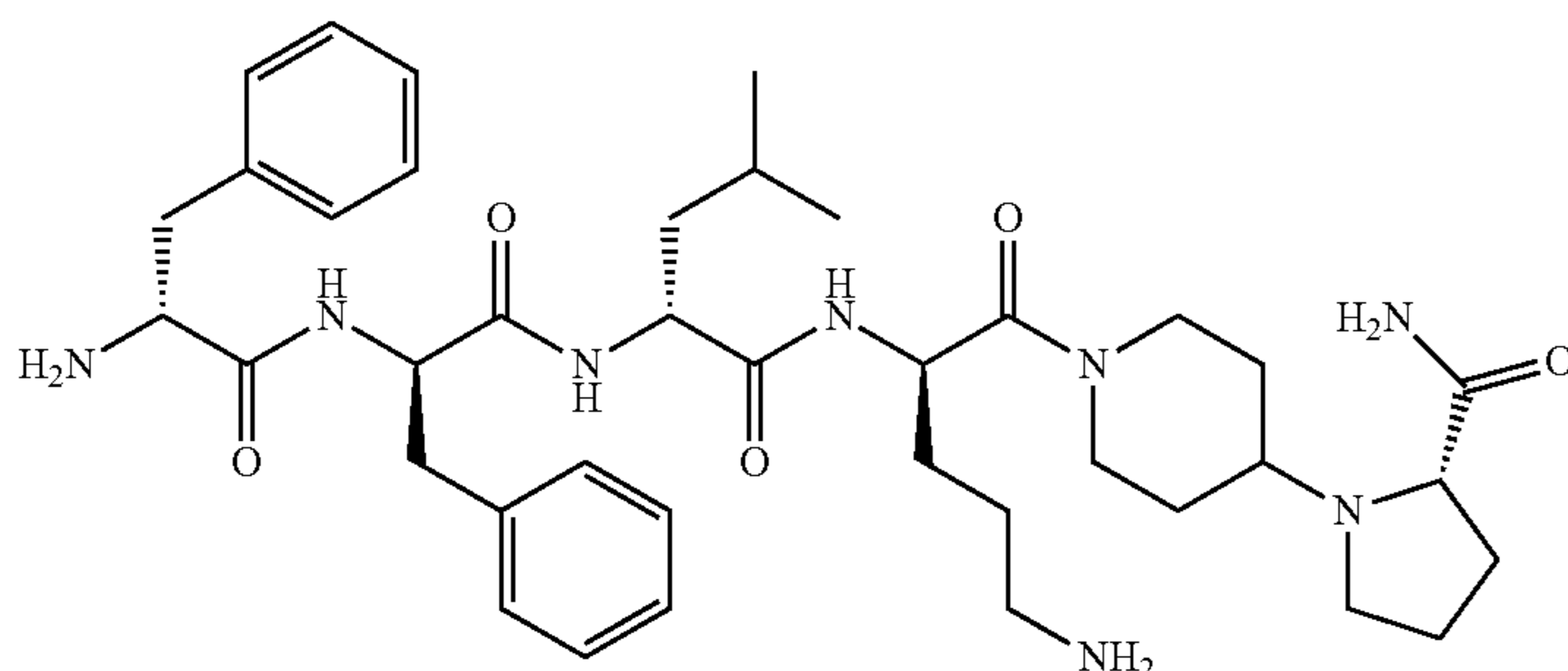
D-Phe-D-Phe-D-Leu-D-Orn-[N-(4-piperidinyl)-L-proline]-NH 2
