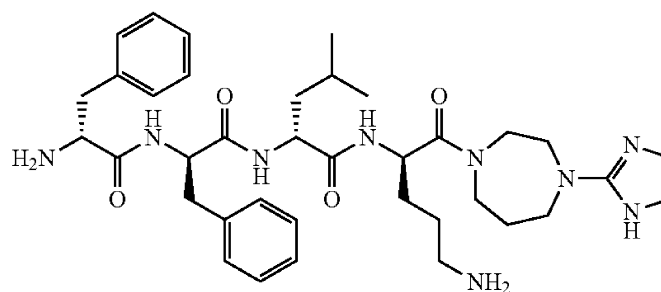
D-Phe-D-Phe-D-Leu-D-Orn-[4-(4,5-dihydro-1H-imidazol-2-yl)homopiperazine amide]
