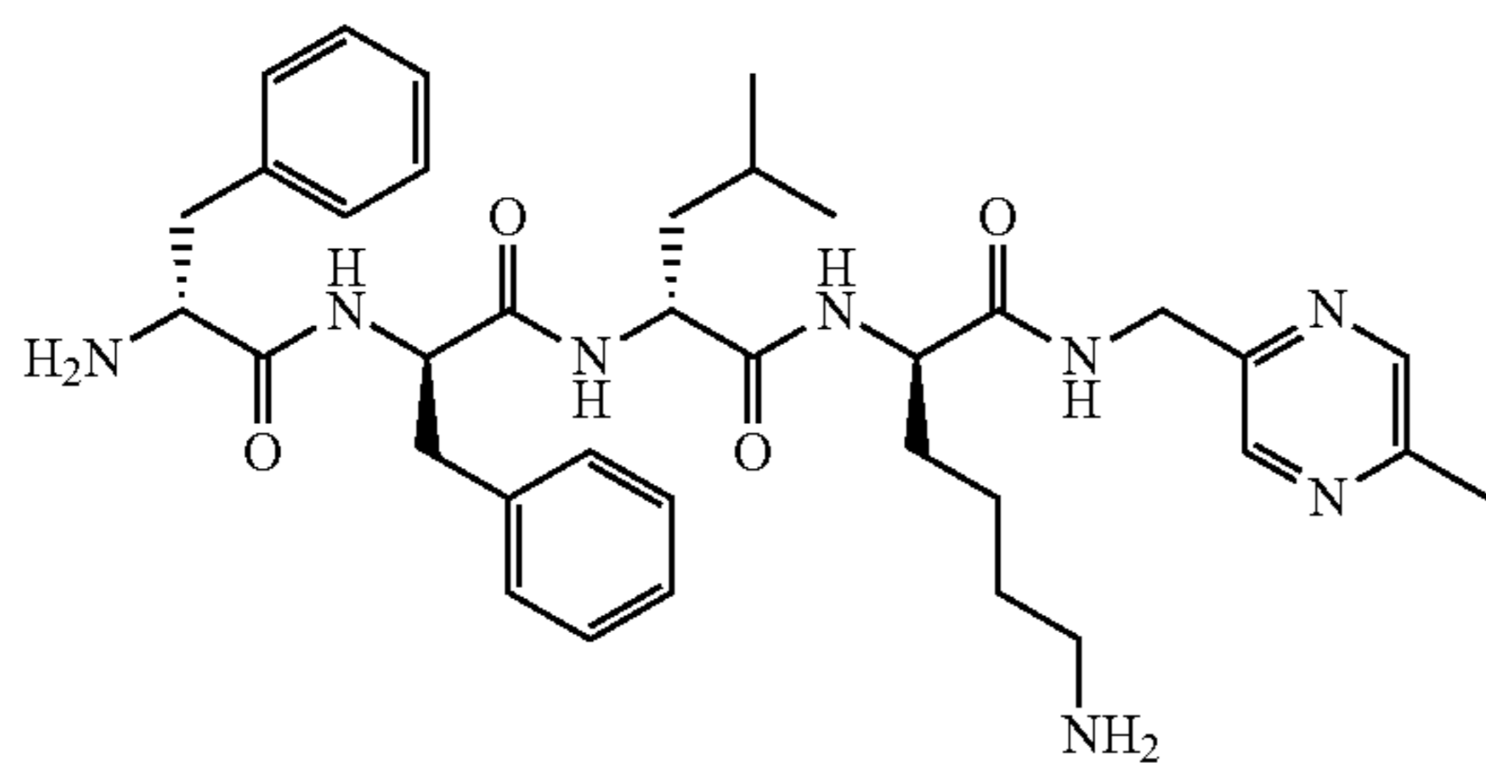
D-Phe-D-Phe-D-Leu-D-Lys-N-methyl-1-(5-methylpyrazin-2-yl)-methanamine amide
