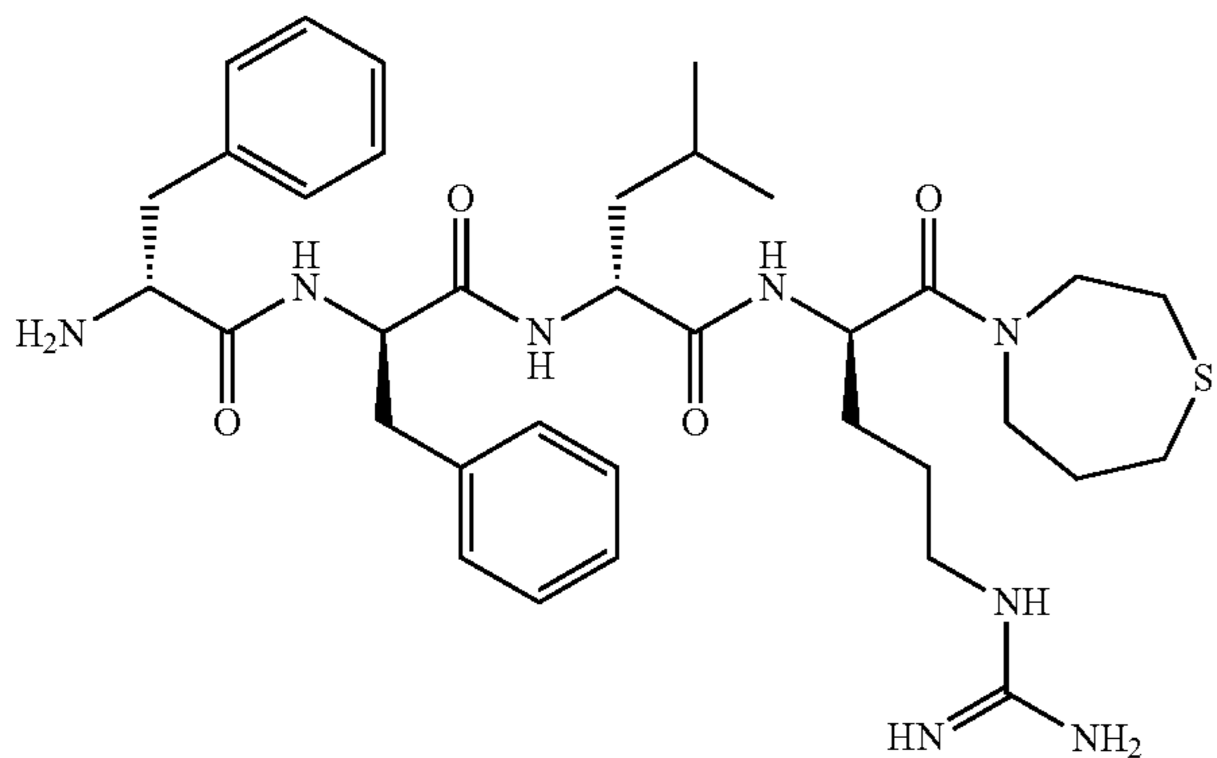
D-Phe-D-Phe-D-Leu-D-Arg-[homothiopiperazine amide]
