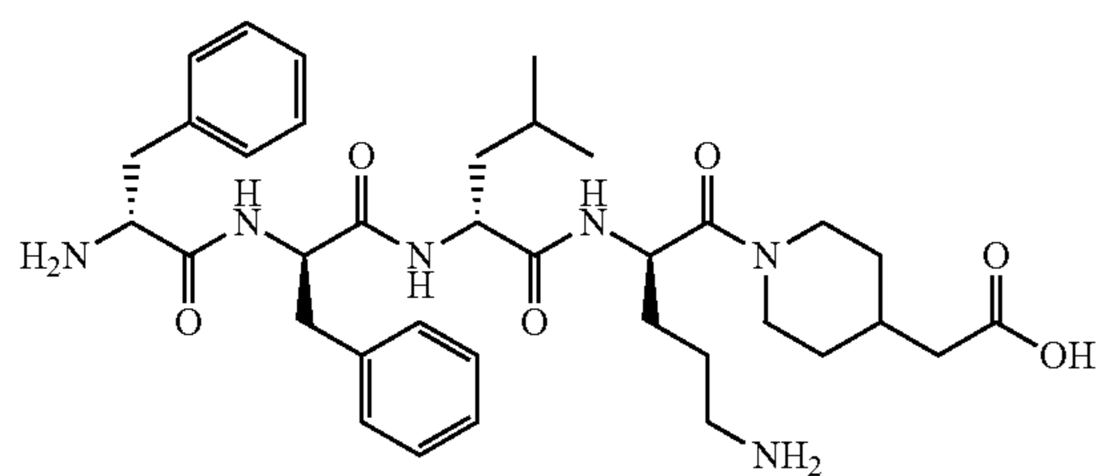
D-Phe-D-Phe-D-Leu-D-Orn-[4-carboxymethyl-piperidine]-OH
