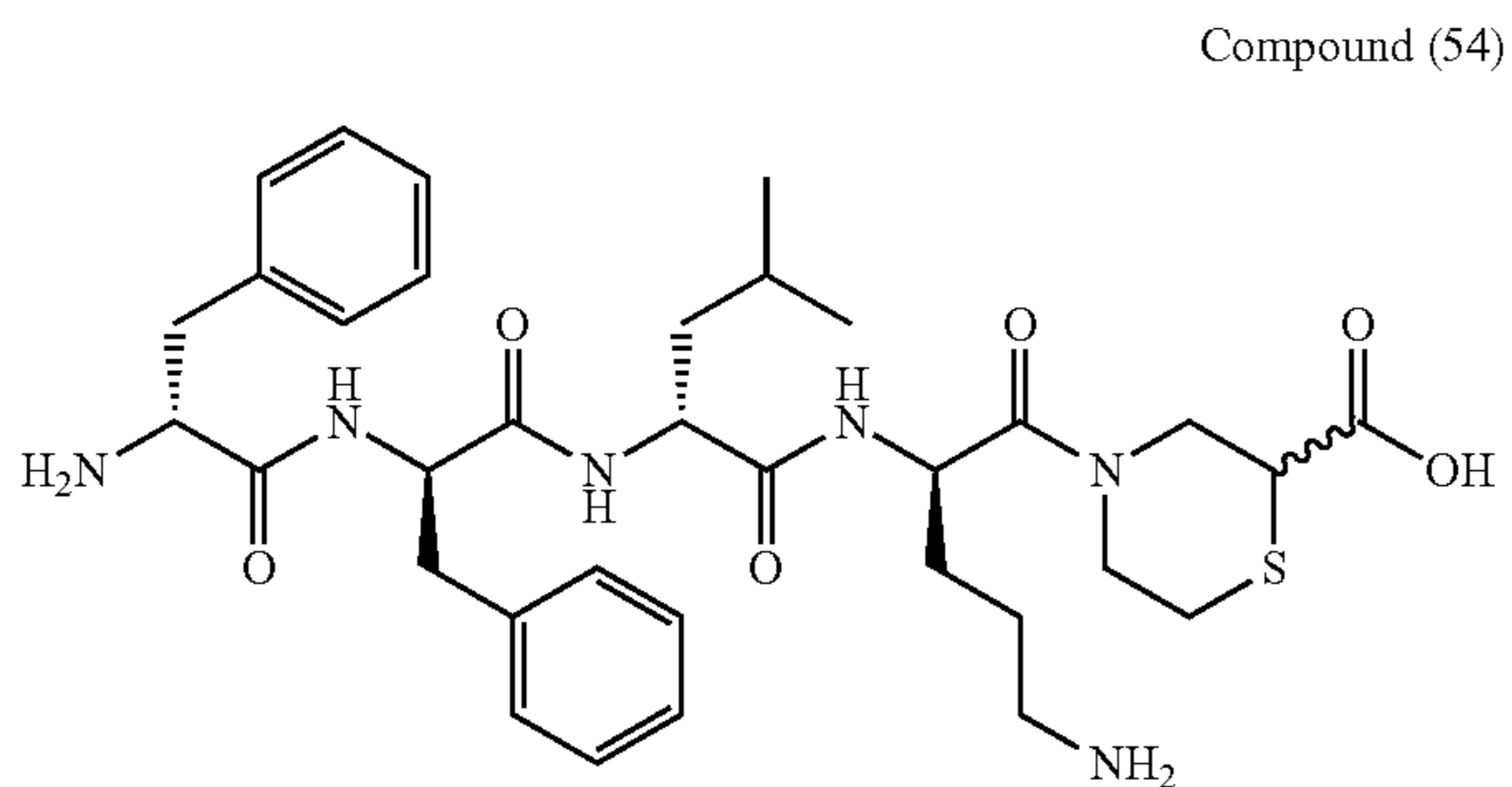
D-Phe-D-Phe-D-Leu-D-Orn-[R/S-2-carboxythiomorpholine]-OH
