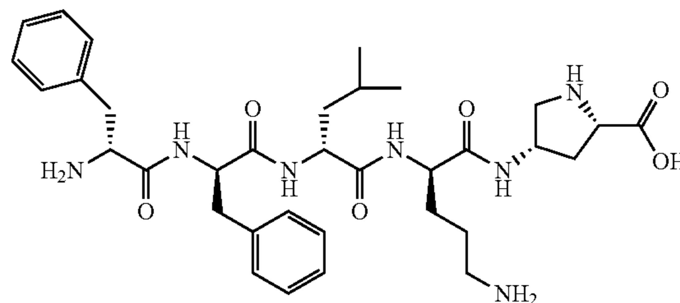
D-Phe-D-Phe-D-Leu-D-Orn-[(2S,4S)-4-amino-pyrrolidine-2-carboxylic acid]-OH
