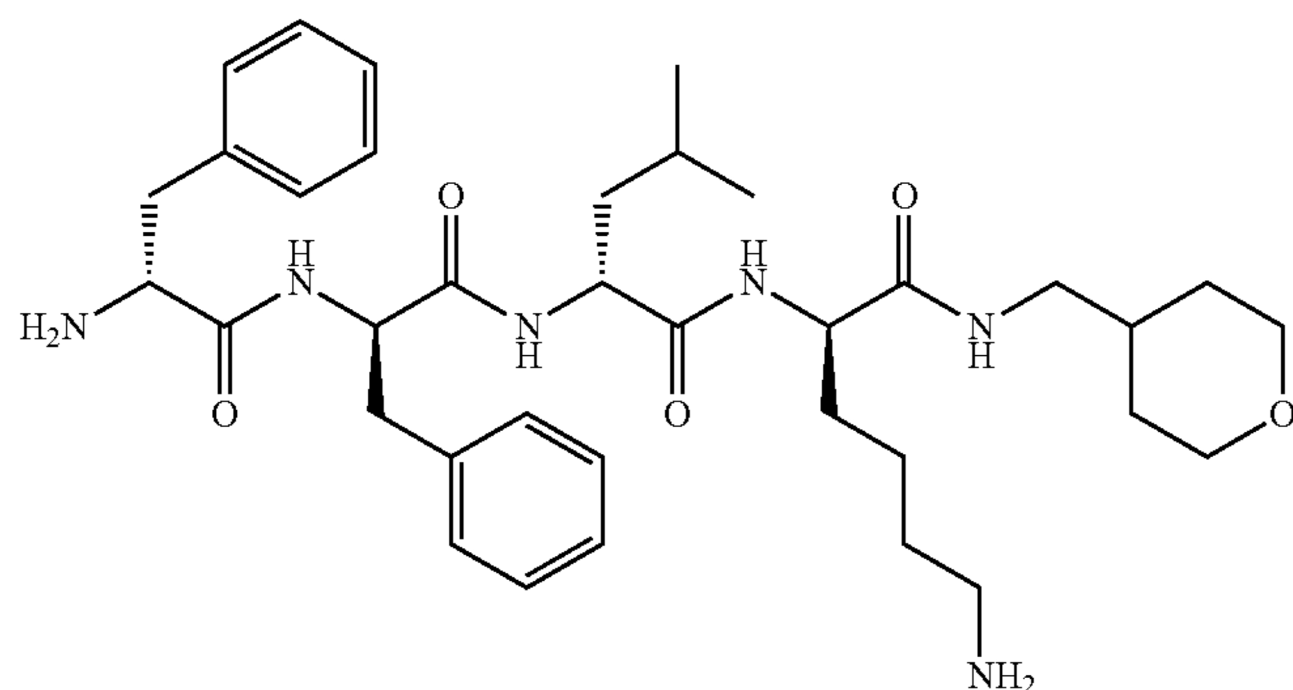
D-Phe-D-Phe-D-Leu-D-Lys-N-methyl-1-(tetrahydro-2H-pyran-4-yl)methanamine amide
