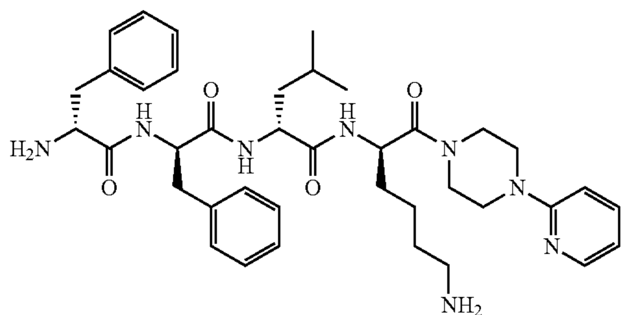
D-Phe-D-Phe-D-Leu-D-Lys-[1-(pyridin-2-yl)piperazine amide]
