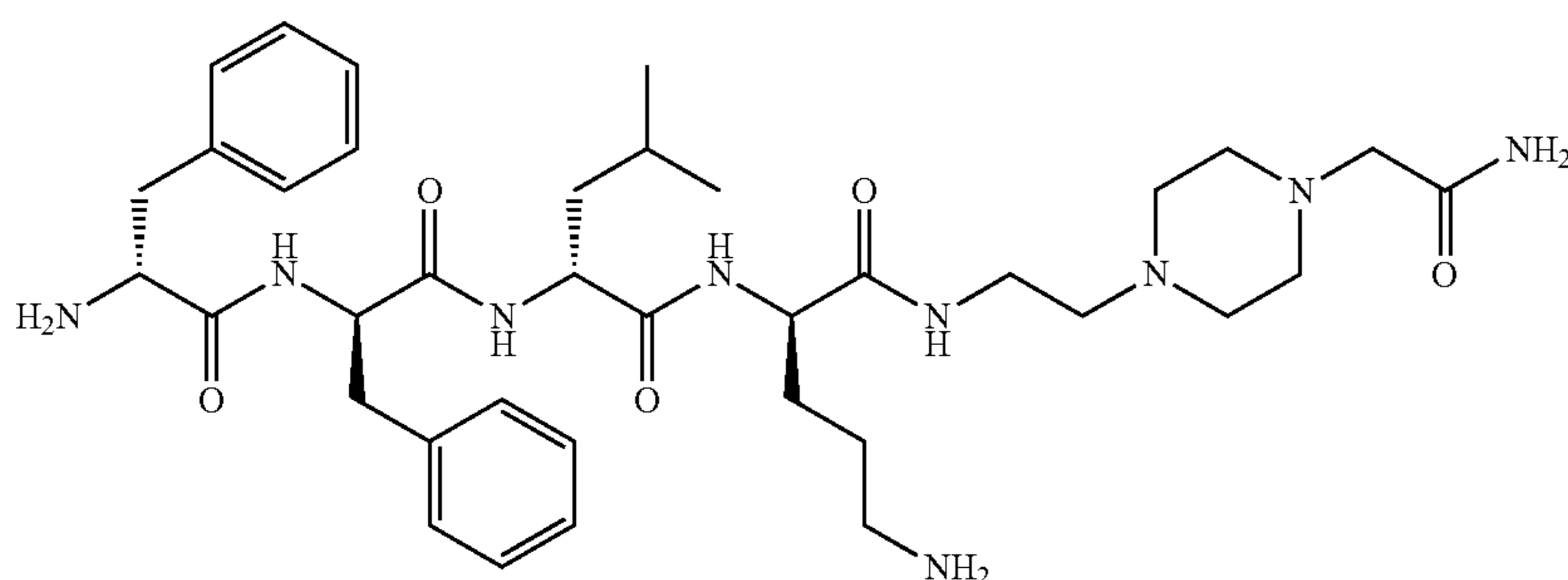
D-Phe-D-Phe-D-Leu-D-Orn-[4-(2-aminoethyl)-1-carboxymethyl-piperazine]-NH 2
