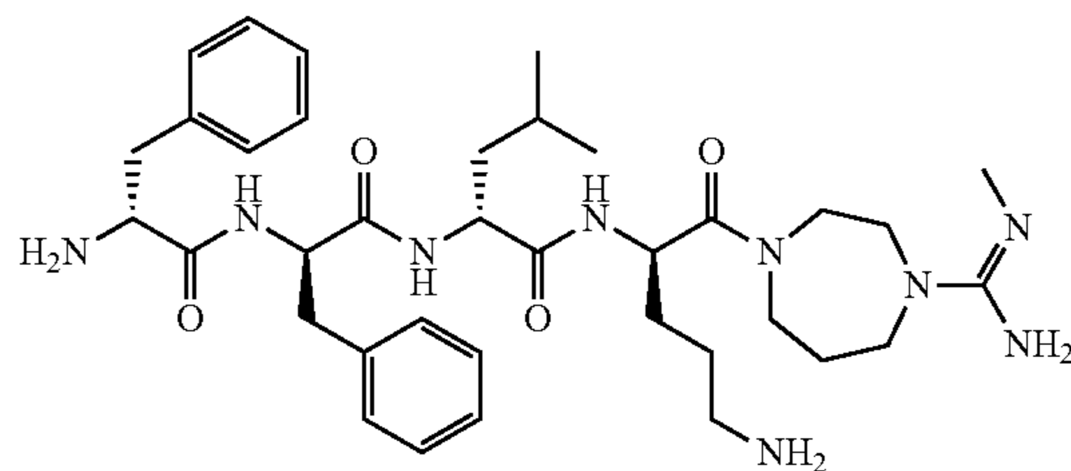
D-Phe-D-Phe-D-Leu-D-Orn-[4-(N-methyl)amidino-homopiperazine amide]
