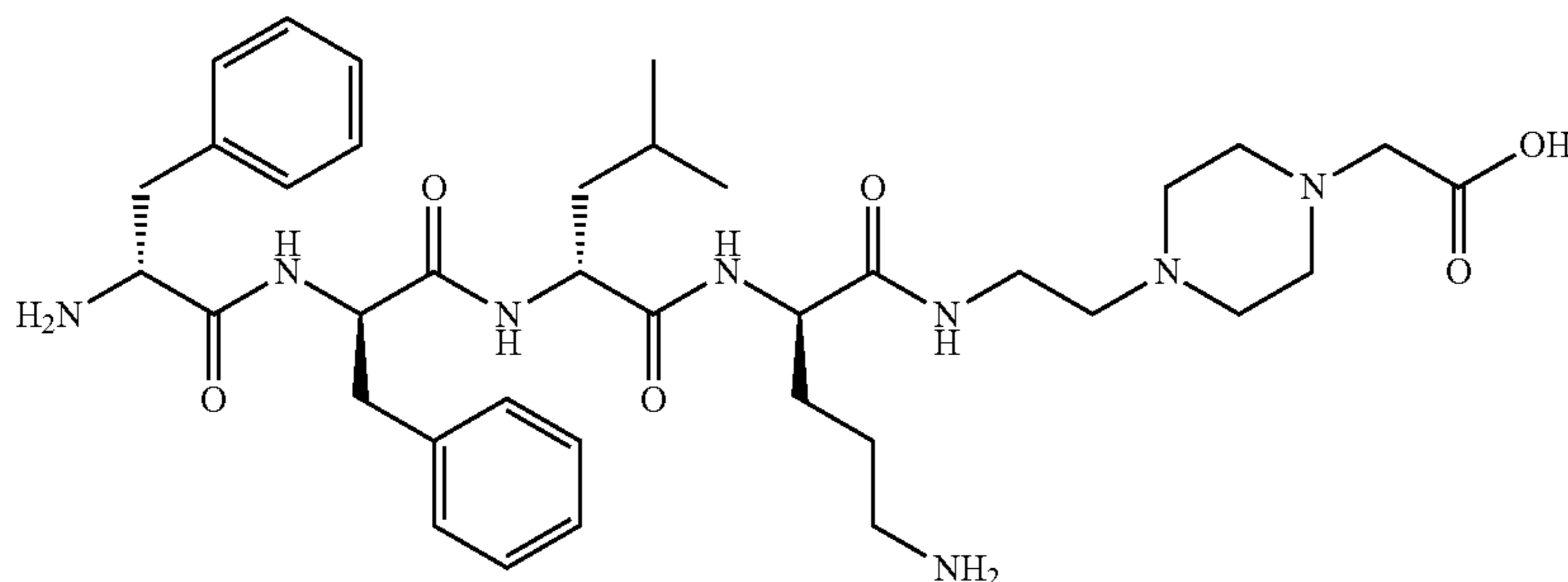
D-Phe-D-Phe-D-Leu-D-Orn-[4-(2-aminoethyl)-1-carboxymethyl-piperazine]-OH
