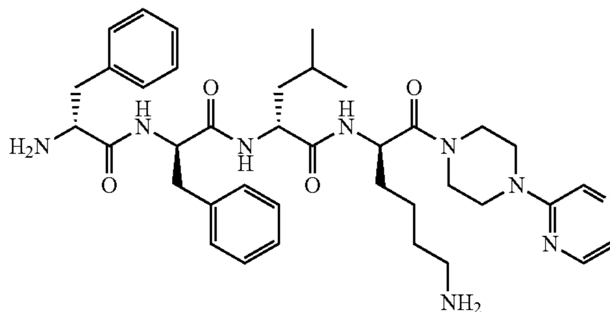
D-Phe-D-Phe-D-Leu-D-Lys-[2-(piperazin-1-yl)pyrazine amide]
