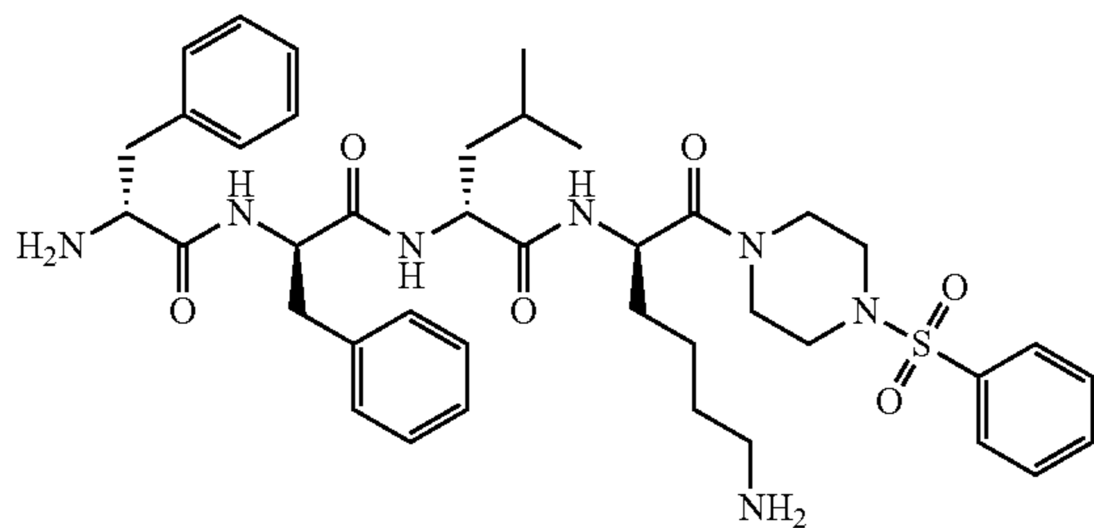
D-Phe-D-Phe-D-Leu-D-Lys-[1-(phenylsulfonyl)piperazine amide]
