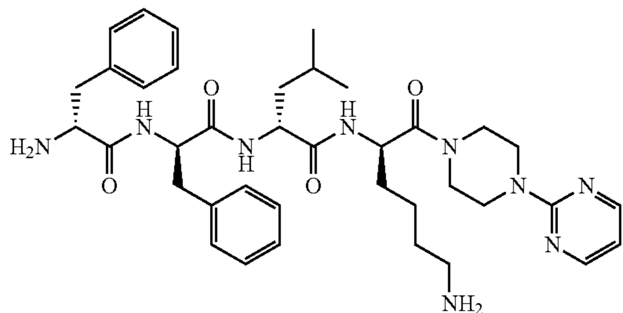
D-Phe-D-Phe-D-Leu-D-Lys-[2-(piperazin-1-yl)pyrimidine amide]
