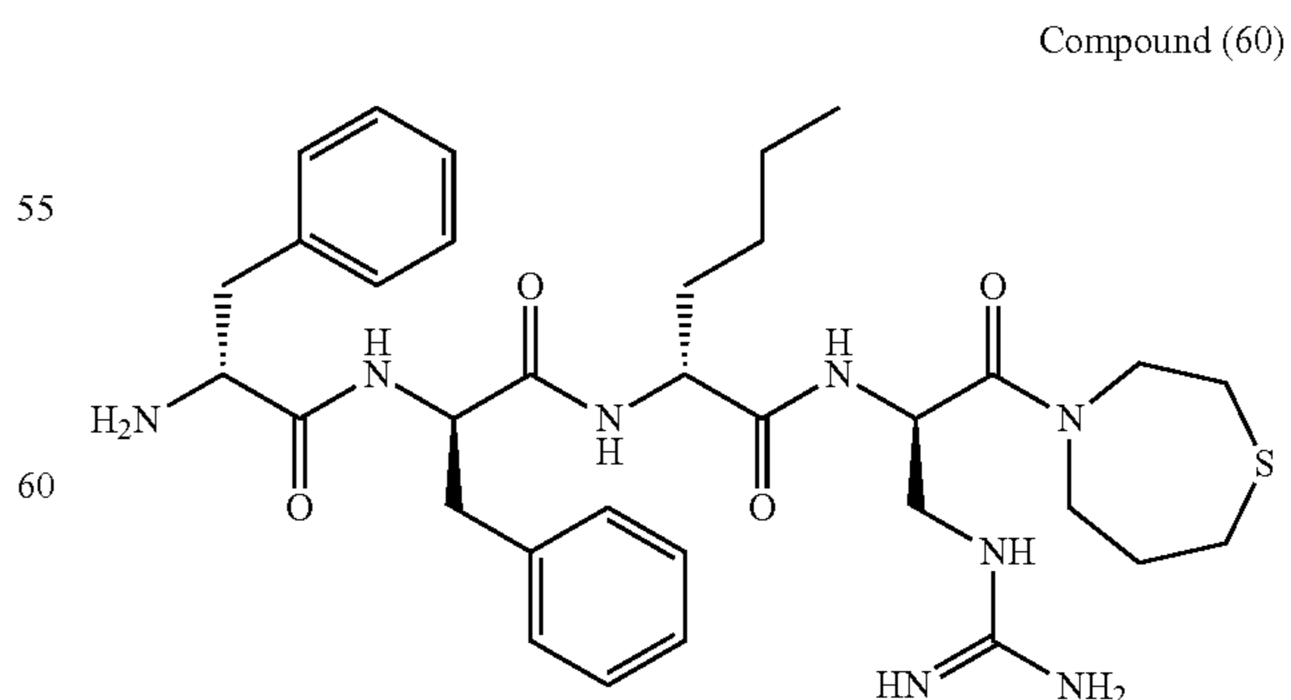
D-Phe-D-Phe-D-Nle-D-Dap(amidino)-[homothiomorpholine amide]
