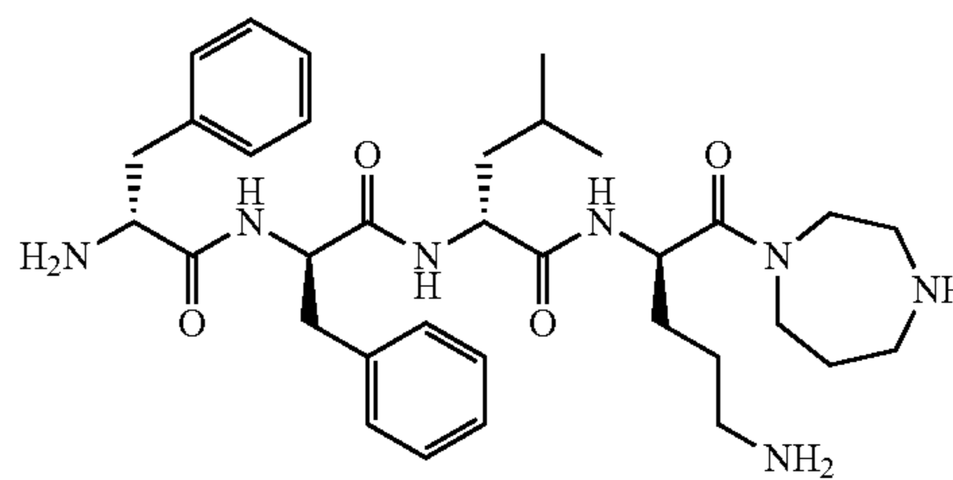
D-Phe-D-Phe-D-Leu-D-Orn-[homopiperazine amide]
