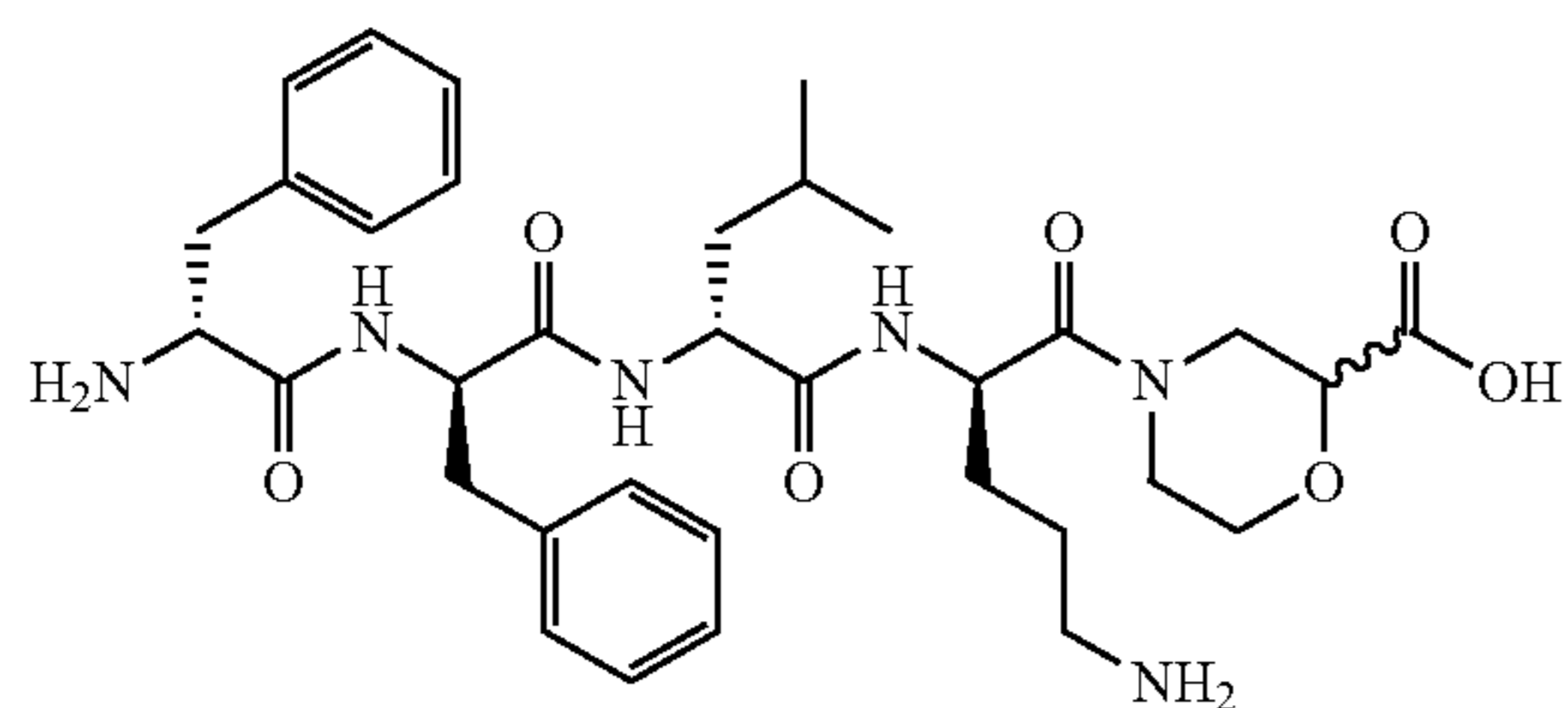
D-Phe-D-Phe-D-Leu-D-Orn-[R/S-2-carboxymorpholine]-OH
