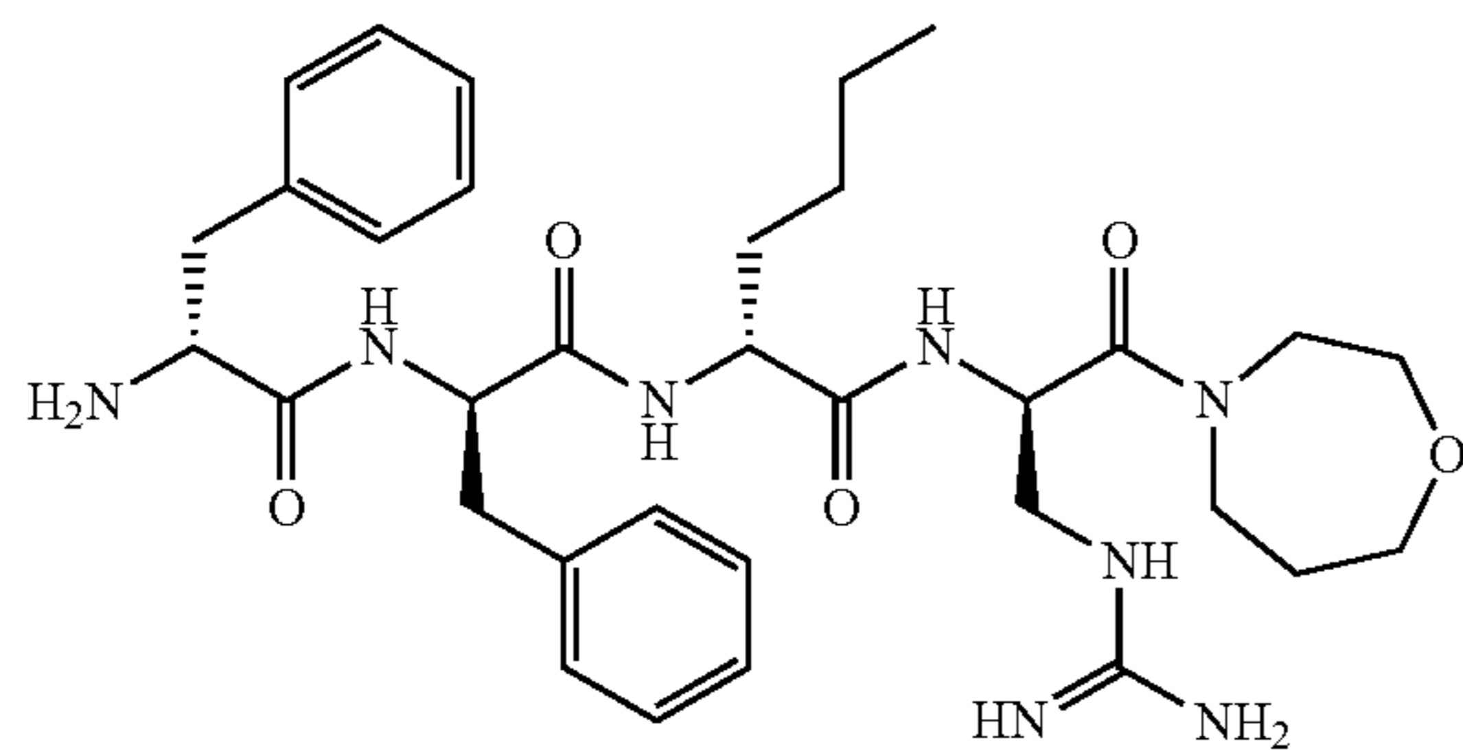
D-Phe-D-Phe-D-Nle-D-Dap(amidino)-[homomorpholine amide]
