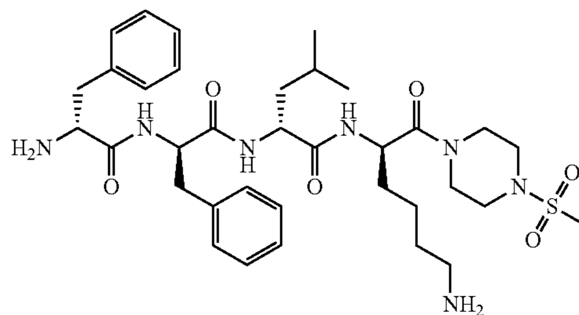
D-Phe-D-Phe-D-Leu-D-Lys-[1-(methylsulfonyl)piperazine amide]
