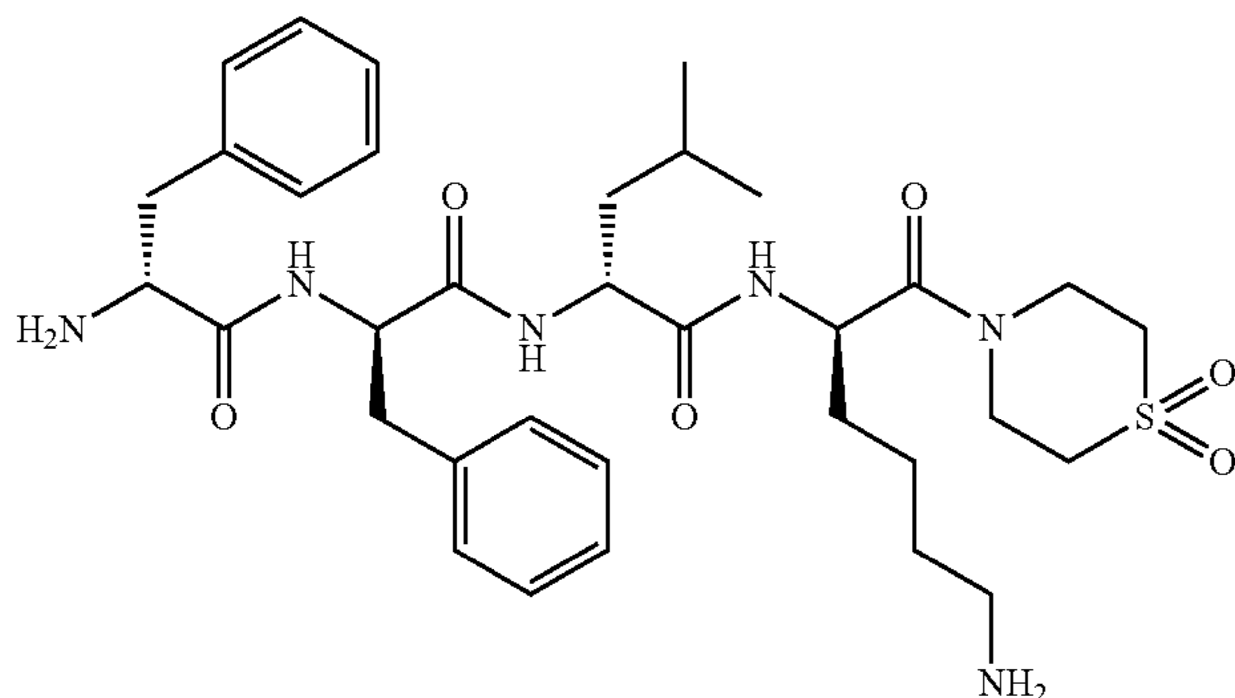
D-Phe-D-Phe-D-Leu-D-Lys-[thiomorpholine-1,1-dioxide amide]
