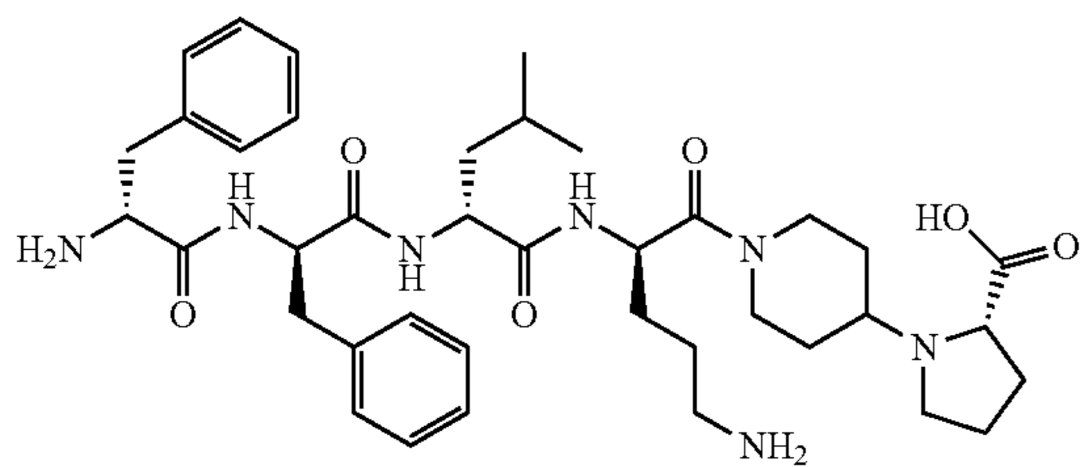
D-Phe-D-Phe-D-Leu-D-Orn-[N-(4-piperidinyl)-L-proline]-OH
