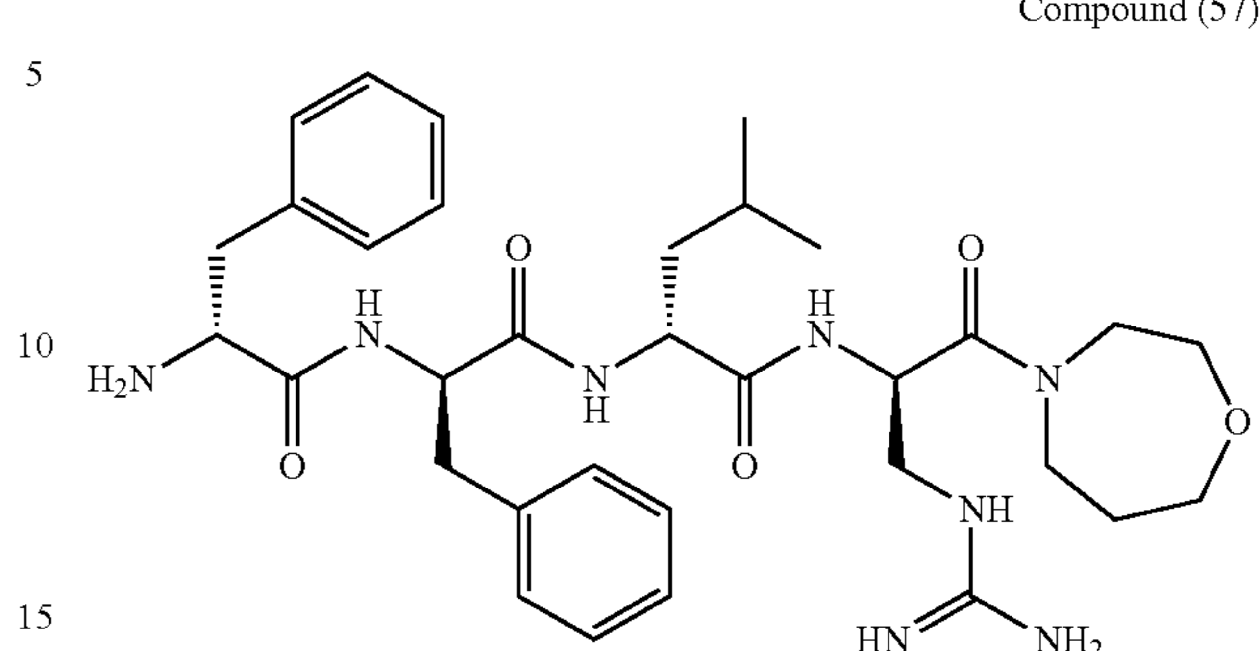
D-Phe-D-Phe-D-Leu-D-Dap(amidino)-[homomorpholine amide]
