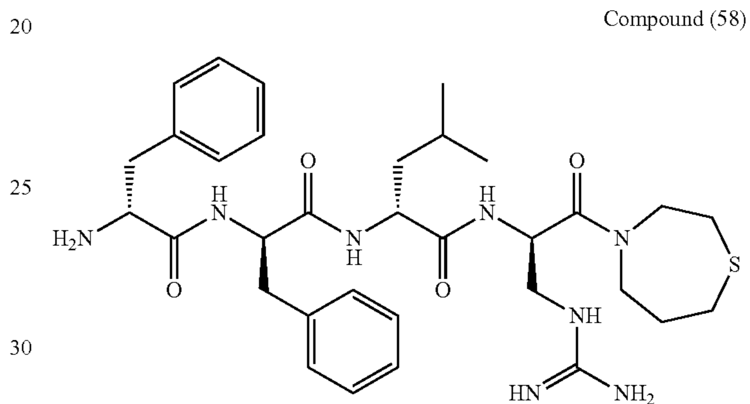
D-Phe-D-Phe-D-Leu-D-Dap(amidino)-[homothiomorpholine amide]
