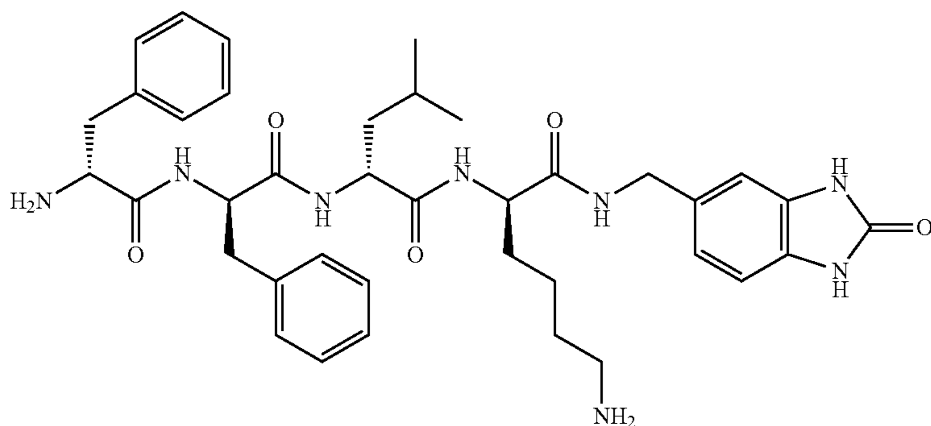
H-D-Phe-D-Phe-D-Leu-D-Lys-[5-(aminomethyl)-1H-benzo[d]imidazol-2(3H)-one amide]
