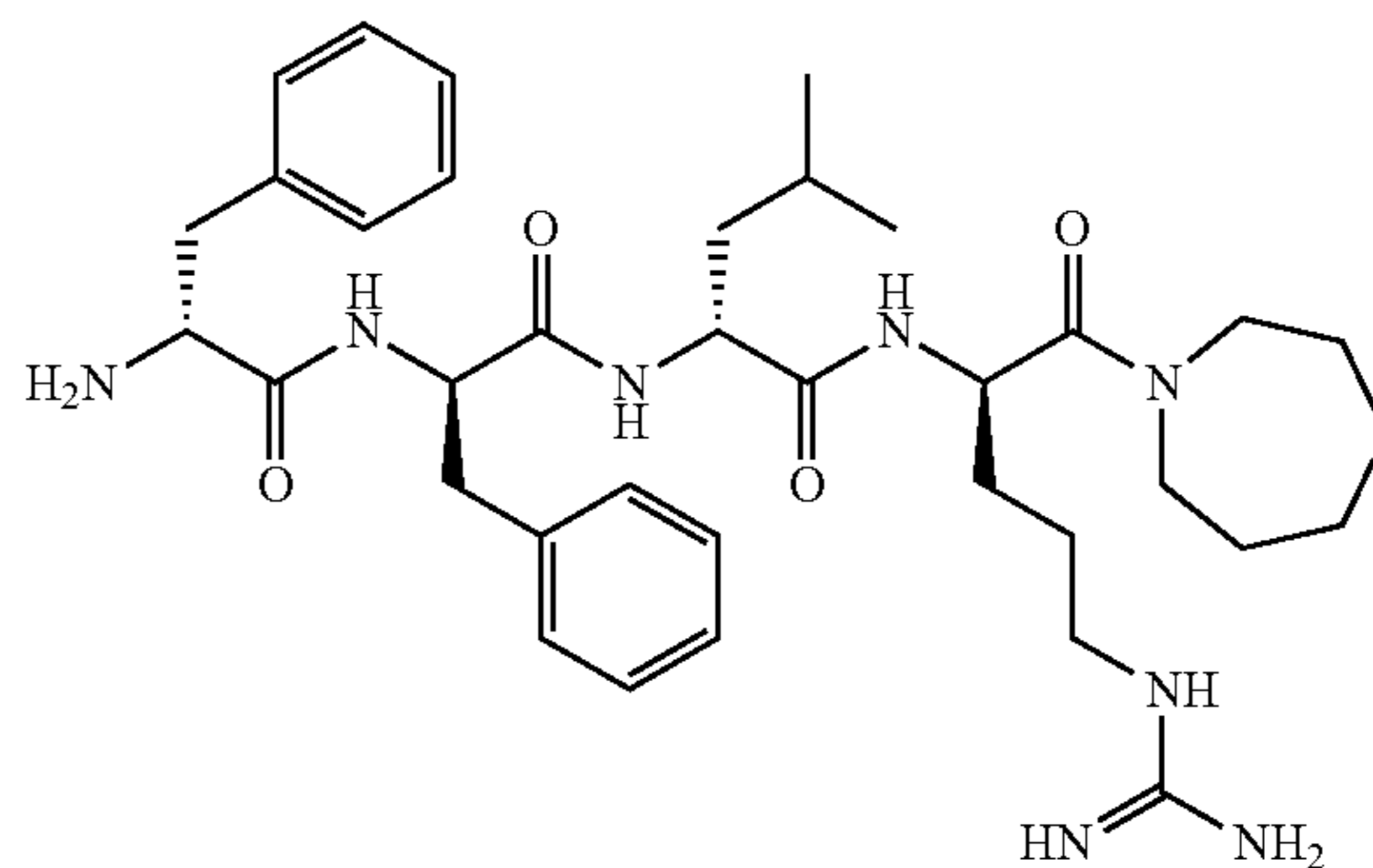
D-Phe-D-Phe-D-Leu-D-Arg-[homothiopiperazine amide]
