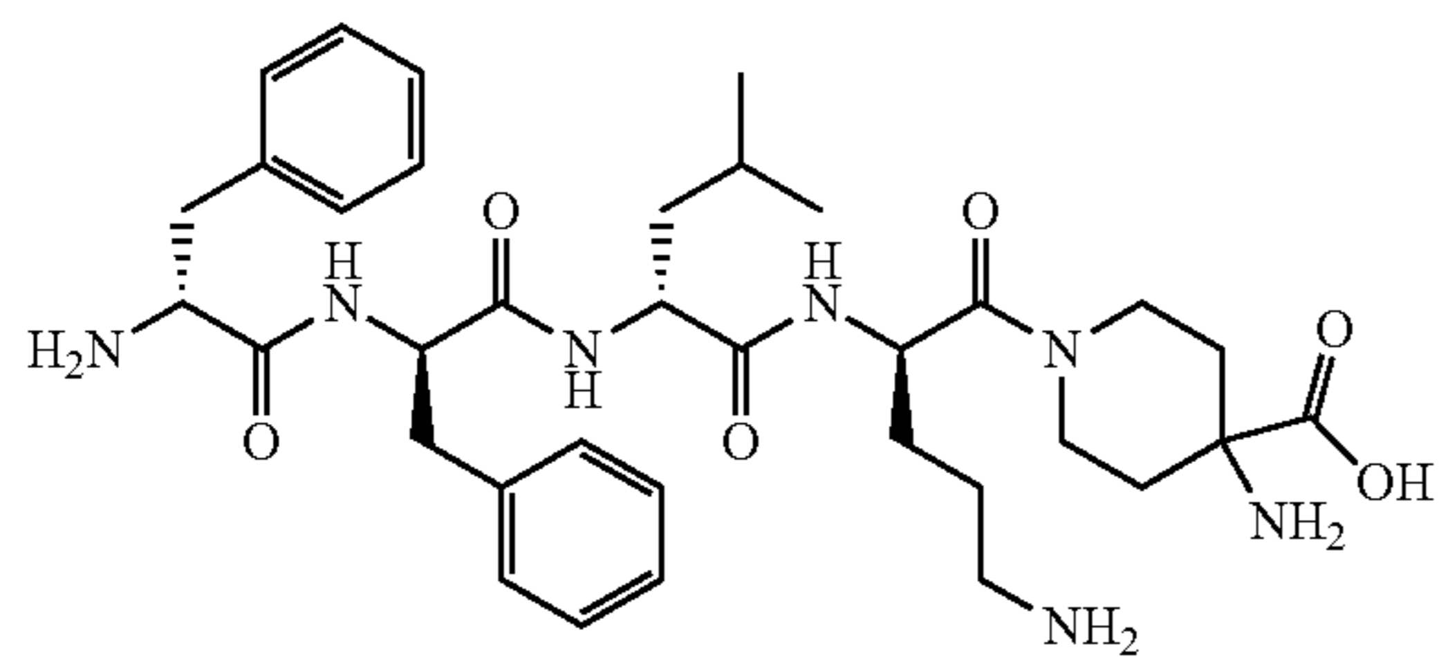
D-Phe-D-Phe-D-Leu-D-Orn-[omega(4-aminopiperidine-4-carboxylic acid)]-OH
