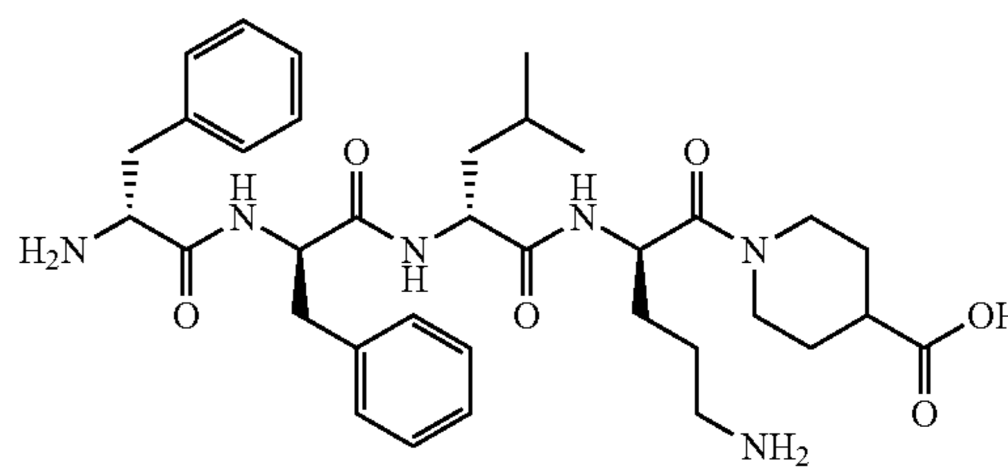
D-Phe-D-Phe-D-Leu-D-Orn-[Isonipepic acid]-OH
