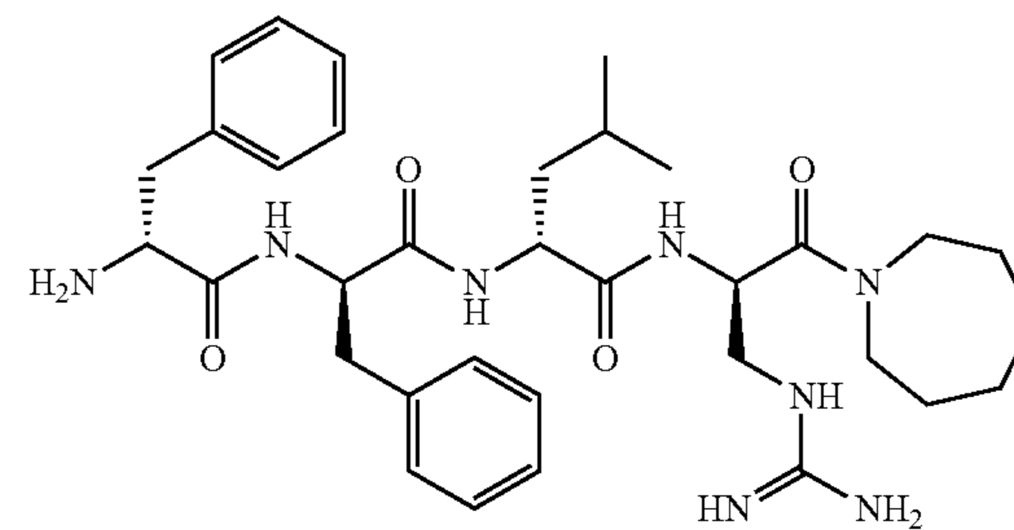
D-Phe-D-Phe-D-Leu-D-Dap(amidino)-[homothiomorpholine amide]
