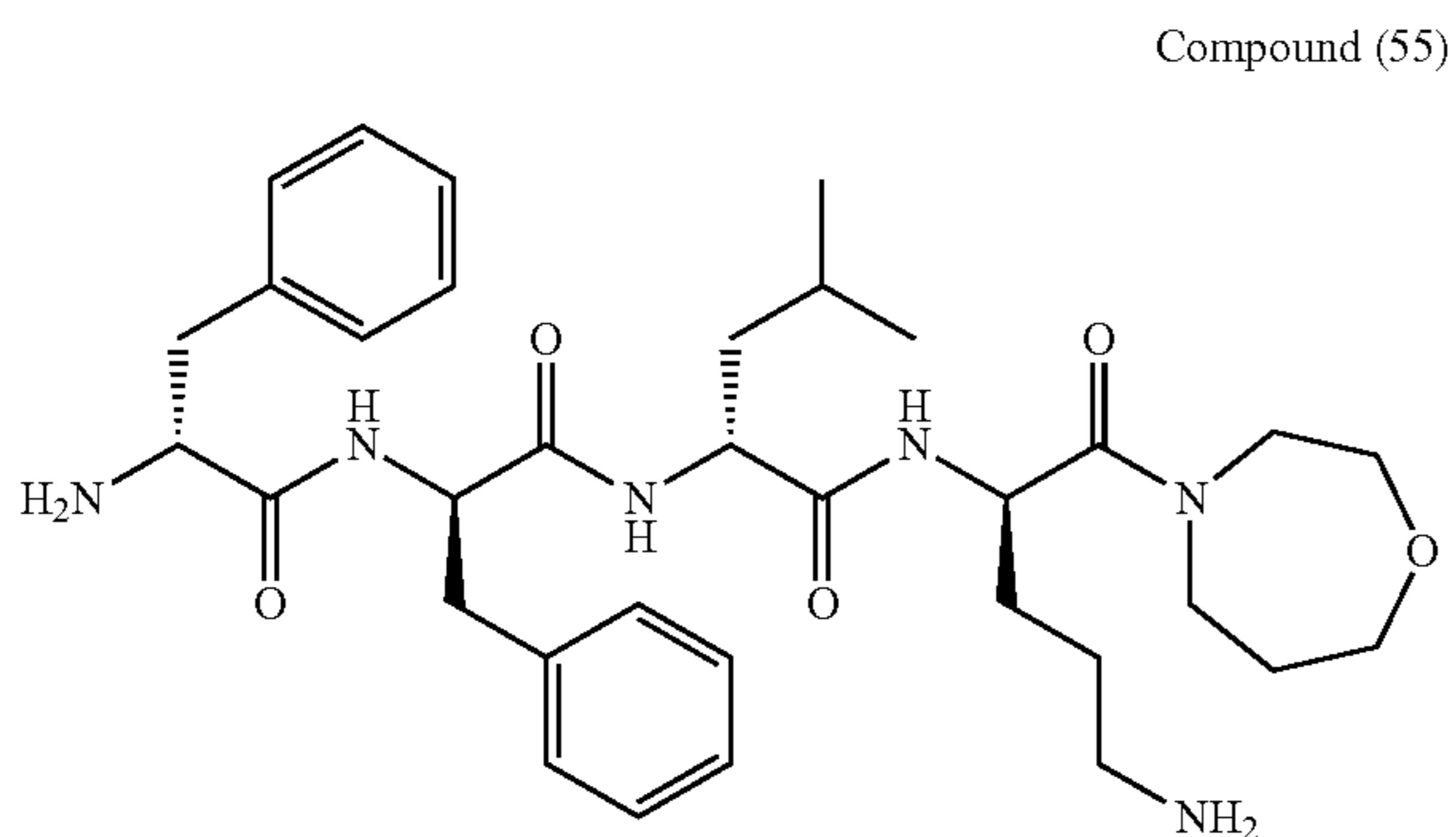
D-Phe-D-Phe-D-Leu-D-Orn-N(homomorpholine)
