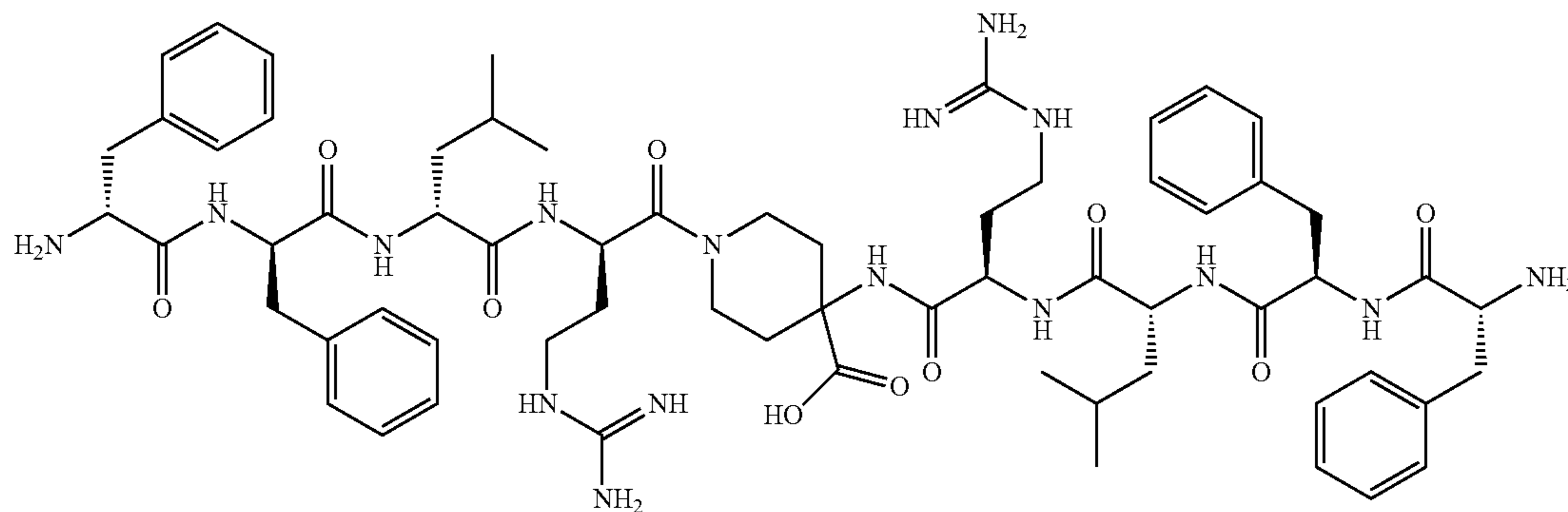
1N,4N-bis-(D-Phe-D-Phe-D-Leu-D-Nar)-4-amino-4-carboxylic piperidine
