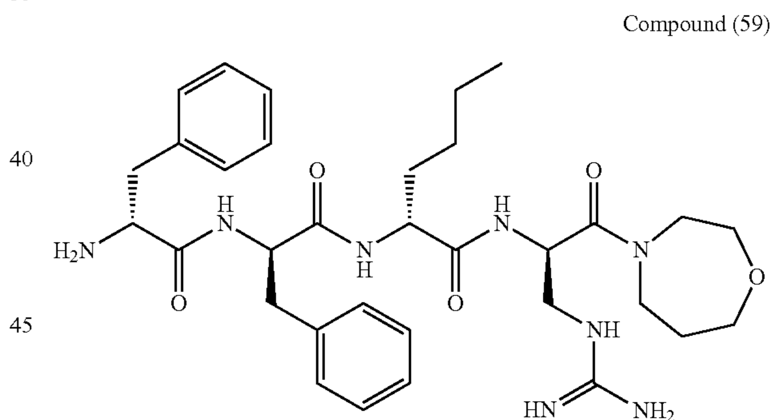
D-Phe-D-Phe-D-Nle-D-Dap(amidino)-[homomorpholine amide]
