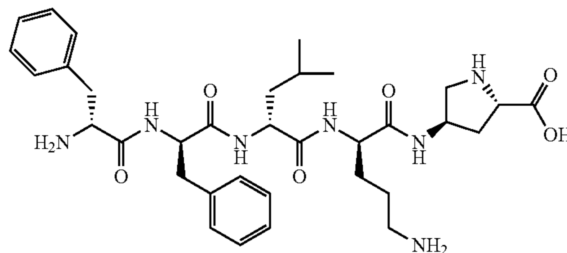
D-Phe-D-Phe-D-Leu-D-Orn-[(2S,4R)-4-amino-pyrrolidine-2-carboxylic acid]-OH
