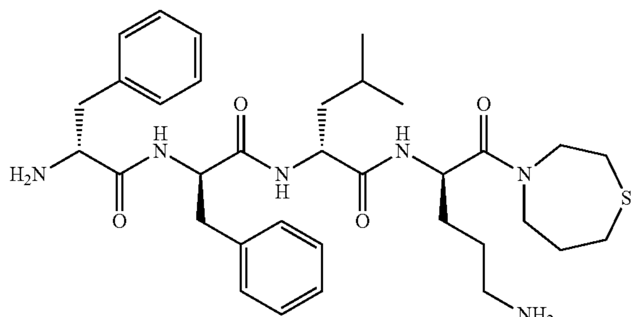
D-Phe-D-Phe-D-Leu-D-Orn-N(homothiomorpholine)
