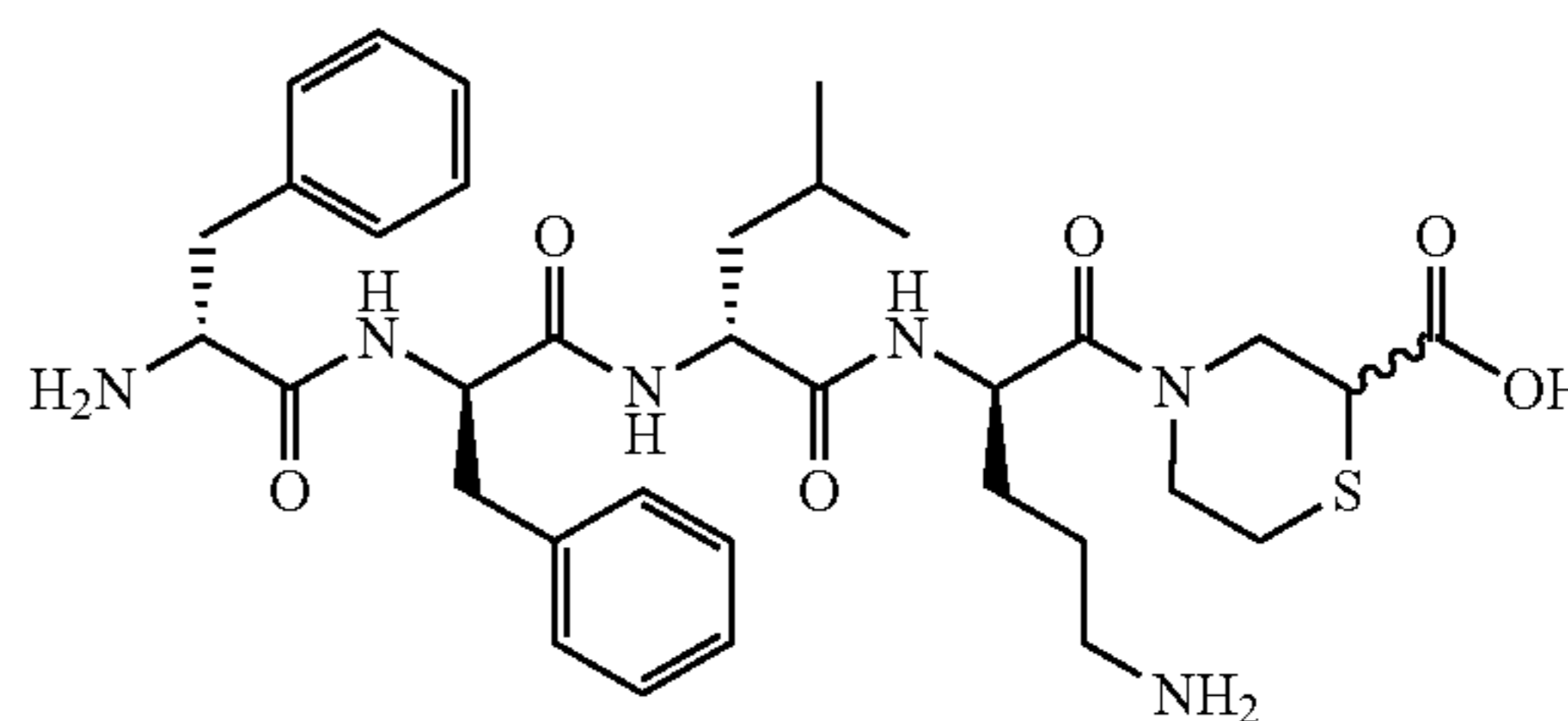
D-Phe-D-Phe-D-Leu-D-Orn-[R/S-2-carboxythiomorpholine]-OH
