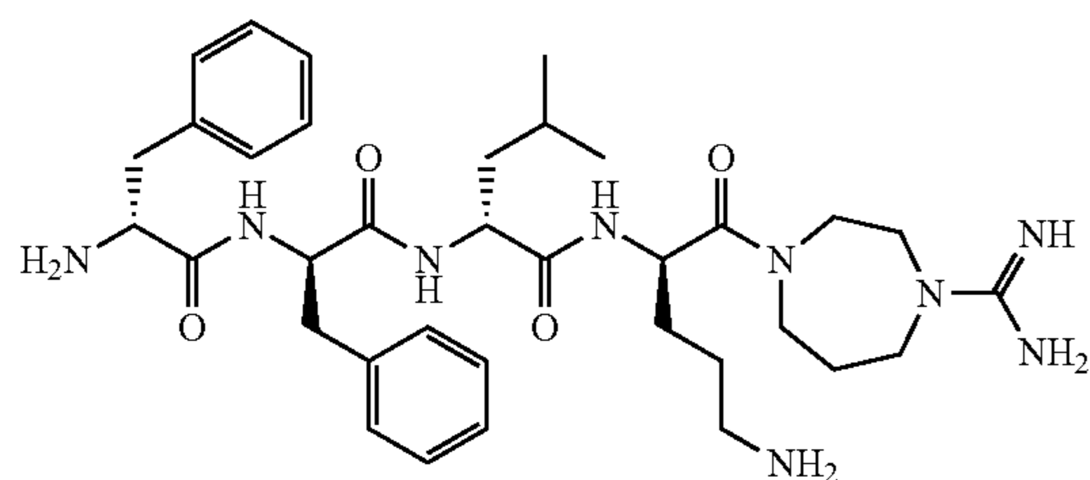
D-Phe-D-Phe-D-Leu-D-Orn-[4-amidinohomopiperazine amide]
