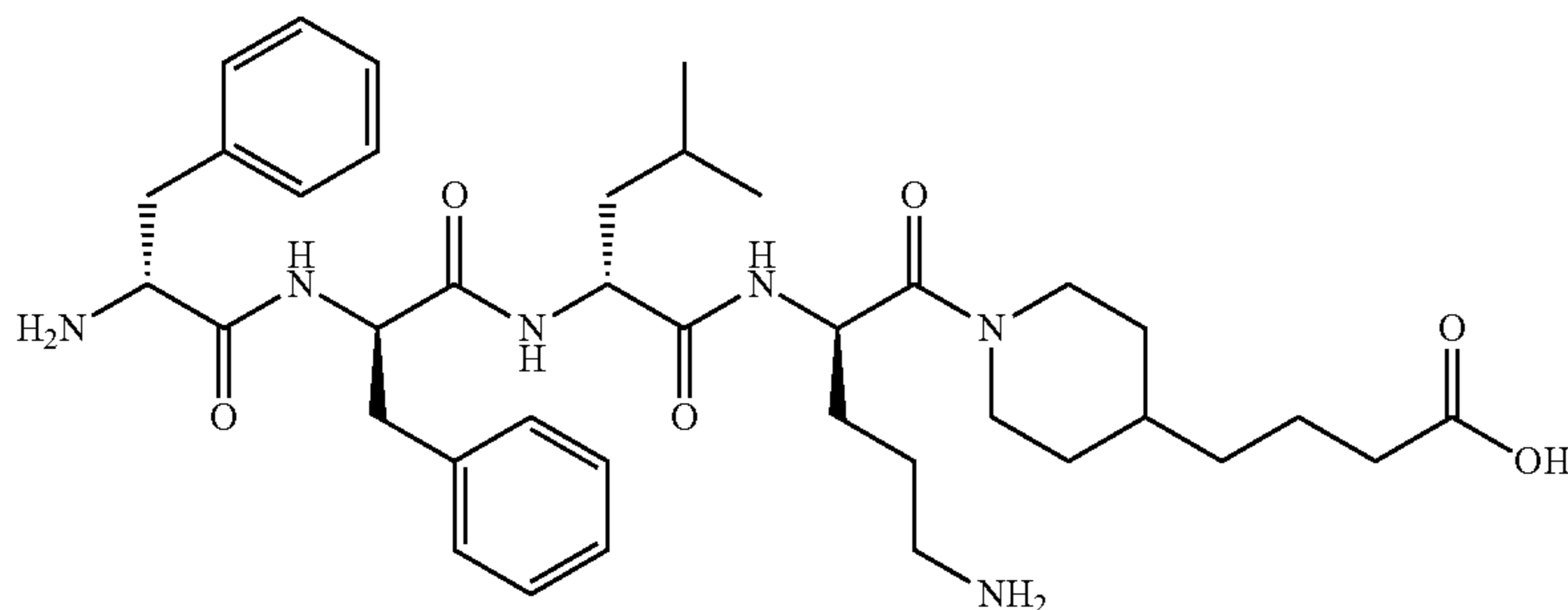
D-Phe-D-Phe-D-Leu-D-Orn-[4-(4-piperidinyl)-butanoic acid]-OH
