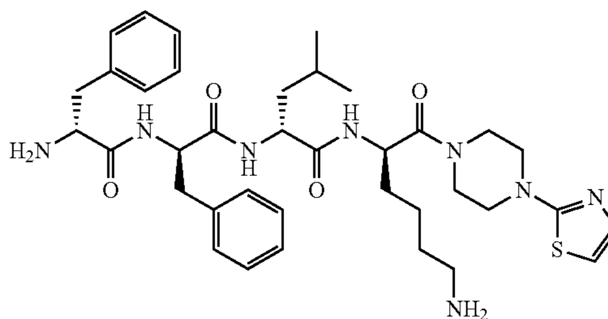
D-Phe-D-Phe-D-Leu-D-Lys-[2-(piperazin-1-yl)thiazole amide]
