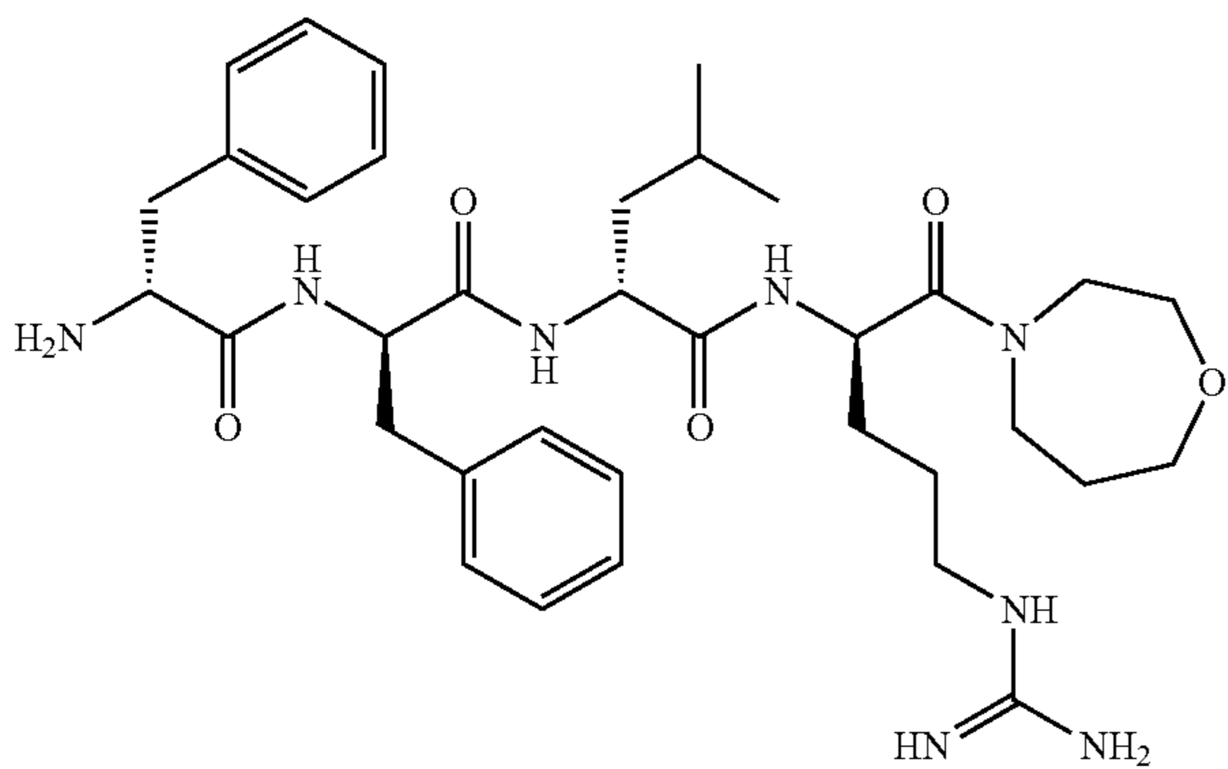
D-Phe-D-Phe-D-Leu-D-Arg-[homomorpholine amide]
