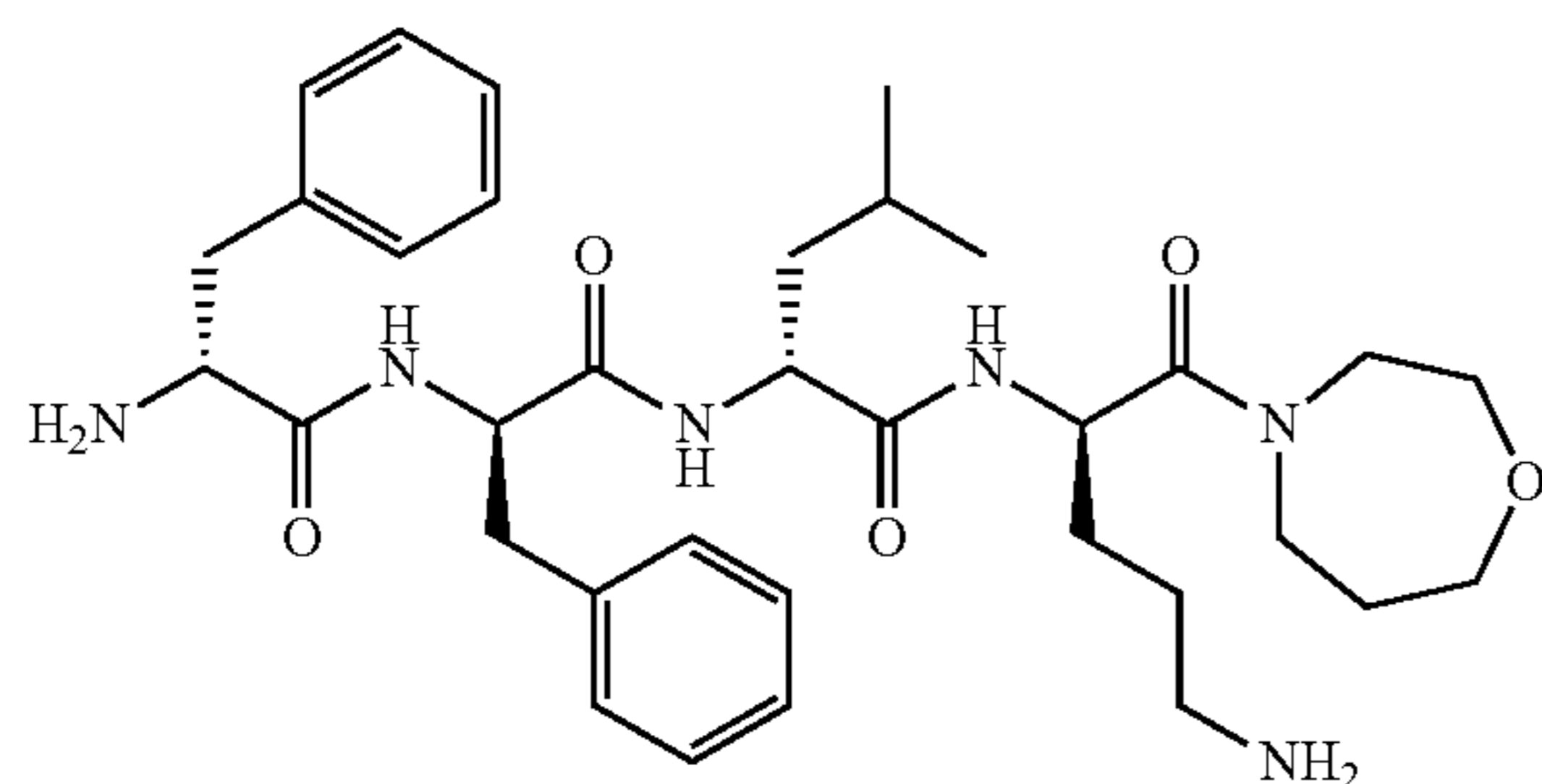
D-Phe-D-Phe-D-Leu-D-Orn-N(homomorpholine)
