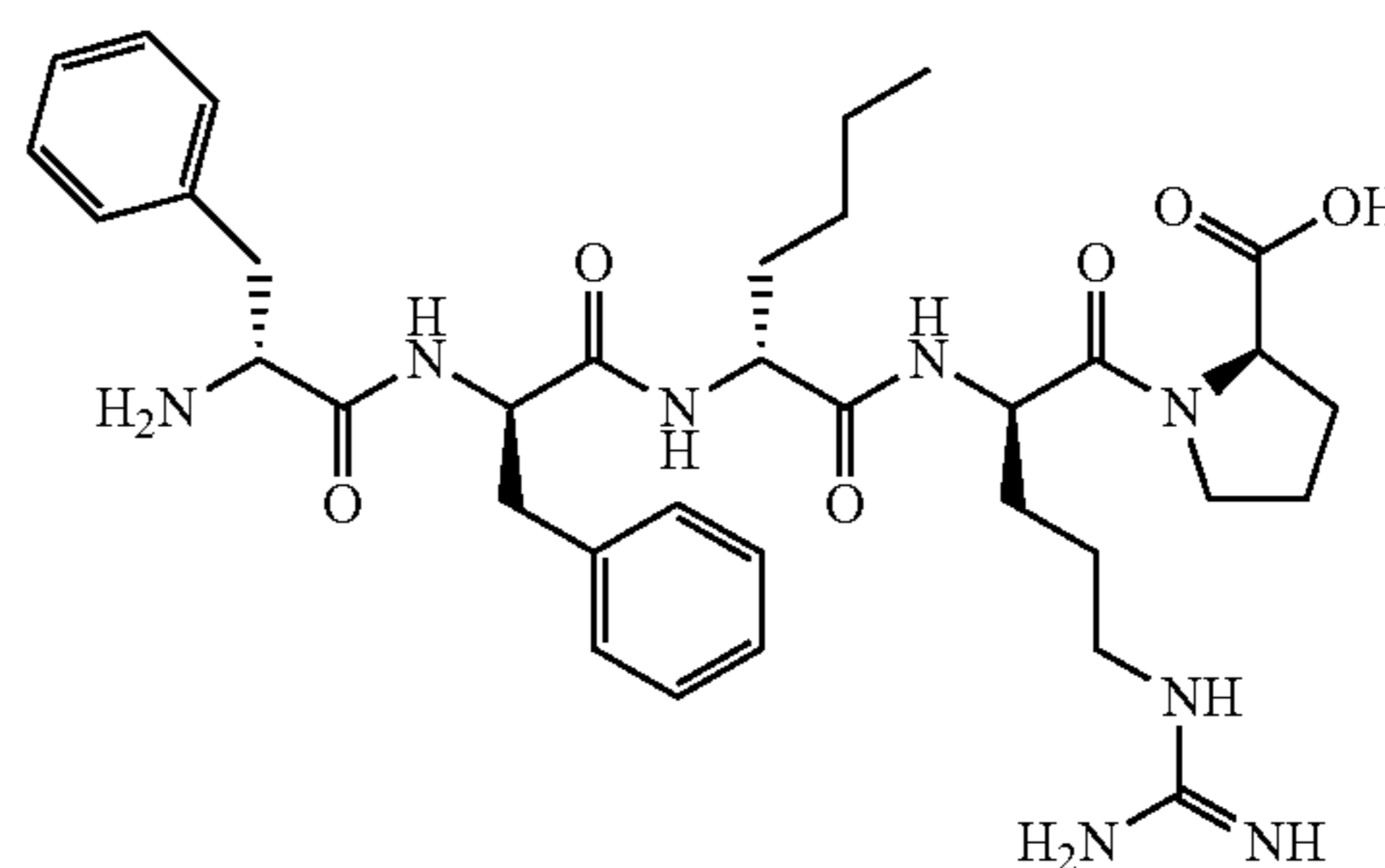
D-Phe-D-Phe-D-Nle-D-Arg-D-Pro-OH
