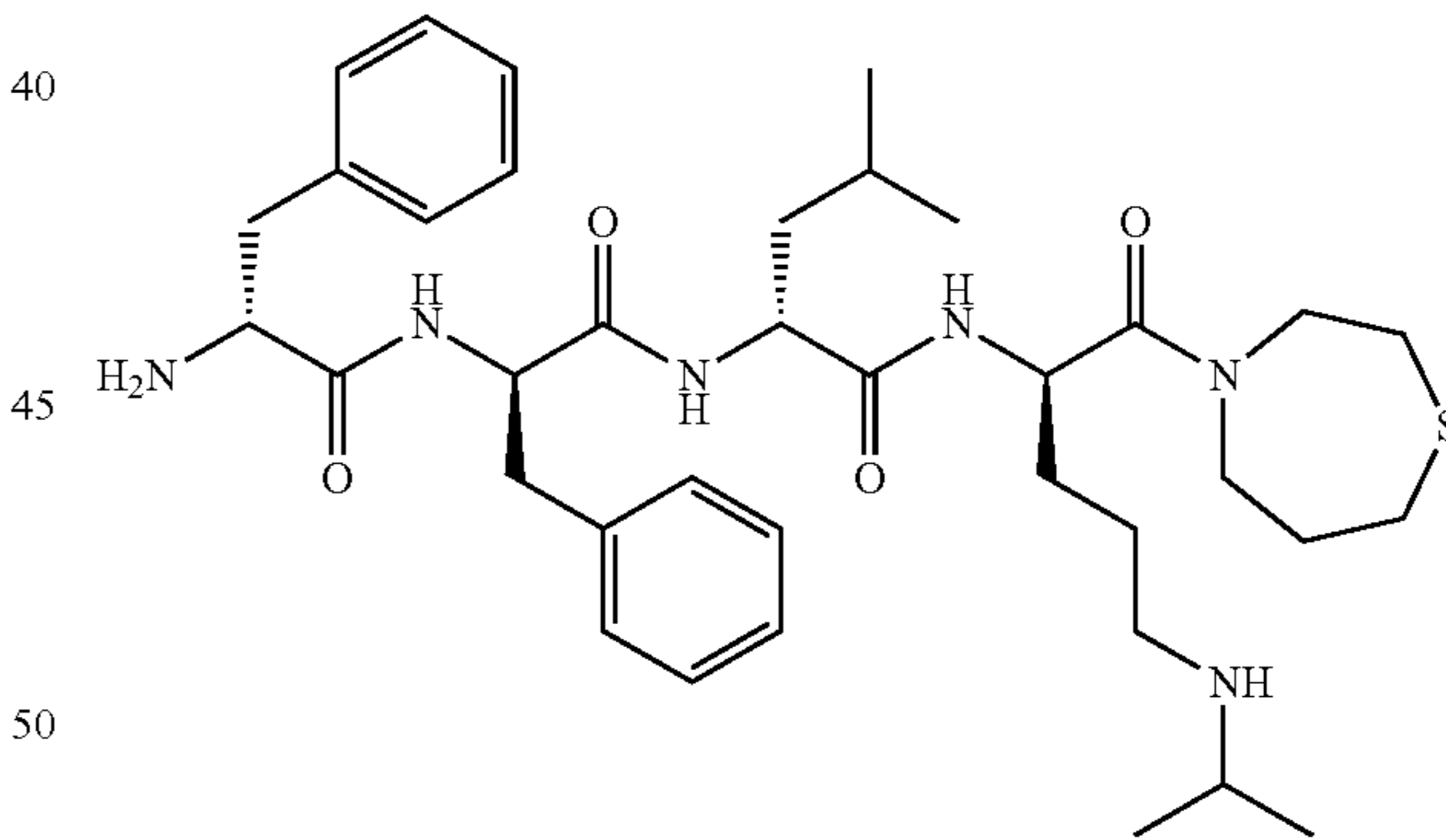
D-Phe-D-Phe-D-Leu-D-Orn(iPr)-[homothiomorpholine amide]
