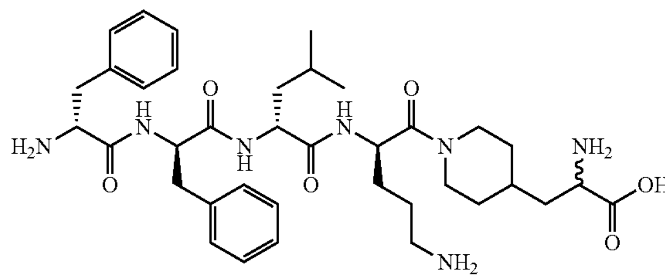
D-Phe-D-Phe-D-Leu-D-Orn-[omega(D/L-2-amino-3-(4-N-piperidinyl)propionic acid)]-OH
