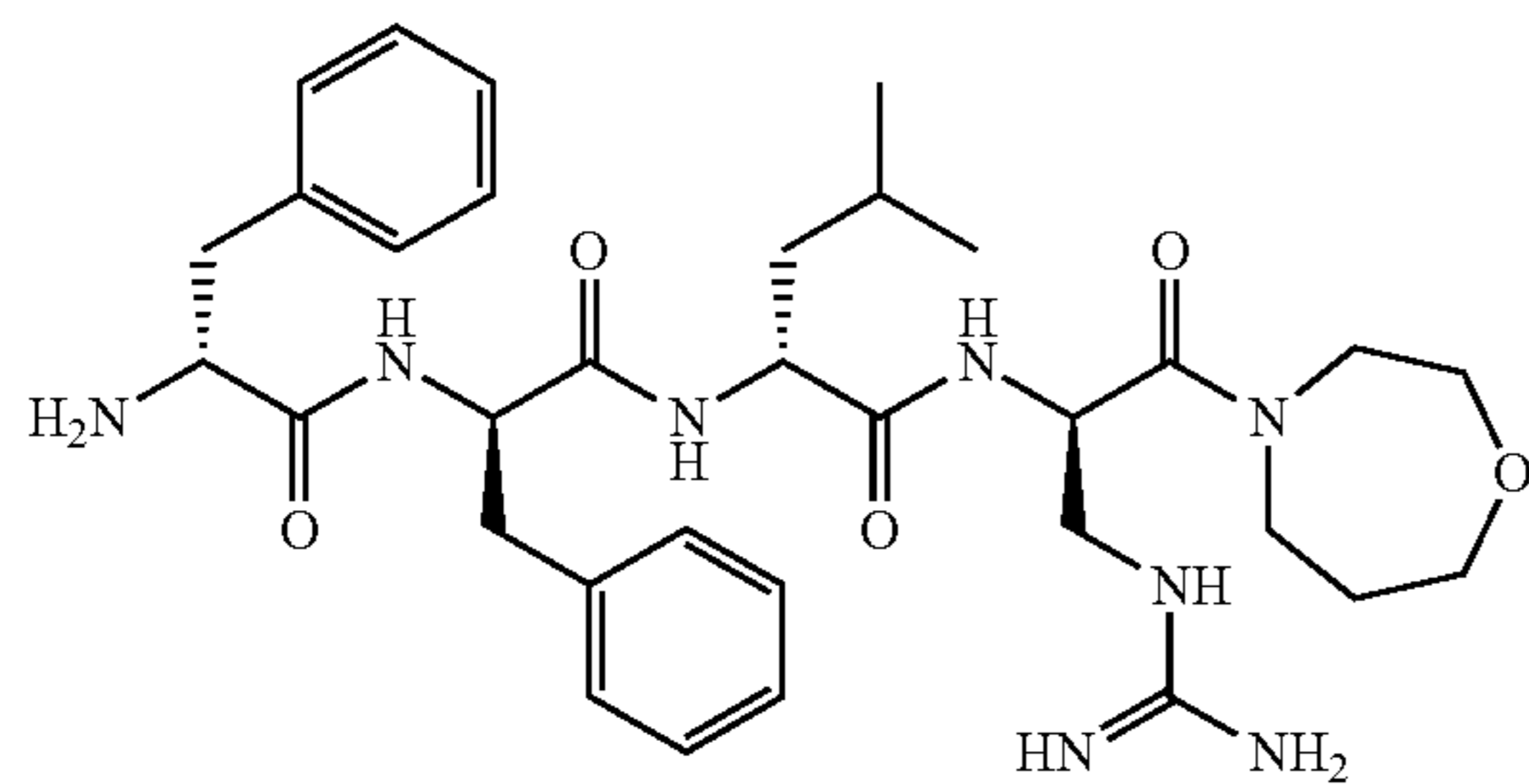
D-Phe-D-Phe-D-Leu-D-Dap(amidino)-[homomorpholine amide]
