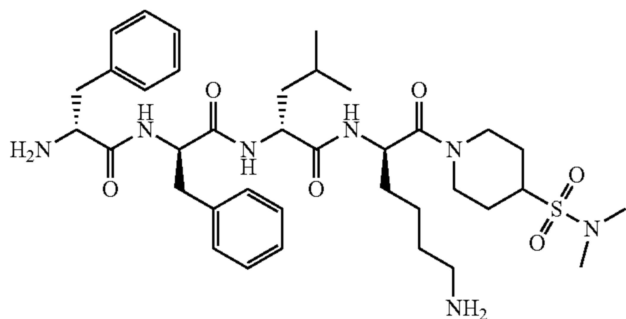
D-Phe-D-Phe-D-Leu-D-Lys-[N,N-dimethylpiperazine-1-sulfonamide amide]
