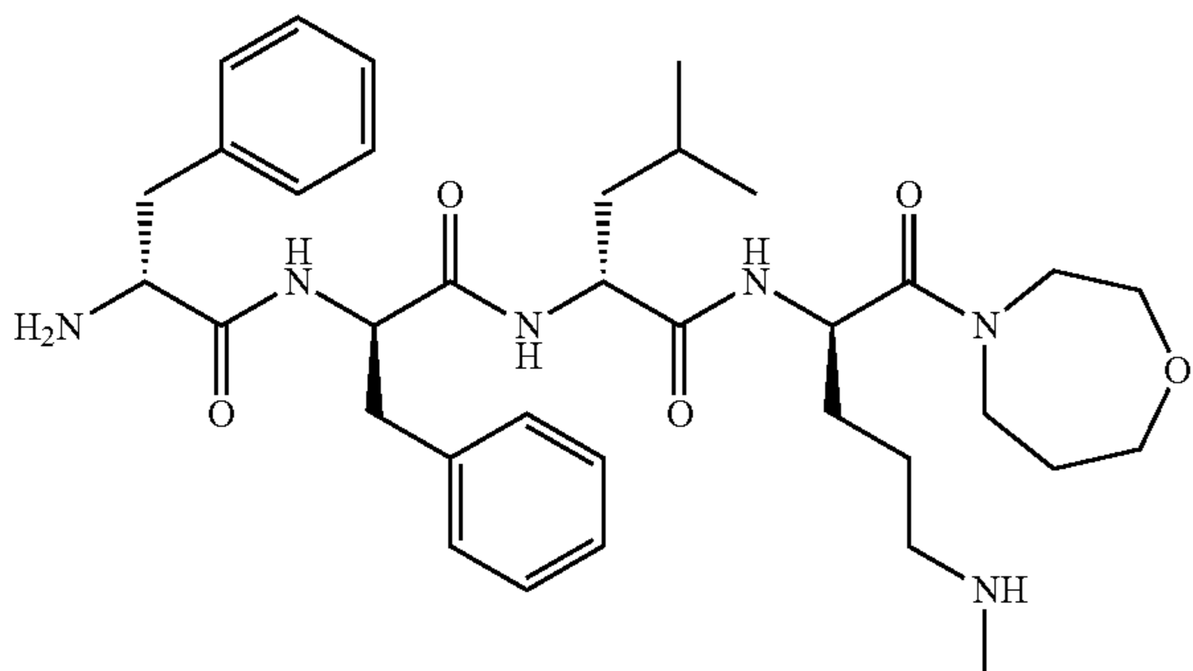
D-Phe-D-Phe-D-Leu-D-Orn(Me)-[homomorpholine amide]
