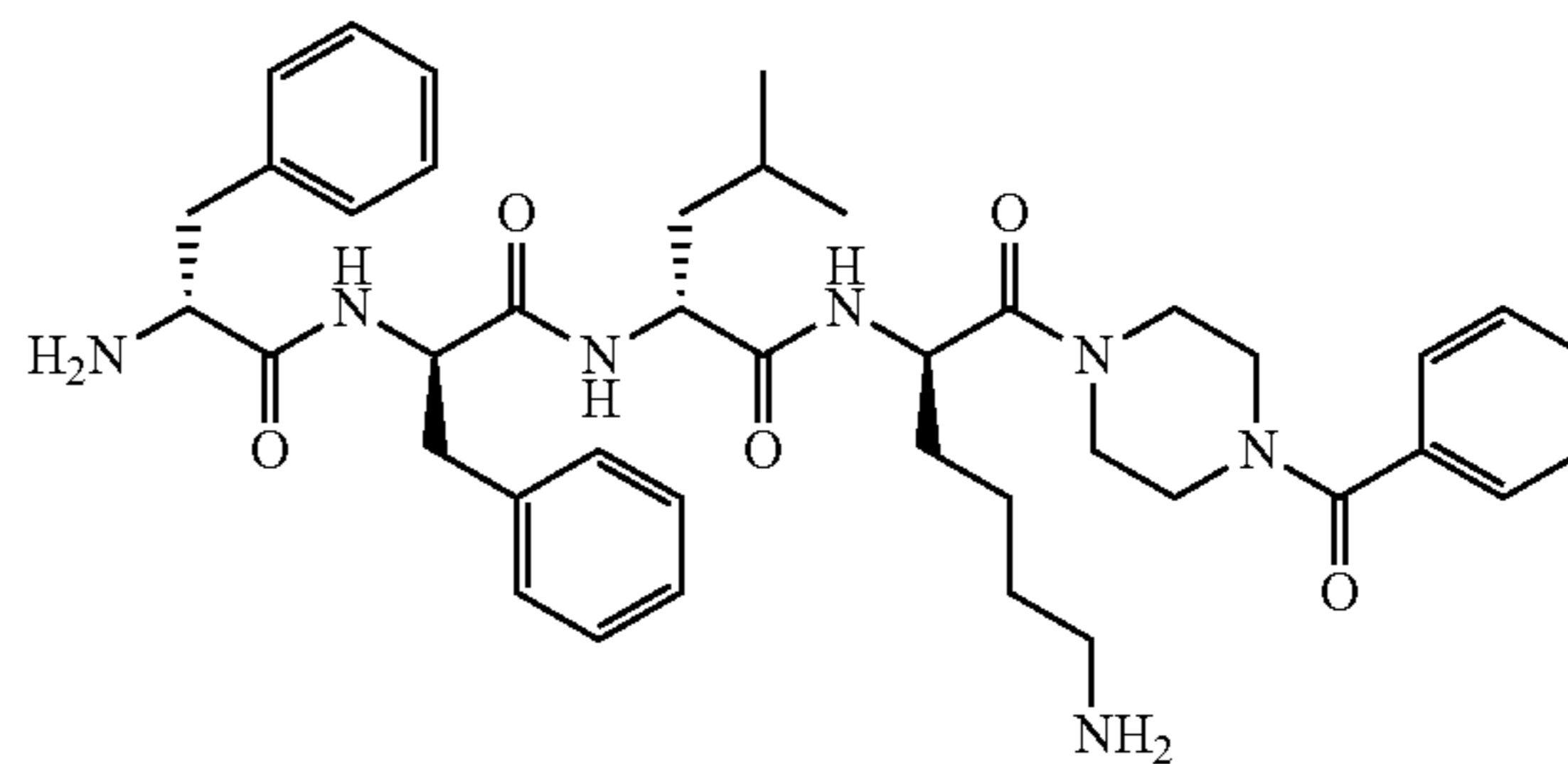
D-Phe-D-Phe-D-Leu-D-Lys-[phenyl(piperazin-1-yl)methanone amide]
