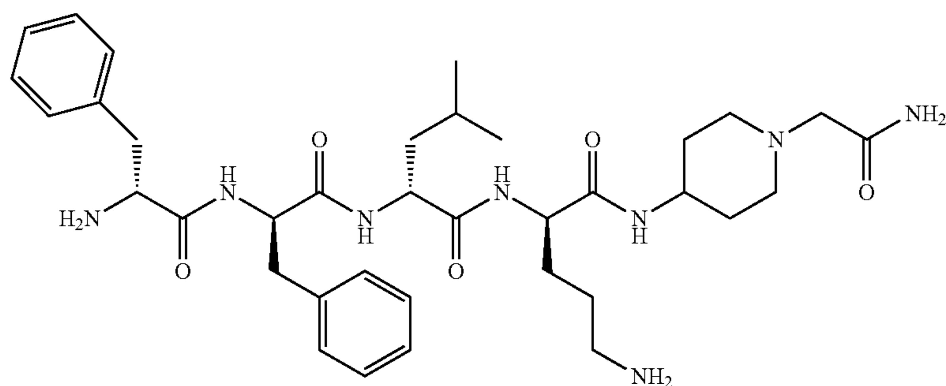
D-Phe-D-Phe-D-Leu-D-Orn-[4-amino-1-carboxymethyl-piperidine]-NH 2
