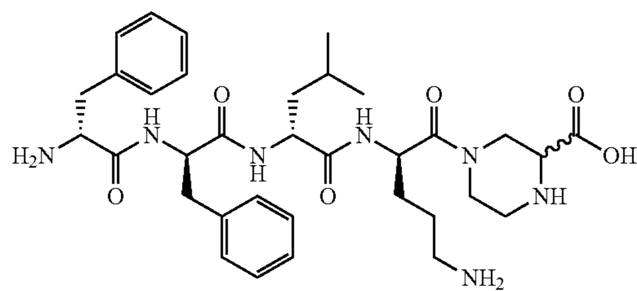
D-Phe-D-Phe-D-Leu-D-Orn-[omega(D/L-4-piperazine-2-carboxylic acid)]-OH
