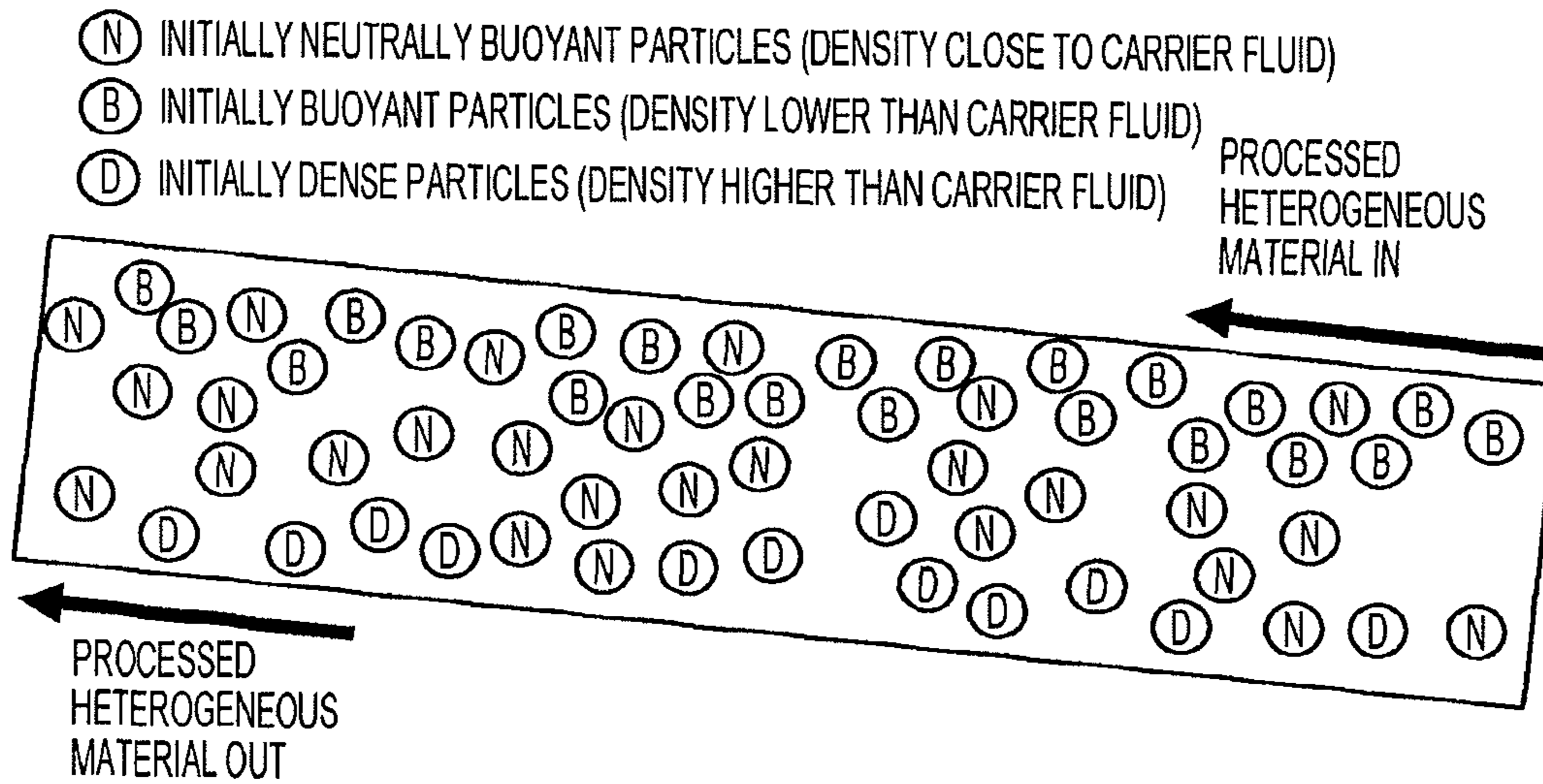
TRANSPARENT CONDUIT DETAIL WITH CARRIER FLUID AND INDIVIDUAL PARTICULATE COMPONENTS WITH DIFFERENT DENSITY RANGES
