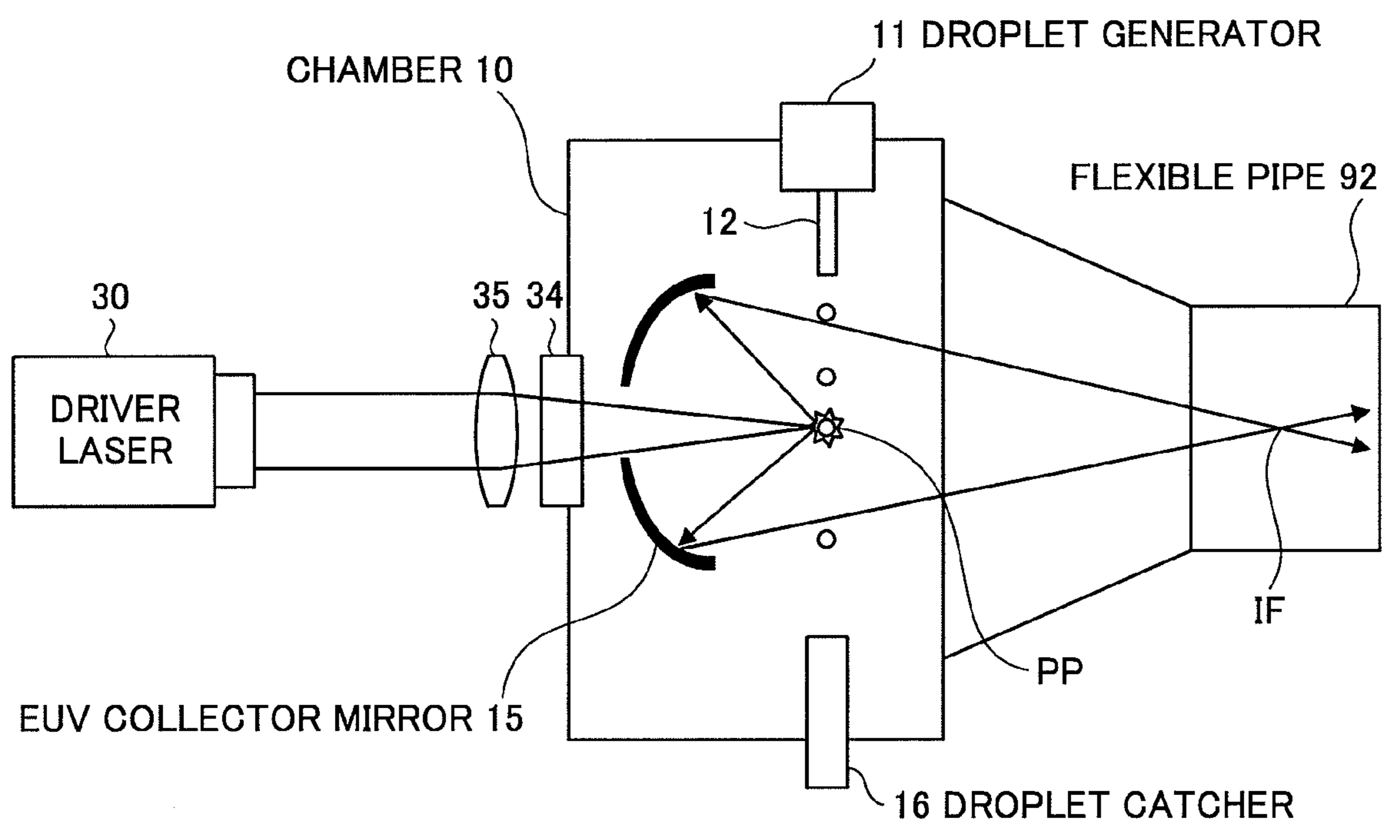
1 EUV LIGHT SOURCE APPARATUS
