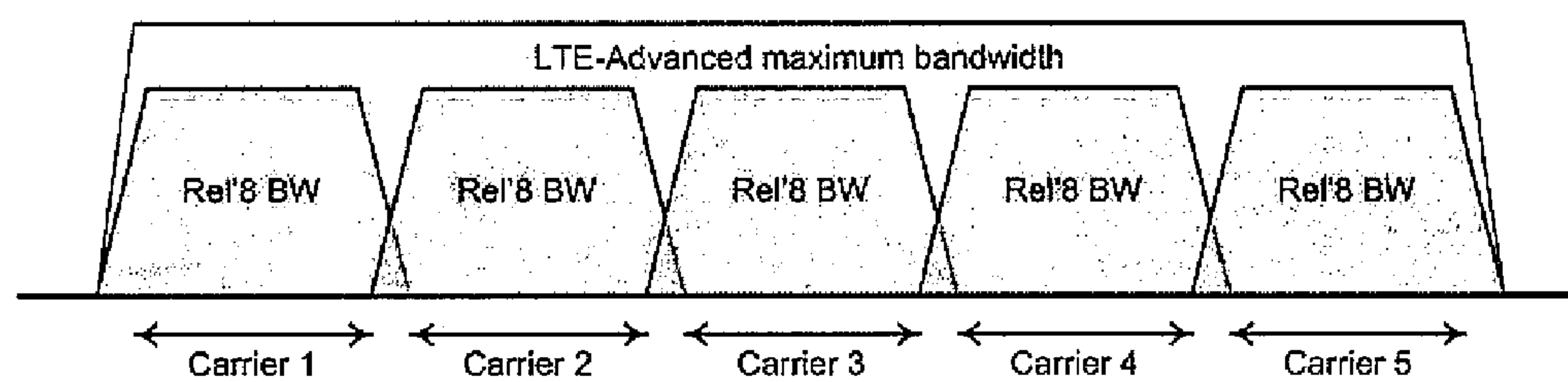
Figure 2: Prior Art
