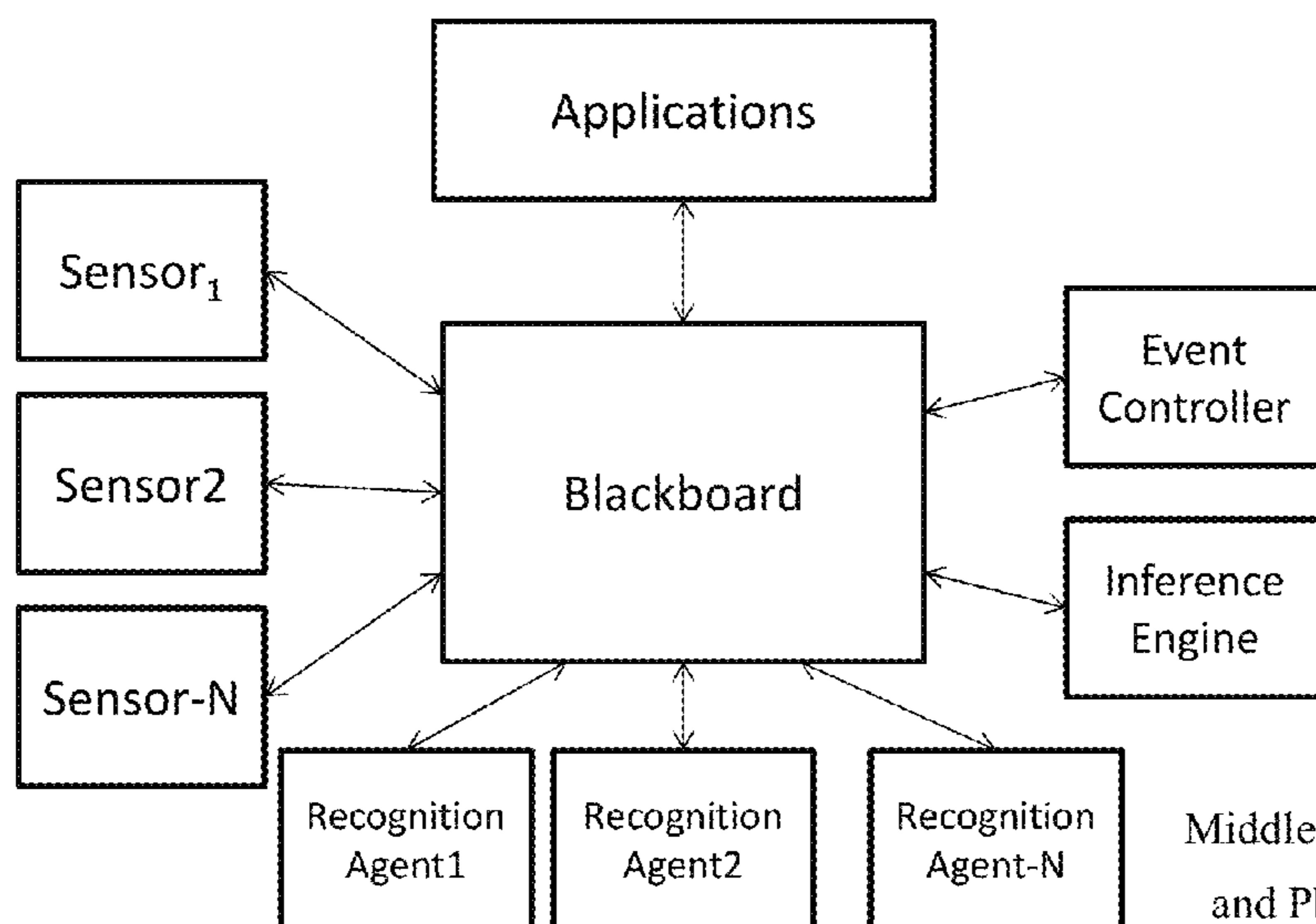
FIG. 16 Middleware Architecture for Media and Physical Object Recognition
