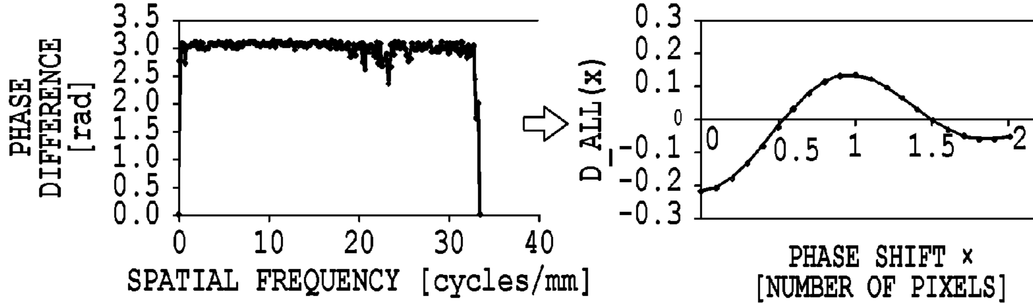
FIG.23A ALL FREQUENCY EXCLUSION (FIG. 12)
