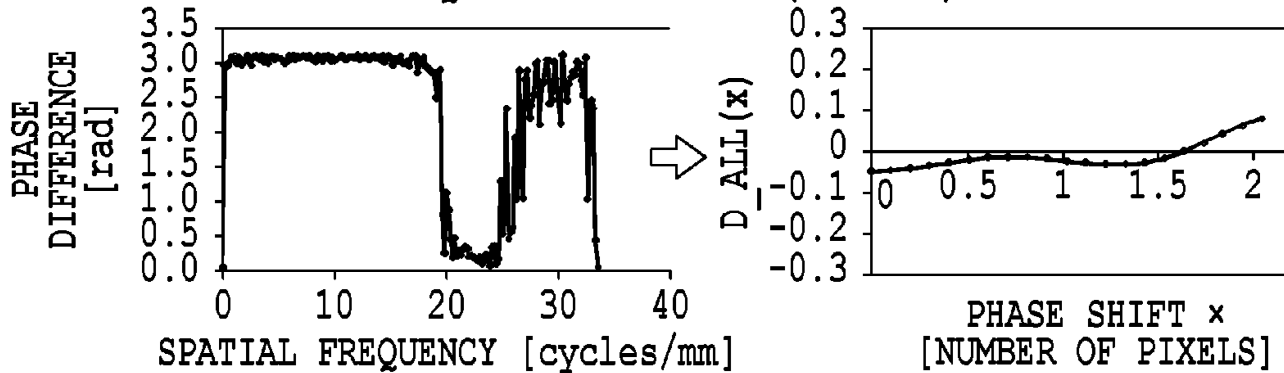
FIG.23D LOW-FREQUENCY EXCLUSION • MIDDLE-FREQUENCY IN-PHASE • HIGH-FREQUENCY EXCLUSION (FIG. 22)
