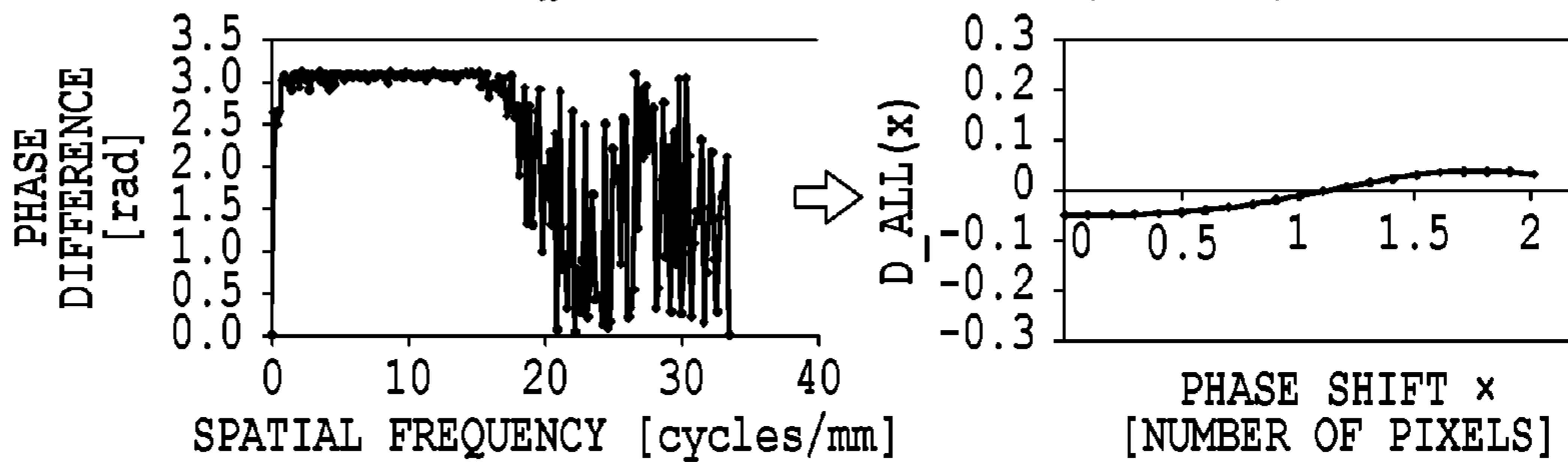
FIG.23D LOW-FREQUENCY EXCLUSION • MIDDLE-FREQUENCY IN-PHASE • HIGH-FREQUENCY EXCLUSION (FIG. 22)
