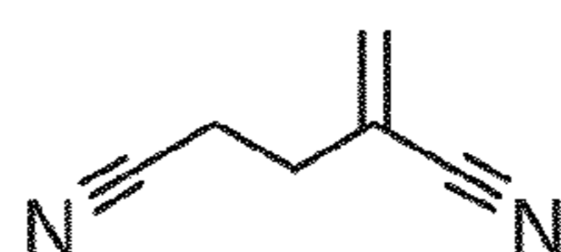
19 D 2-methyleneglutaronitrile
