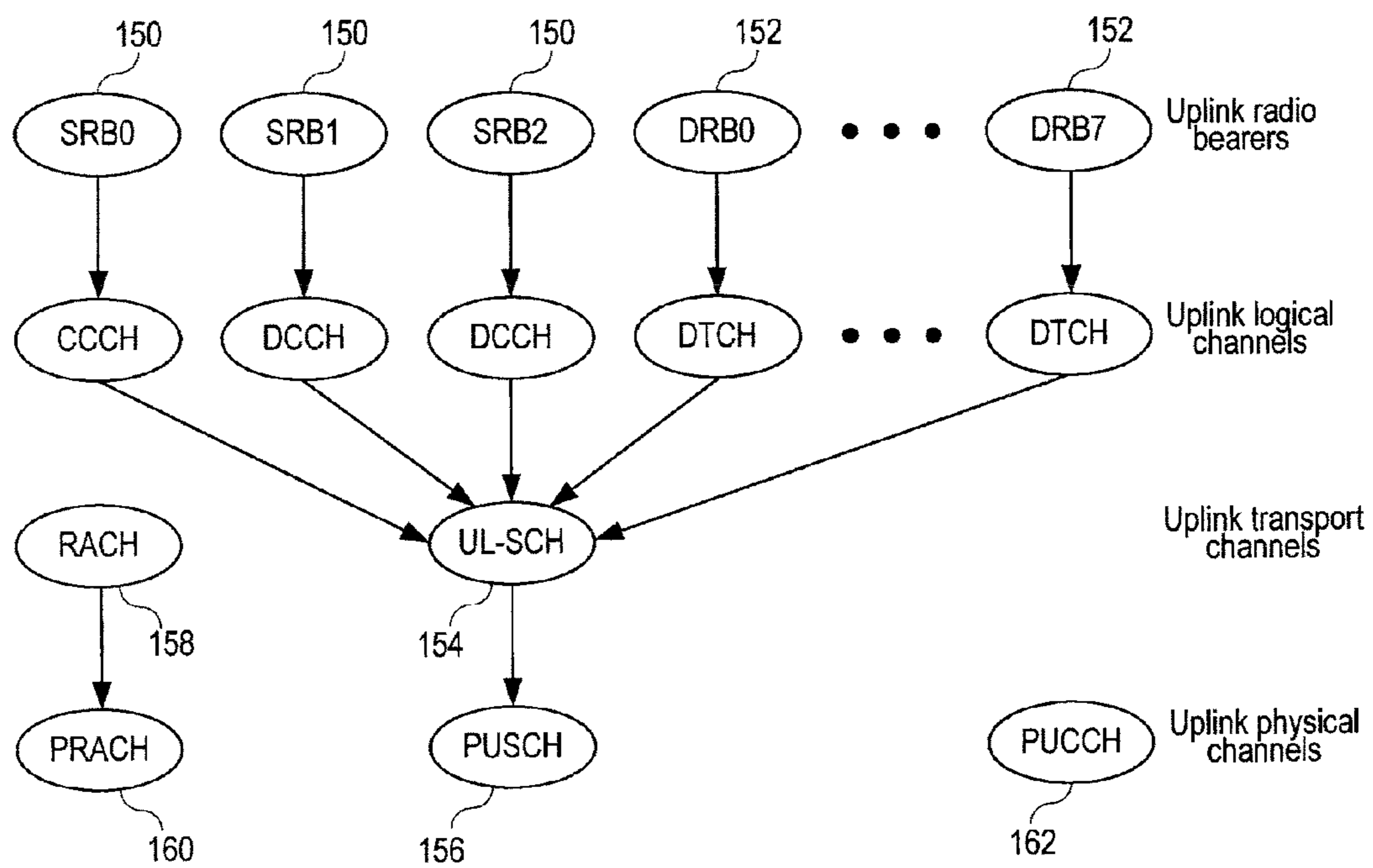
FIG. 4 PRIOR ART
