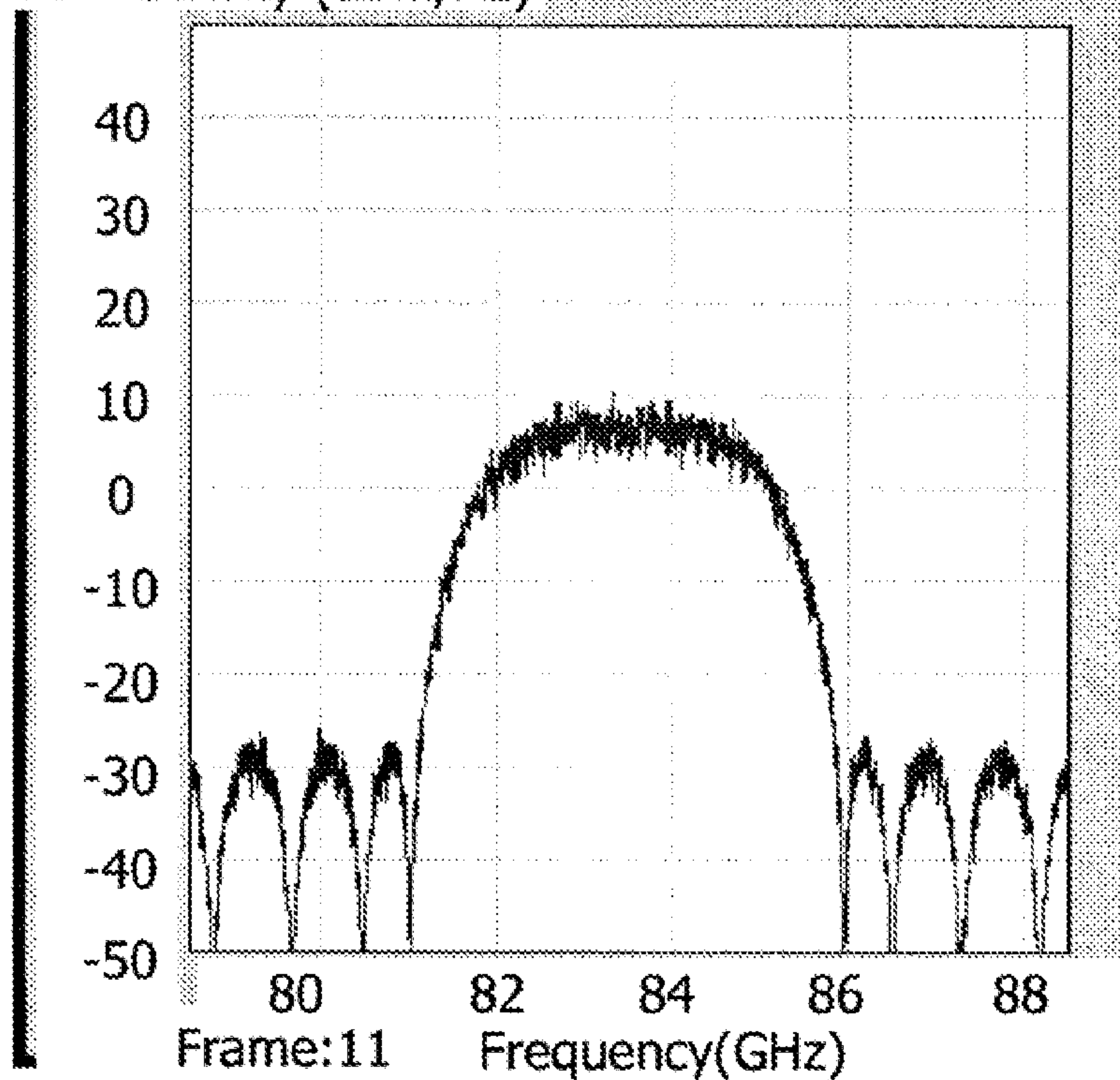
FIG.7B SPECTRUM WHEN REFERENCE PULSE IS USED
