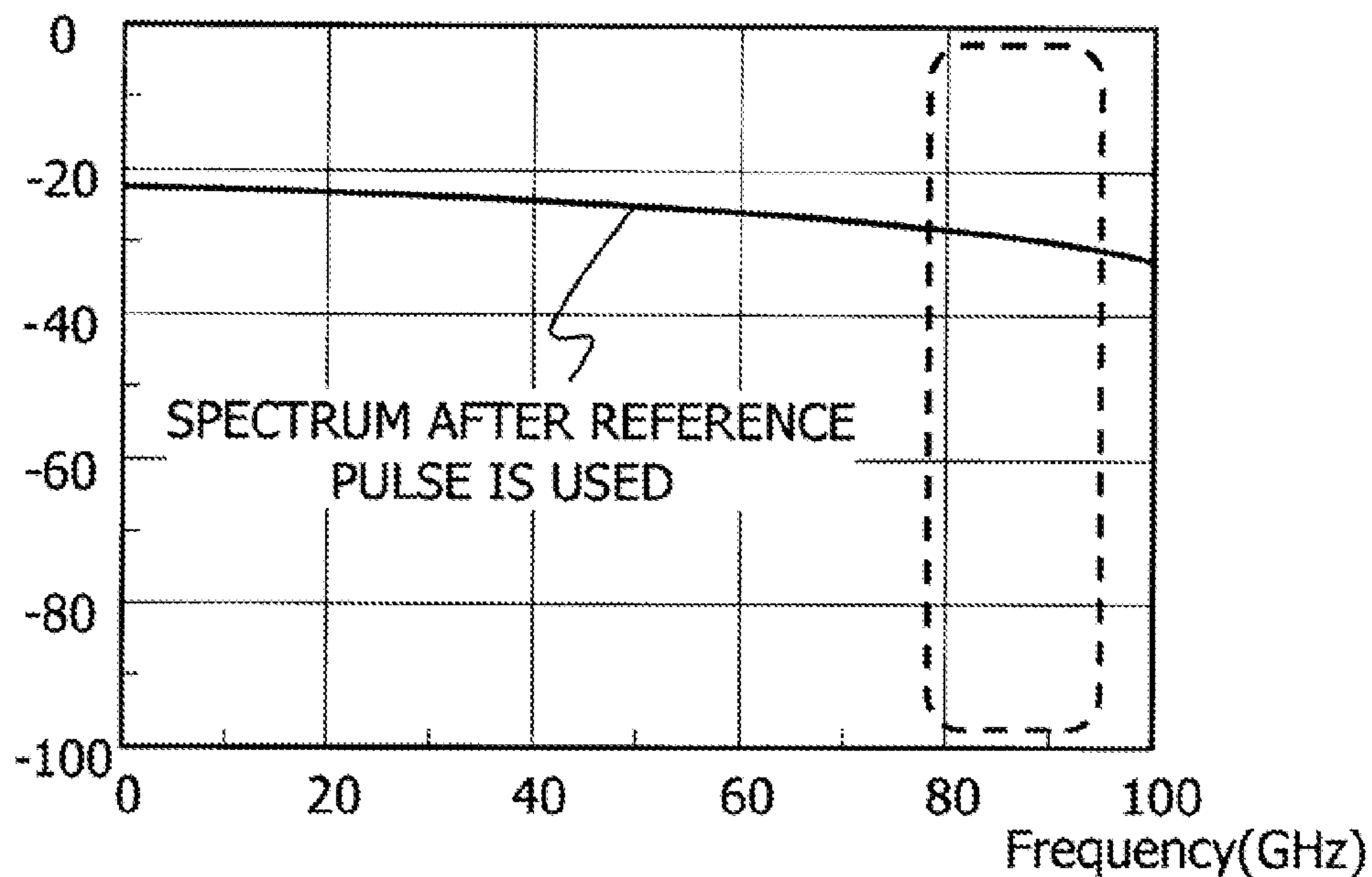
FIG.7B SPECTRUM WHEN REFERENCE PULSE IS USED
