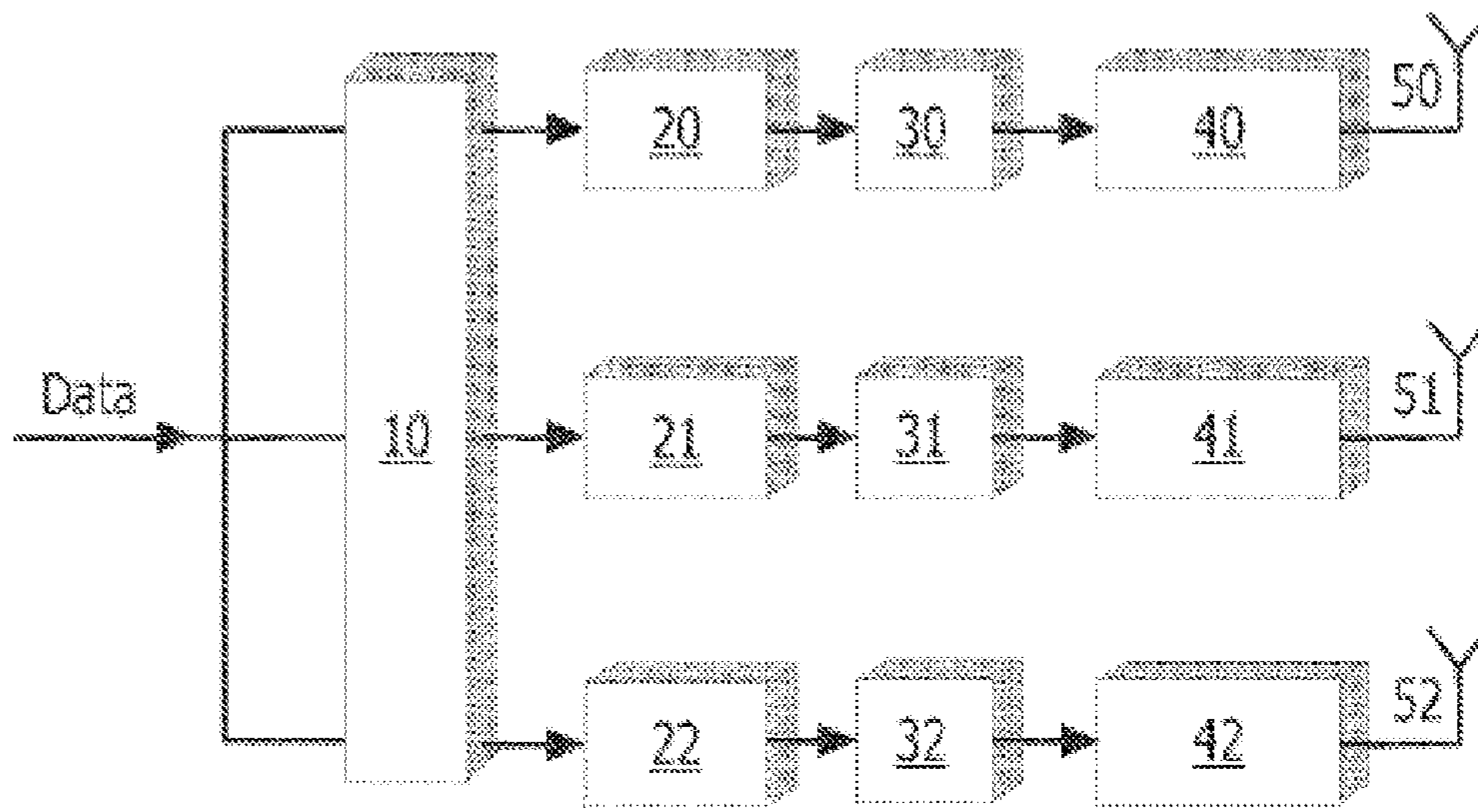
FIG. 1 (PRIOR ART)
