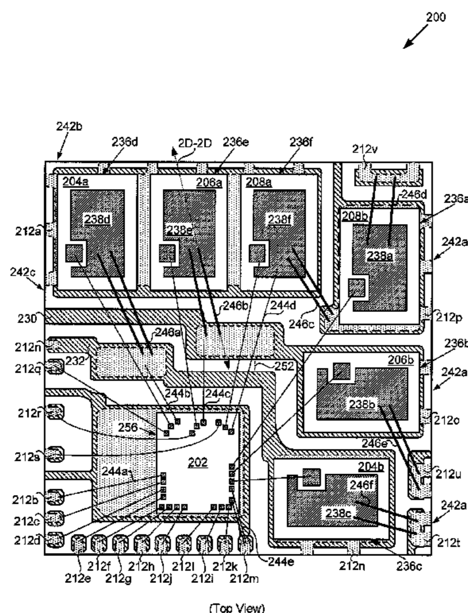
(Top View)
