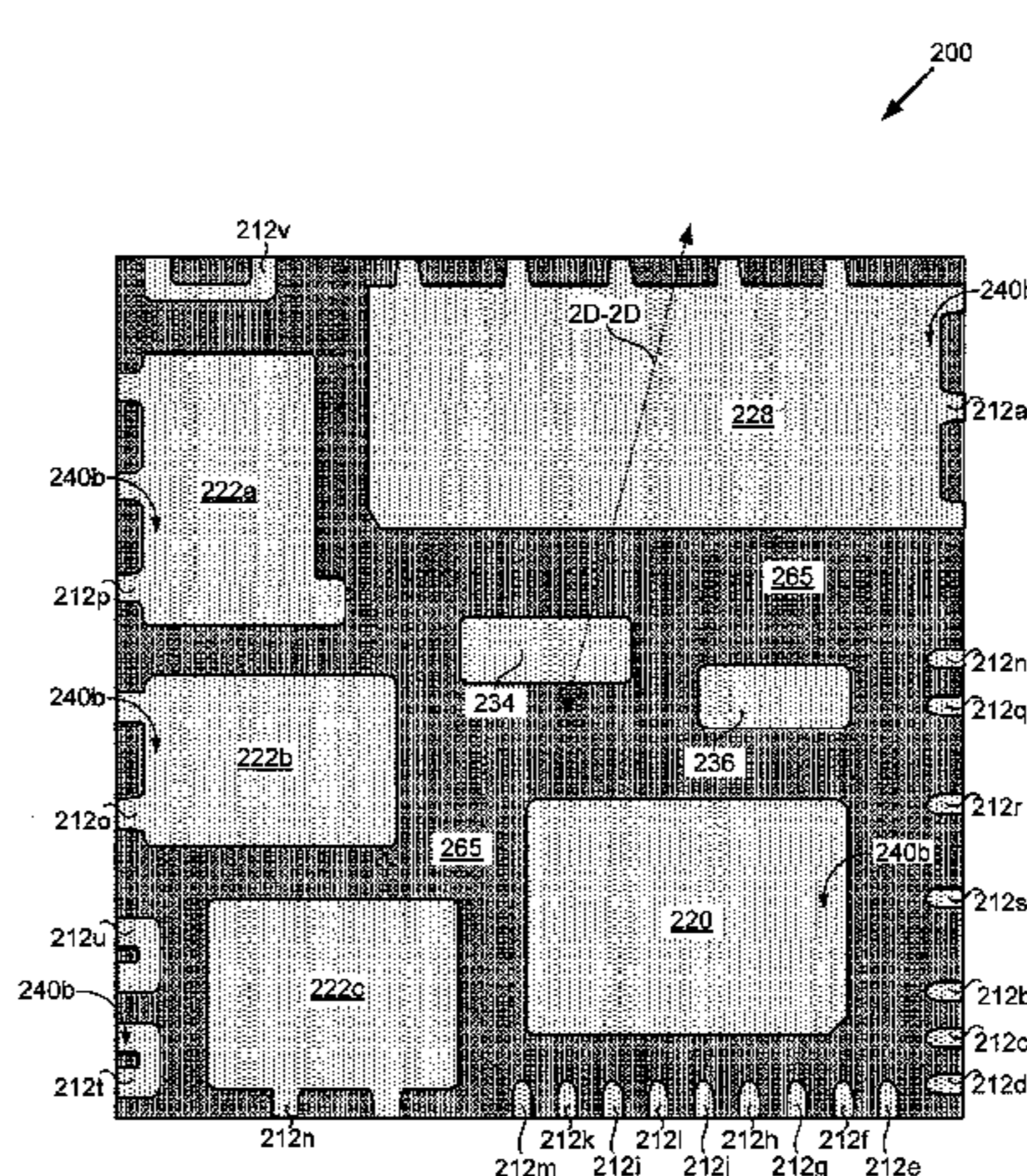
(Bottom View)
