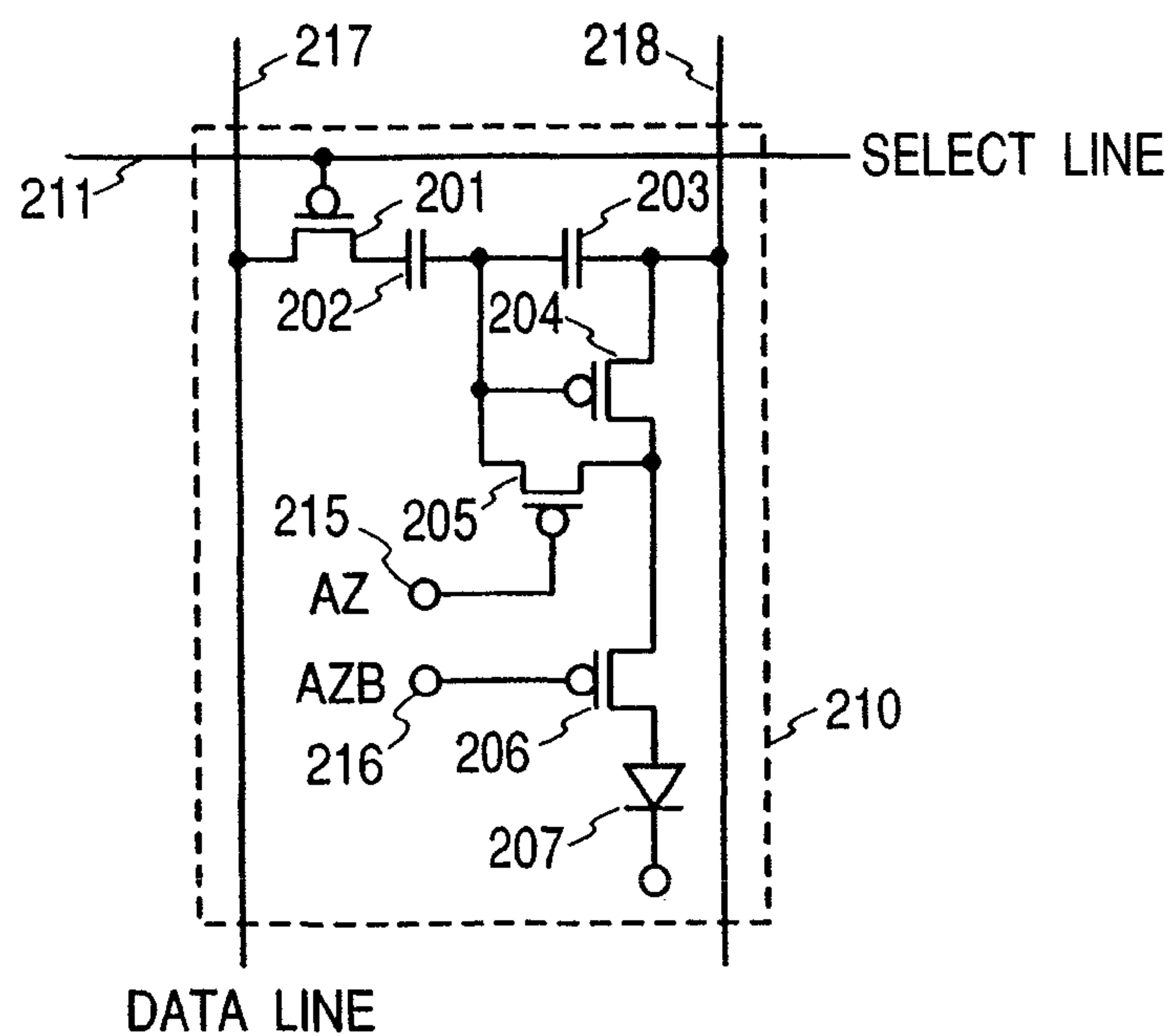
FIG. 23 PRIOR ART
