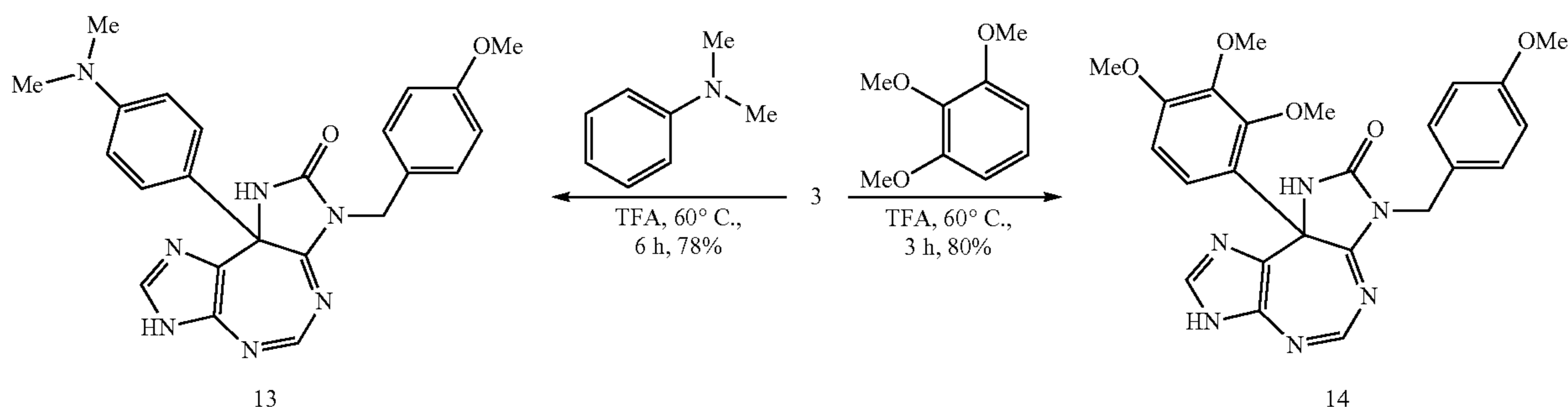
Scheme 5
