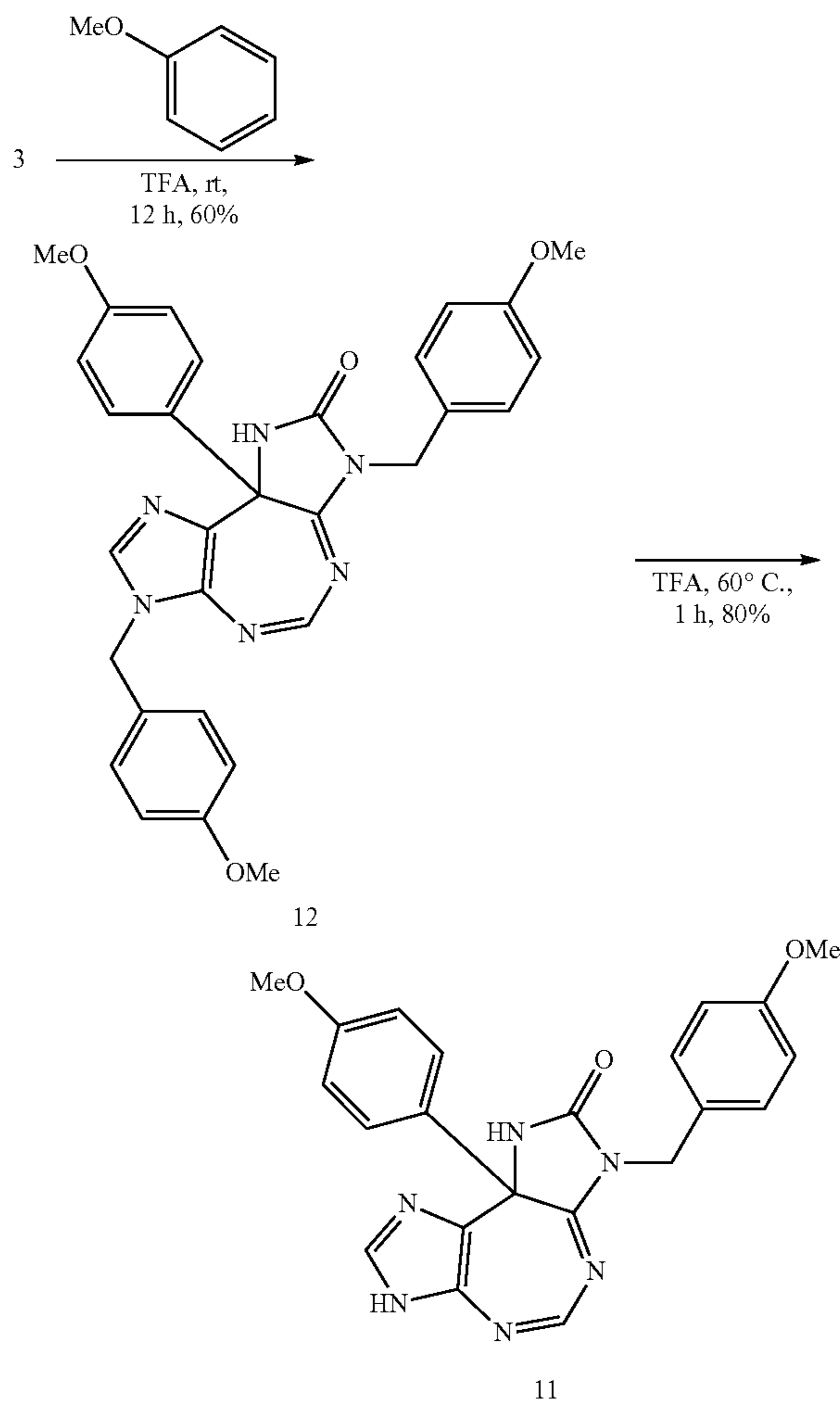
Scheme 4
