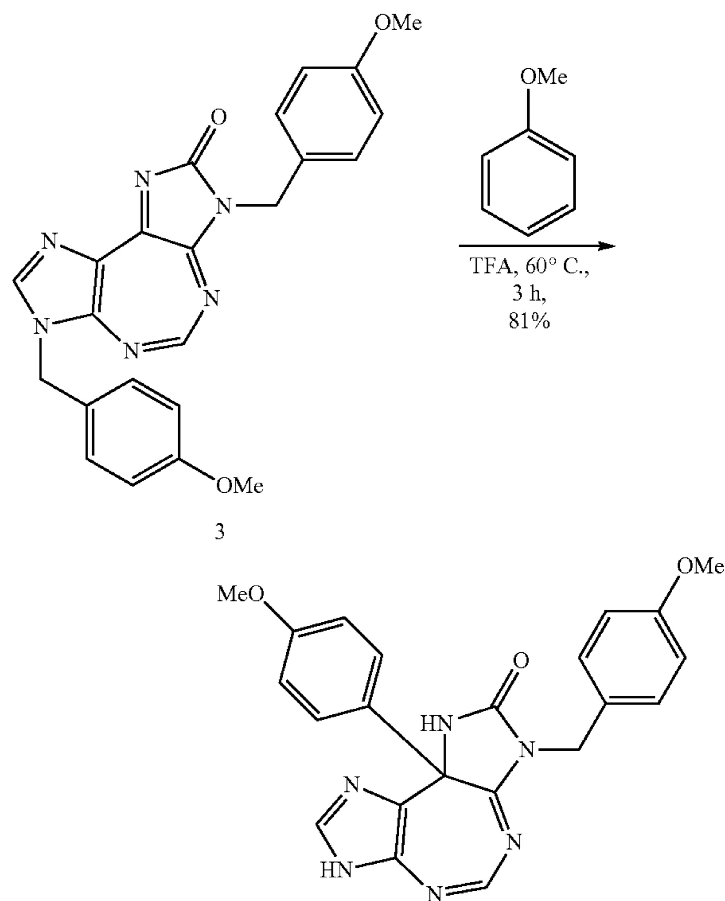
Scheme 3
