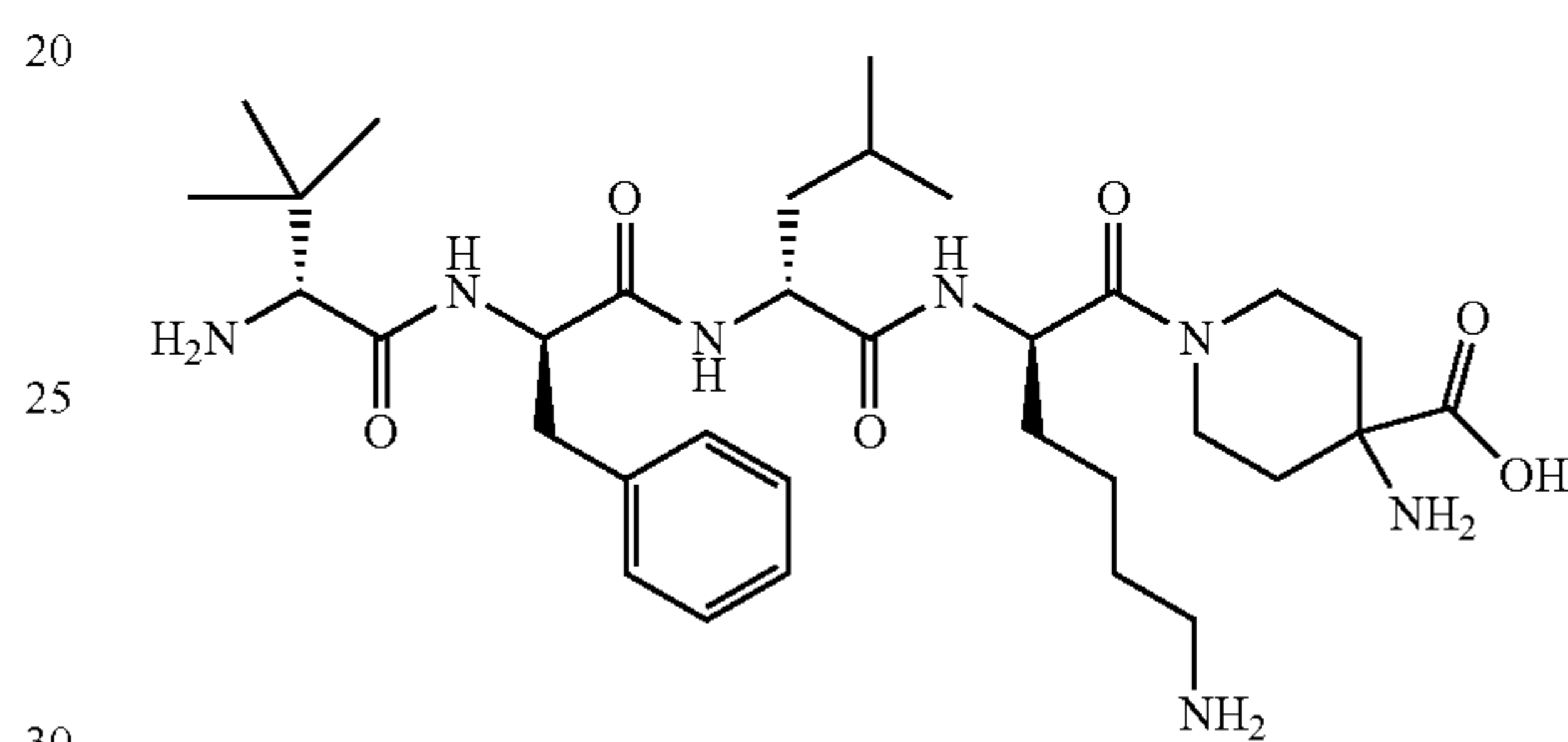
Compound (105): D-tert-Leu-D-Phe-D-Leu-D-Lys- [ \omega (4-aminopiperidine-4-carboxylic acid)]-OH
