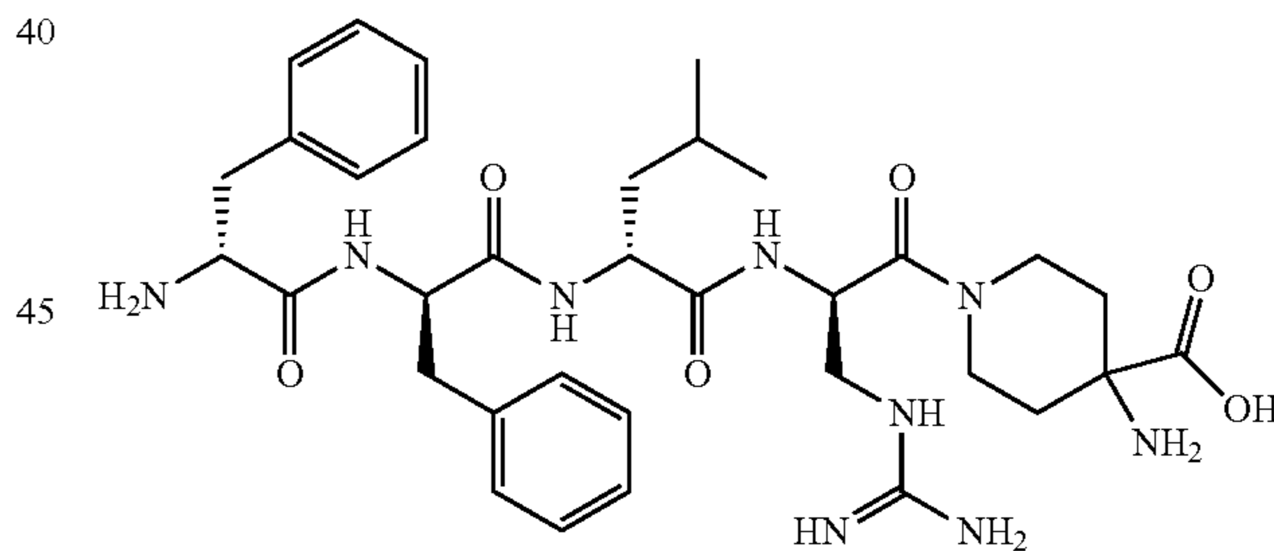
Compound (10): D-Phe-D-Phe-D-Leu-(β-amidino)D-Dap-[ω(4-aminopiperidine-4-carboxylic acid)]-OH
