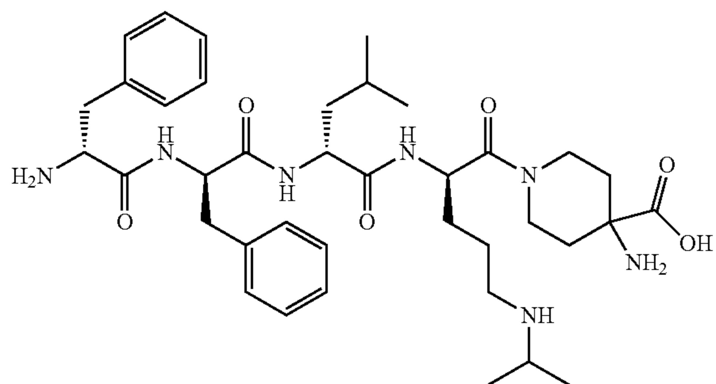
Compound (59) D-Phe-D-Phe-D-Leu-( \delta -iPr)D-Orn- [4-amidinohomopiperazine amide]
