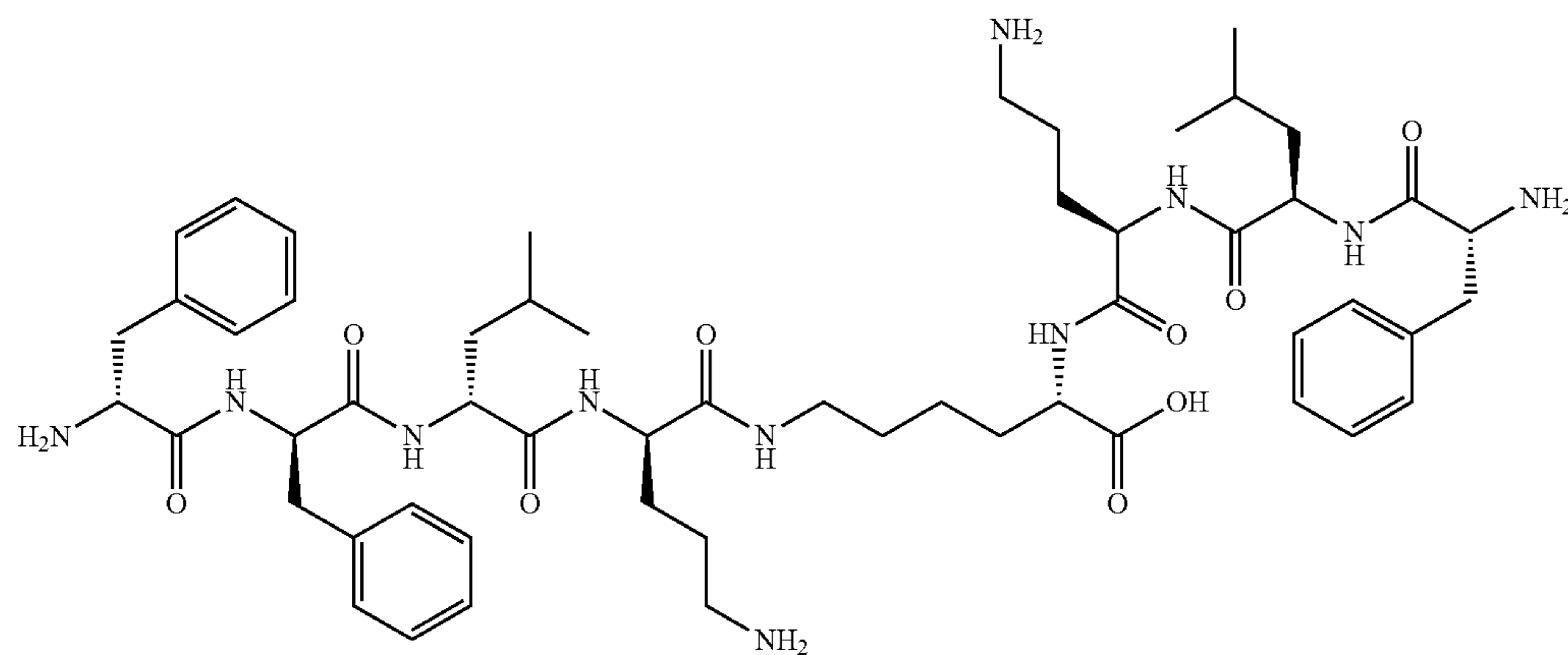
Compound (79)
