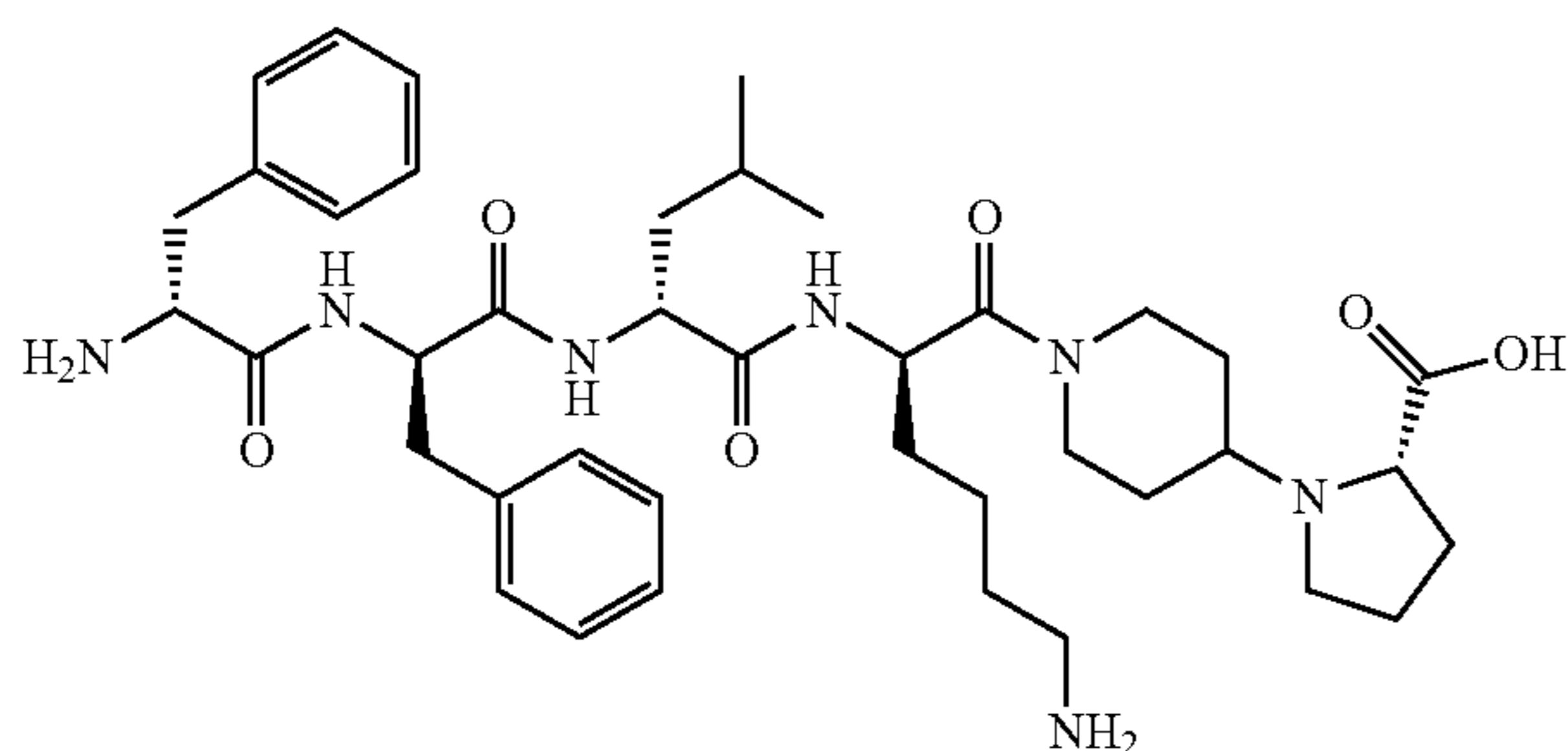
Compound (5): D-Phe-D-Phe-D-Leu-D-Har-[N-(4-piperidinyl)-L-proline]-OH
