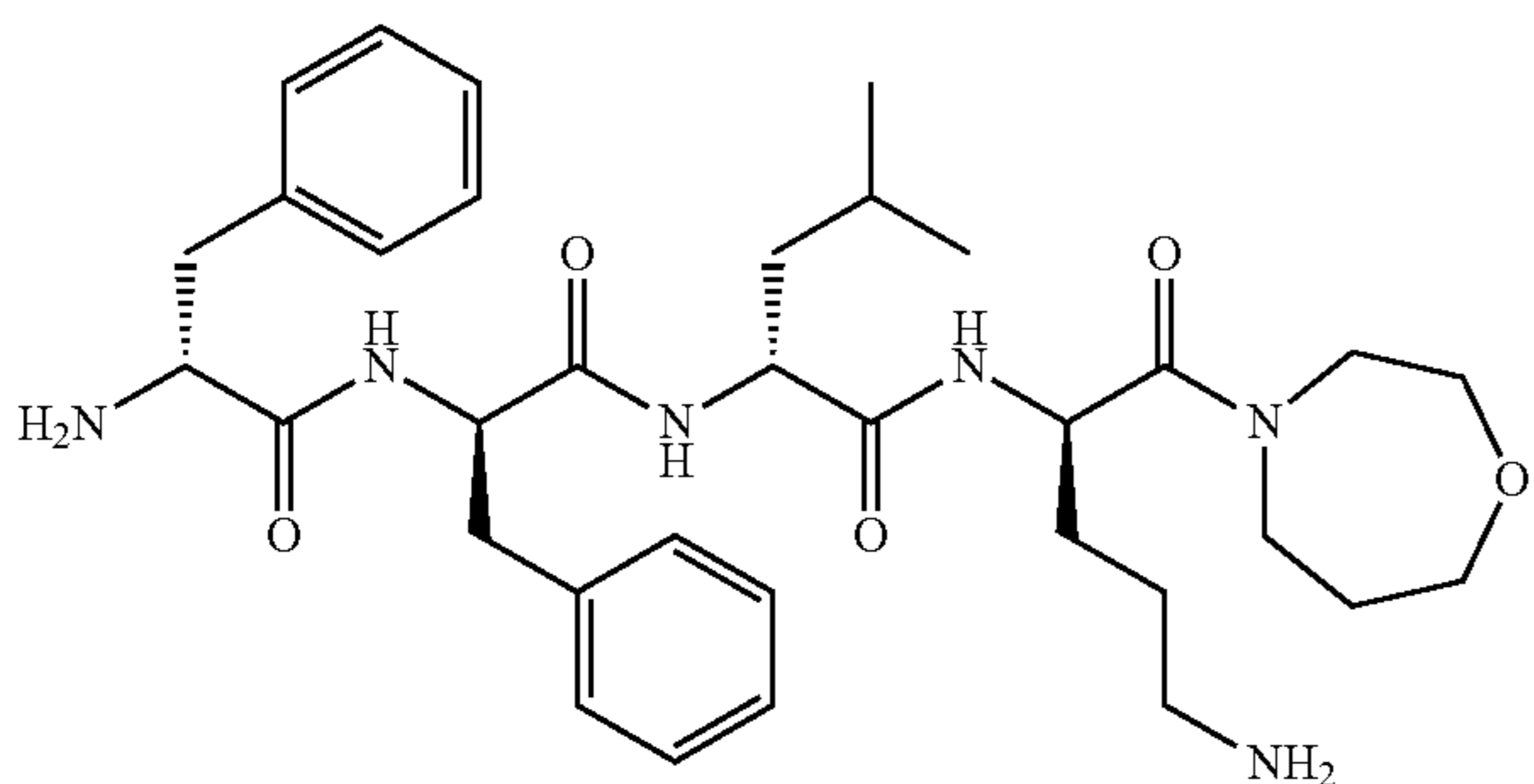
Compound (93) D-Phe-D-Phe-D-Leu-D-Orn-N(homothiomorpholine)
