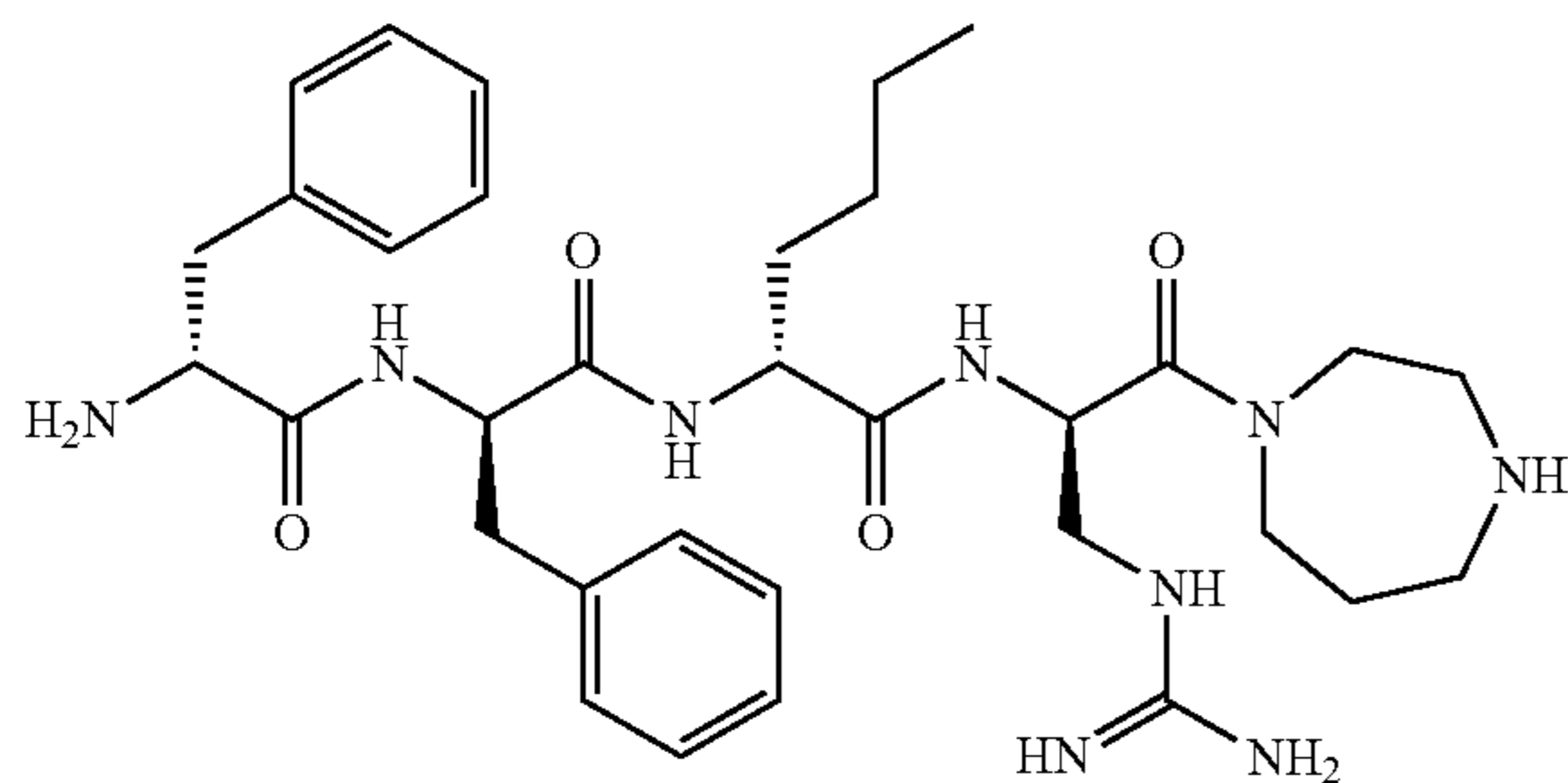
Compound (21): D-Phe-D-Phe-D-Nle-( \beta -amidino) D-Dap-[homopiperazine amide]
