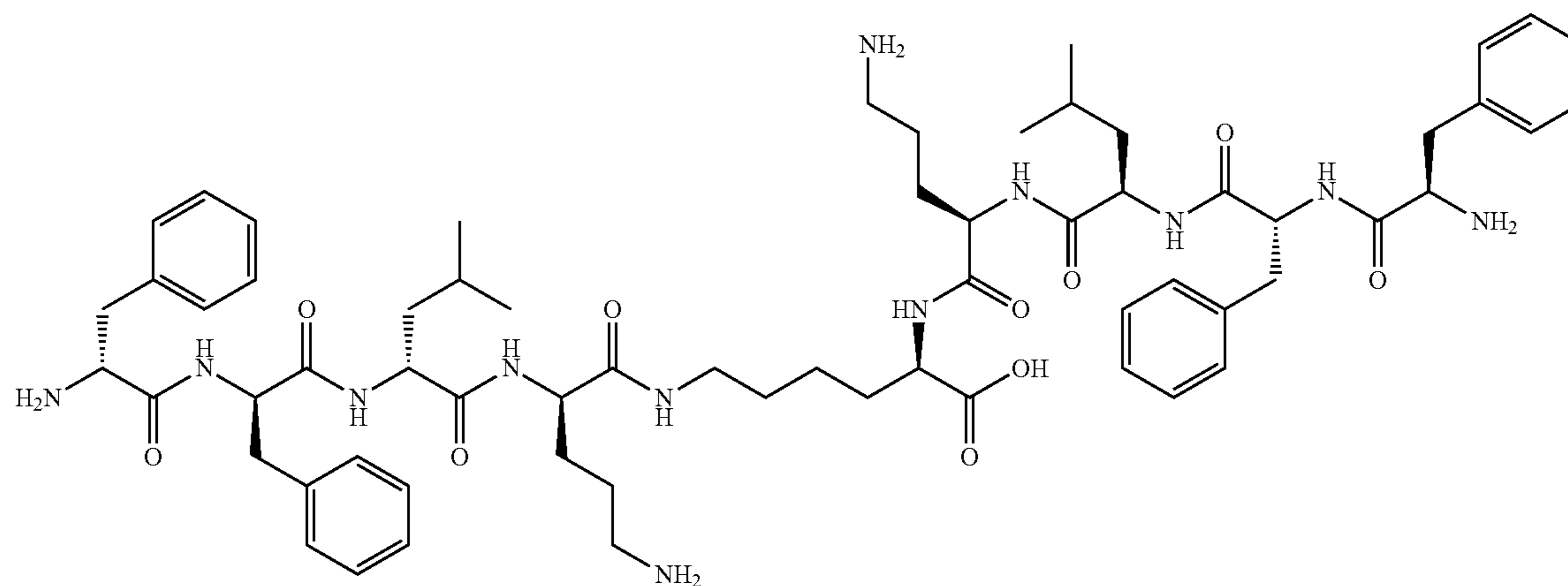
Compound (86): 1N,4N-bis-[D-Phe-D-Phe-D-Leu-(iPr)D-Orn]-4-amino-4-carboxylic-piperidine
