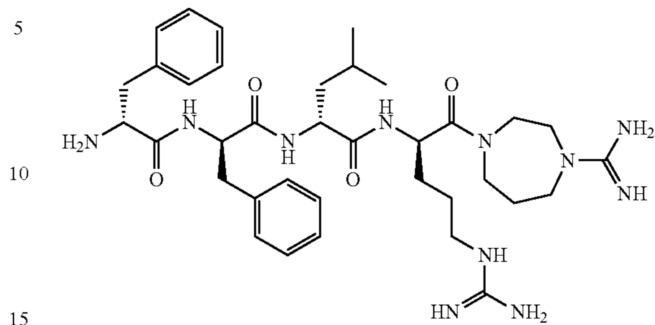
Compound (25): D-Phe-D-Phe-D-Leu-D-Lys-[2,8- diazaspiro[4,5]decan-1-one amide]
