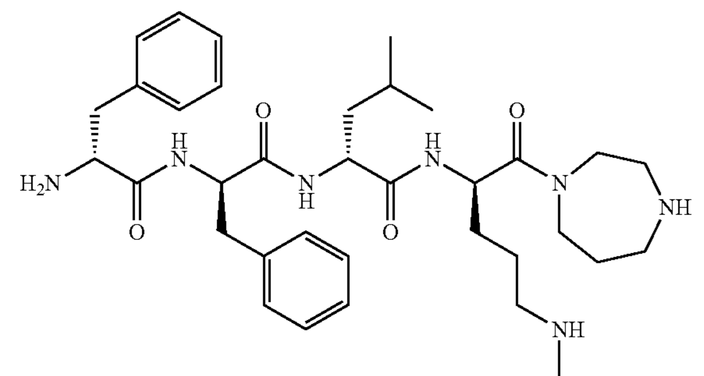
Compound (61) D-Phe-D-Phe-D-Leu-( \delta -iPr)D-Orn- [homopiperazine amide]
