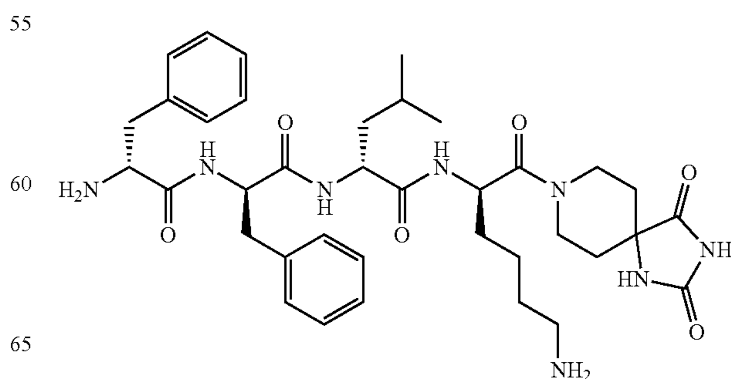
Compound (27): D-Phe-D-Phe-D-Leu-D-Lys-[1,3,8- triazaspiro[4,5]decane-2,4-dione amide]
