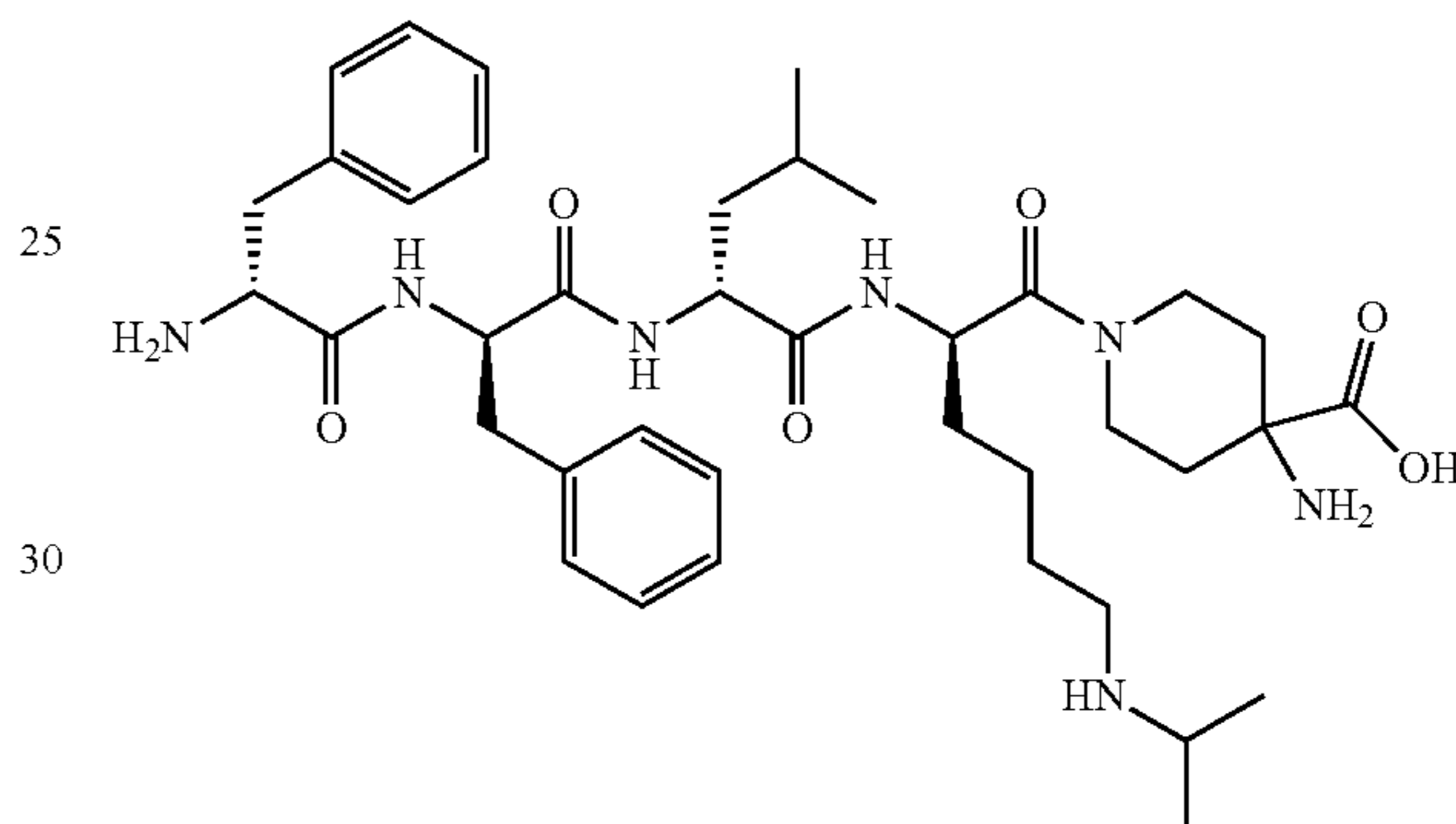
Compound (10): D-Phe-D-Phe-D-Leu-(β-amidino)D-Dap-[ω(4-aminopiperidine-4-carboxylic acid)]-OH
