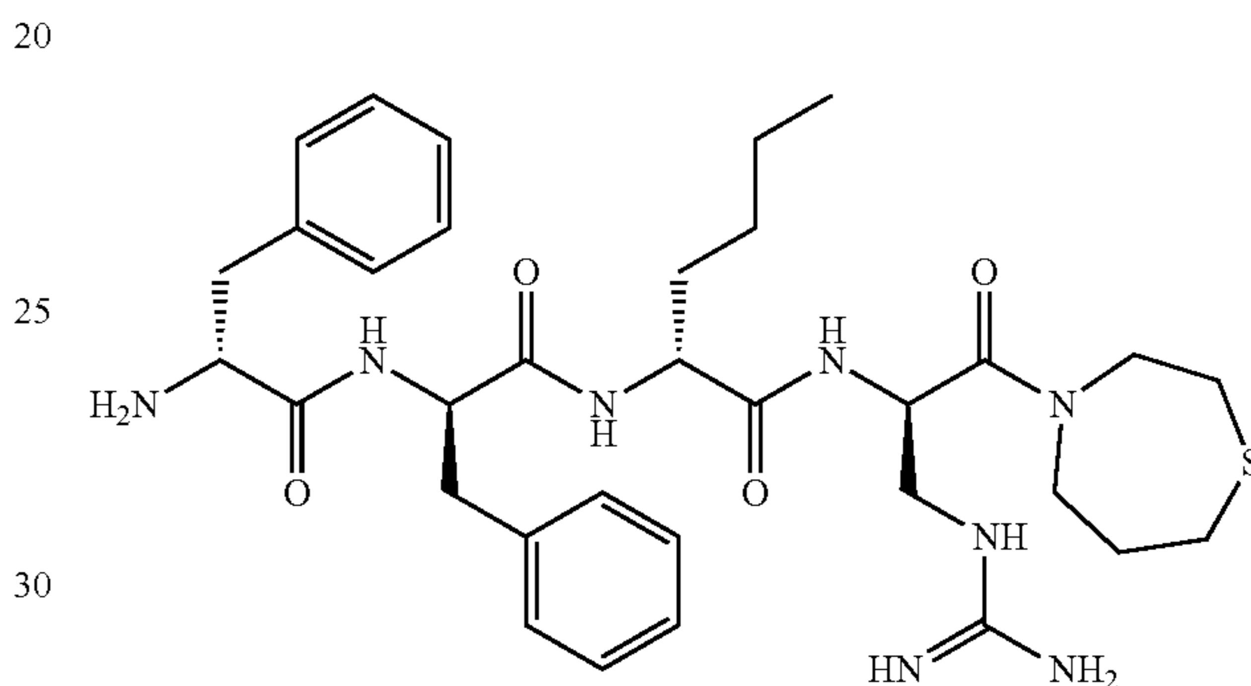
Compound (97) D-Phe-D-Phe-D-Nle-D-Dap(amidino)-[homothiomorpholine amide]
