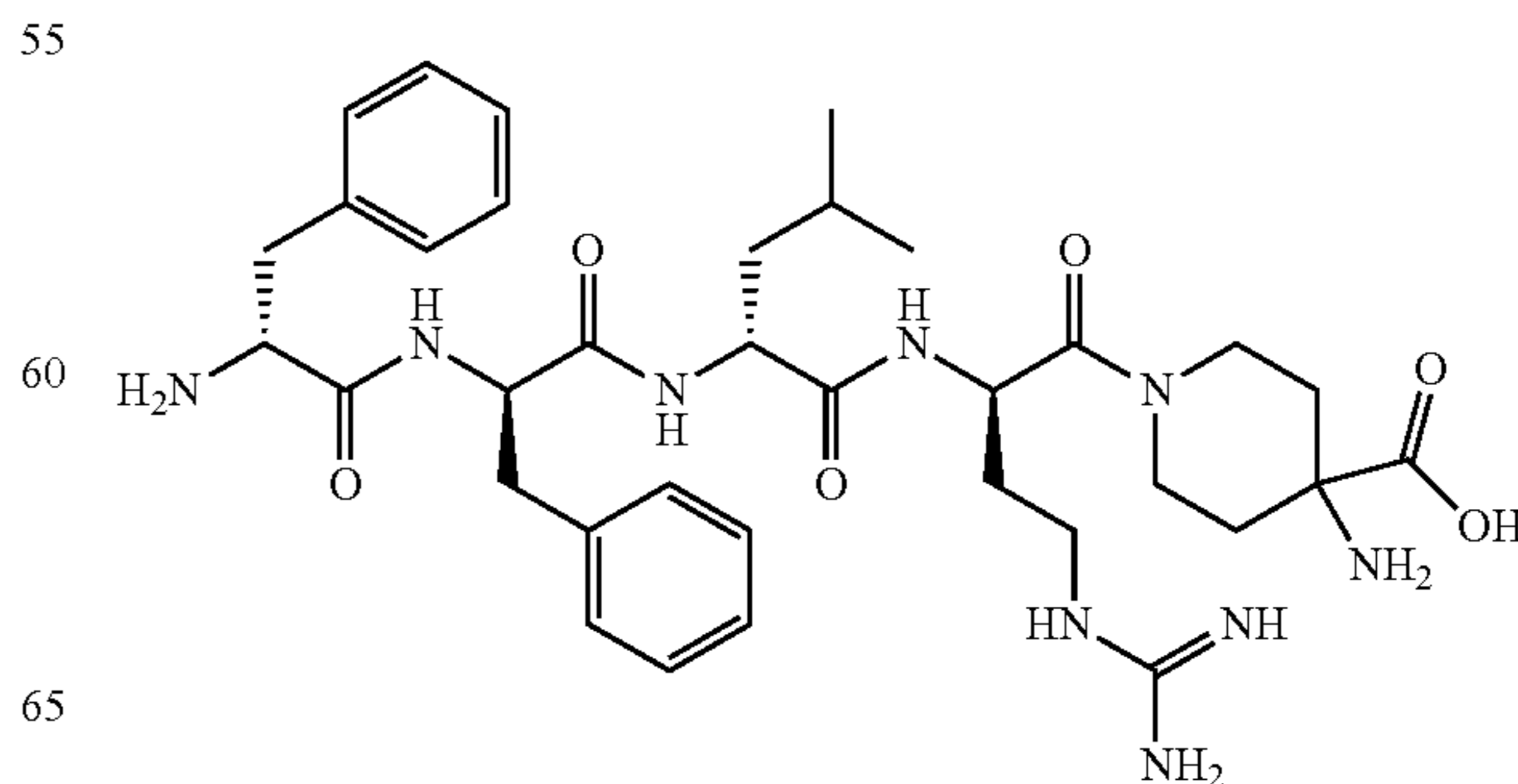
Compound (11): D-Phe-D-Phe-D-Leu-D-Nar-[ω(4-aminopiperidine-4-carboxylic acid)]-OH
