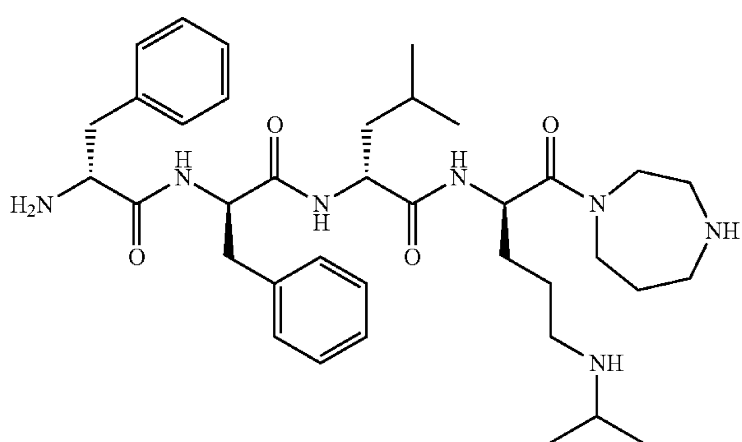
Compound (61) D-Phe-D-Phe-D-Leu-( \delta -iPr)D-Orn- [homopiperazine amide]
