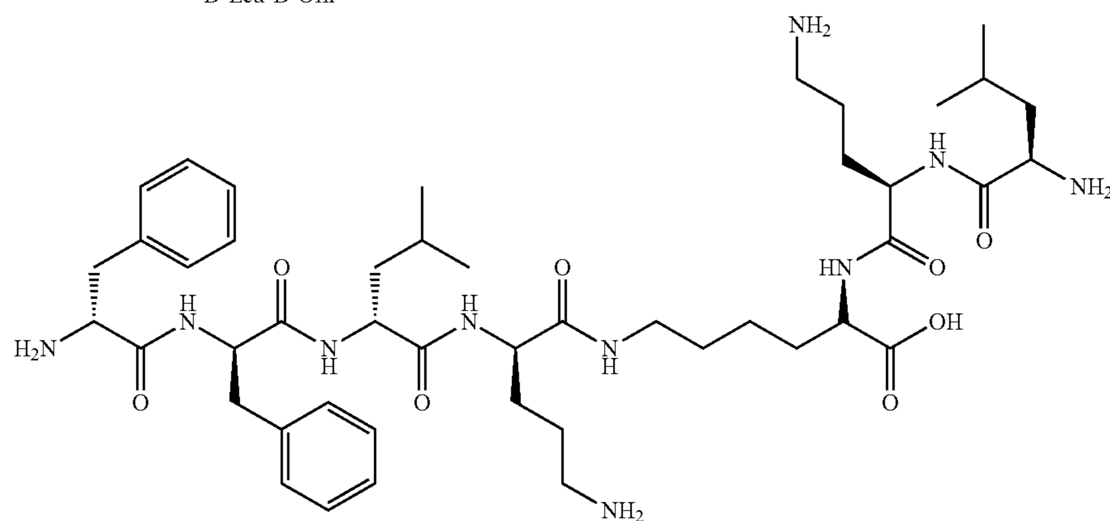
Compound (78)
