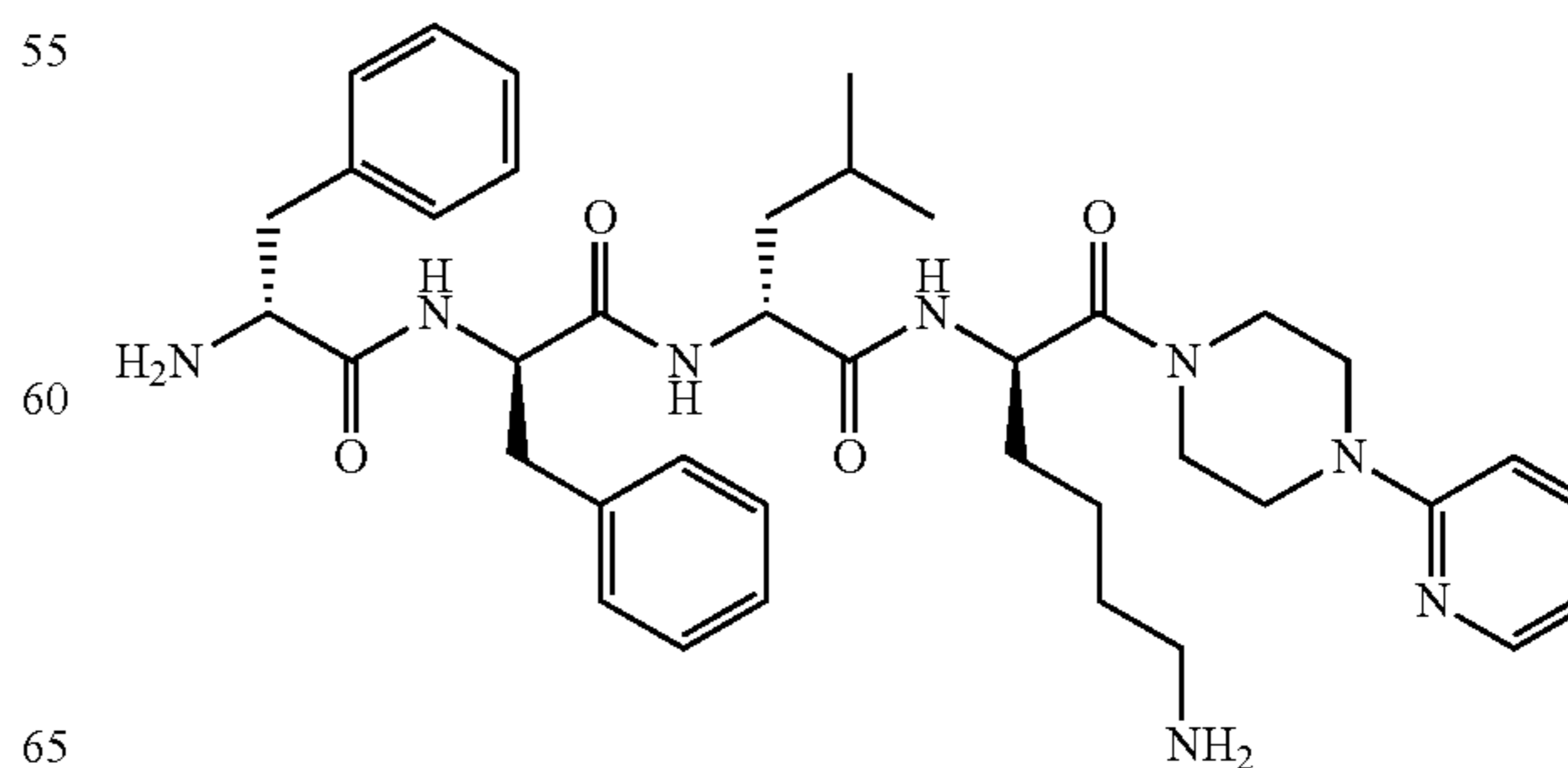
Compound (65): D-Phe-D-Phe-D-Leu-D-Lys-[1- (pyridin-2-yl)piperazine amide]
