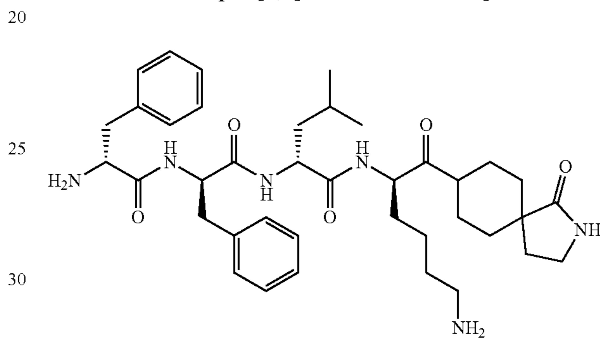
Compound (25): D-Phe-D-Phe-D-Leu-D-Lys-[2,8- diazaspiro[4,5]decan-1-one amide]
