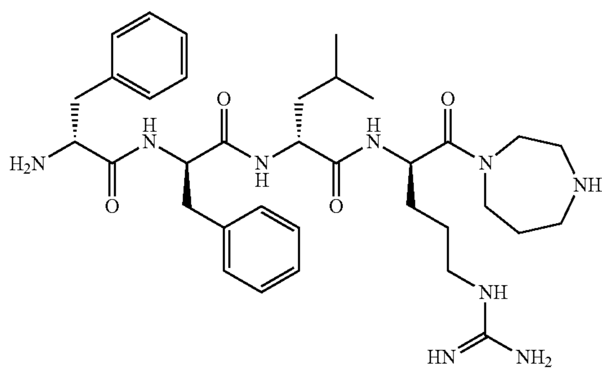
Compound (7): D-Phe-D-Phe-D-Leu-D-Arg-[homopiperazine amide]
