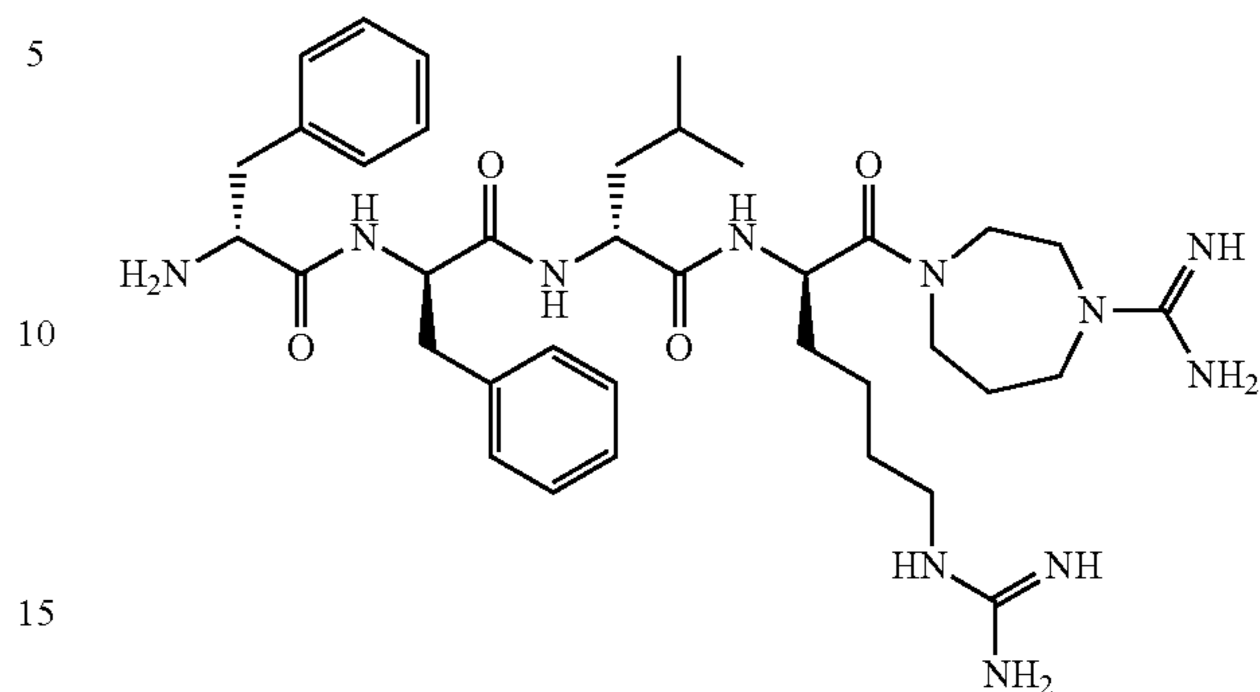
Compound (17): D-Phe-D-Phe-D-Leu-(ε-iPr)D-Lys-[4-amidinohomopiperazine amide]
