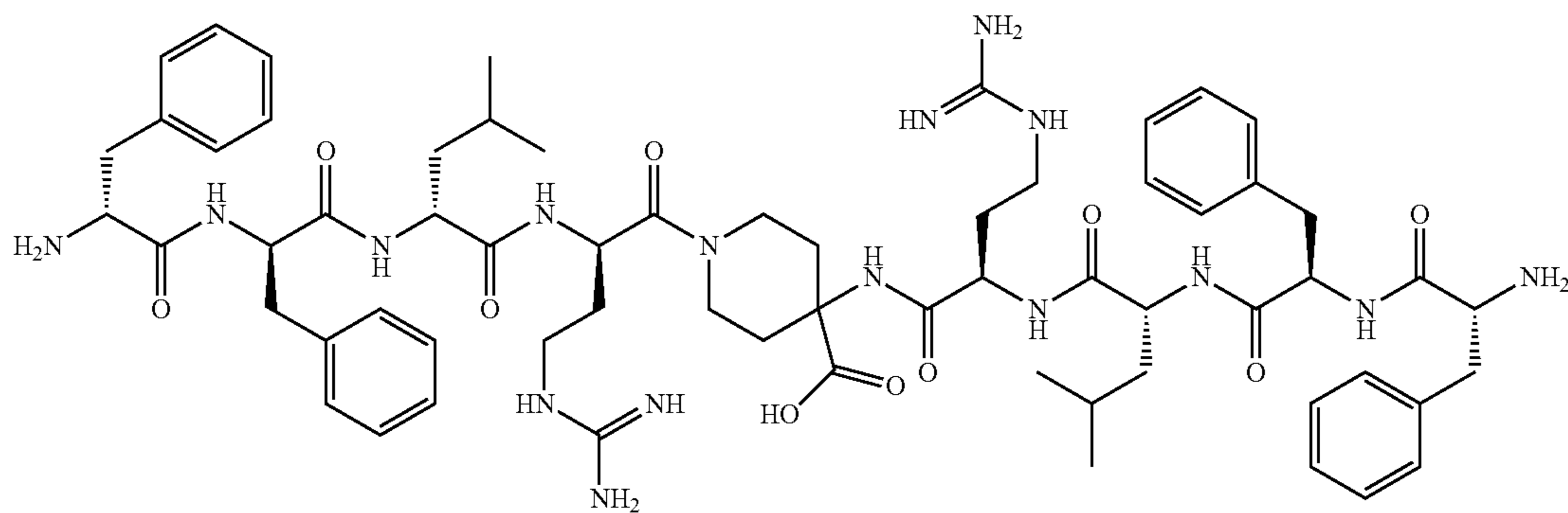
Compound (88): 1N,4N-bis-(D-Phe-D-Phe-D-Leu-D-Nar)-4-amino-4-carboxylic piperidine
