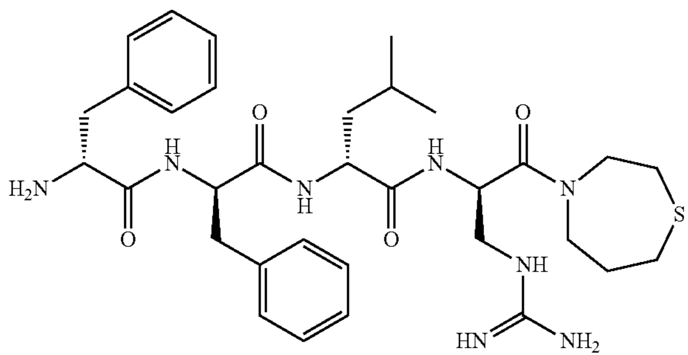
Compound (95) D-Phe-D-Phe-D-Leu-D-Dap(amidino)-[homothiomorpholine amide]
