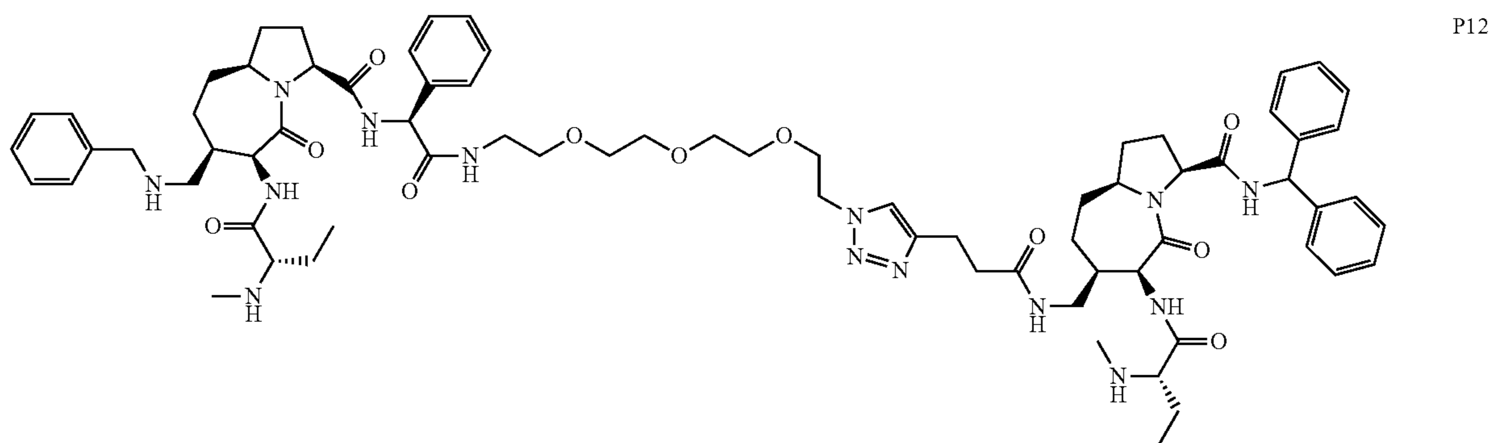
Compound 34a
