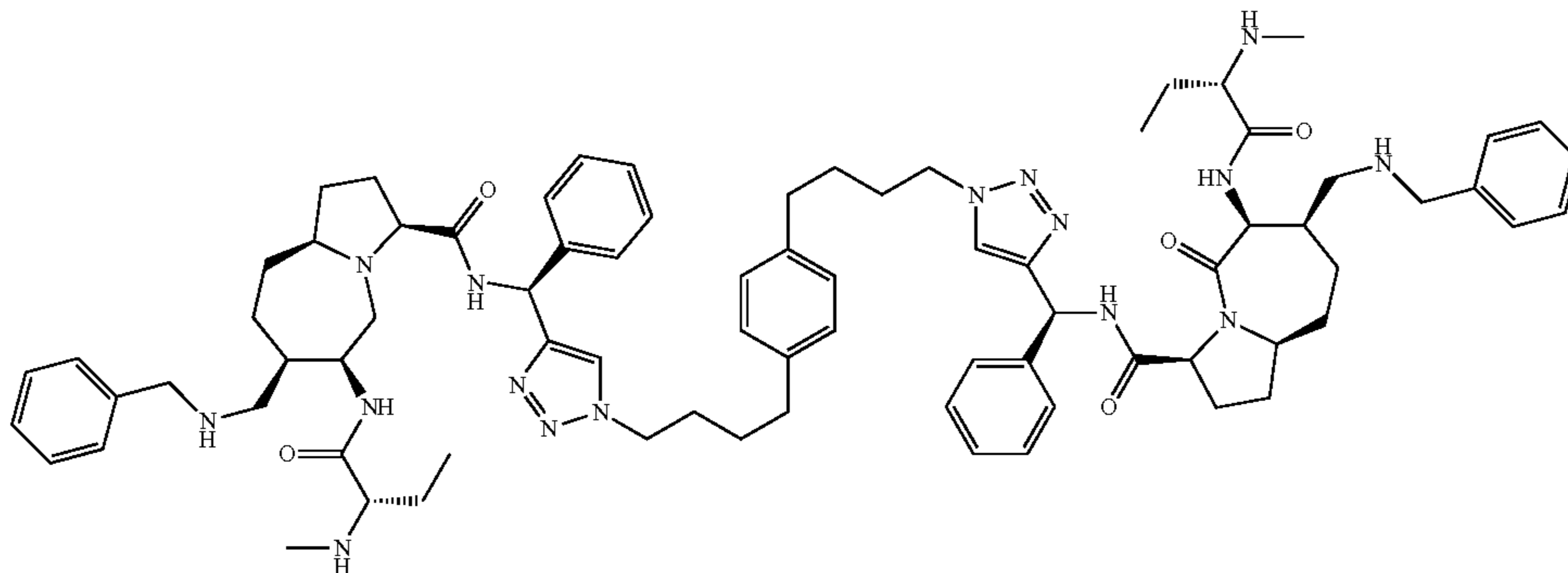
Compound 28a
