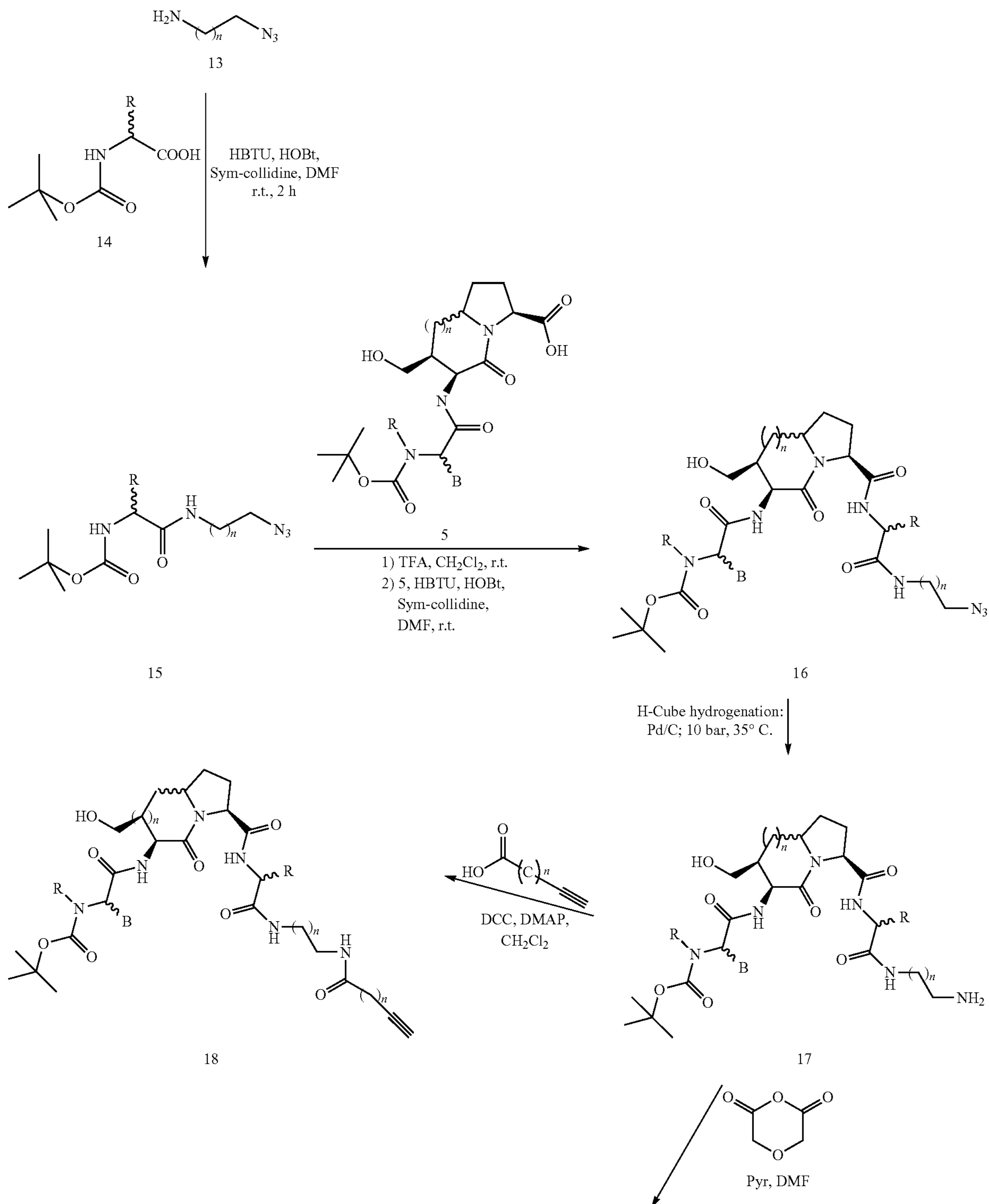
Scheme 3
