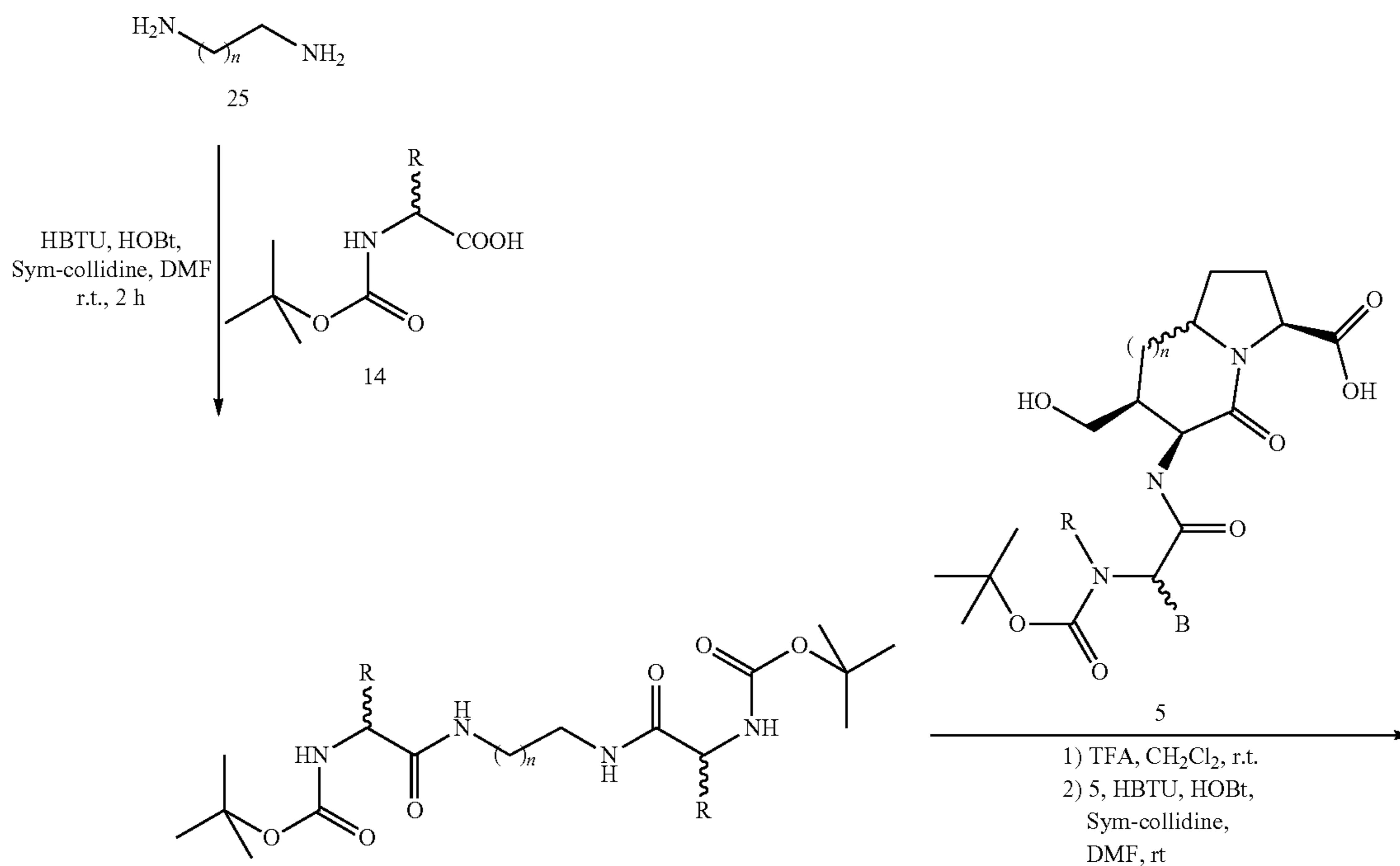
Scheme 8
