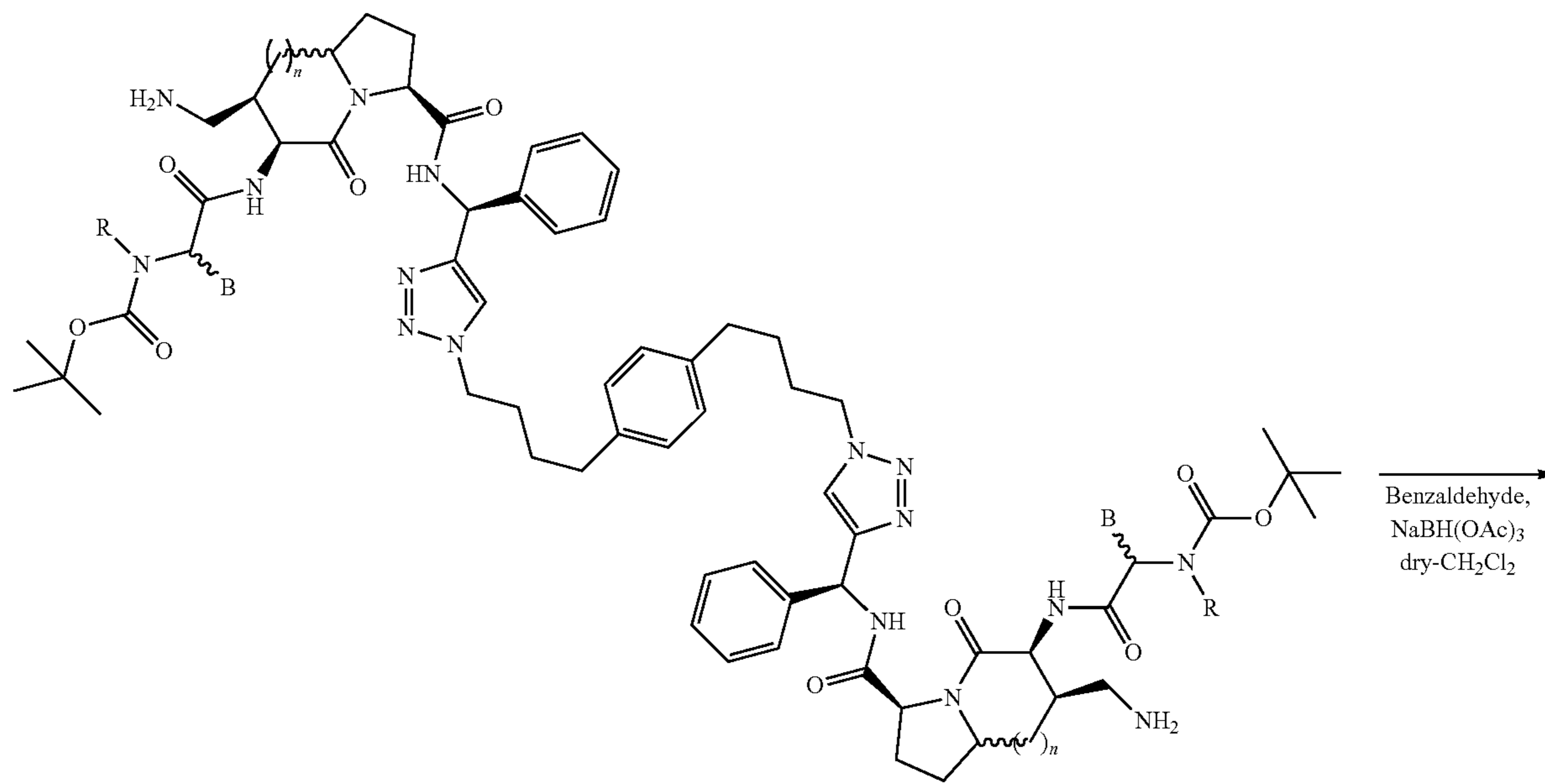
Scheme 7
