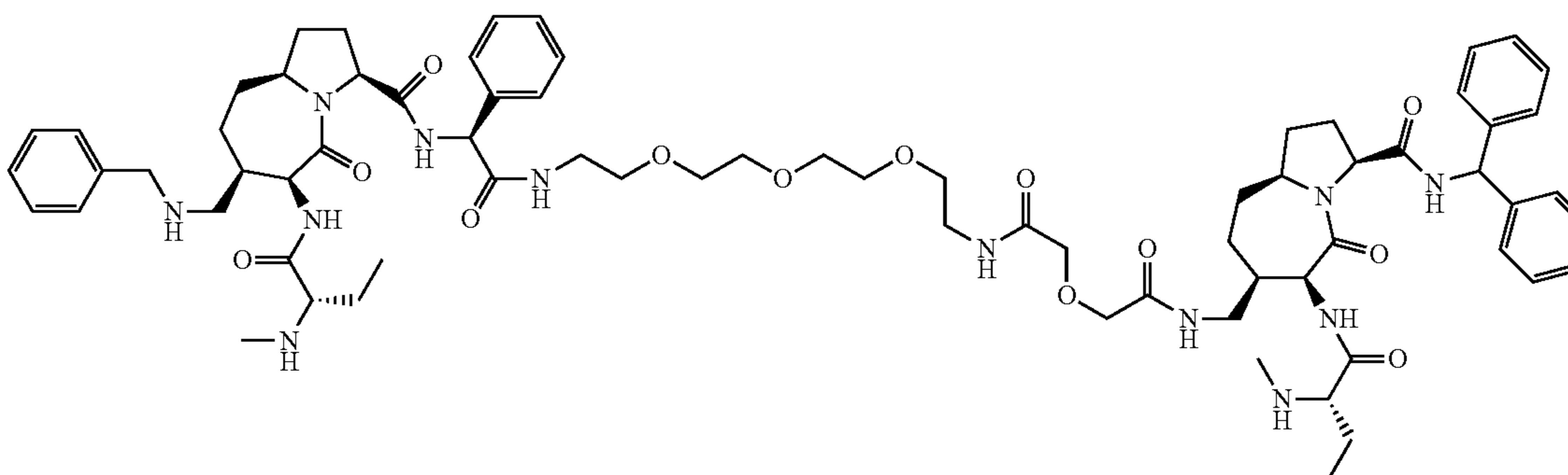
Compound 36a
