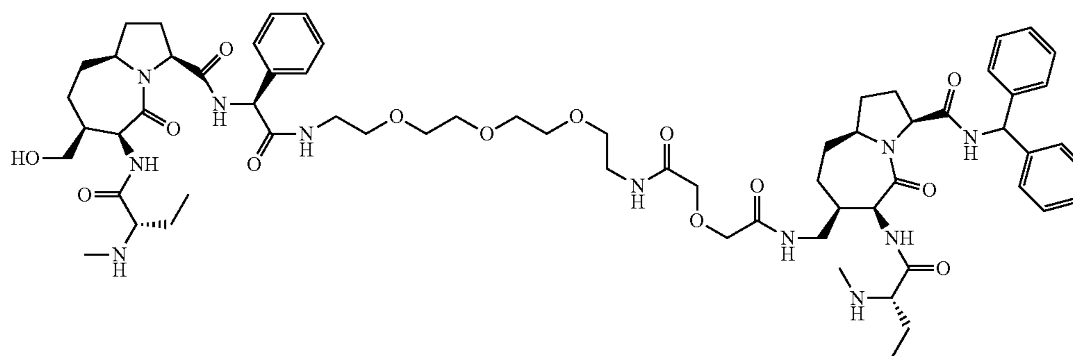
Compound 36a
