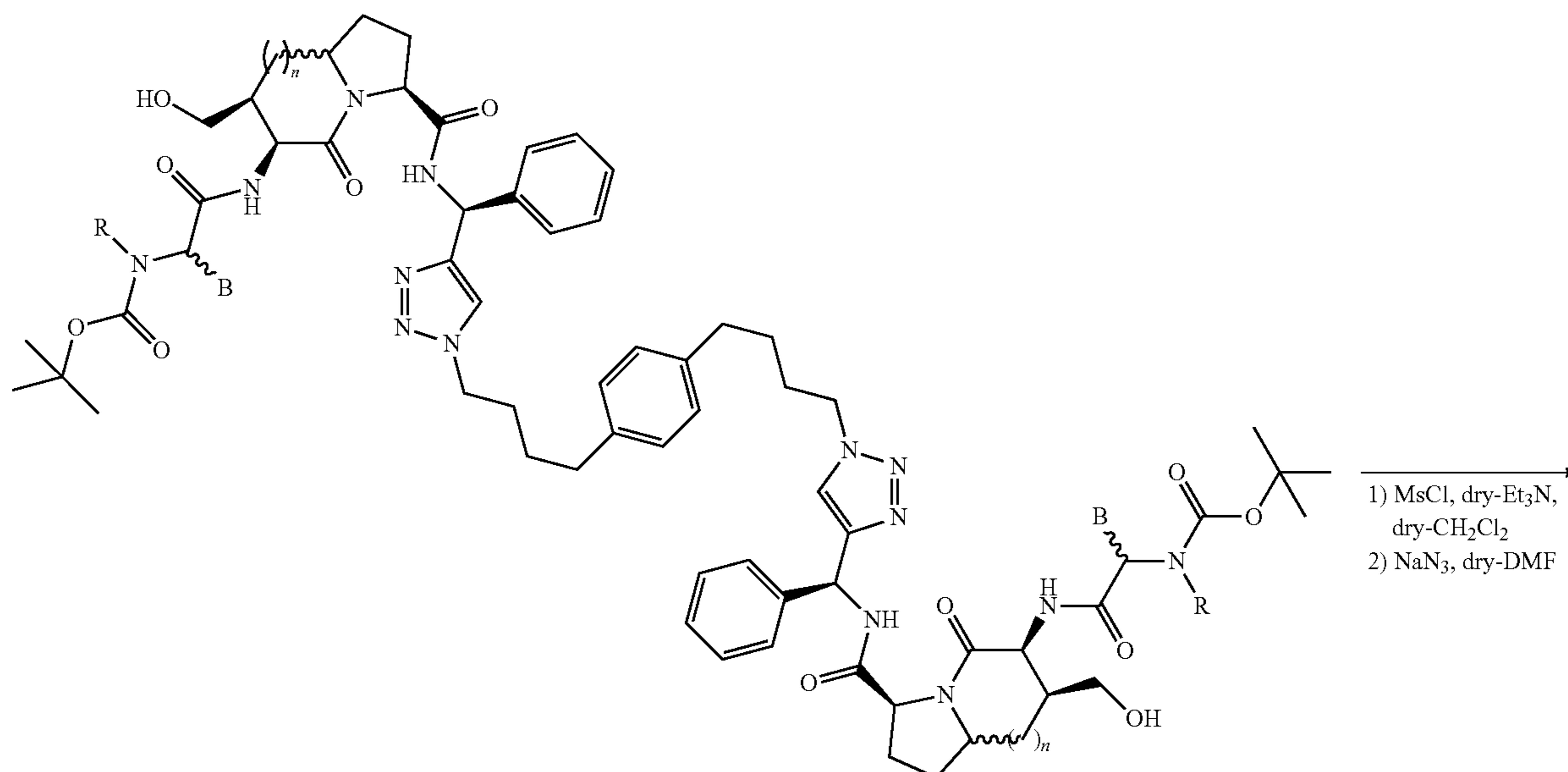
Scheme 5
