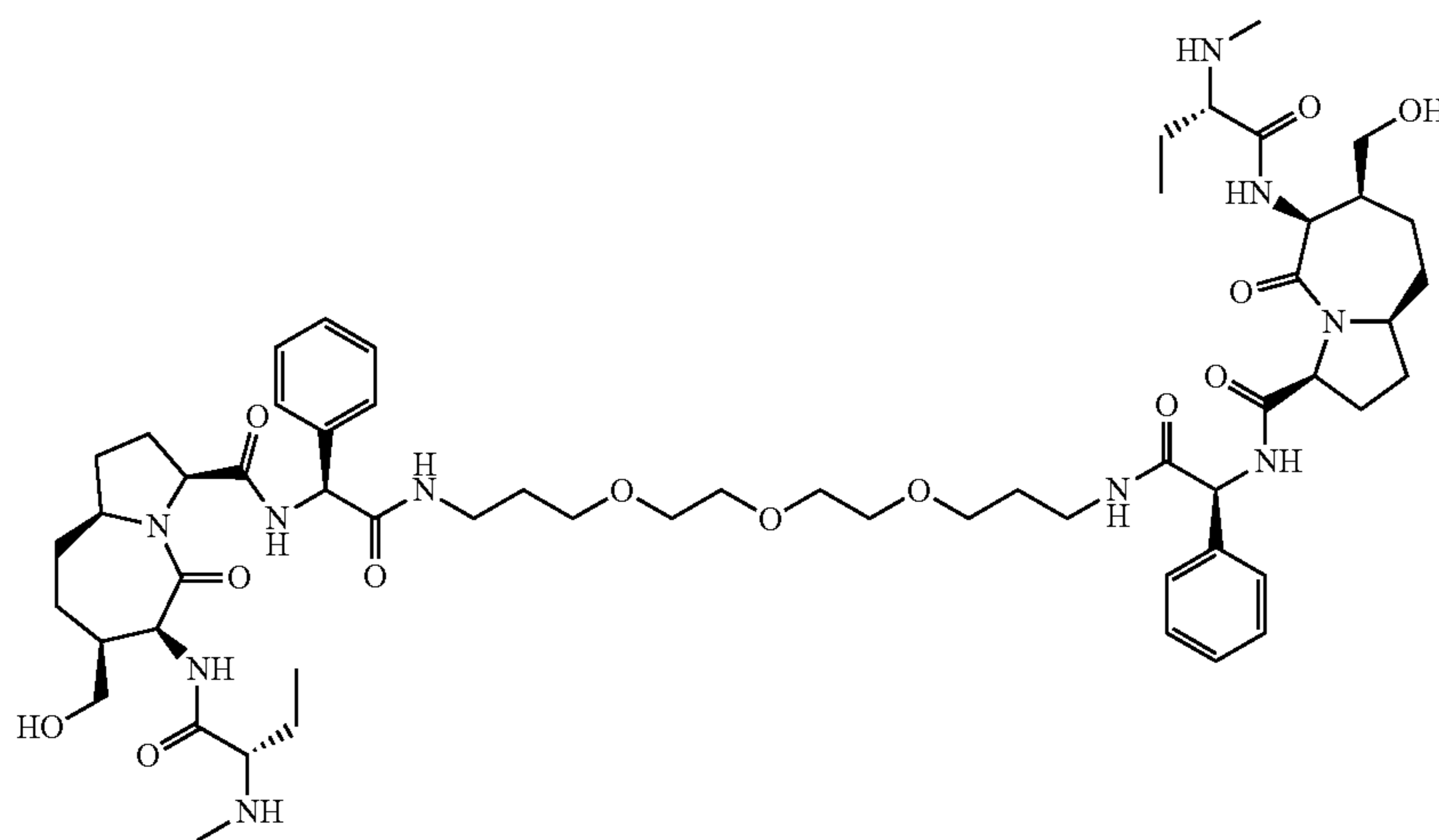
Compound 30d
