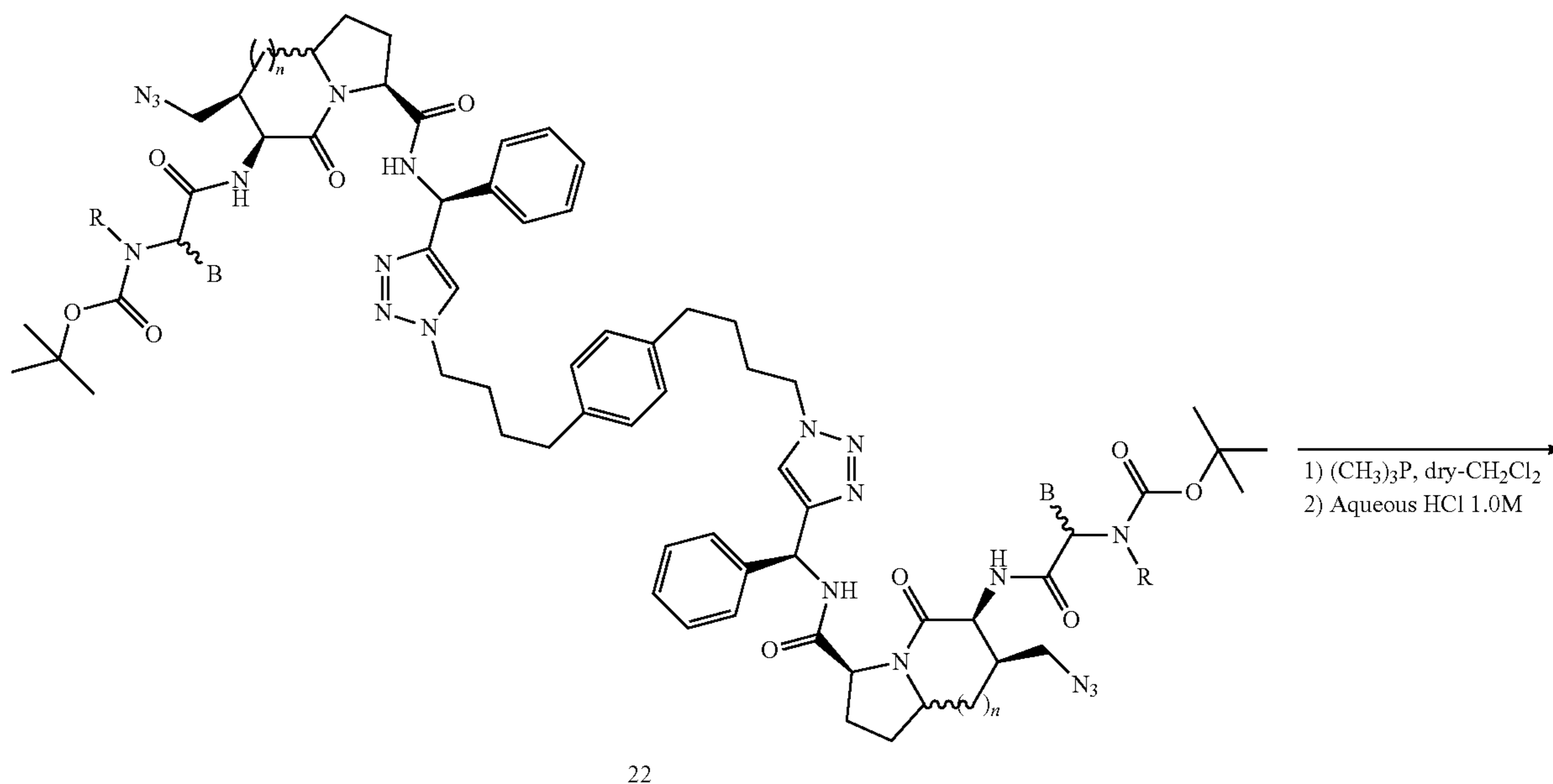
Scheme 6
