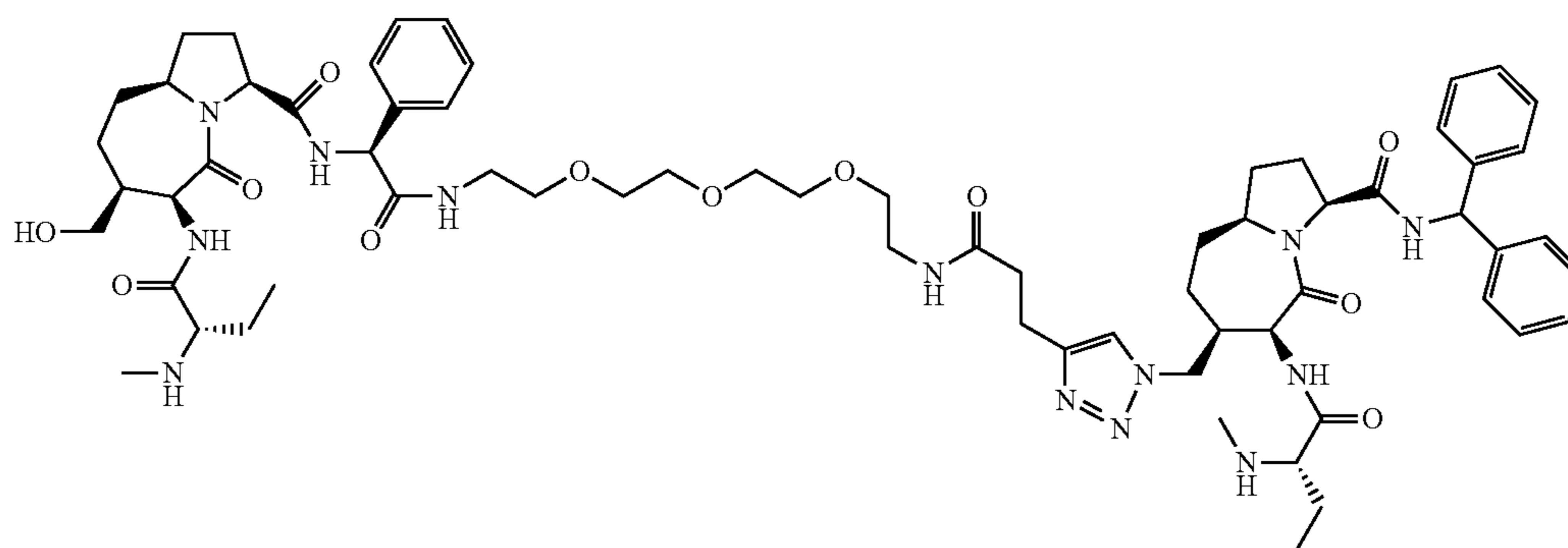
Compound 35a
