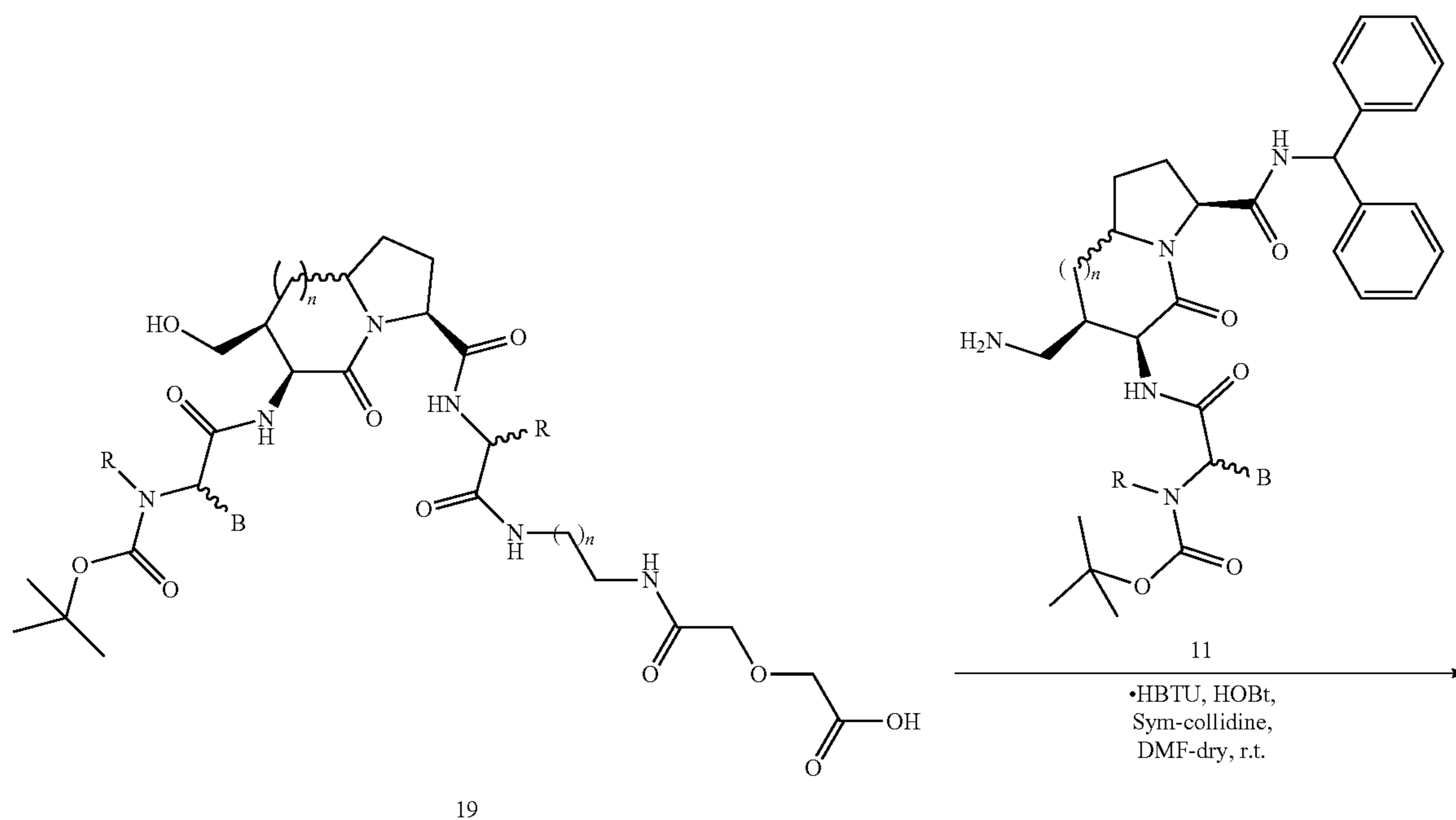
Scheme 11
