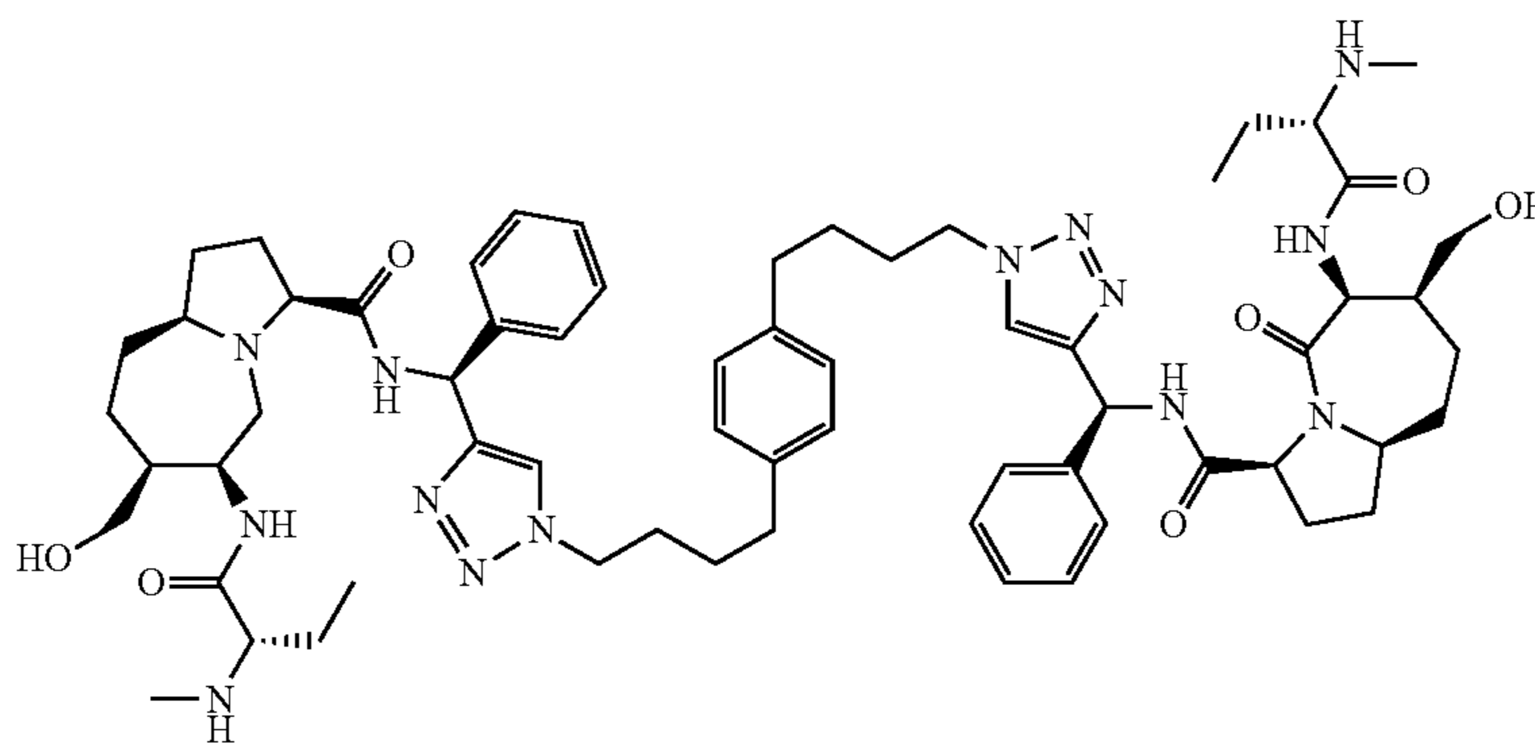
Compound 28a
