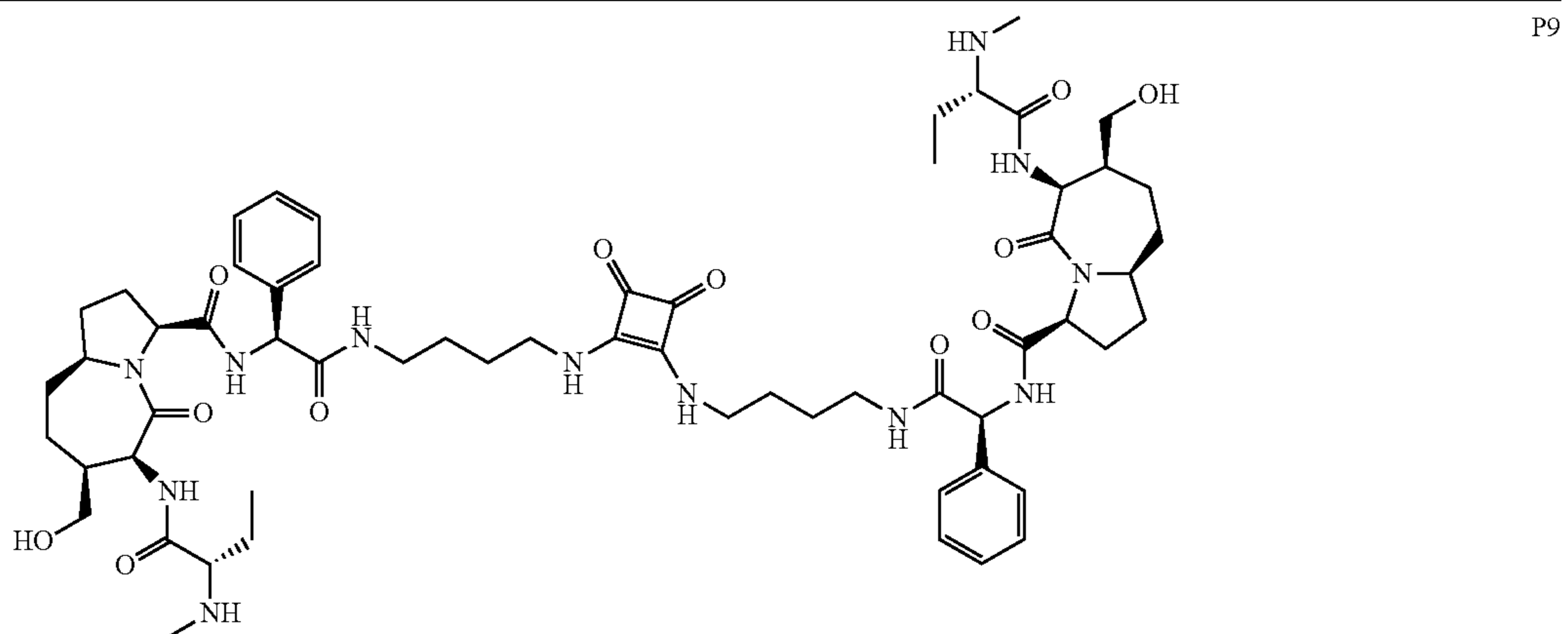
Compound 30b
