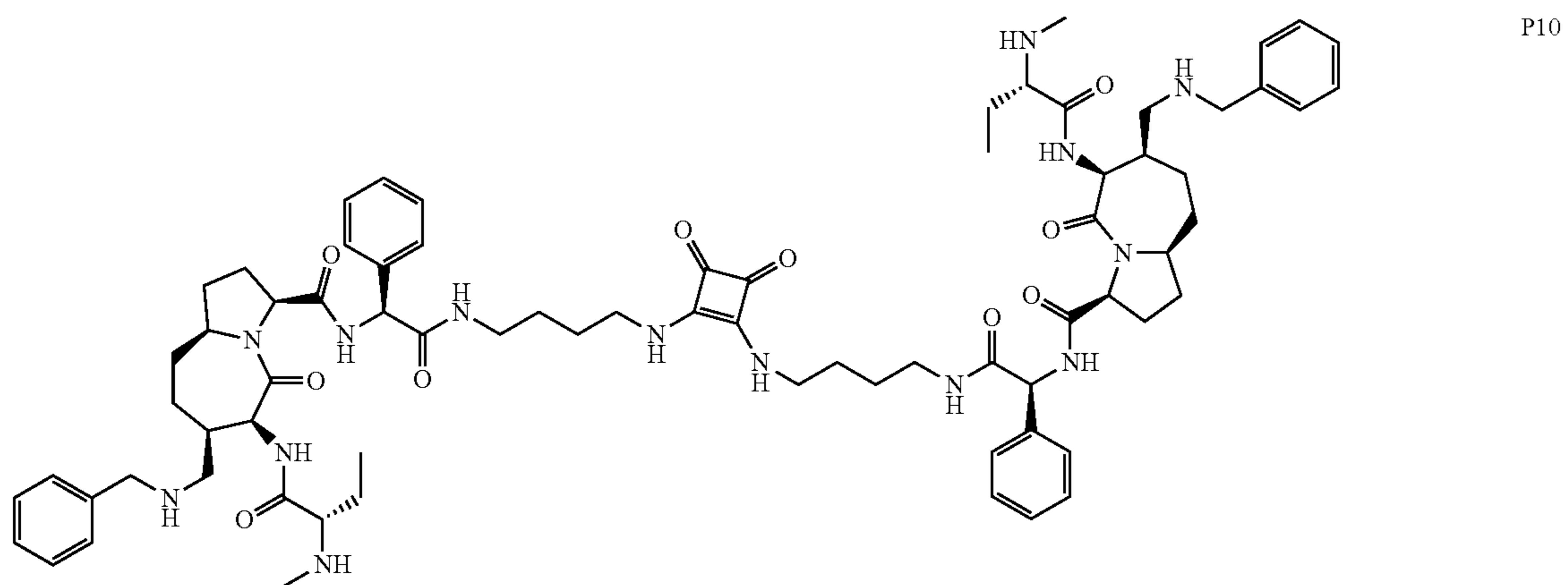
Compound 30b
