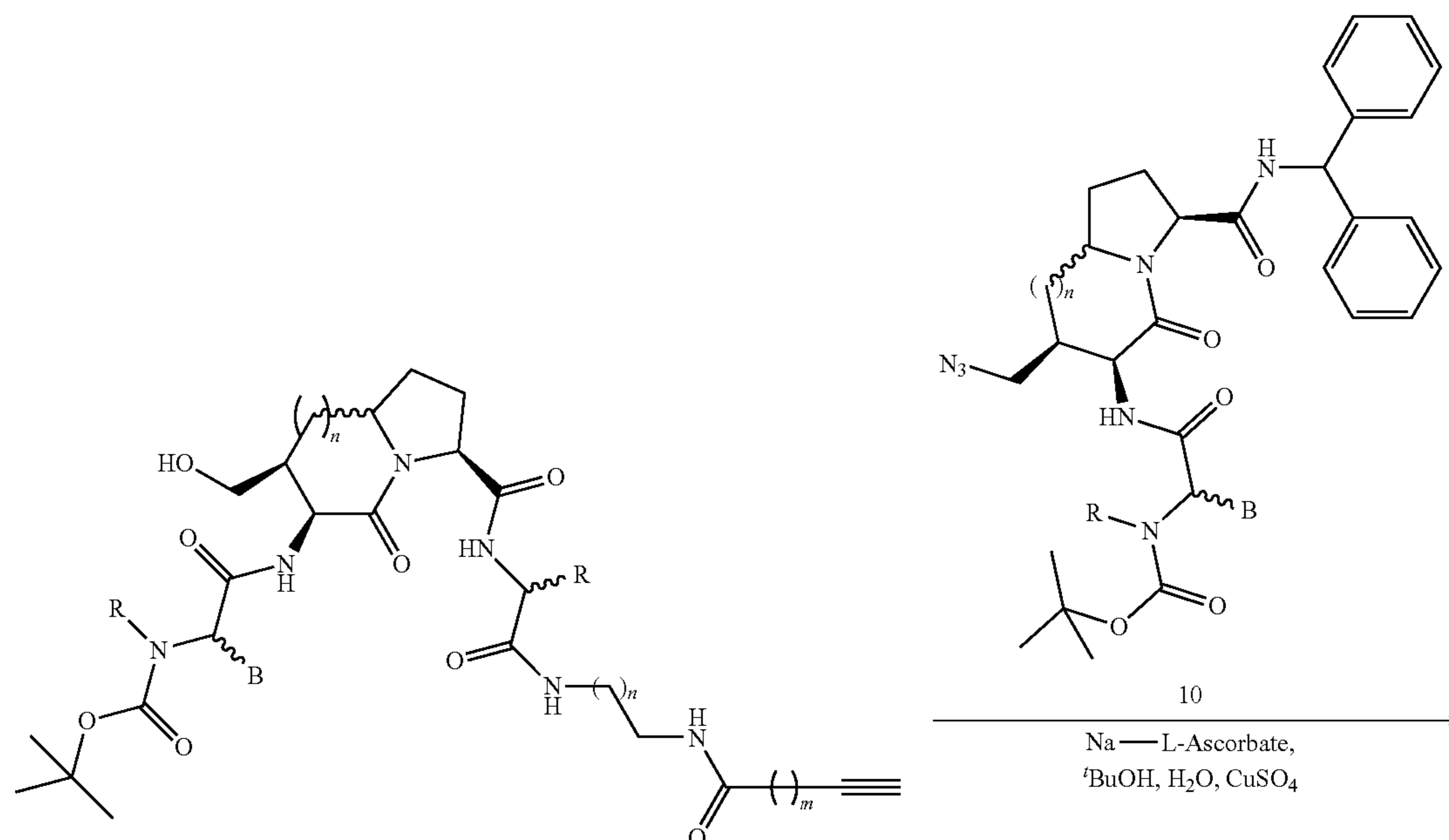
Scheme 10
