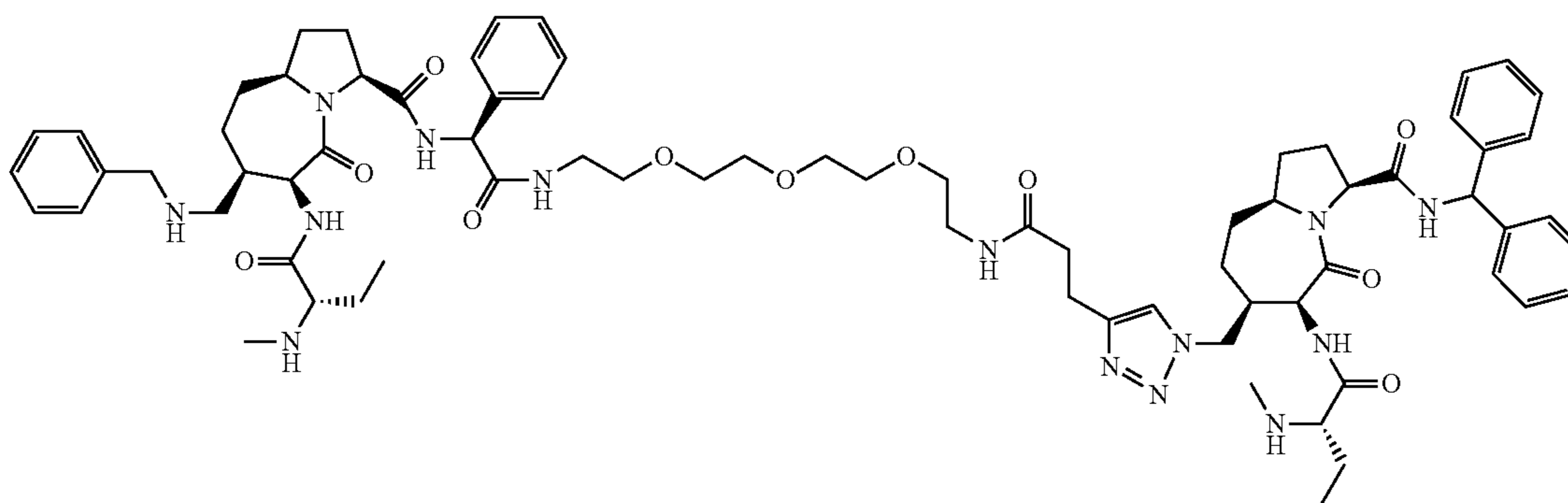
Compound 35a
