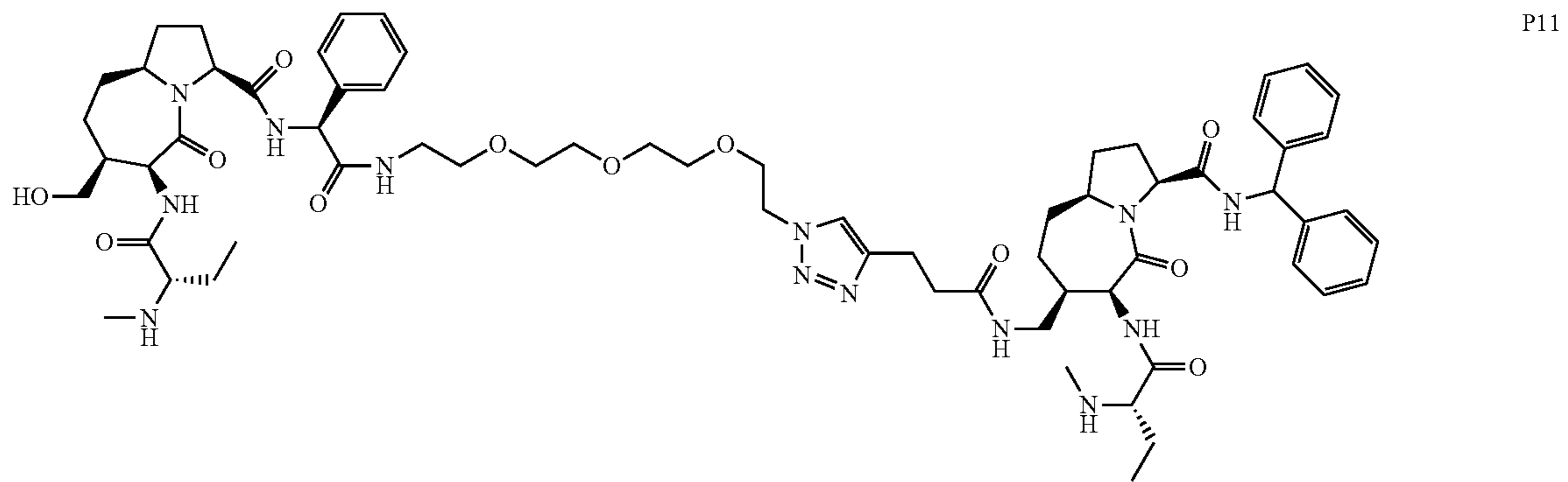
Compound 34a
