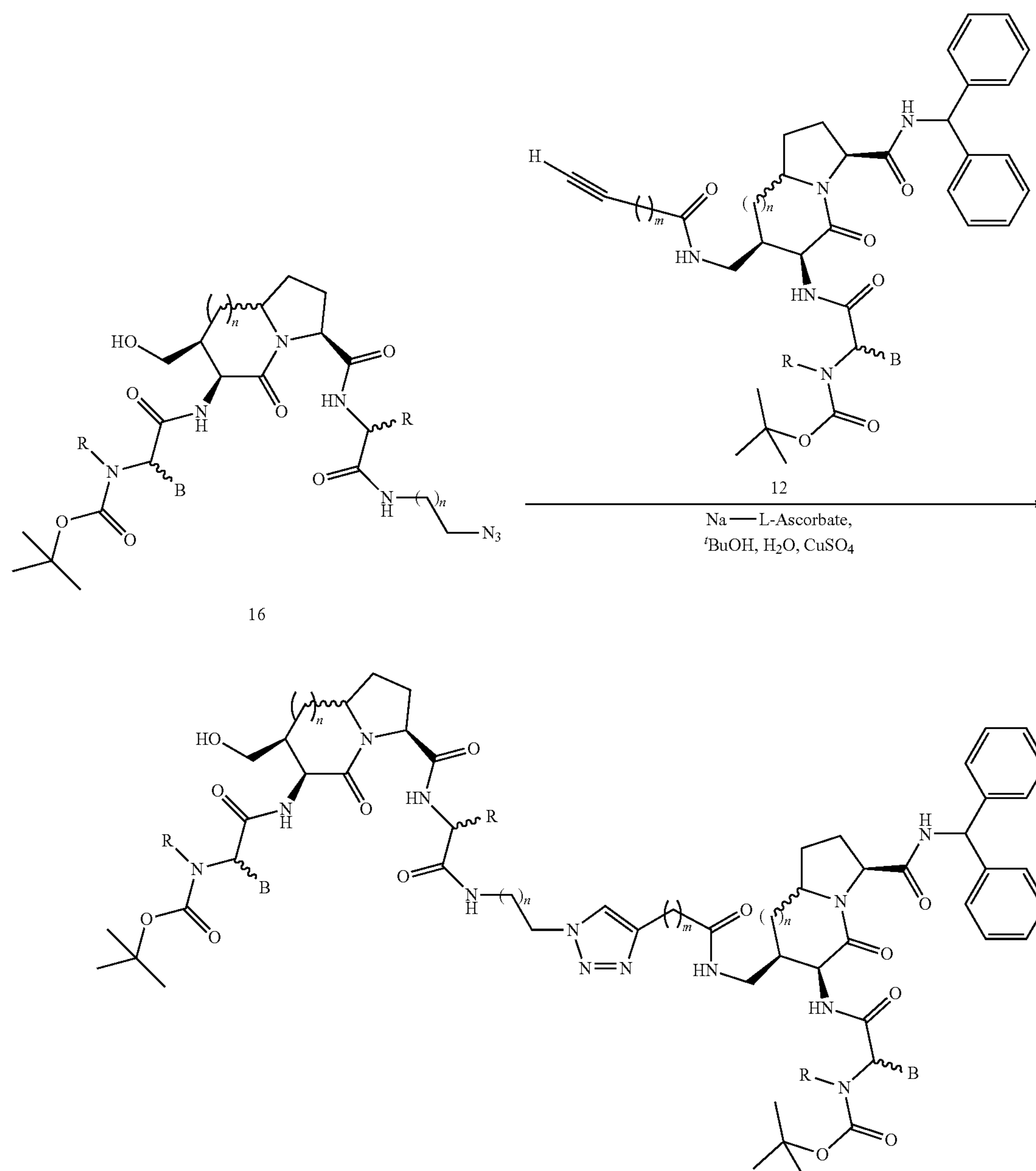
Scheme 9
