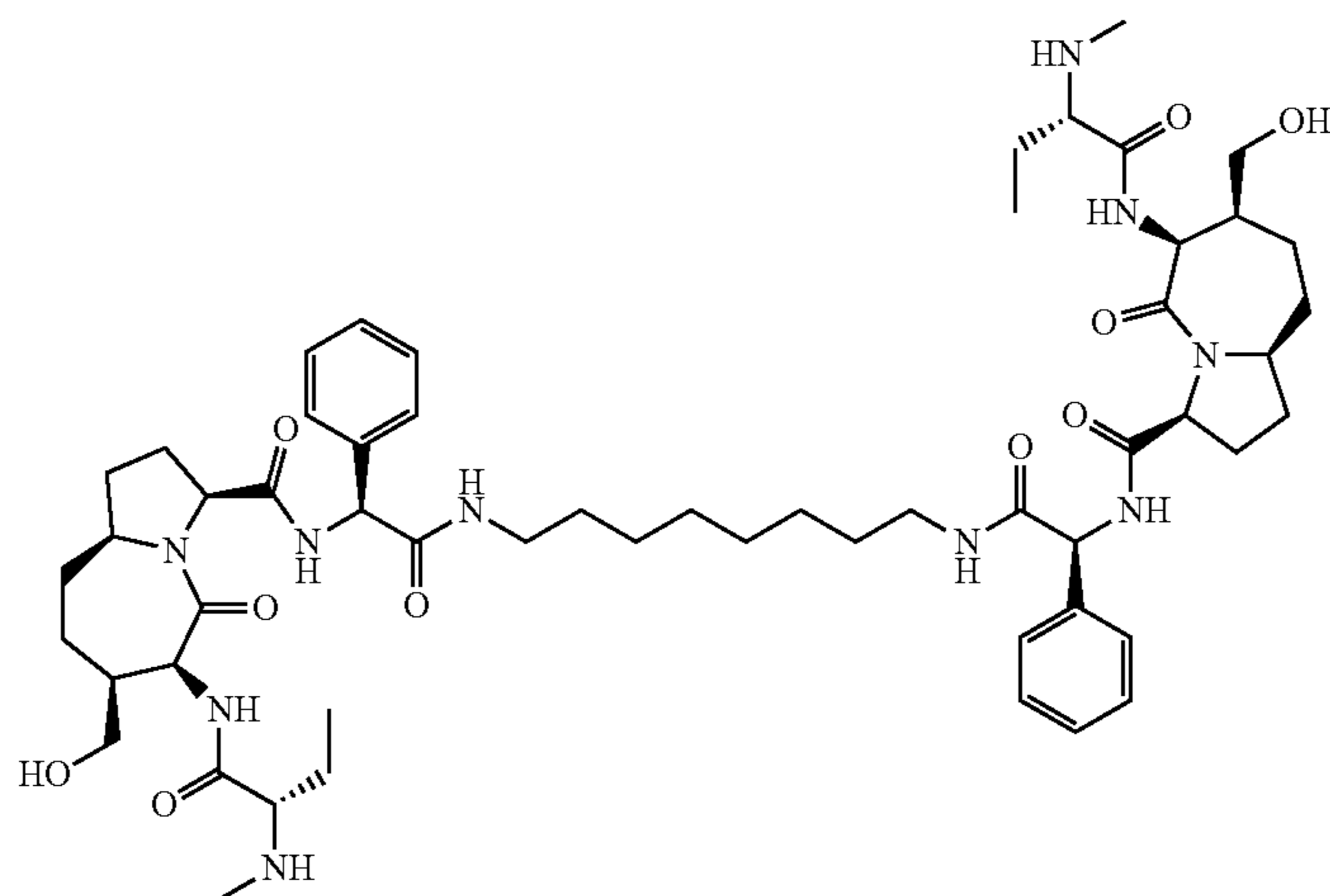
Compound 30a
