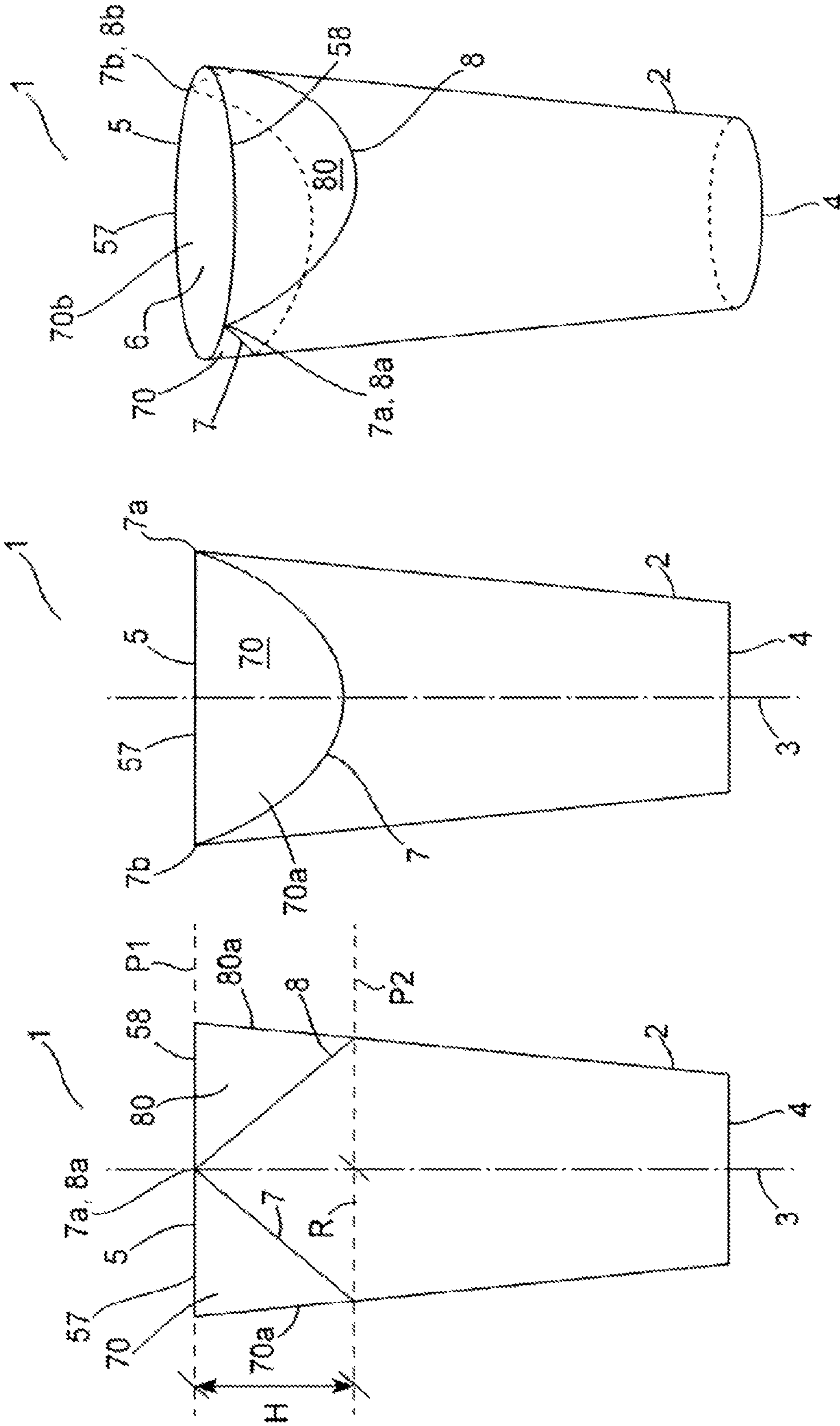
Fig. 1 (PRIOR ART)
