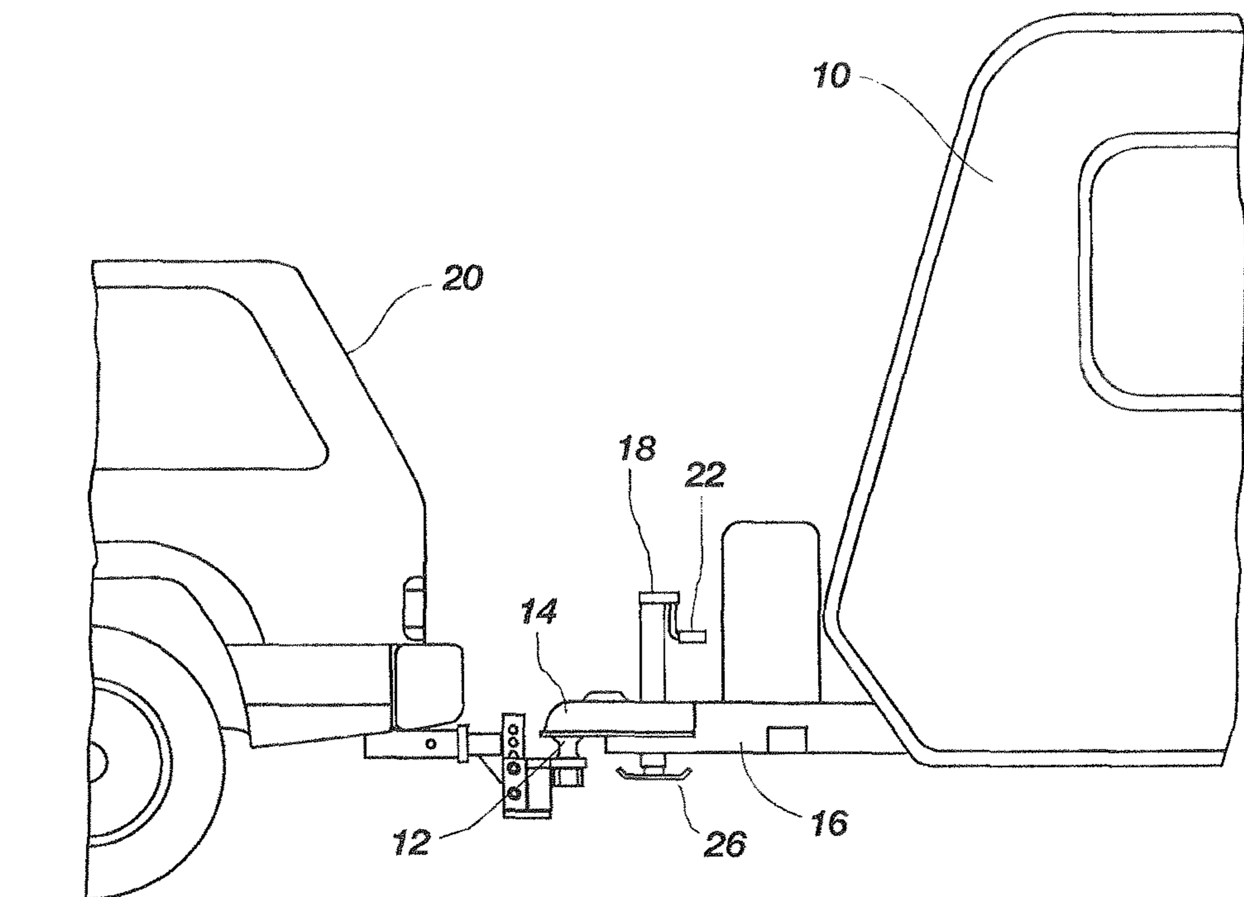
FIG. 3 (PRIOR ART)
