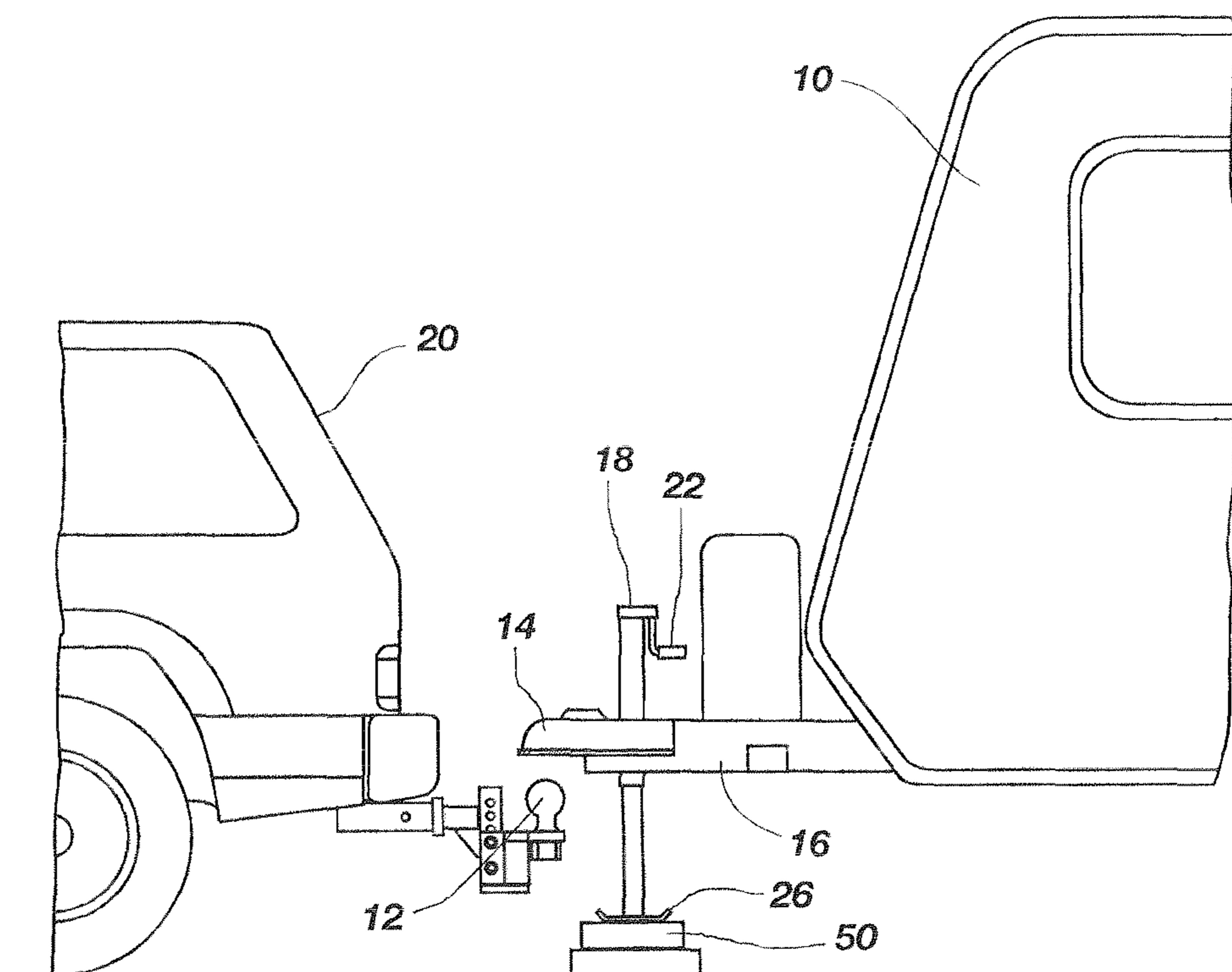
FIG. 5 (PRIOR ART)
