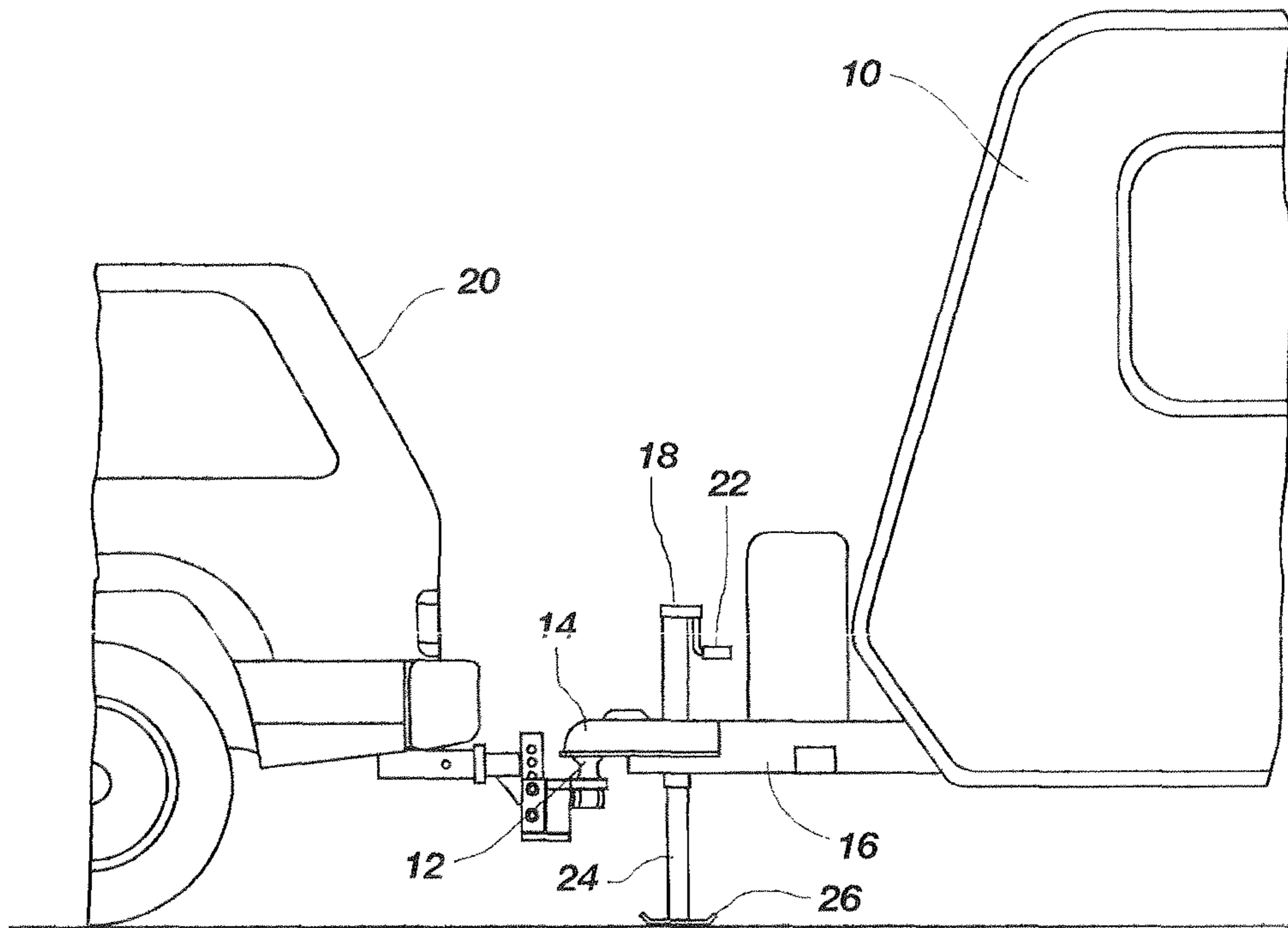
FIG. 2 (PRIOR ART)
