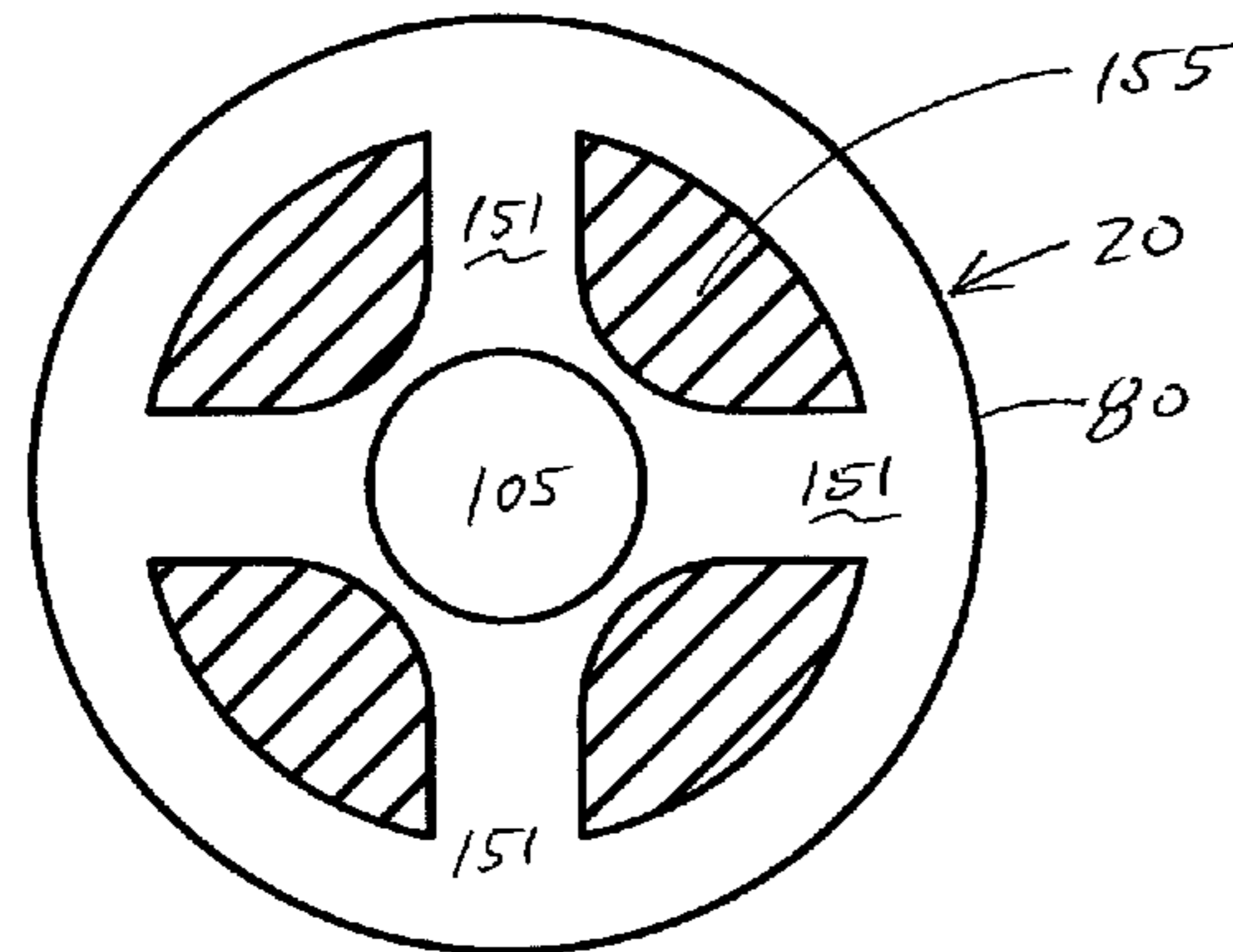
FIG. 10D (SECTION THRU FIG. 10A)
