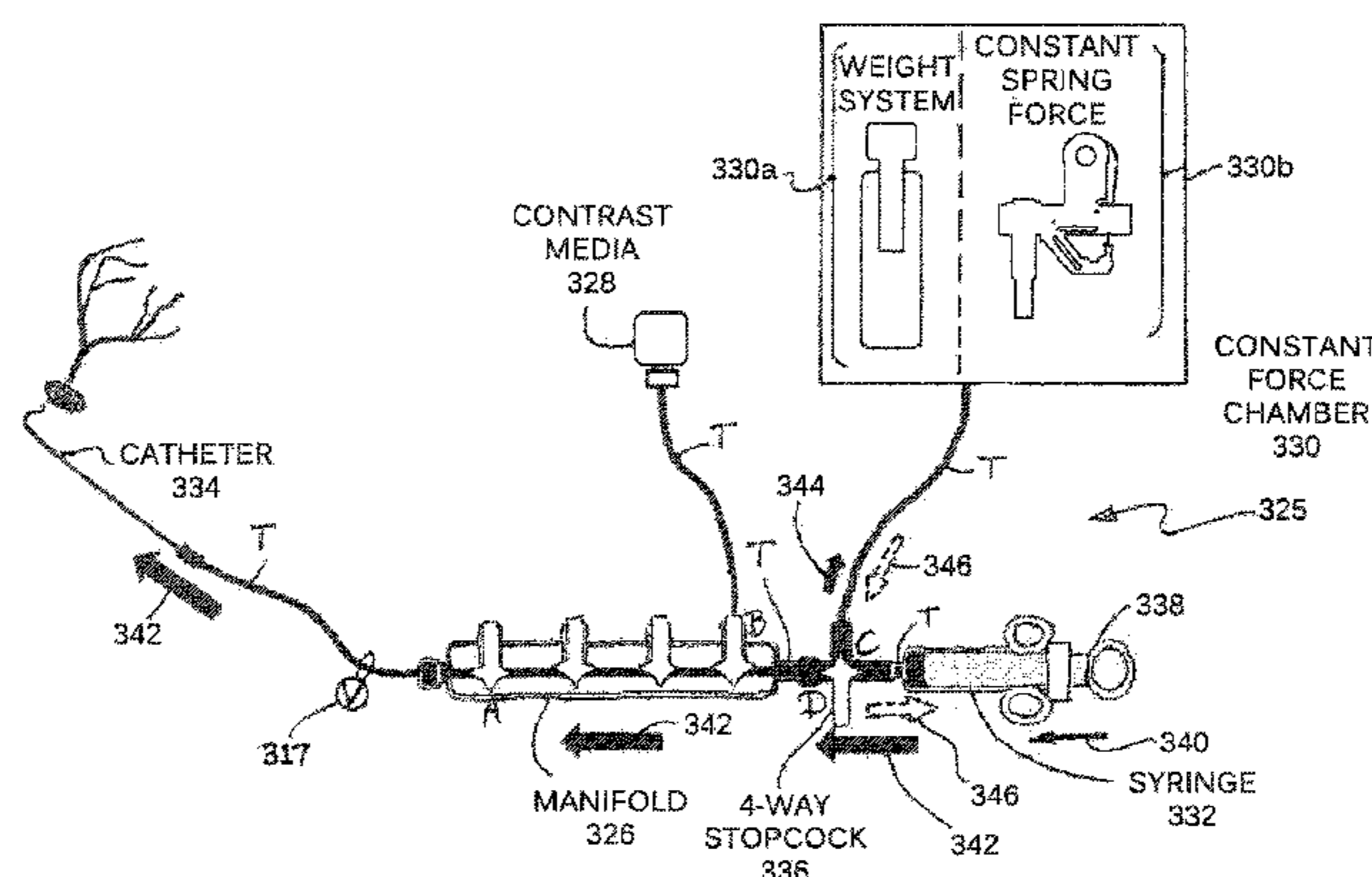
Exemplary Constant Force Modulator - Constant Force Chamber Open
