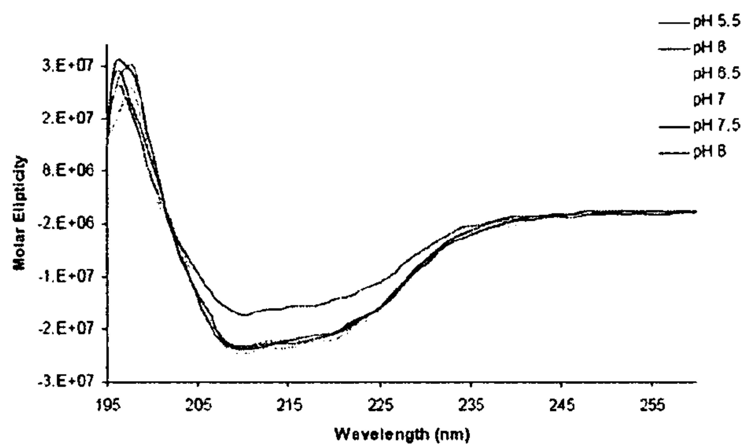
Toxoid A , CD (secondary structure)
