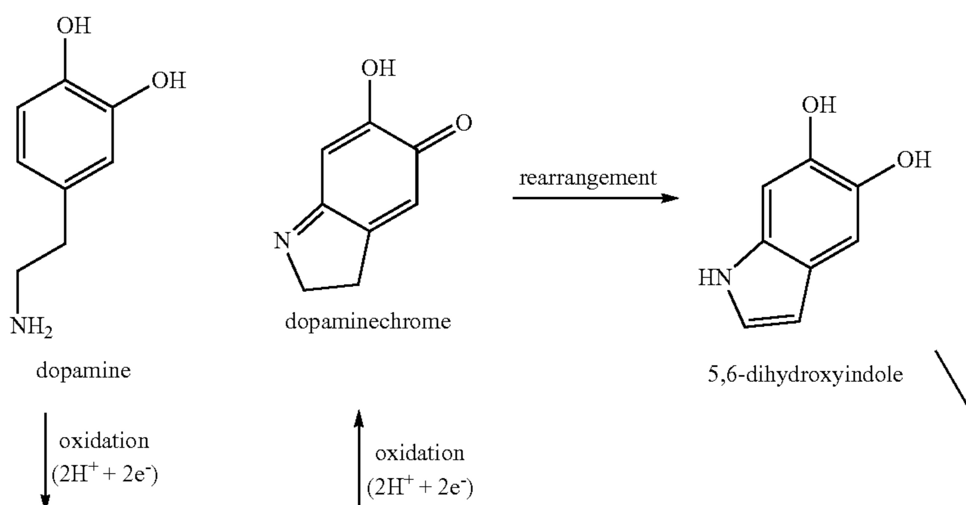
Scheme 1: proposed mechanism for polydopamine formation.
