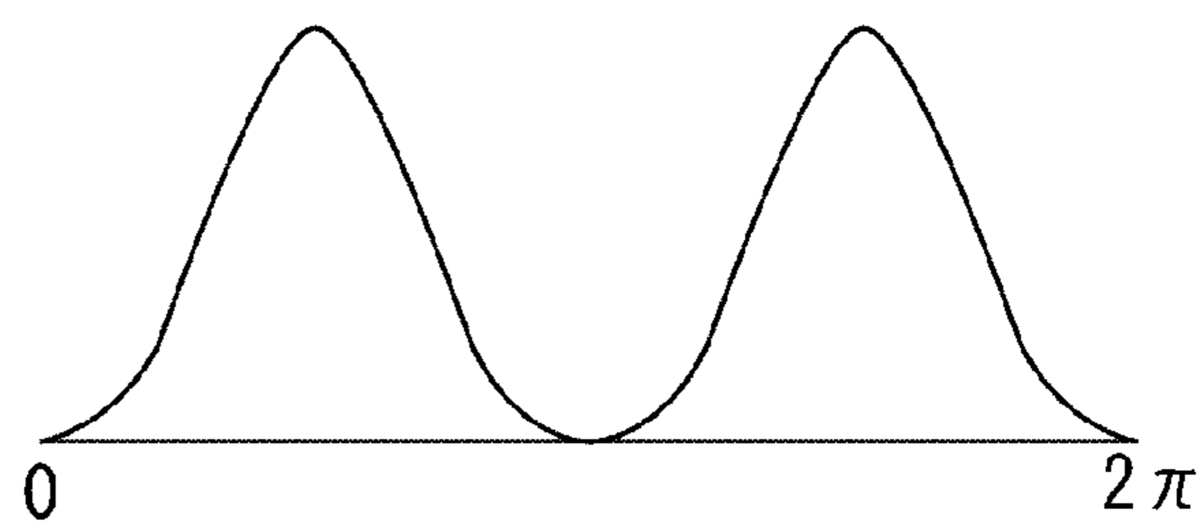
Blackman Window
