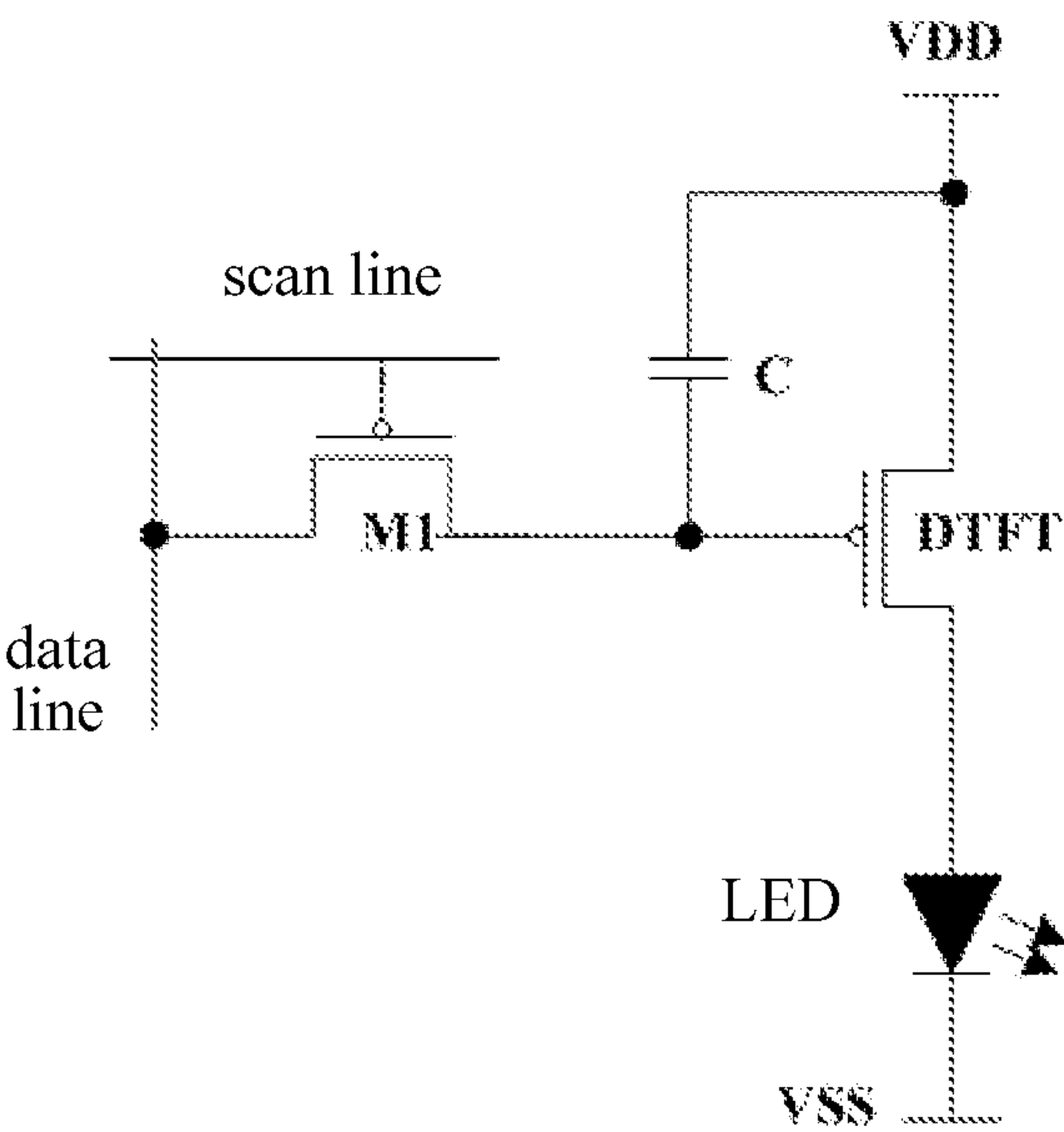
Fig.1 - PRIOR ART
