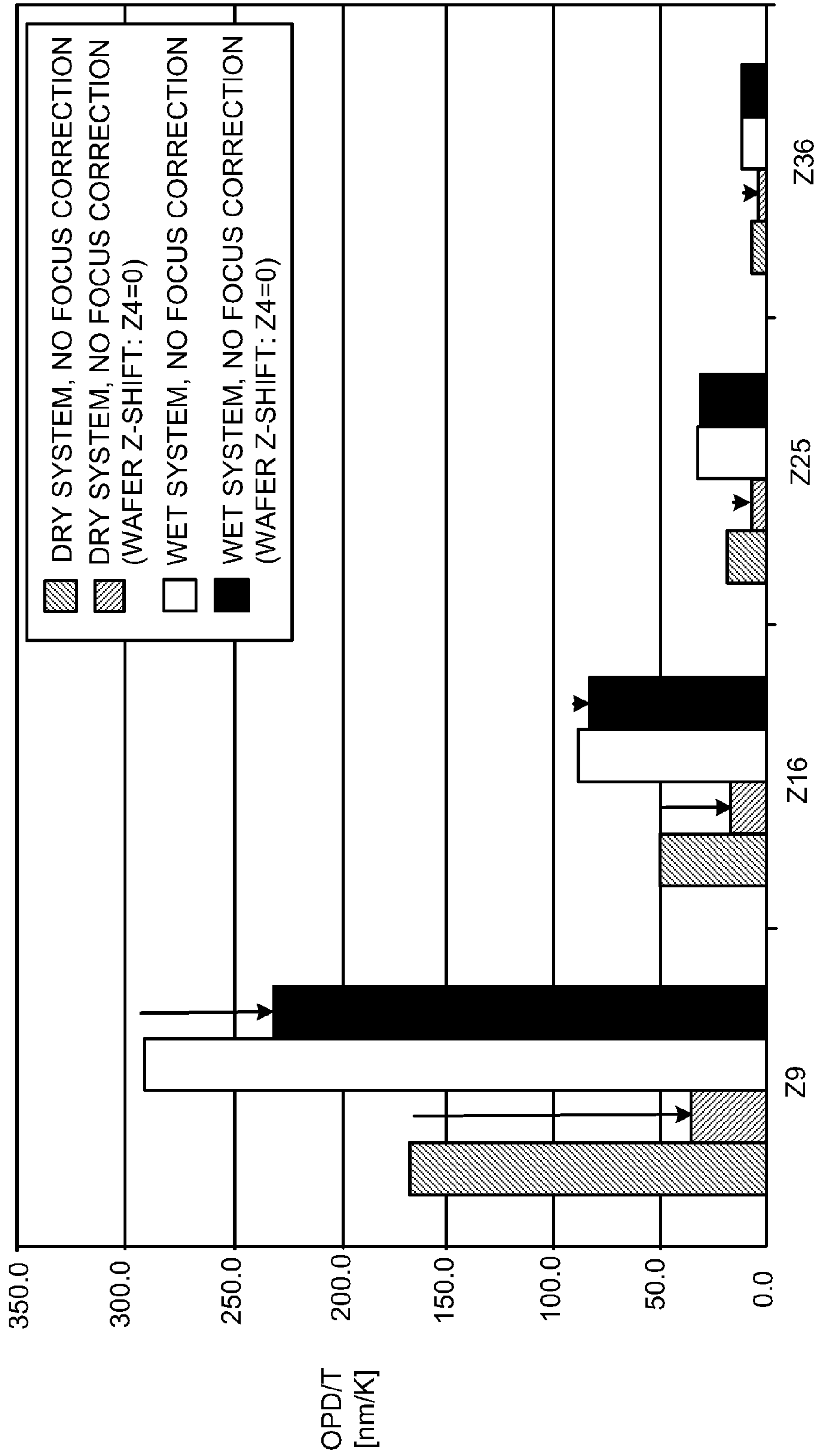
HIGHER SPHERICAL ZERNIKE COEFFICIENTS
