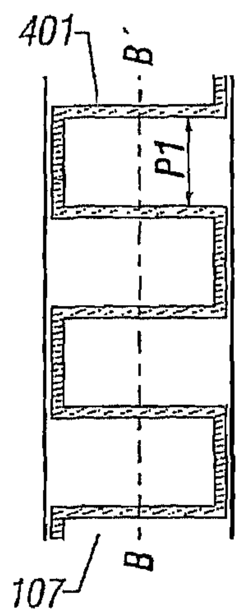
SIGNAL LINE DRIVE CIRCUIT SIDE REGION R1
