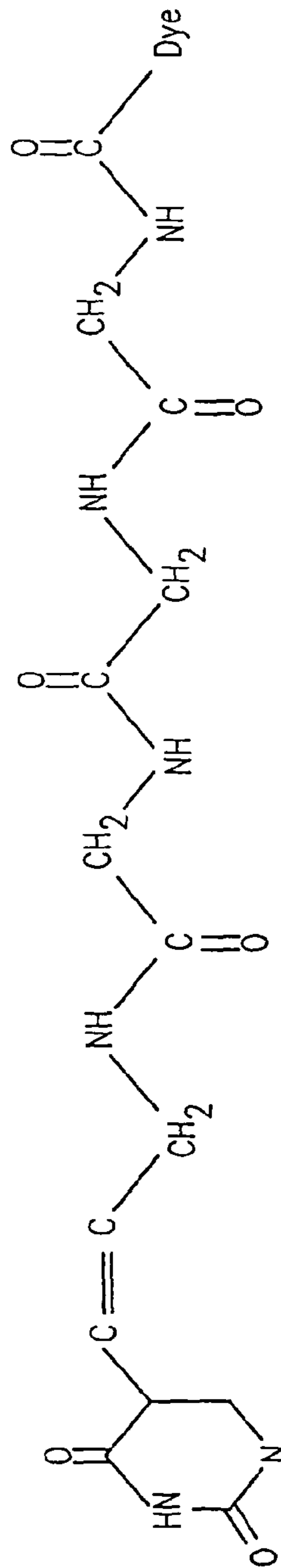
Tetraglycinylnyl linker
