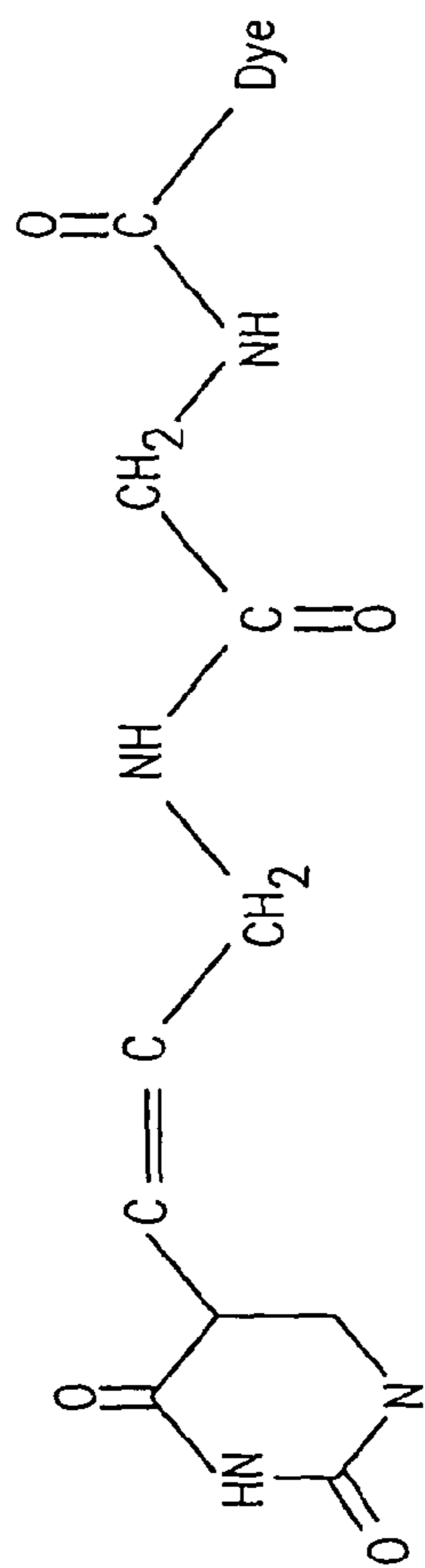
Diglycinylnyl linker
