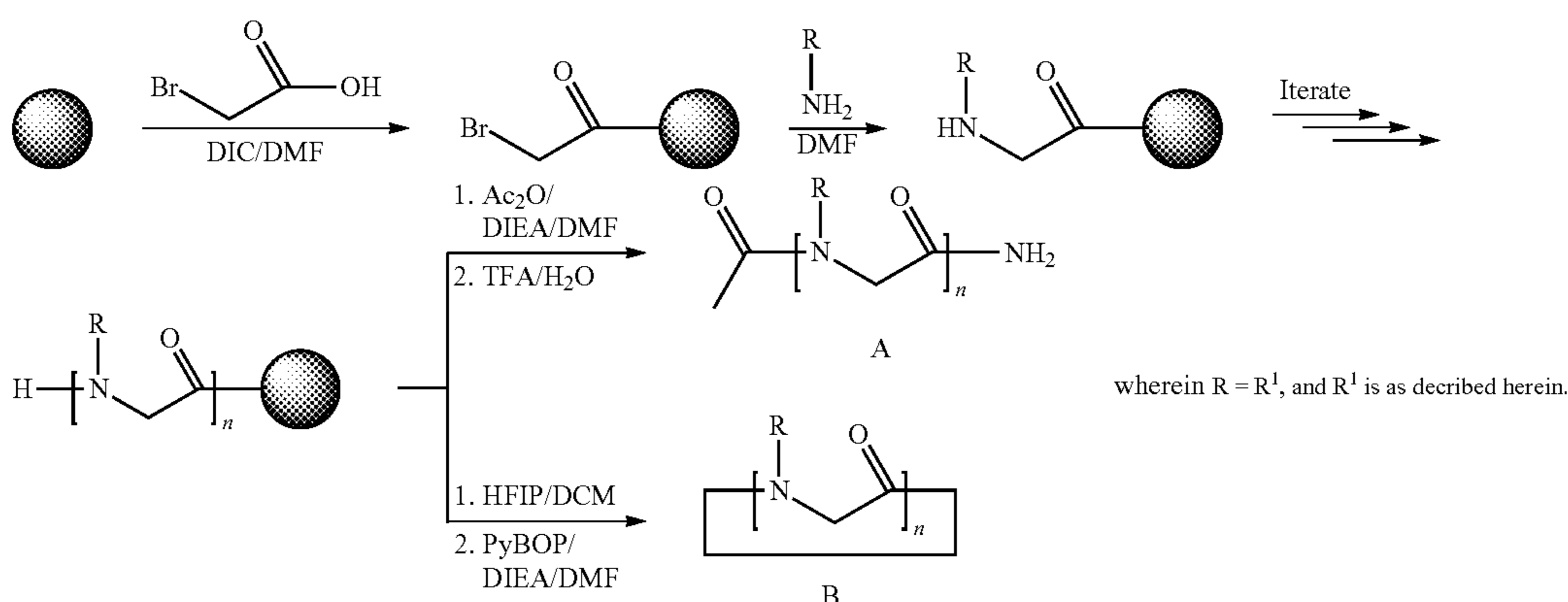
Scheme 1: Synthesis (A) N-acetylated linear peptoid oligomers and (B) cyclic peptoid oligomers.
