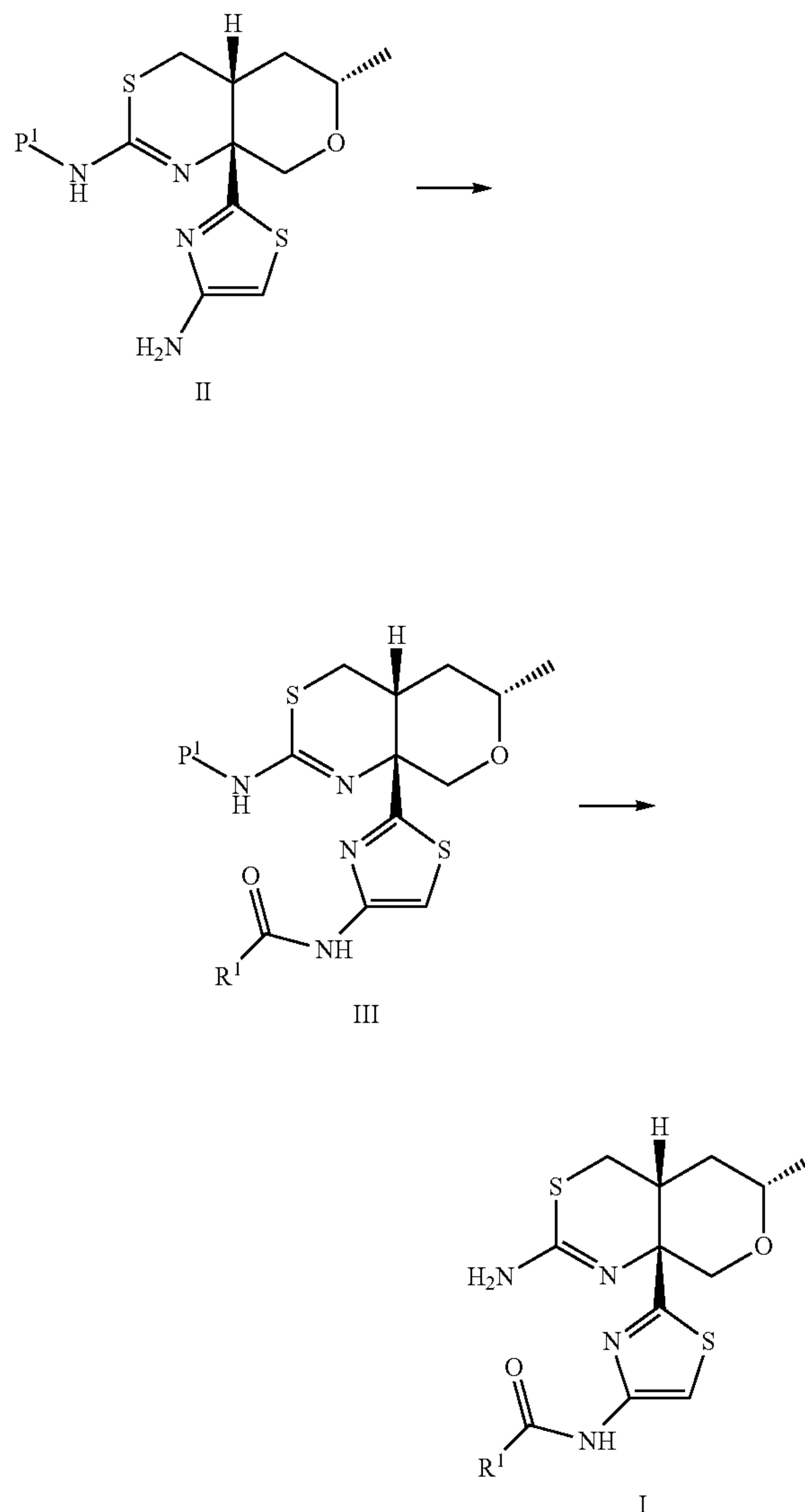
Scheme 1
