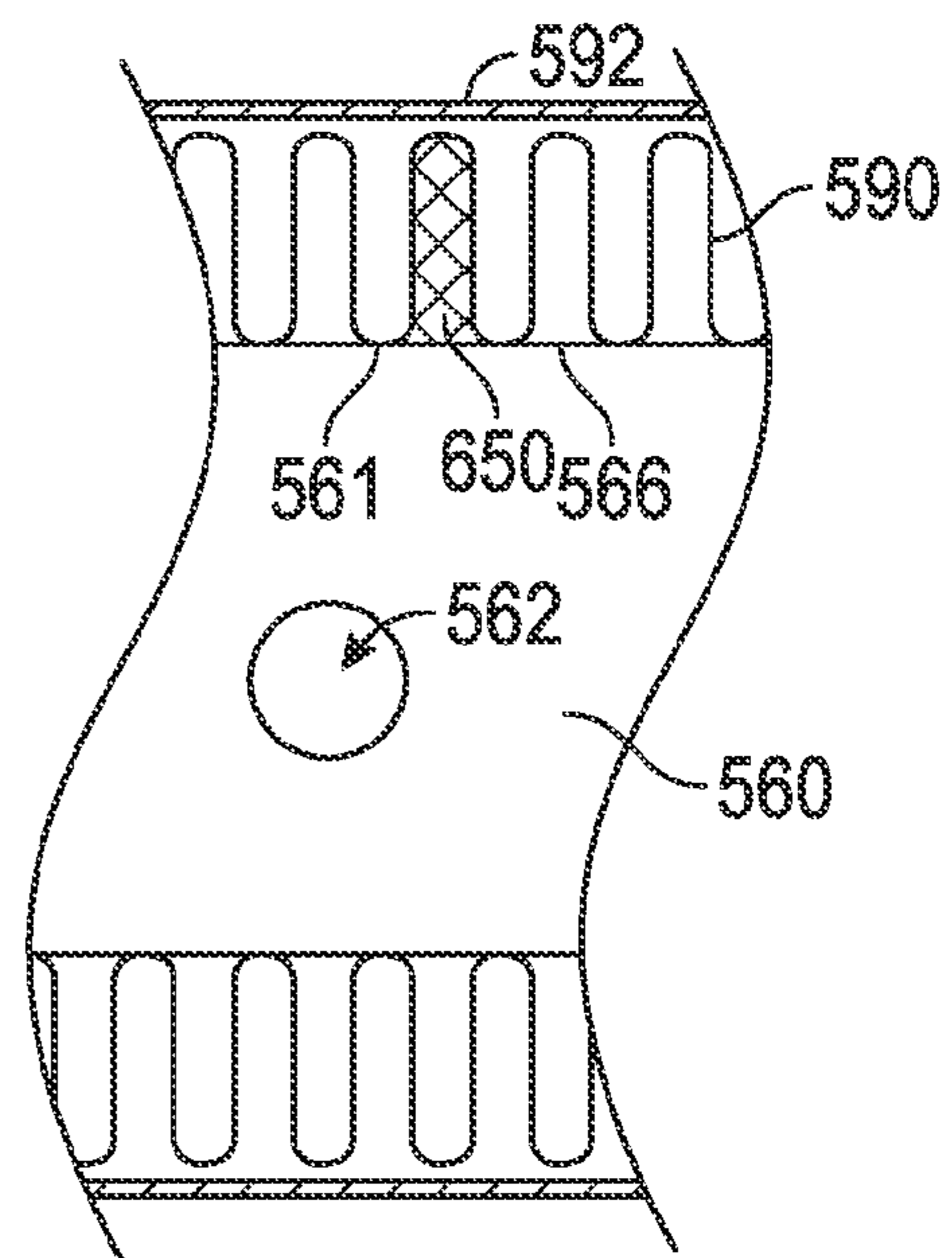
FIG. 12C (Section H-H)
