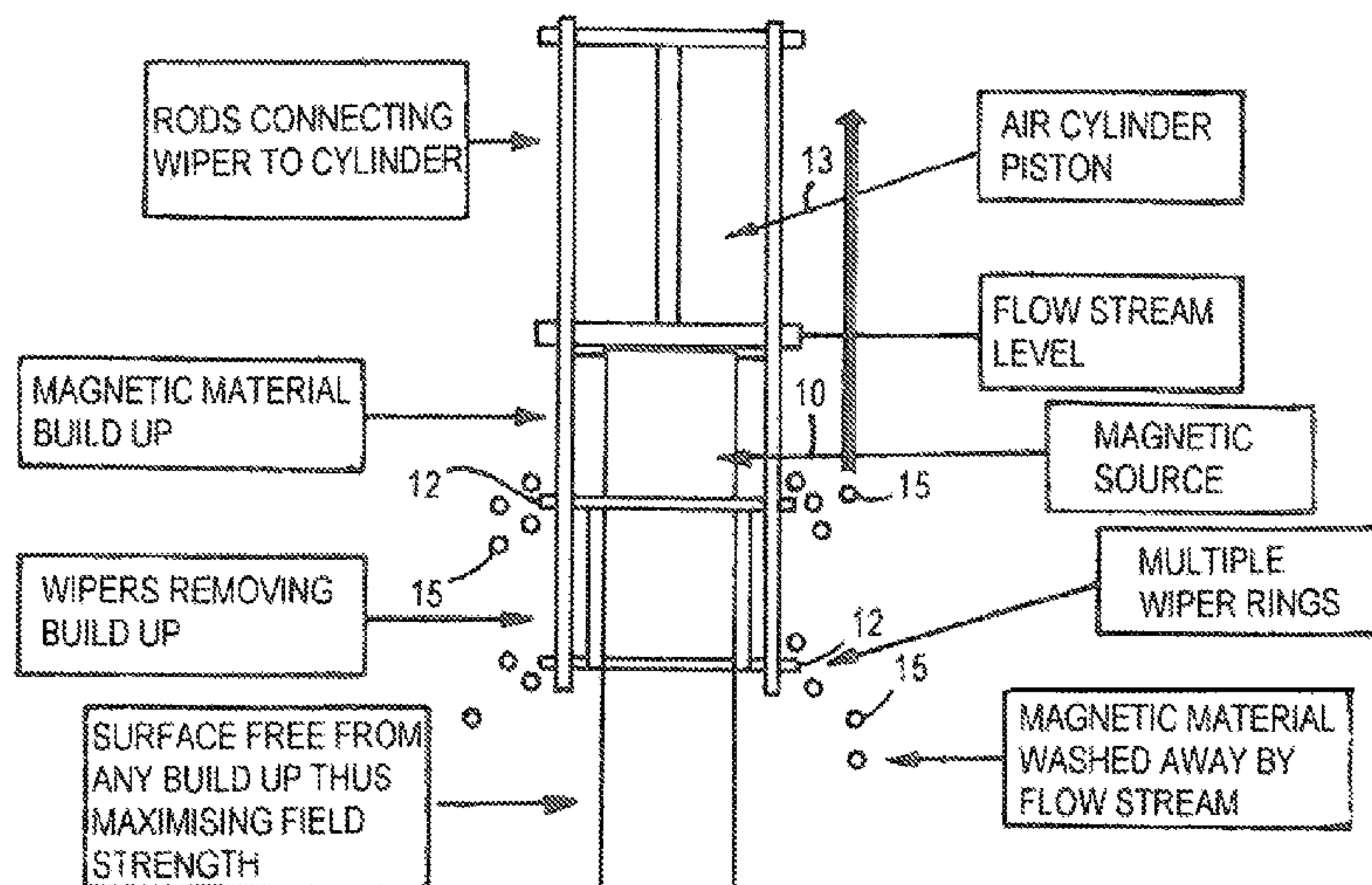
SLURRY MAGNETISING EQUIPMENT
