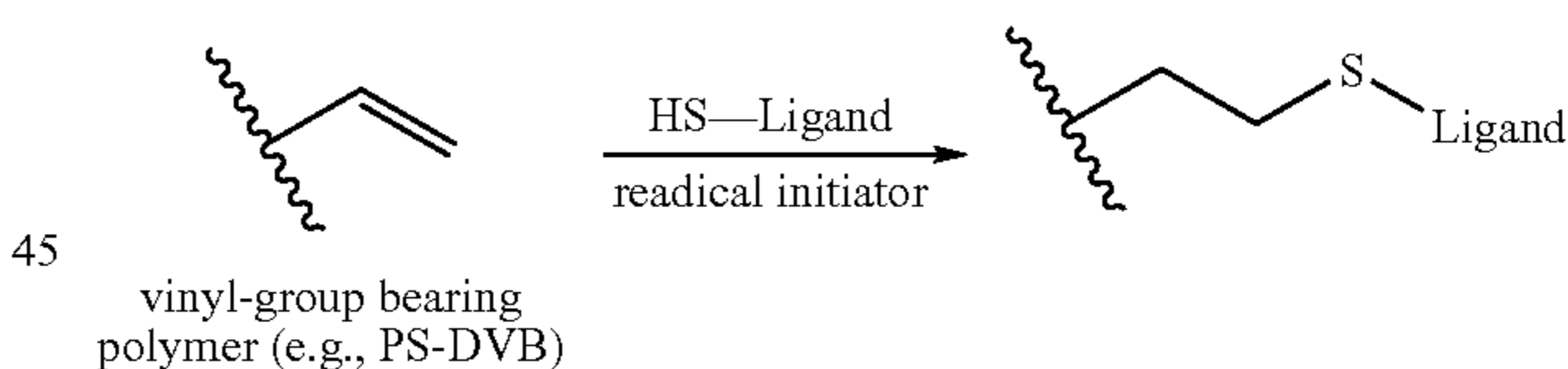
Scheme 1:
