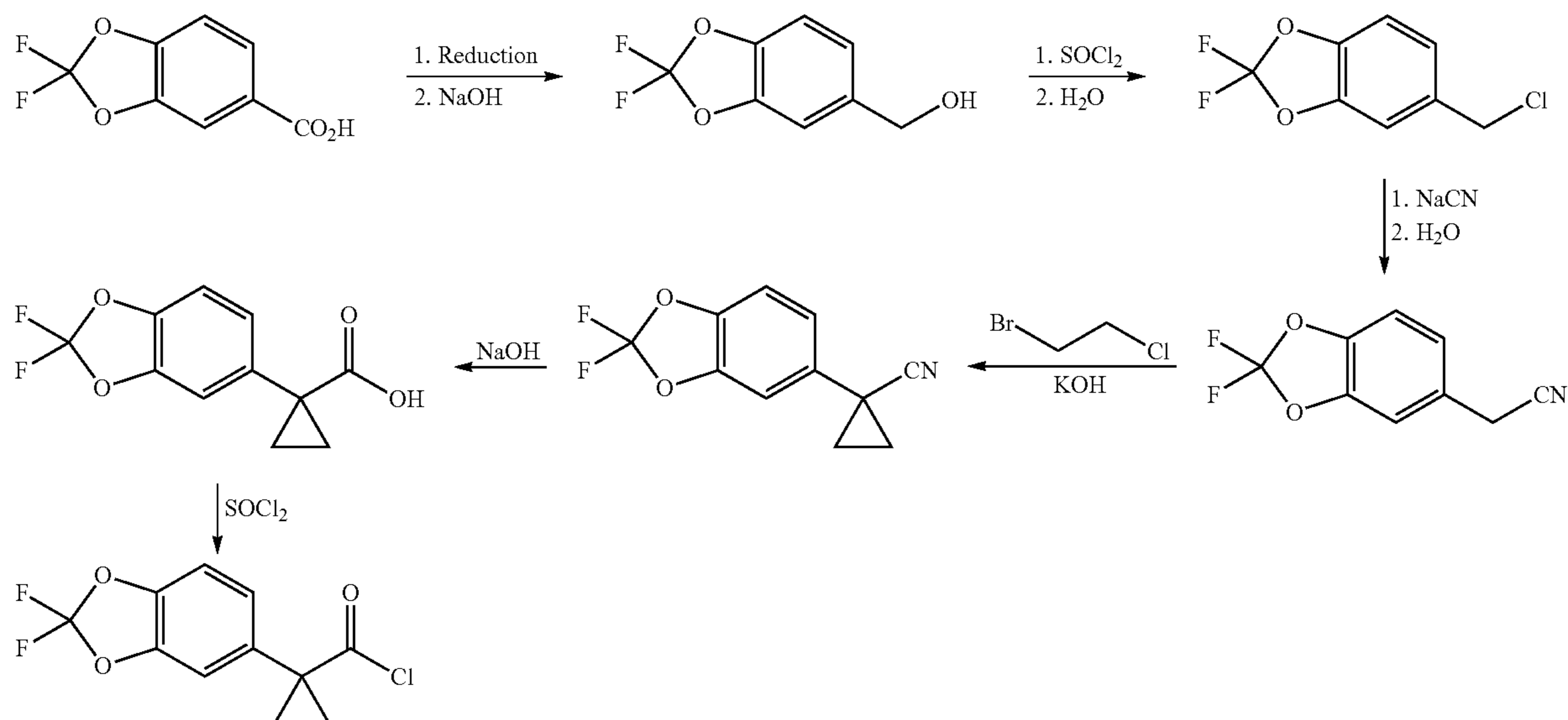
Scheme 1. Synthesis of the acid chloride used to prepare Compound 1.
