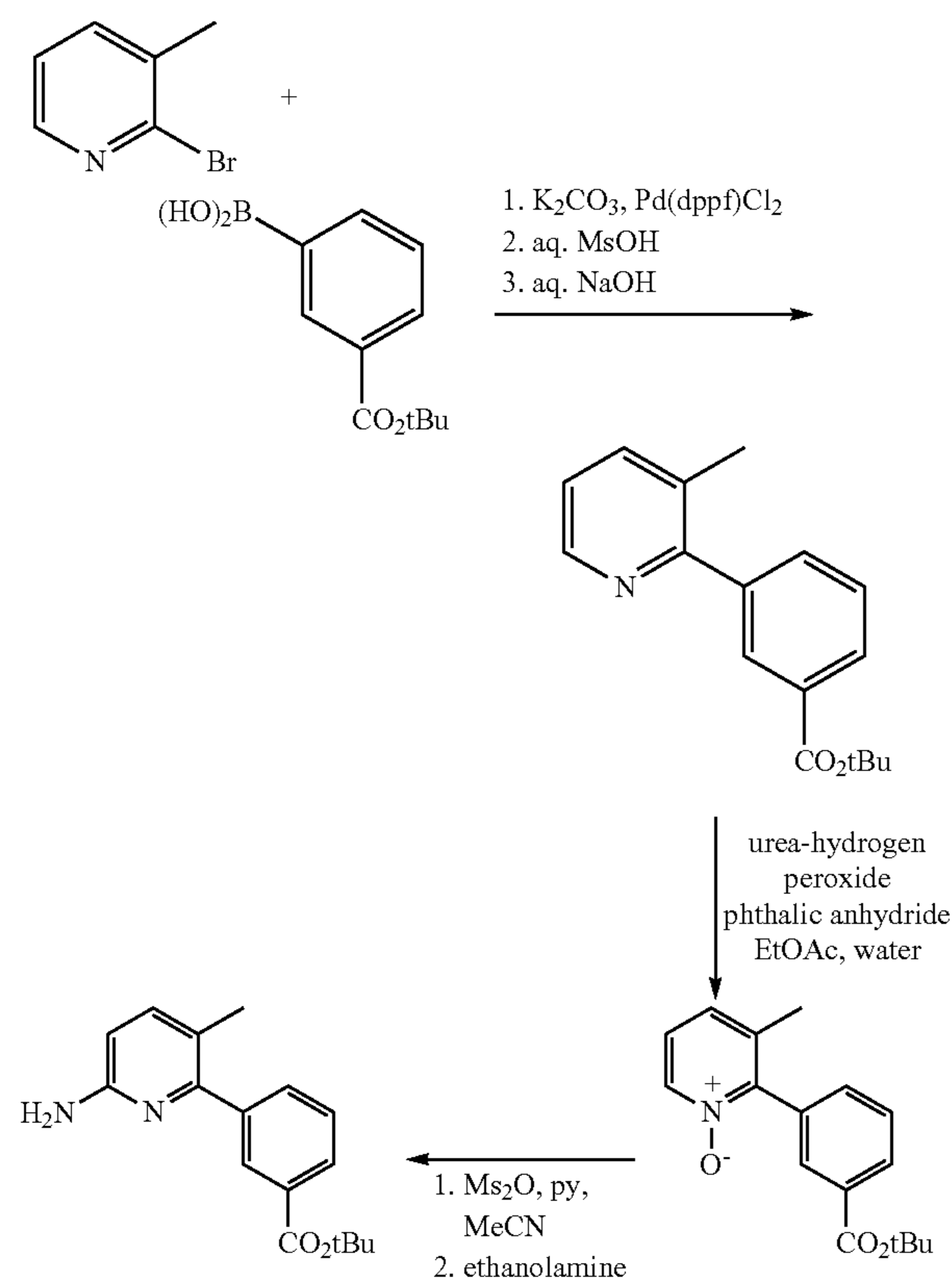
Scheme 3. Synthesis of the amine used to prepare Compound 1.
